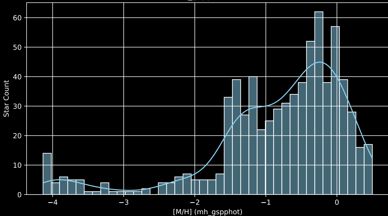
Gaia Cluster: [NGC_6451 [M/H] (mh_gspphot) (n= 716)
