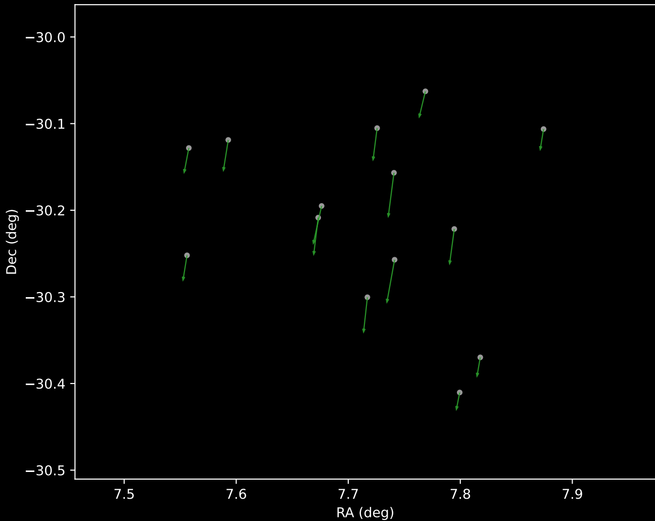
Gaia DR3 Cluster 24 Proper Motion Vectors (n=14)
