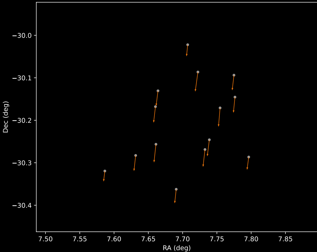
Gaia DR3 Cluster 42 Proper Motion Vectors (n=14)
