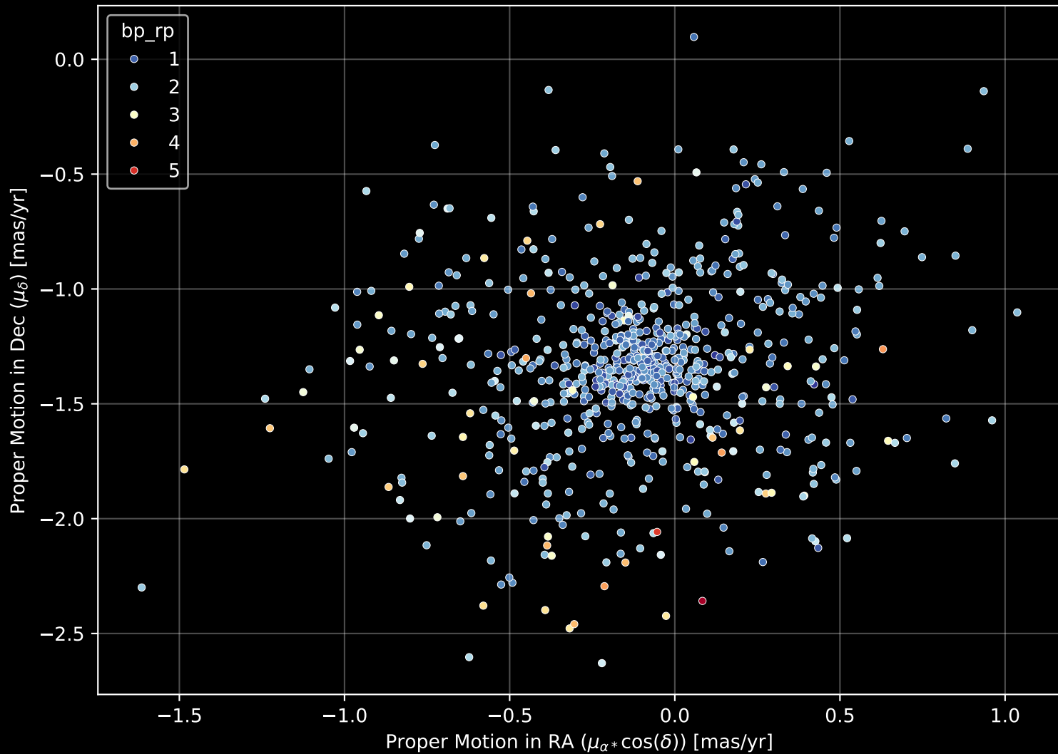
Gaia Cluster: [NGC_6451] Proper Motion Diagram (n= 752)
