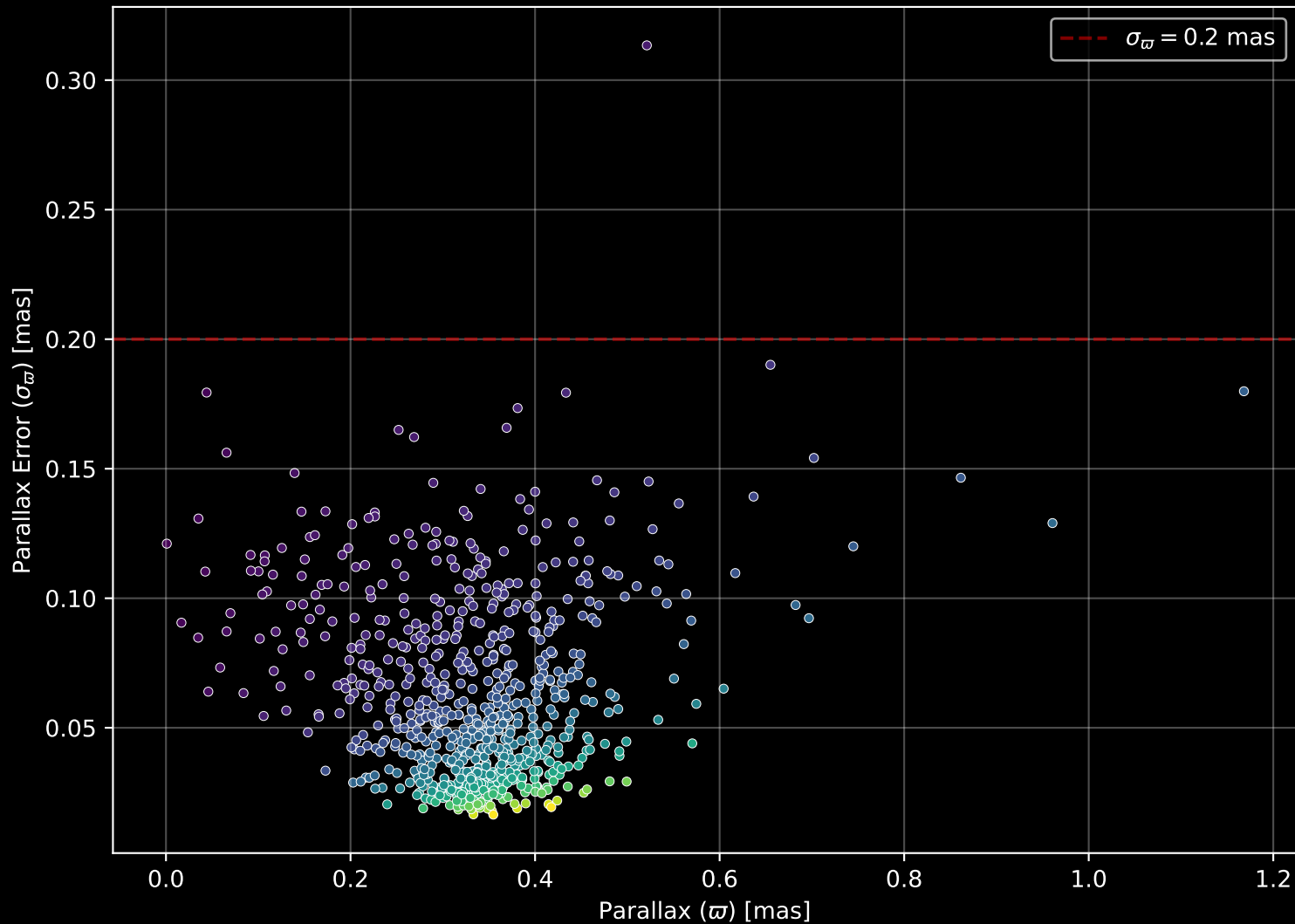
Gaia Cluster: [NGC_6451] Parallax Quality (n= 752)
