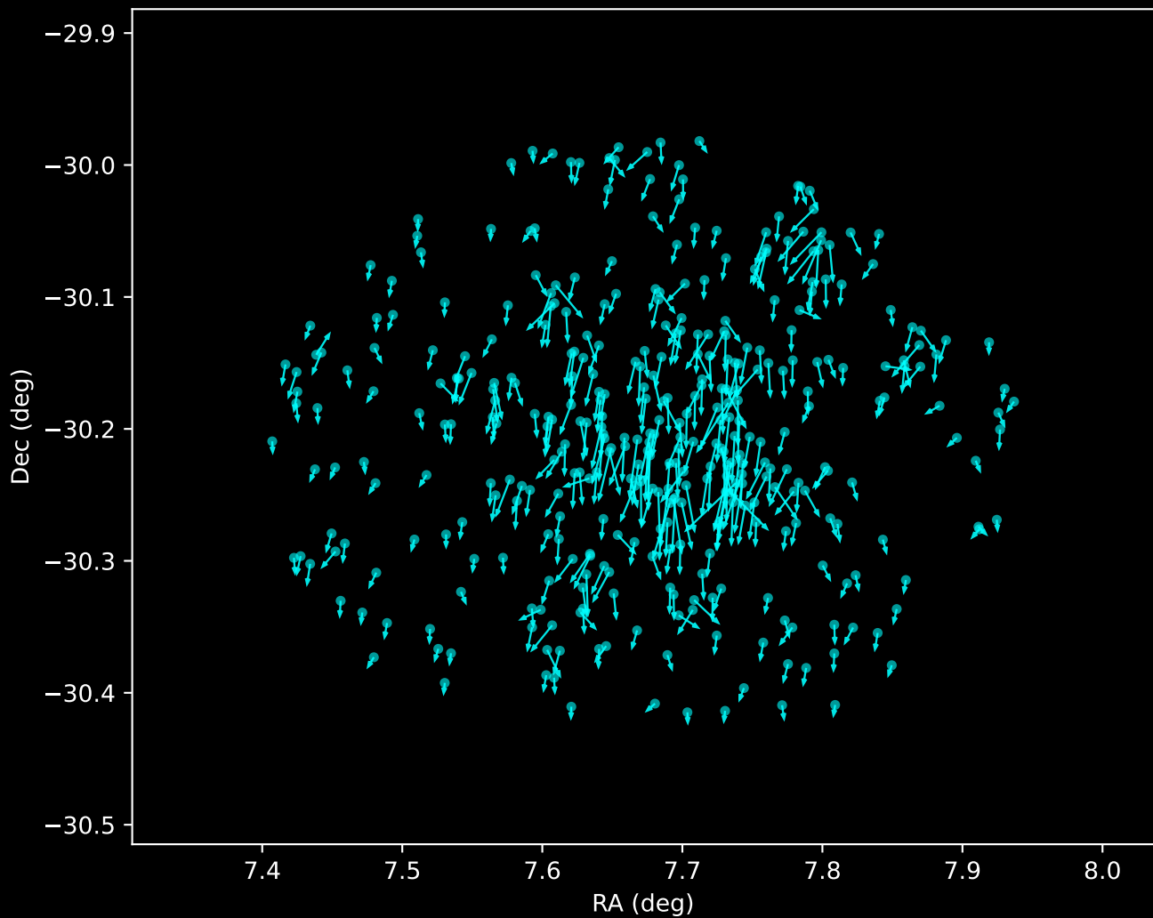
Gaia DR3 Noise Stream Proper Motion Vectors (n=374)
