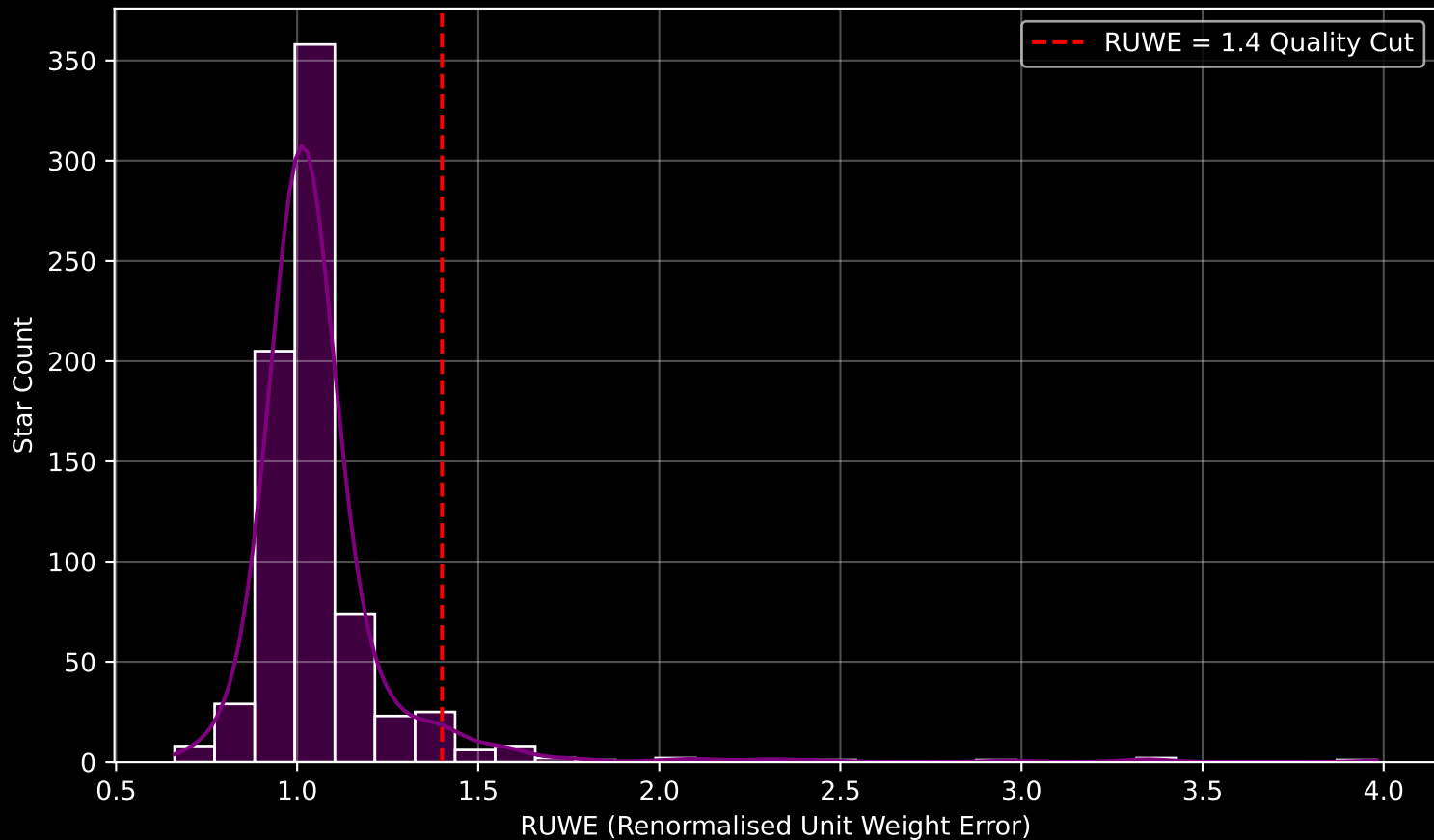
Gaia Cluster: [NGC_6451] RUWE Distribution (n= 749)
