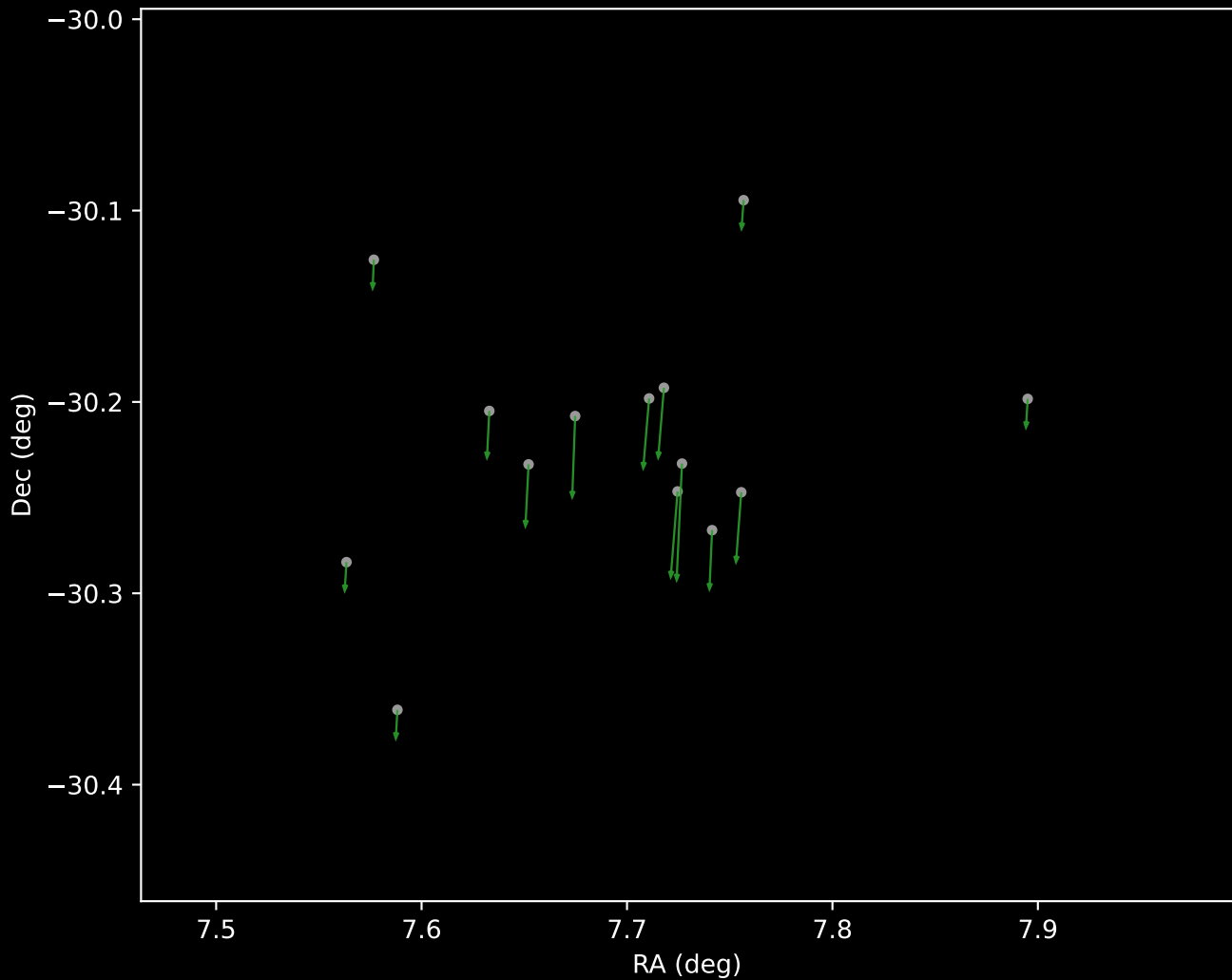
Gaia DR3 Cluster 44 Proper Motion Vectors (n=14)
