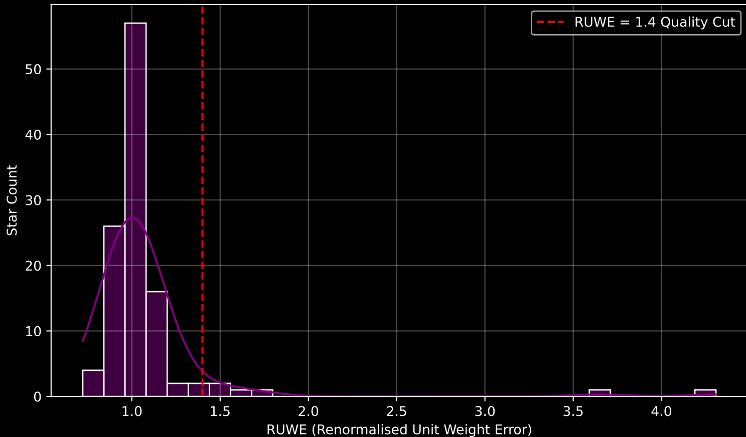
Gaia Cluster: [NGC_6469] RUWE Distribution (n= 113)
