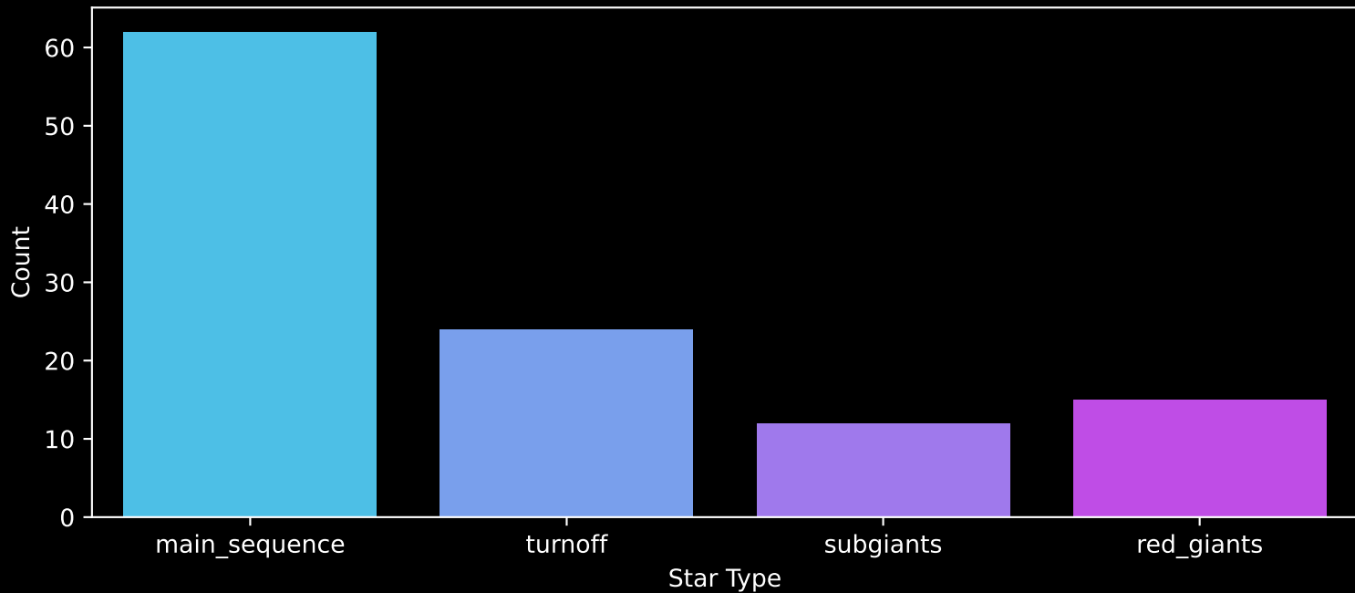
Gaia Cluster: [NGC_6469] Count plot of Star Type
