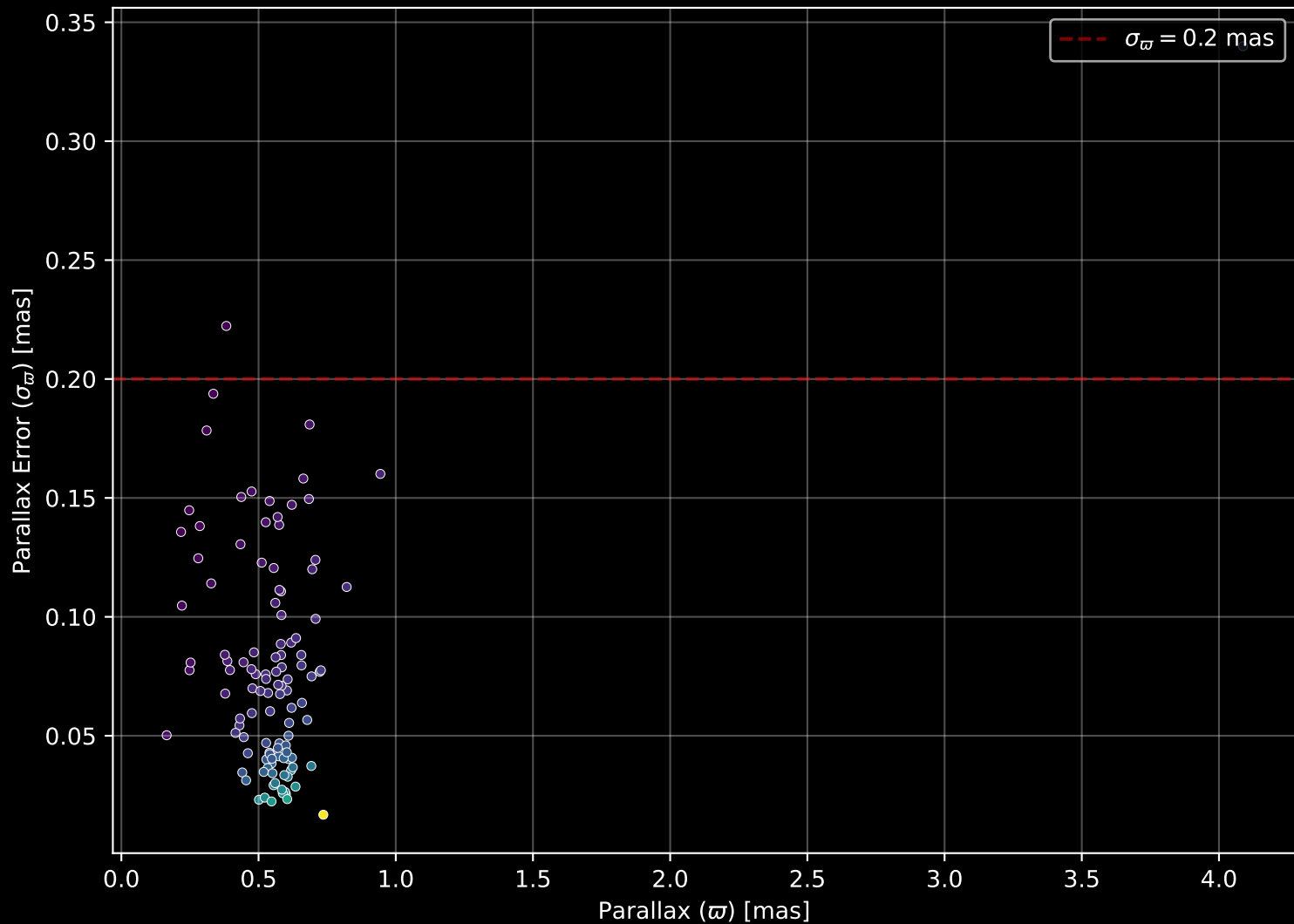
Gaia Cluster: [NGC_6469] Parallax Quality (n= 113)
