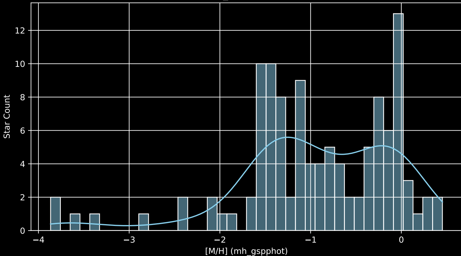
Gaia Cluster: [NGC_6469 [M/H] (mh_gspphot) (n= 113)
