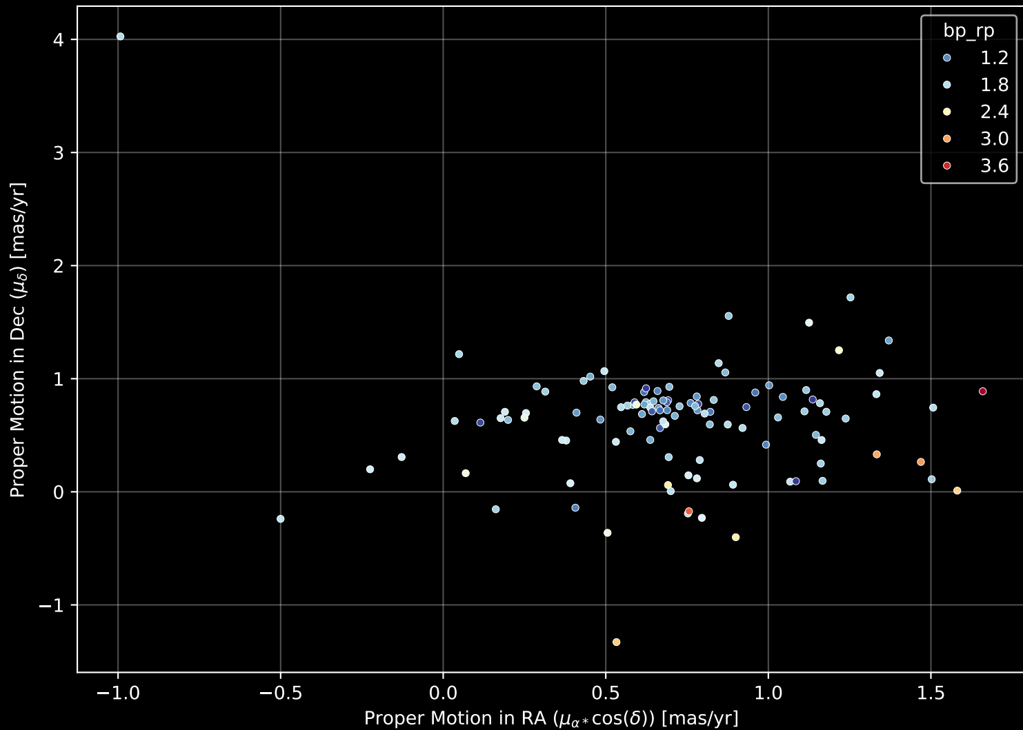
Gaia Cluster: [NGC_6469] Proper Motion Diagram (n= 113)
