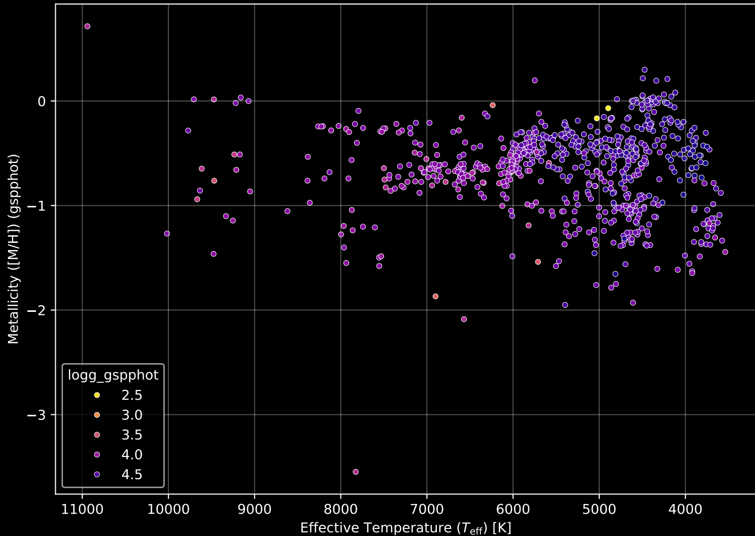
Gaia Cluster: [NGC_6494] Stellar Population Parameters (n= 713)
