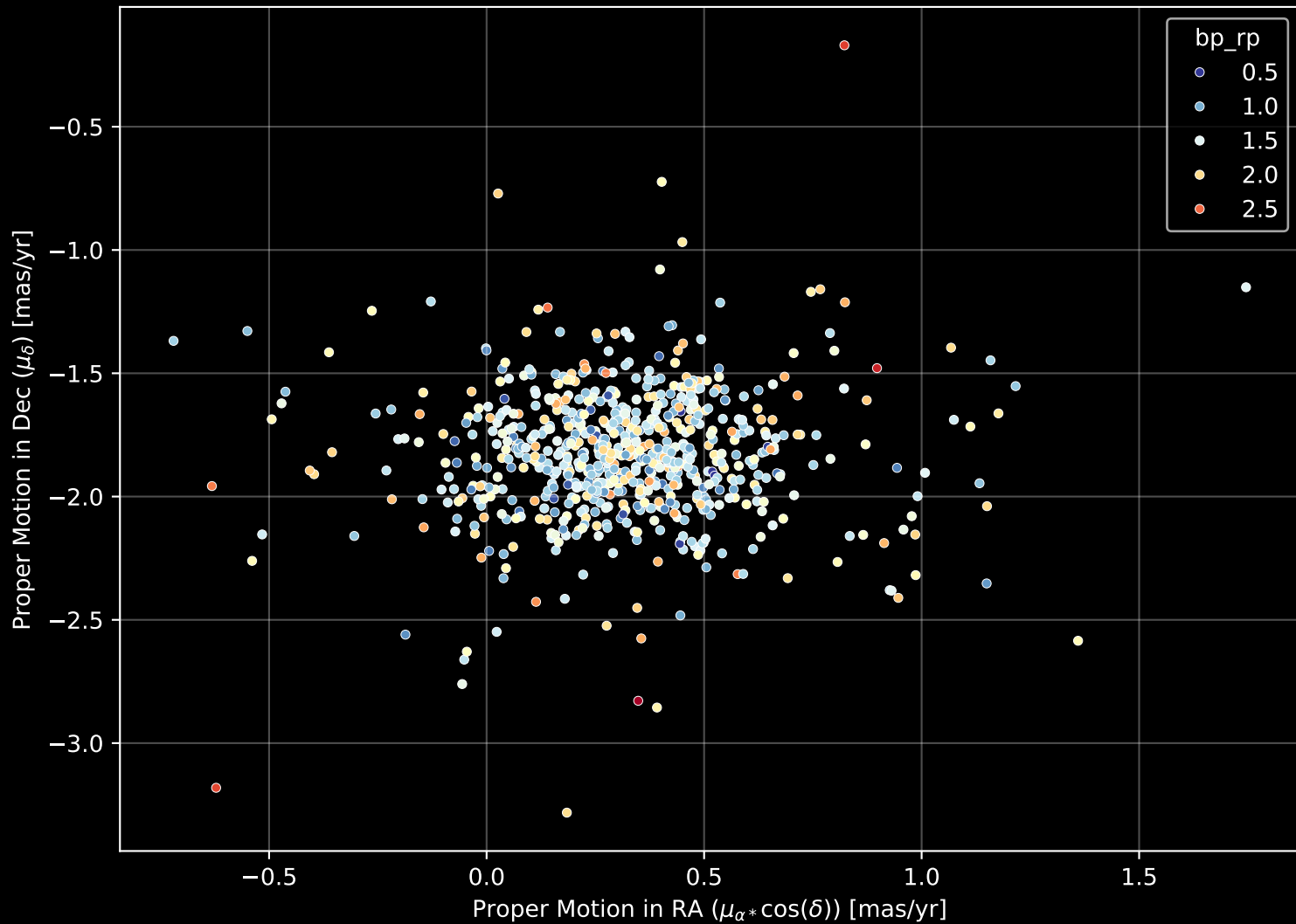
Gaia Cluster: [NGC_6494] Proper Motion Diagram (n= 713)
