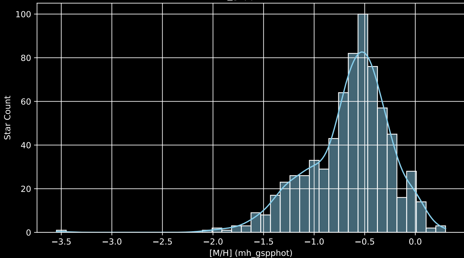
Gaia Cluster: [NGC_6494 [M/H] (mh_gspphot) (n= 712)
