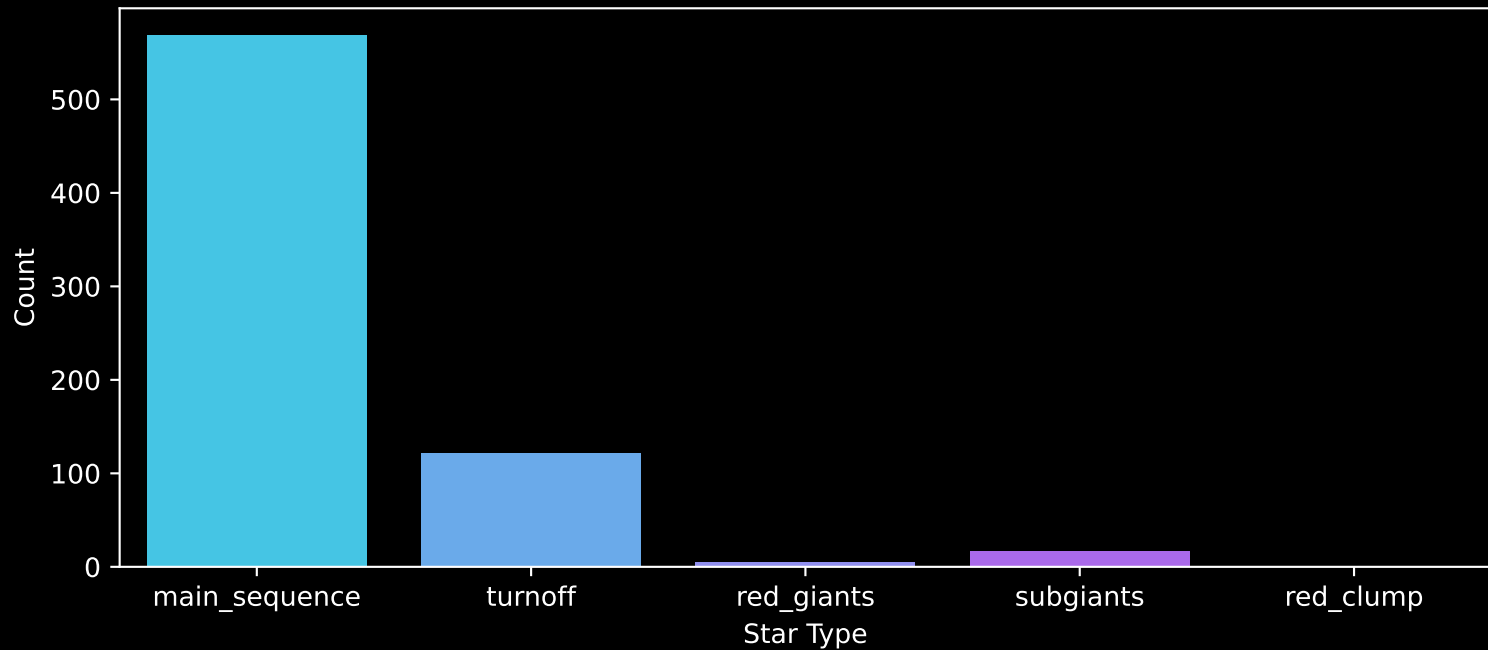
Gaia Cluster: [NGC_6494] Count plot of Star Type
