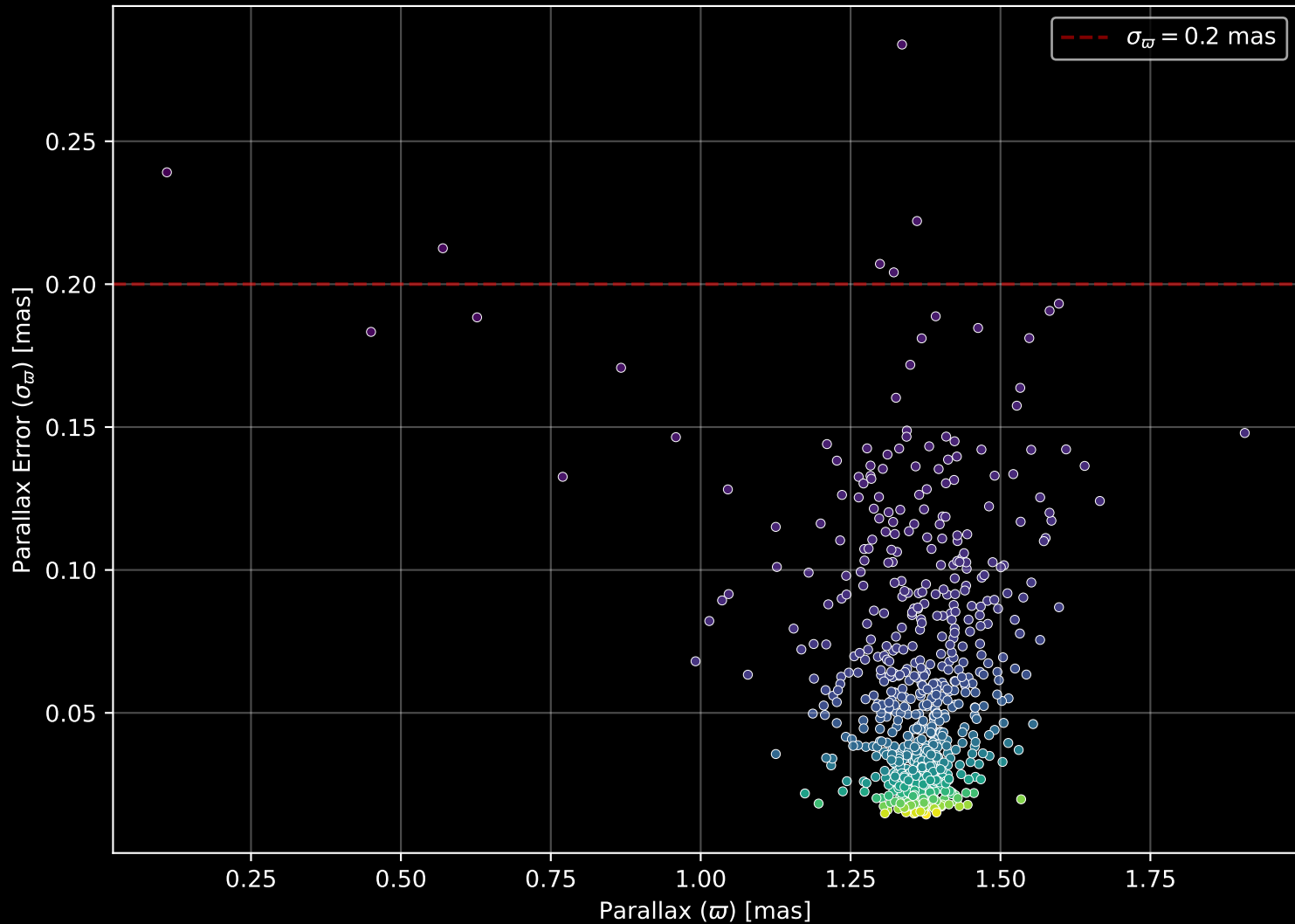
Gaia Cluster: [NGC_6494] Parallax Quality (n= 713)
