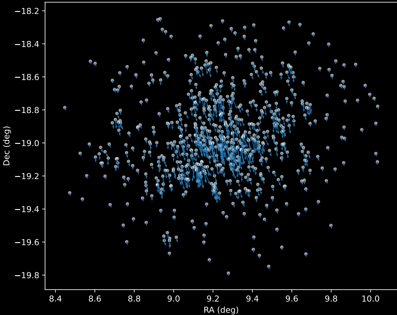
Gaia DR3 Cluster 0 Proper Motion Vectors (n=646)
