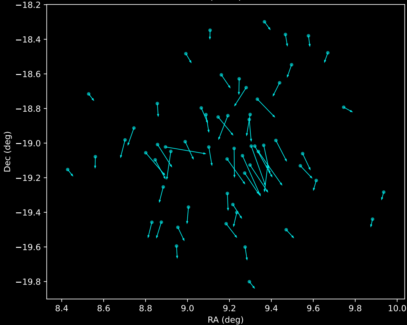
Gaia DR3 Noise Stream Proper Motion Vectors (n=61)
