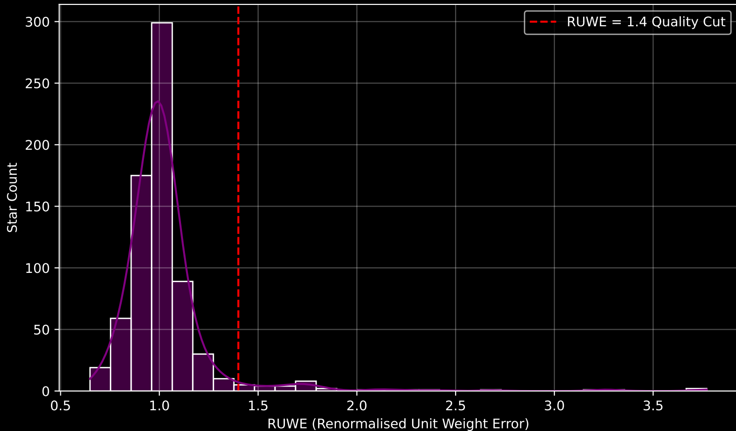
Gaia Cluster: [NGC_6494] RUWE Distribution (n= 713)
