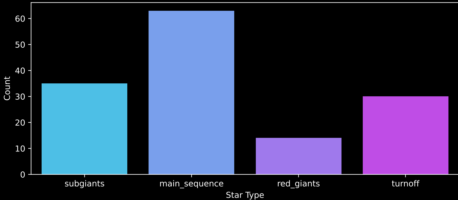
Gaia Cluster: [NGC_6520] Count plot of Star Type
