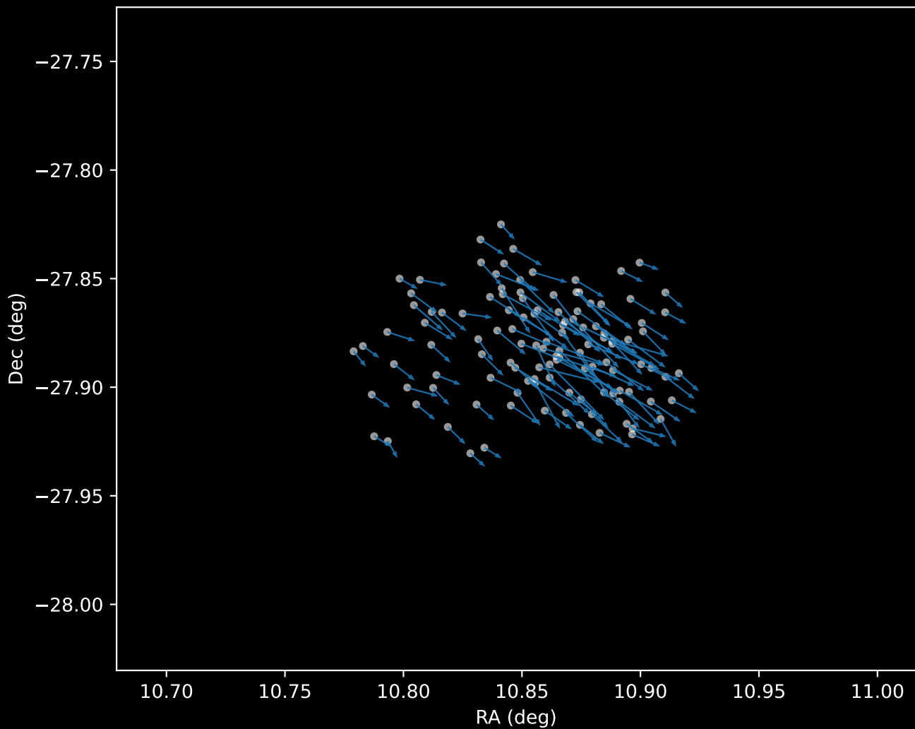
Gaia DR3 Cluster 0 Proper Motion Vectors (n=118)
