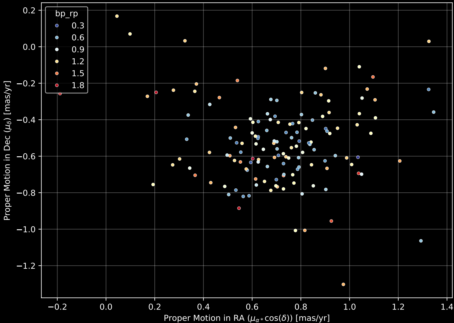
Gaia Cluster: [NGC_6520] Proper Motion Diagram (n= 142)
