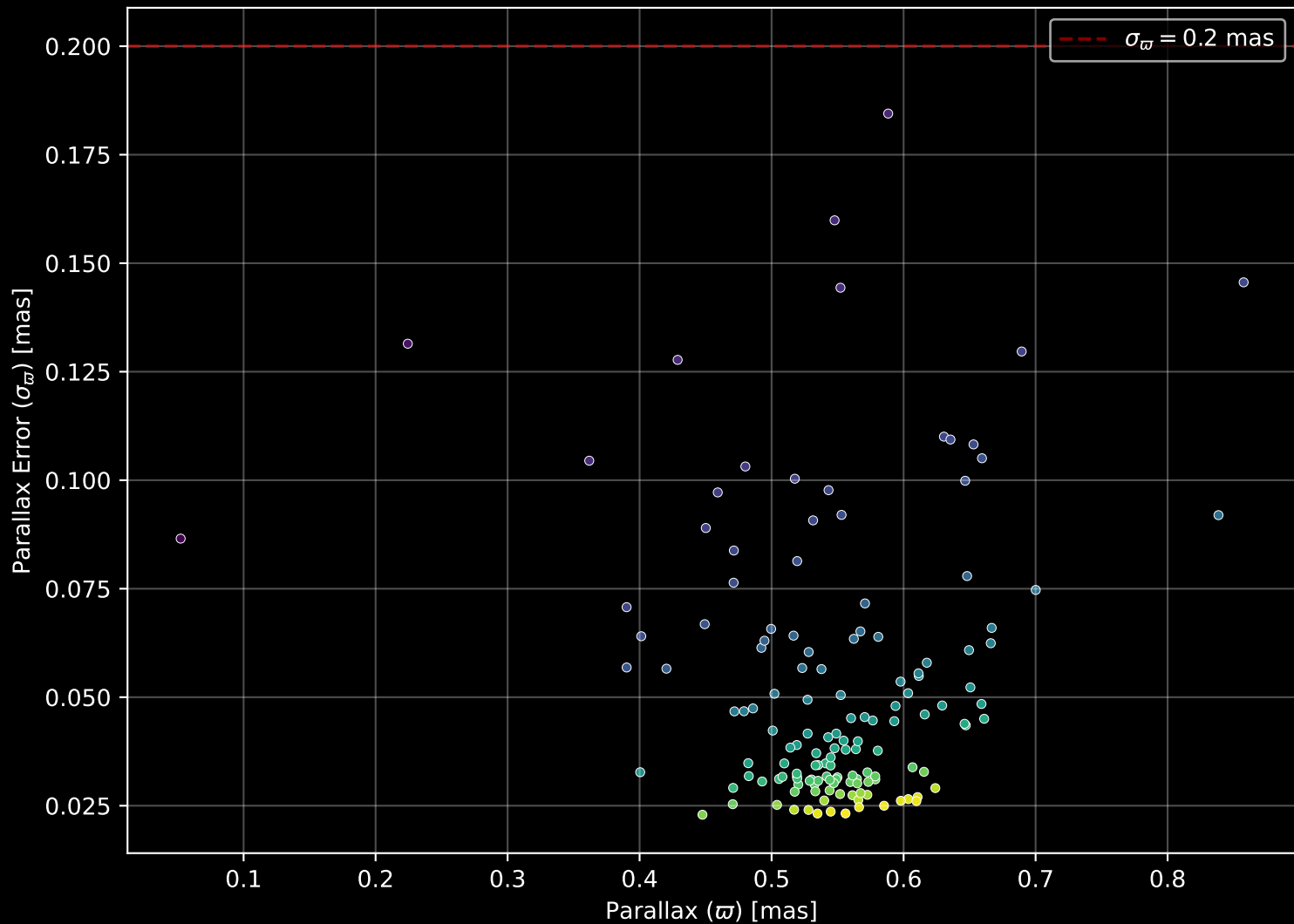
Gaia Cluster: [NGC_6520] Parallax Quality (n= 142)
