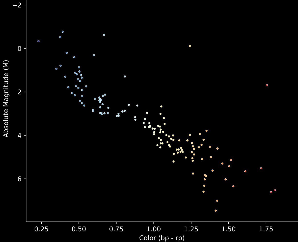
Gaia Cluster: [NGC_6520] Stars (n= 142) Hertzsprung-Russel Diagram
