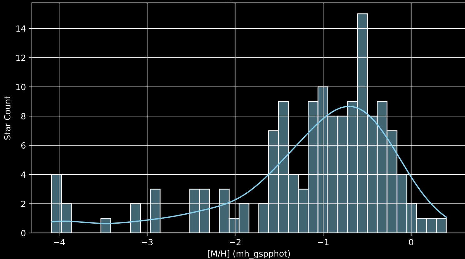
Gaia Cluster: [NGC_6520 [M/H] (mh_gspphot) (n= 141)
