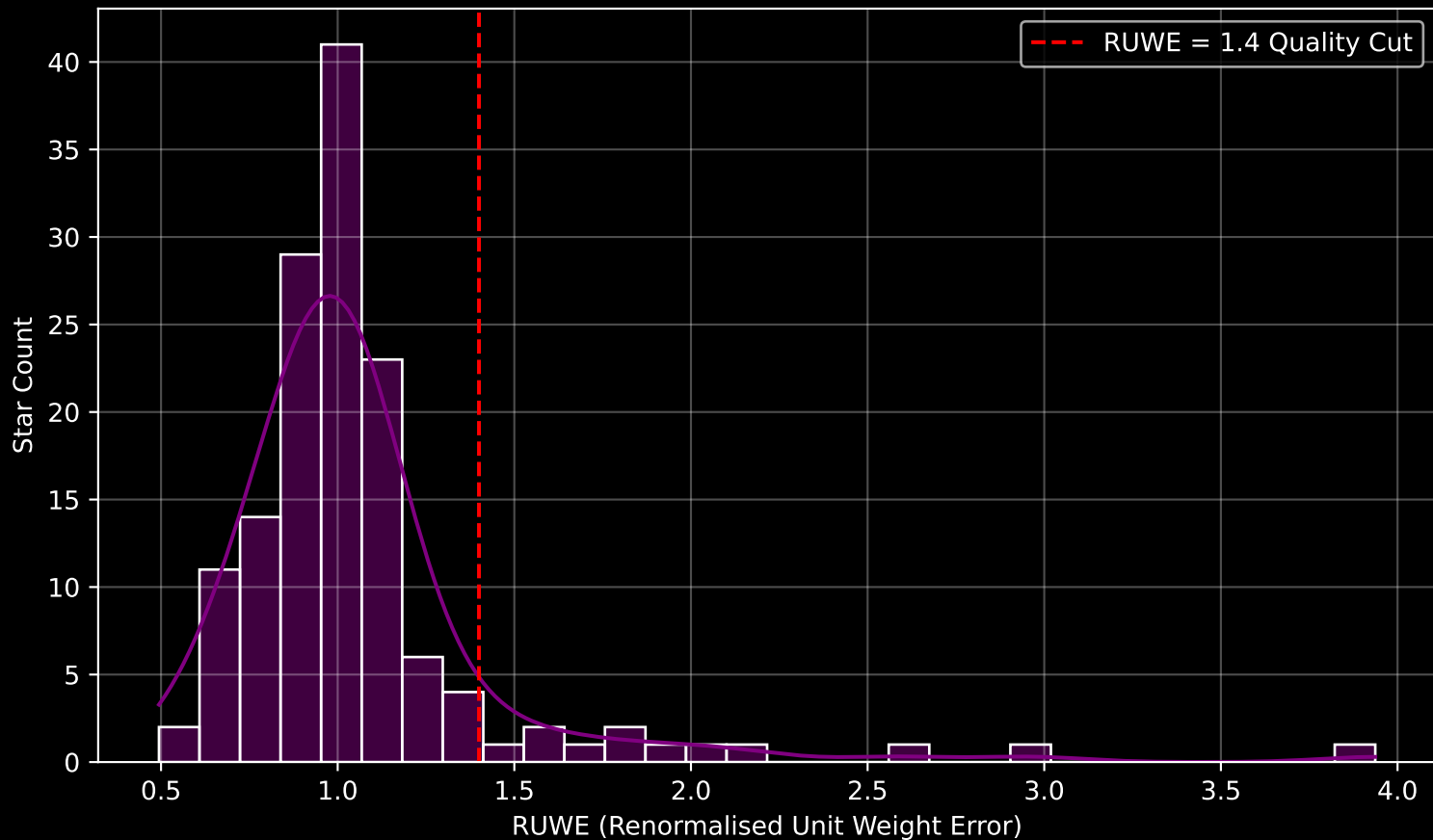
Gaia Cluster: [NGC_6520] RUWE Distribution (n= 142)
