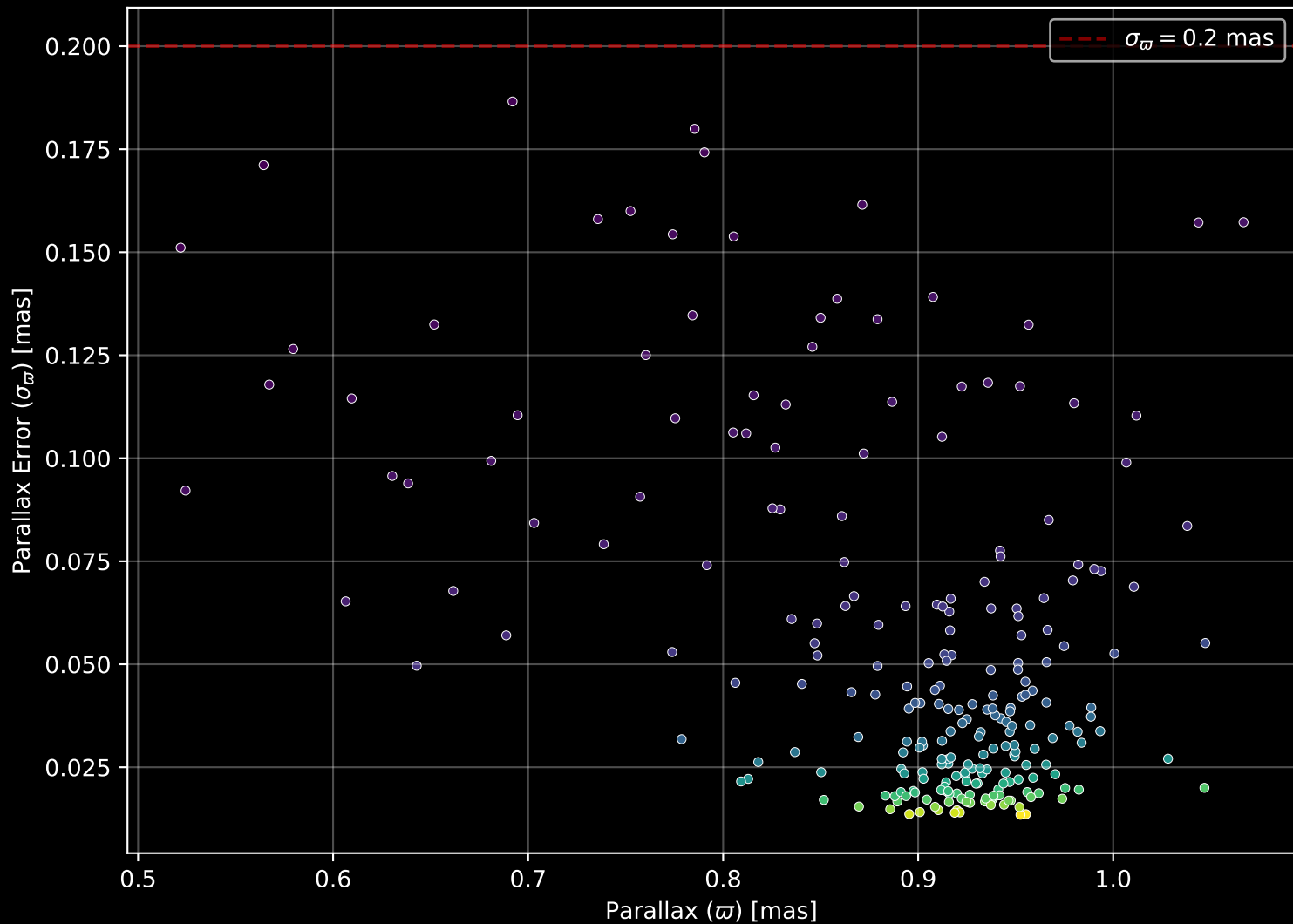
Gaia Cluster: [NGC_6568] Parallax Quality (n= 243)
