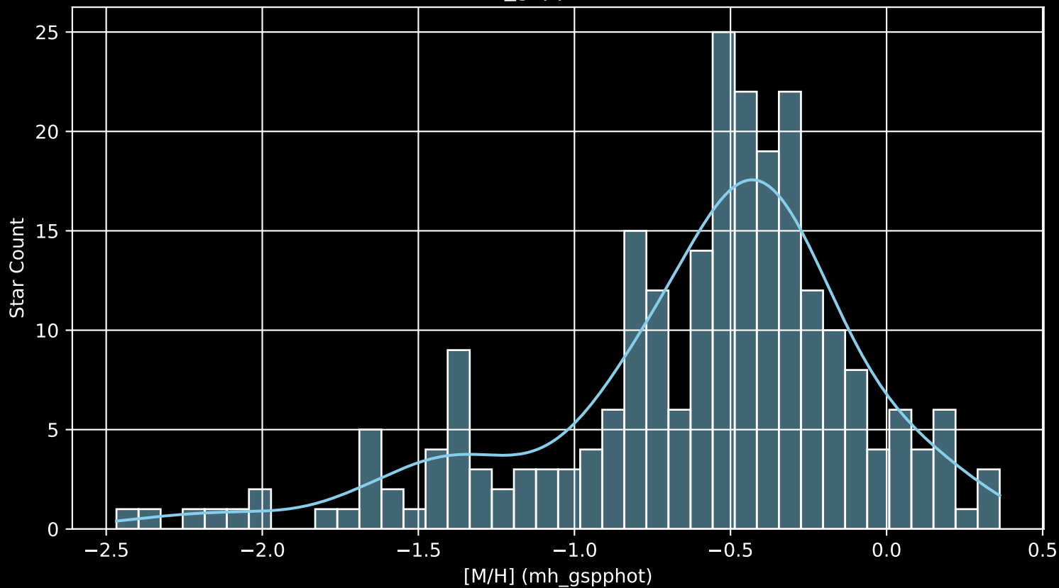
Gaia Cluster: [NGC_6568 [M/H] (mh_gspphot) (n= 243)
