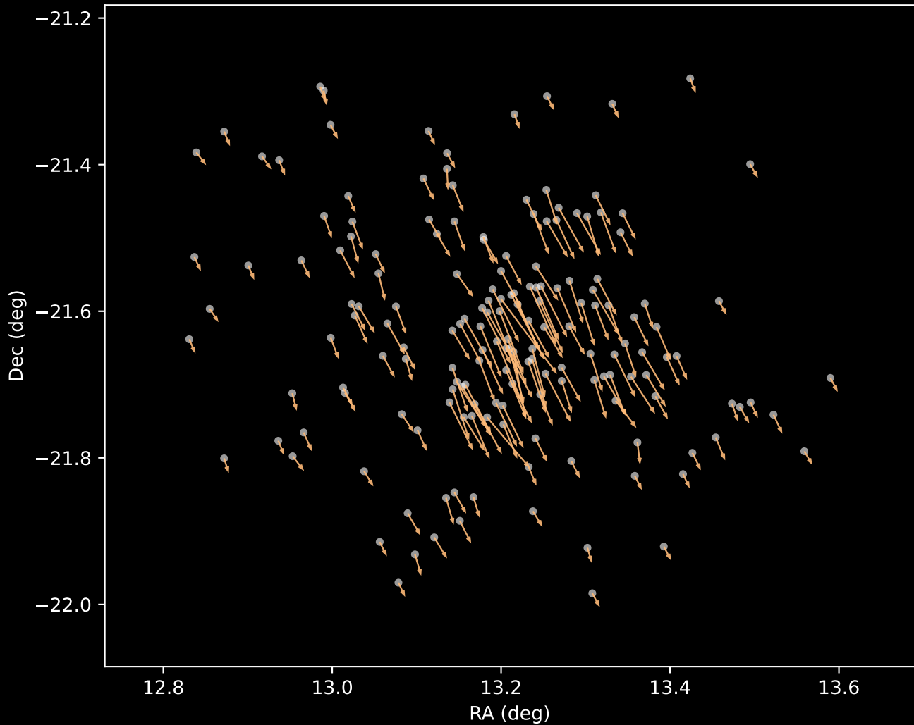
Gaia DR3 Cluster 3 Proper Motion Vectors (n=169)
