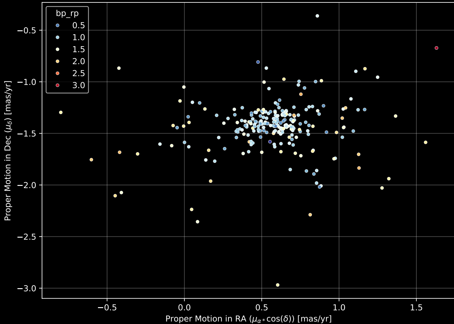
Gaia Cluster: [NGC_6568] Proper Motion Diagram (n= 243)
