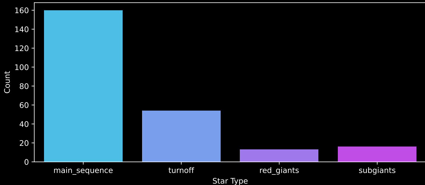
Gaia Cluster: [NGC_6568] Count plot of Star Type
