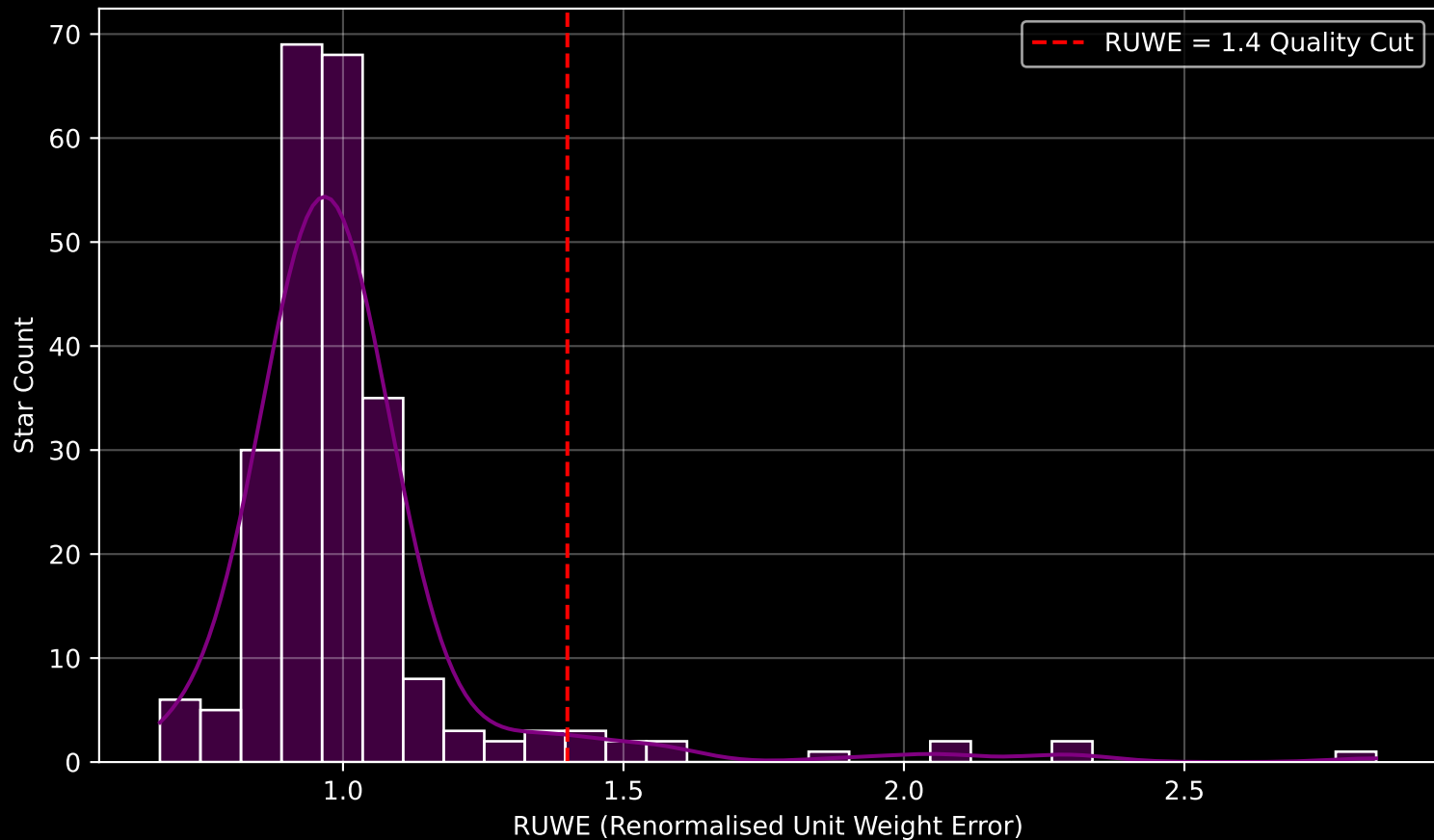
Gaia Cluster: [NGC_6568] RUWE Distribution (n= 242)
