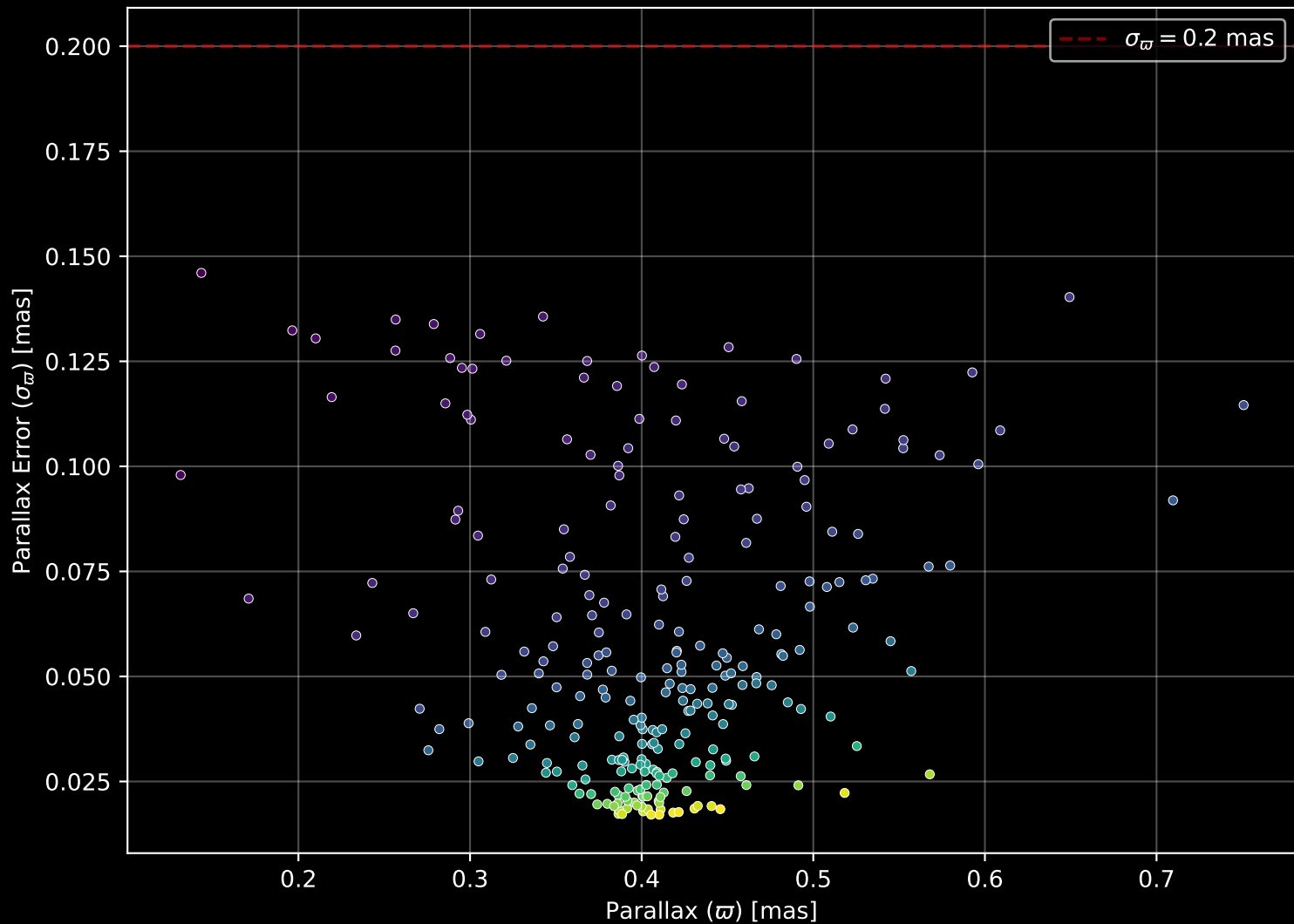
Gaia Cluster: [NGC_6583] Parallax Quality (n= 255)
