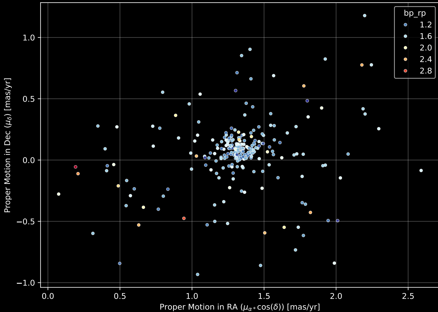
Gaia Cluster: [NGC_6583] Proper Motion Diagram (n= 255)
