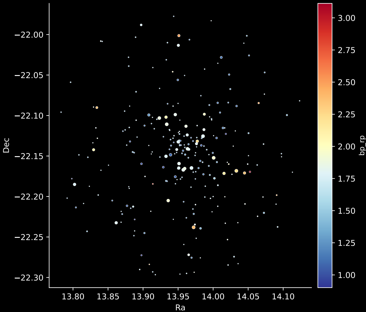
Gaia Cluster: [NGC_6583] Stars: 255
