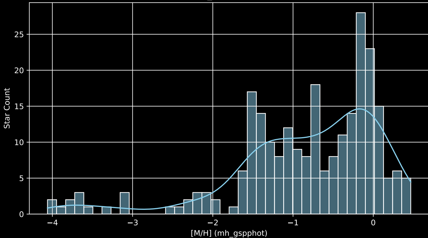
Gaia Cluster: [NGC_6583 [M/H] (mh_gspphot) (n= 249)
