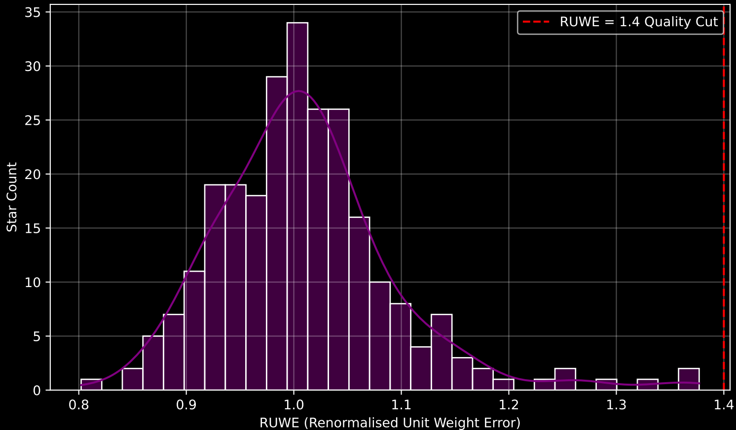
Gaia Cluster: [NGC_6583] RUWE Distribution (n= 255)
