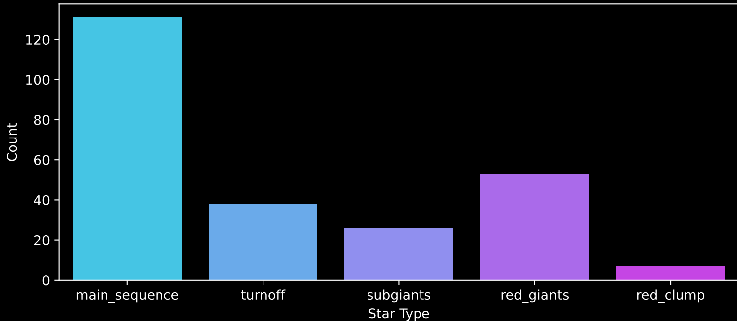
Gaia Cluster: [NGC_6583] Count plot of Star Type
