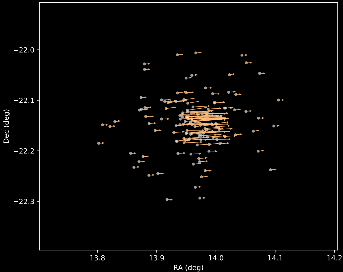
Gaia DR3 Cluster 3 Proper Motion Vectors (n=134)
