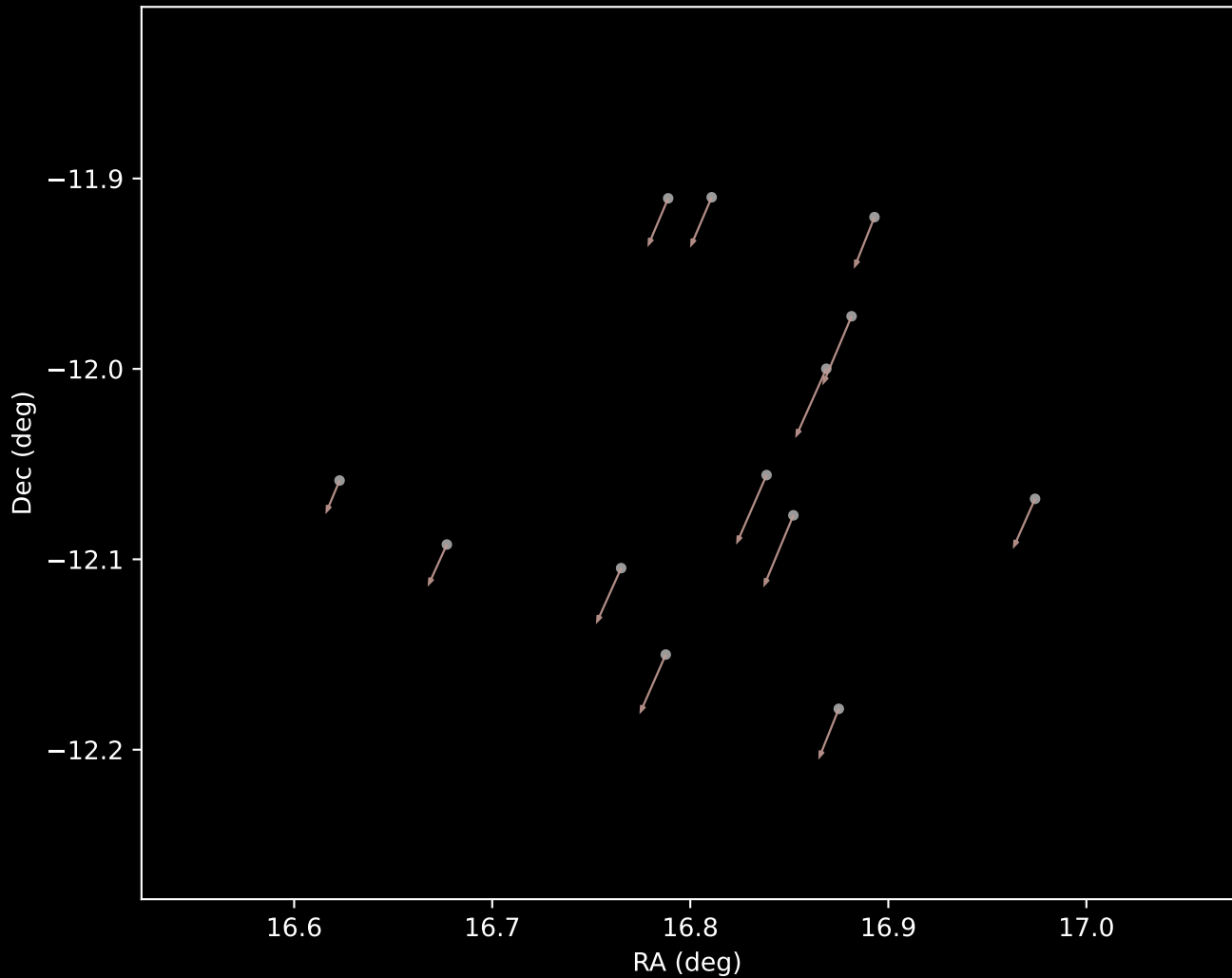
Gaia DR3 Cluster 11 Proper Motion Vectors (n=13)
