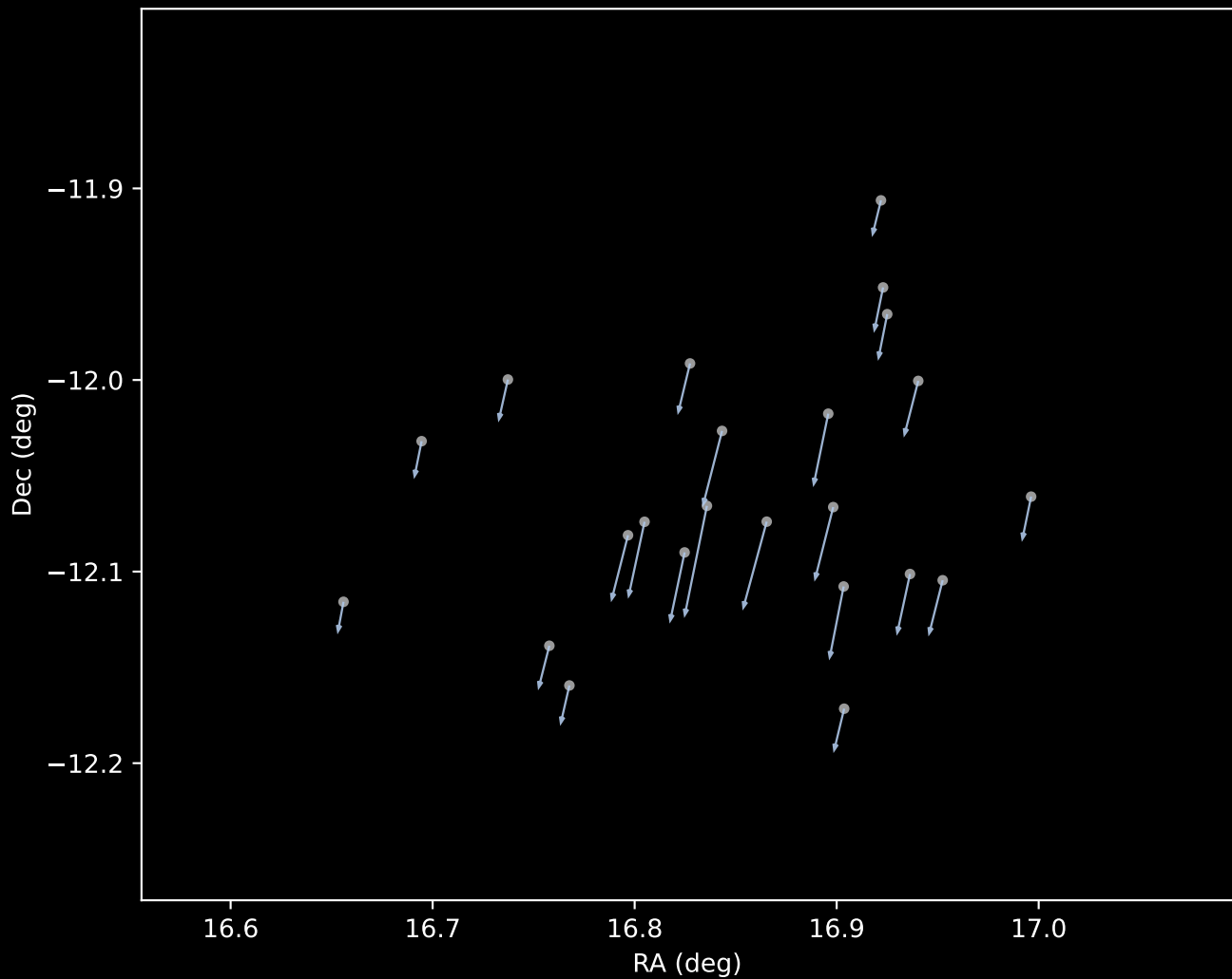
Gaia DR3 Cluster 21 Proper Motion Vectors (n=23)
