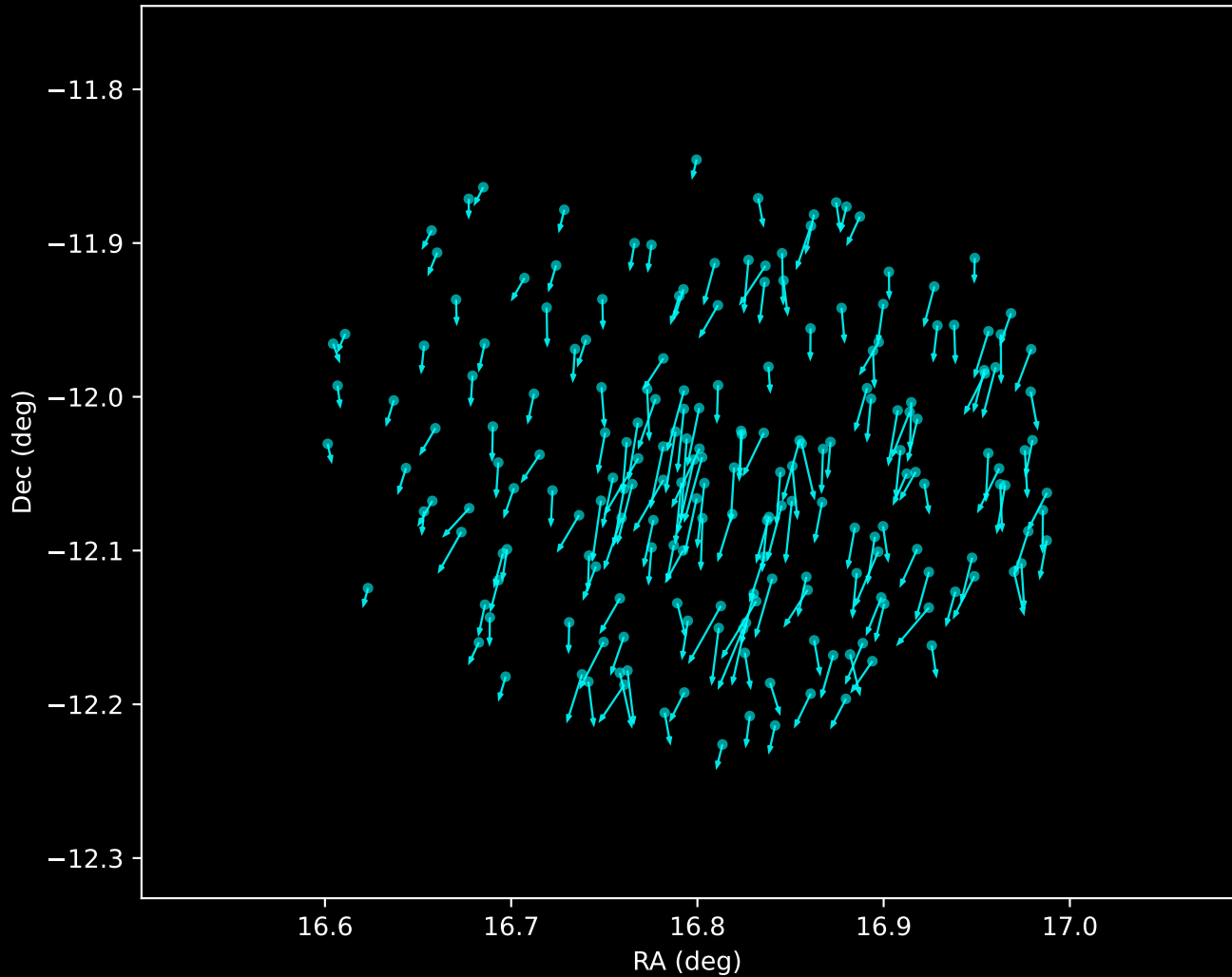
Gaia DR3 Noise Stream Proper Motion Vectors (n=199)
