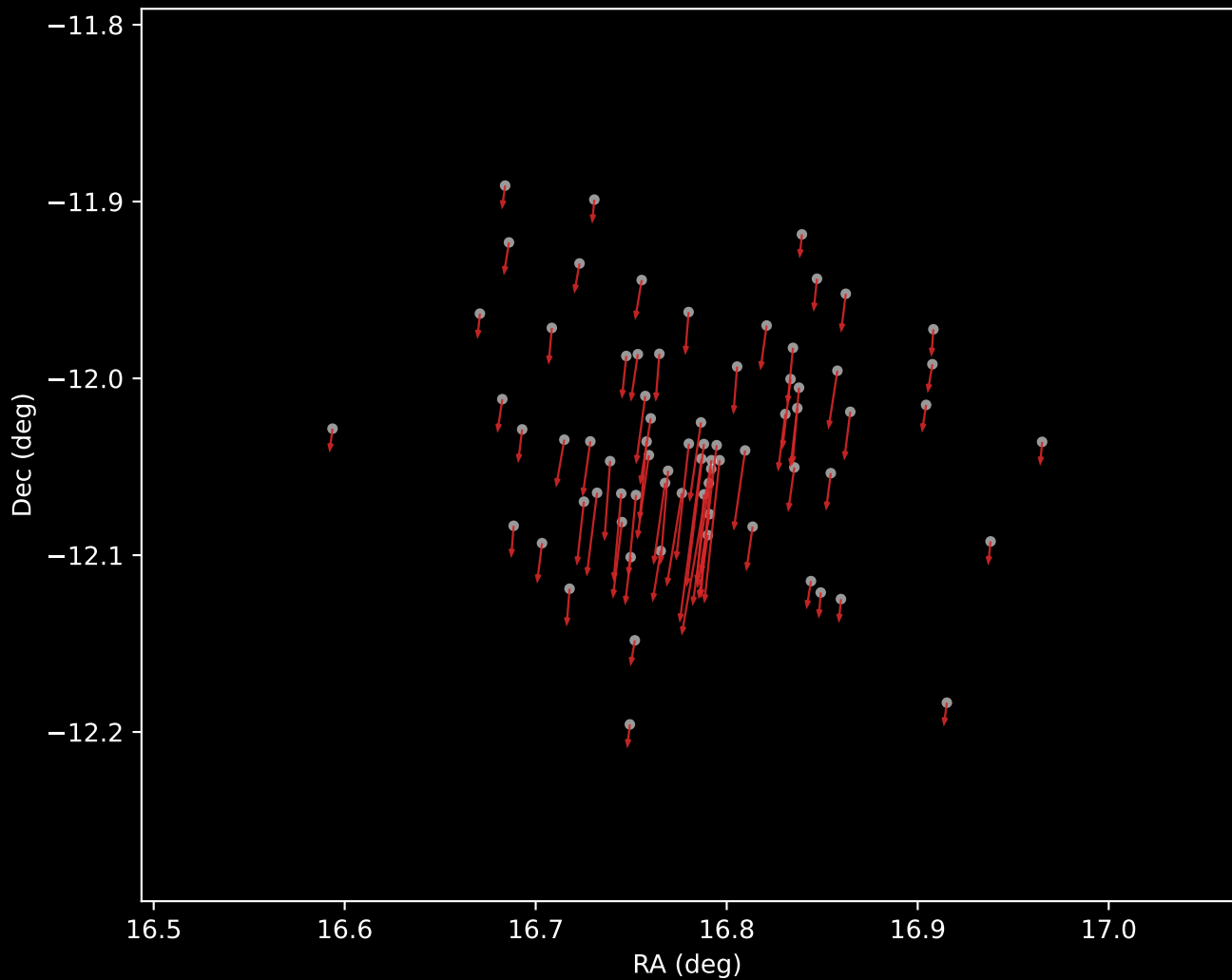
Gaia DR3 Cluster 26 Proper Motion Vectors (n=73)
