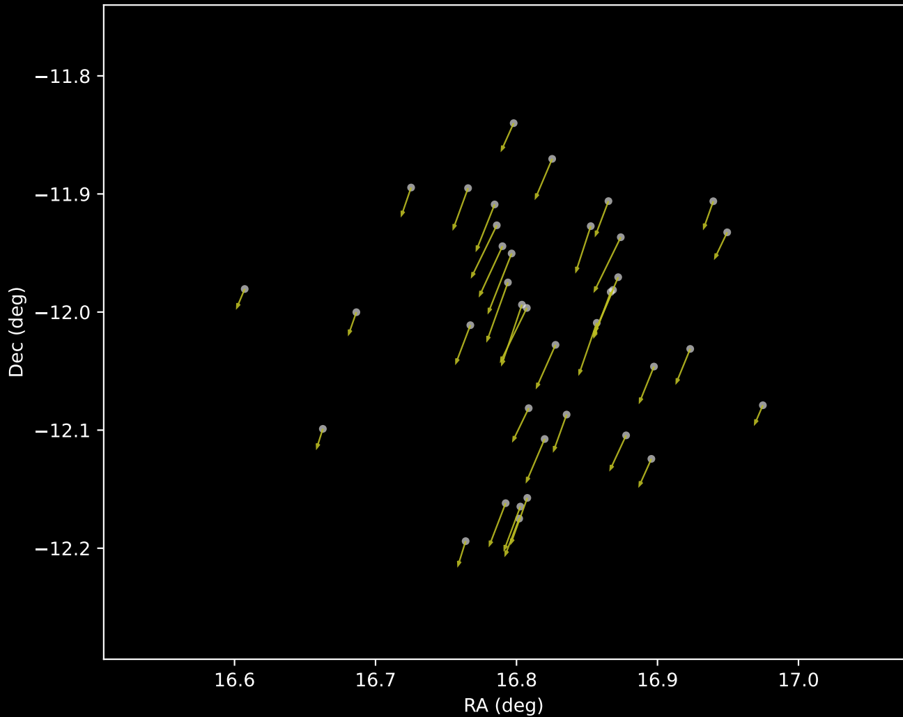
Gaia DR3 Cluster 16 Proper Motion Vectors (n=38)
