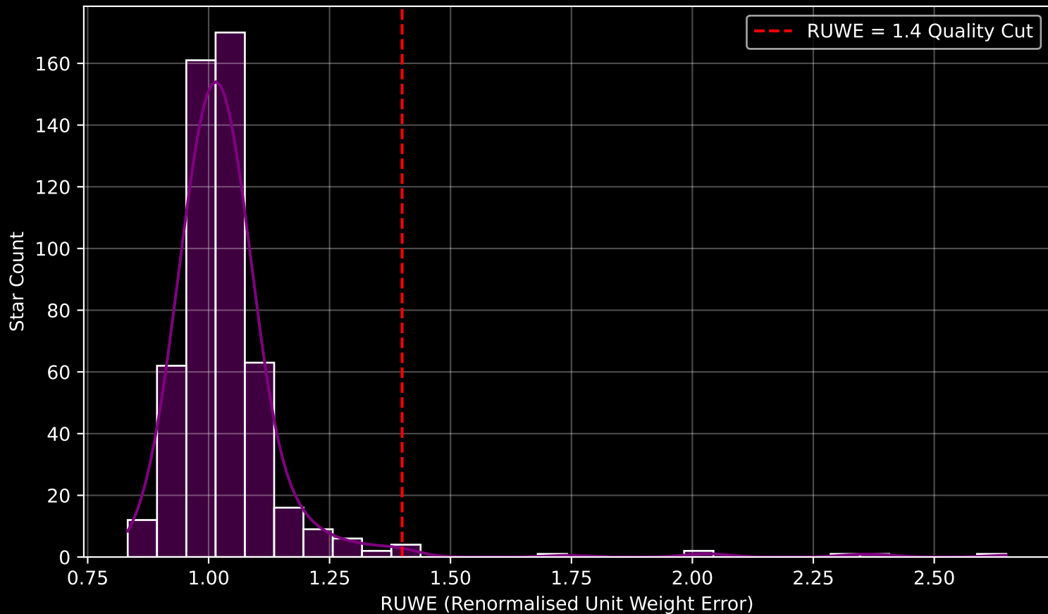
Gaia Cluster: [NGC_6631] RUWE Distribution (n= 511)
