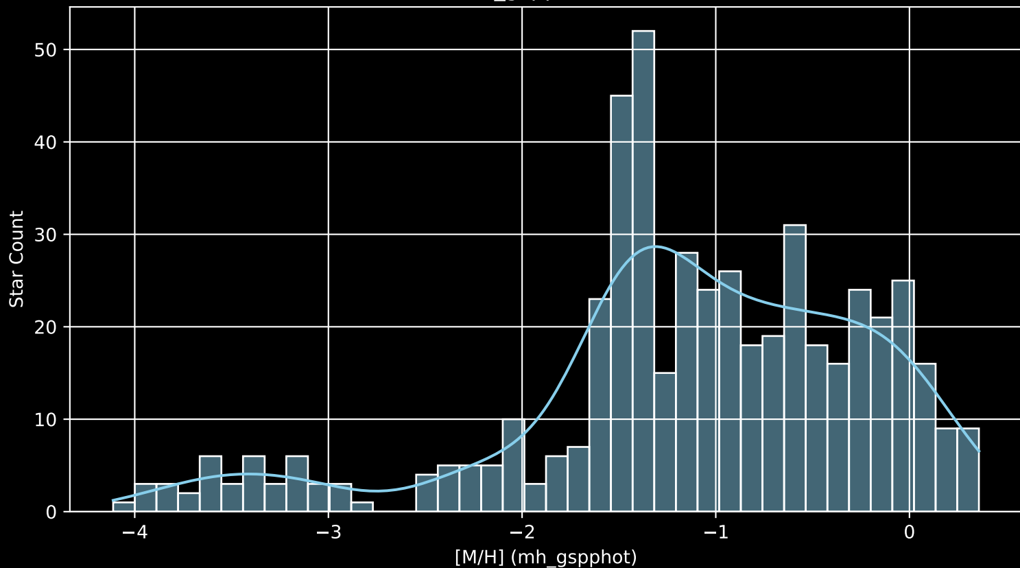
Gaia Cluster: [NGC_6631 [M/H] (mh_gspphot) (n= 504)
