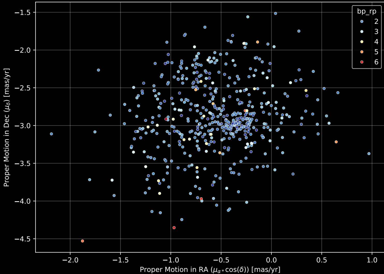
Gaia Cluster: [NGC_6631] Proper Motion Diagram (n= 512)
