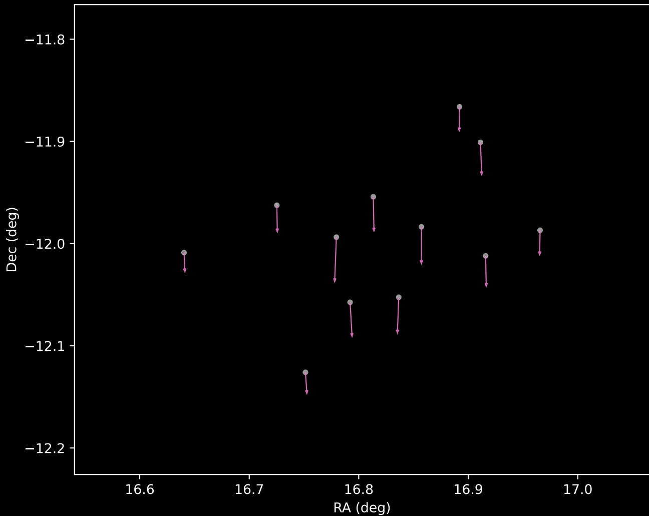
Gaia DR3 Cluster 12 Proper Motion Vectors (n=12)
