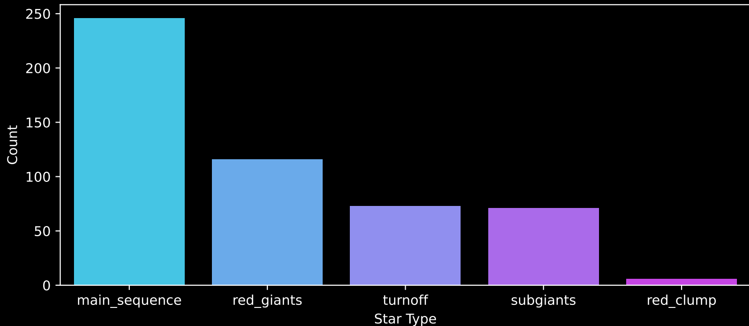
Gaia Cluster: [NGC_6631] Count plot of Star Type
