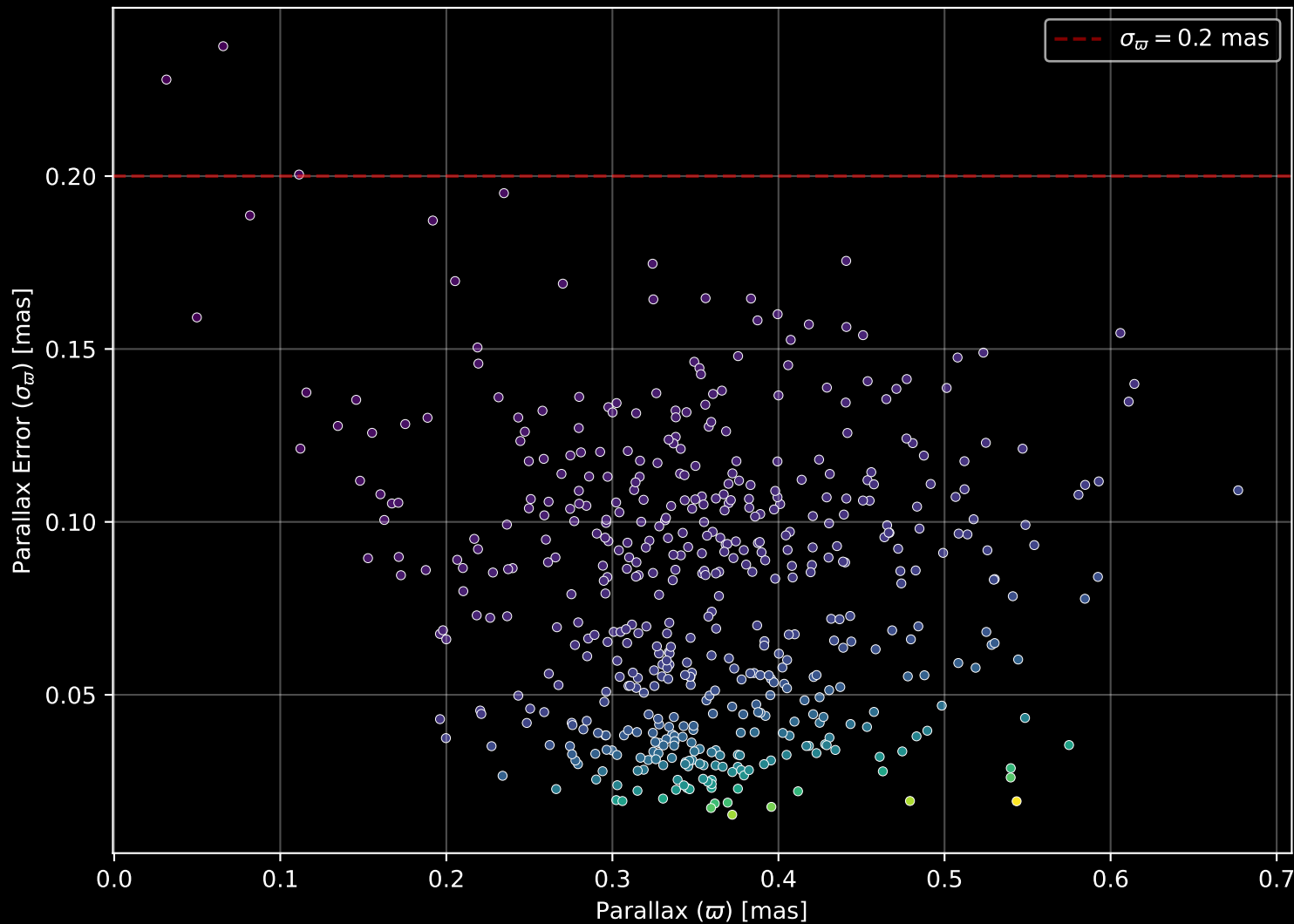
Gaia Cluster: [NGC_6631] Parallax Quality (n= 512)
