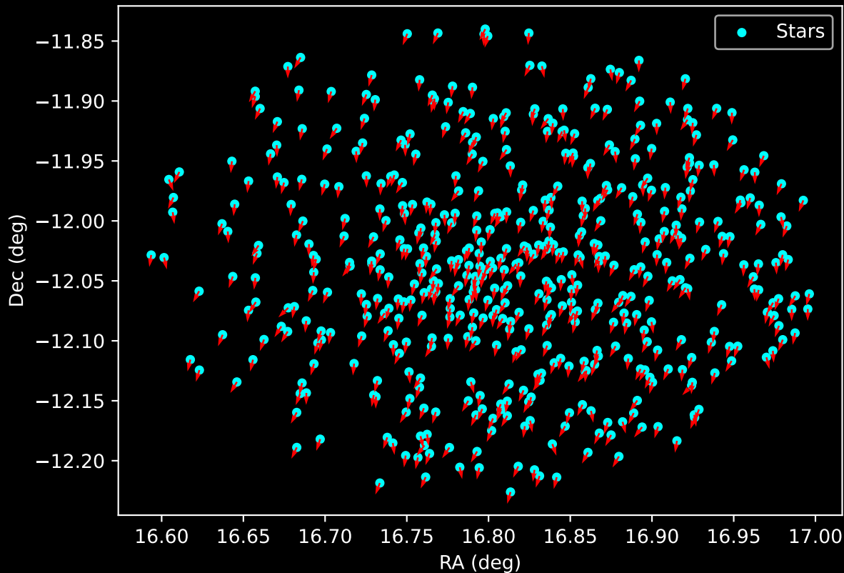
Gaia Cluster: [NGC_6631] Proper Motion Vectors for Gaia Star Field (n= 512)
