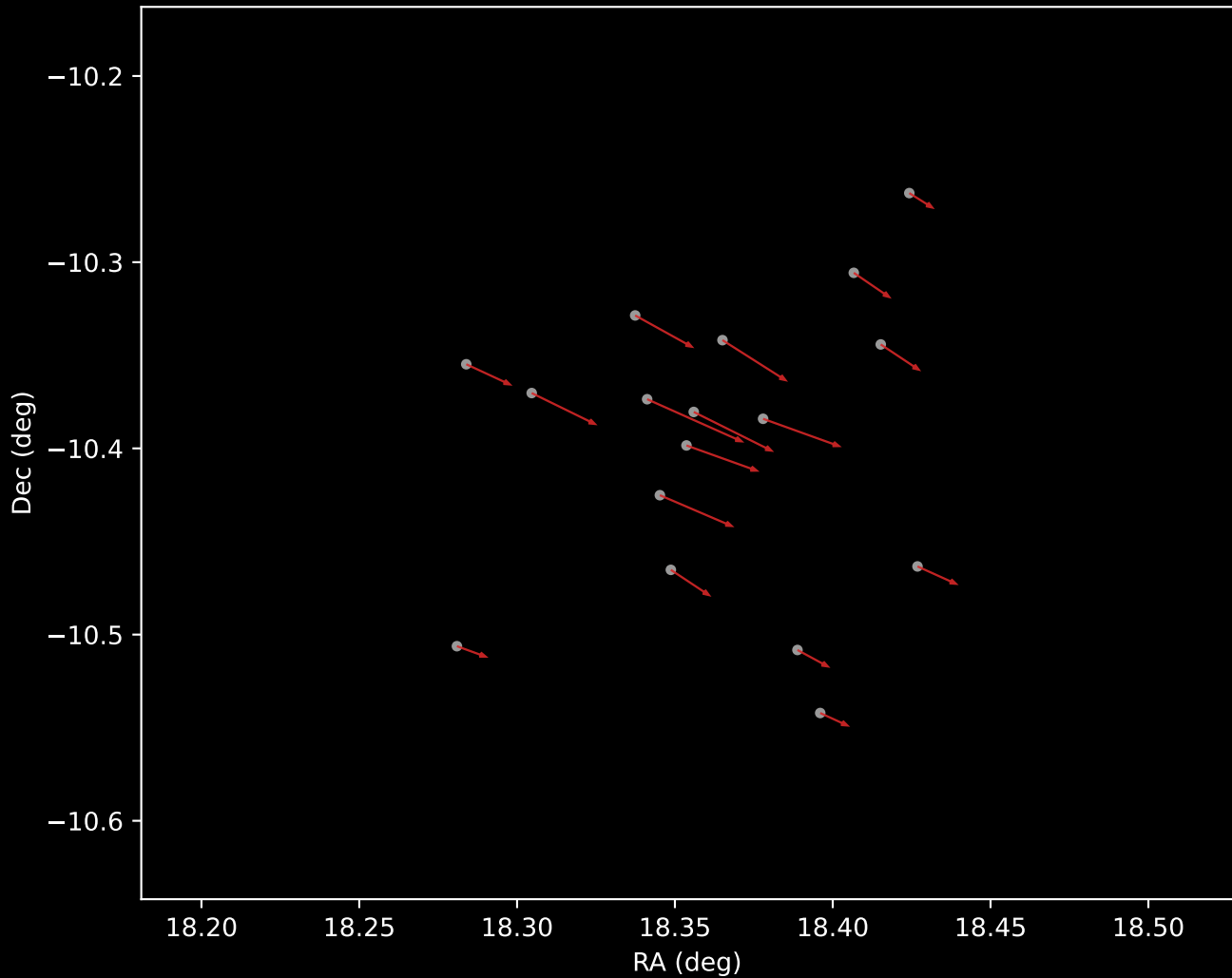
Gaia DR3 Cluster 26 Proper Motion Vectors (n=17)
