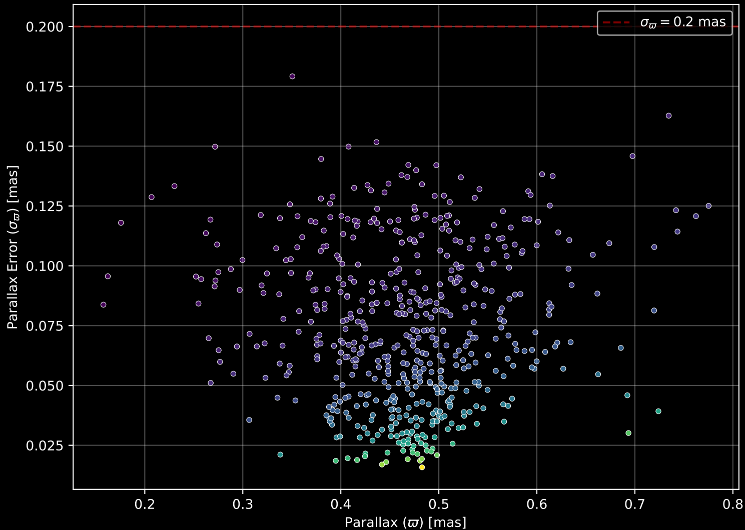
Gaia Cluster: [NGC_6649] Parallax Quality (n= 543)
