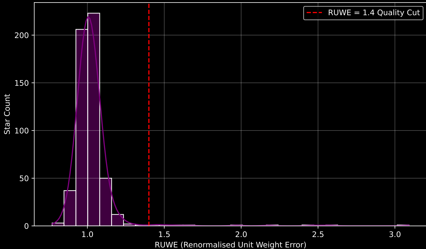
Gaia Cluster: [NGC_6649] RUWE Distribution (n= 543)
