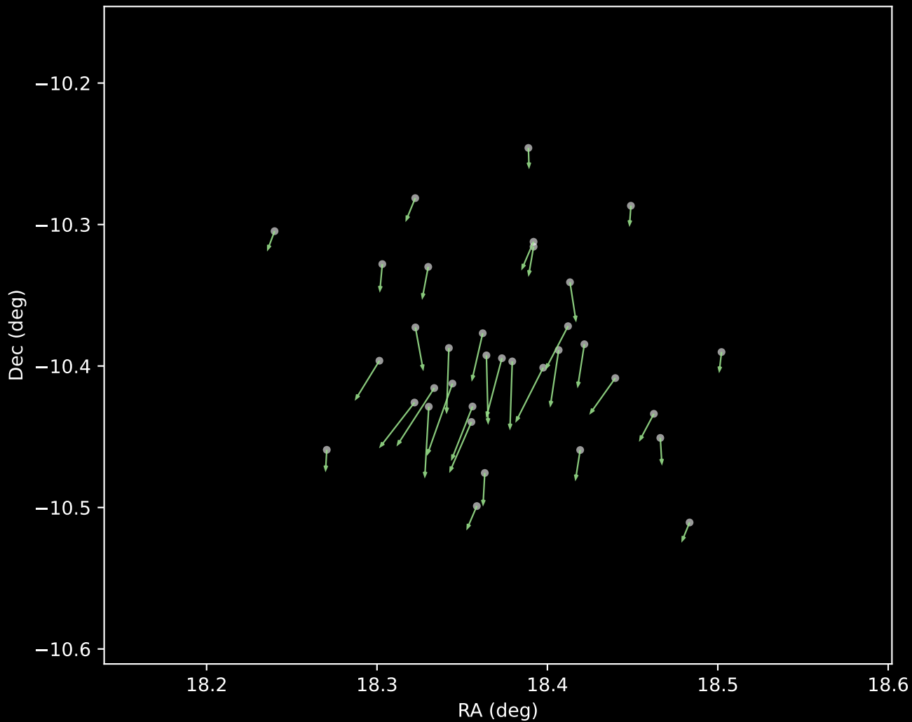
Gaia DR3 Cluster 25 Proper Motion Vectors (n=35)
