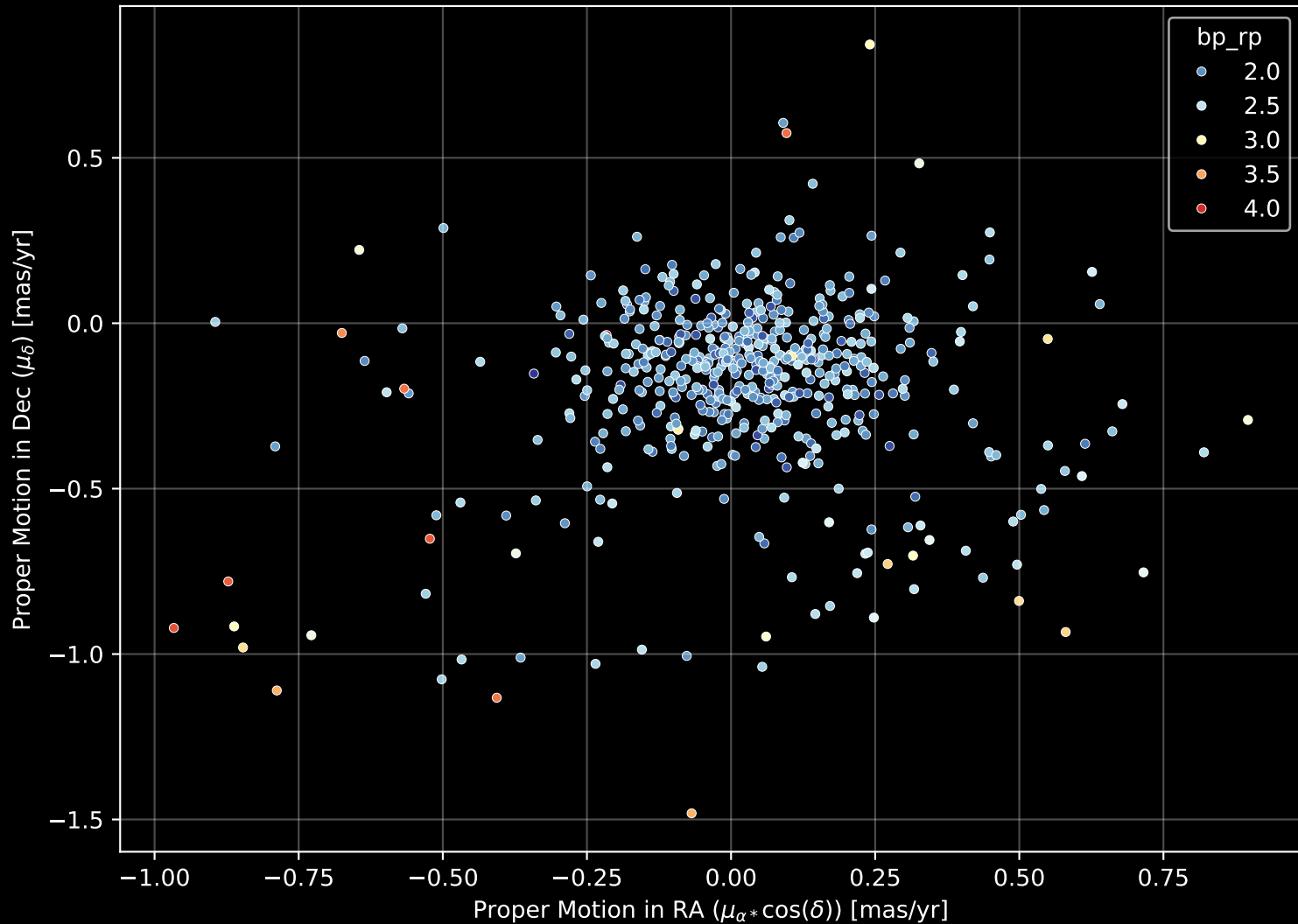
Gaia Cluster: [NGC_6649] Proper Motion Diagram (n= 543)
