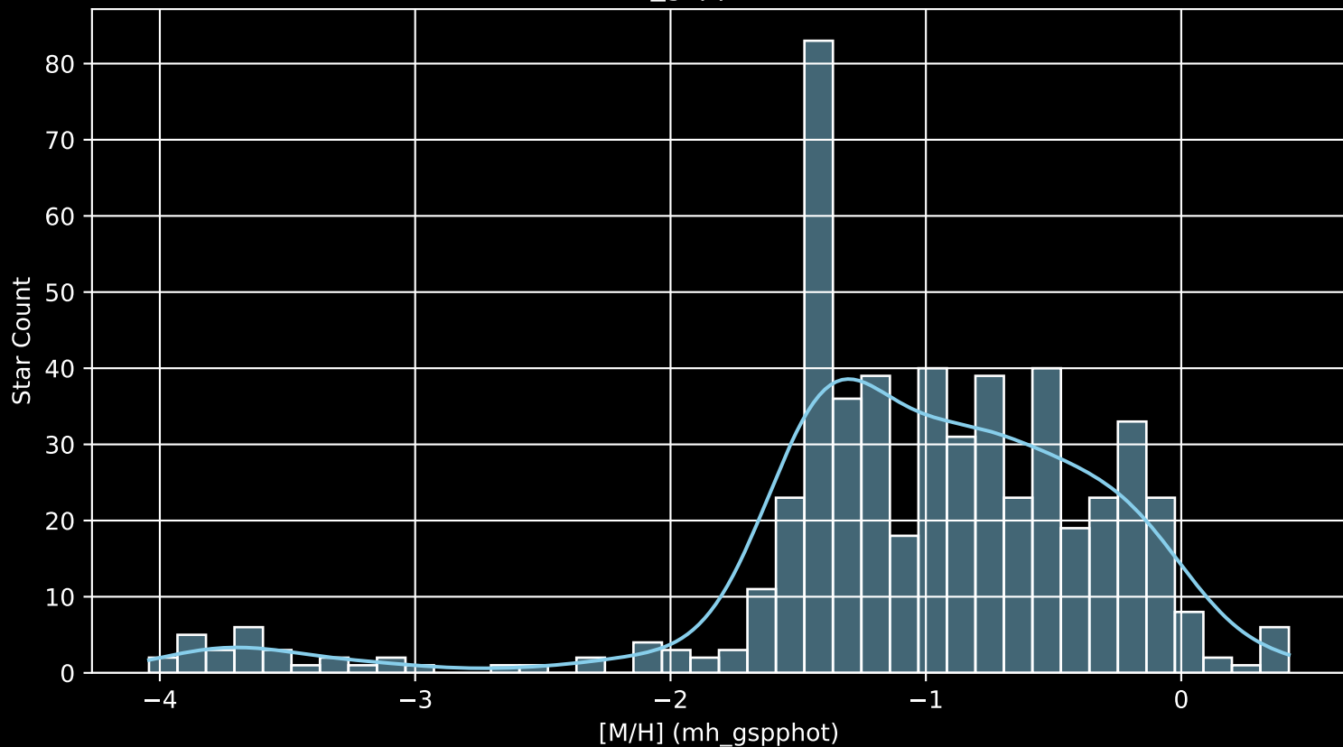
Gaia Cluster: [NGC_6649 [M/H] (mh_gspphot) (n= 540)
