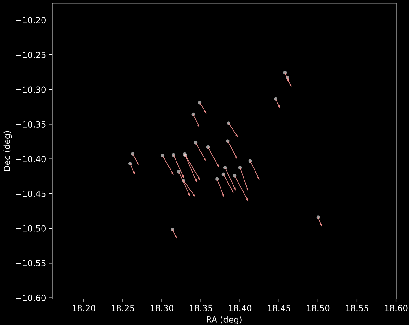
Gaia DR3 Cluster 27 Proper Motion Vectors (n=25)
