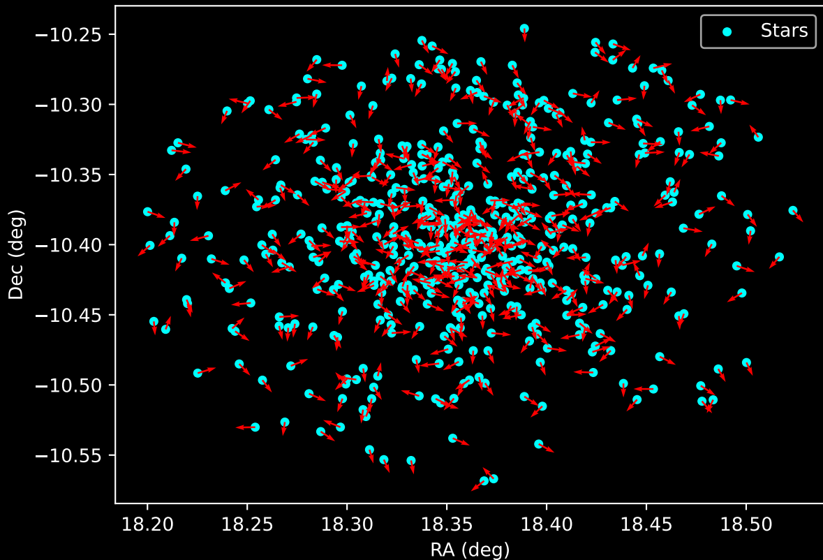
Gaia Cluster: [NGC_6649] Proper Motion Vectors for Gaia Star Field (n= 543)
