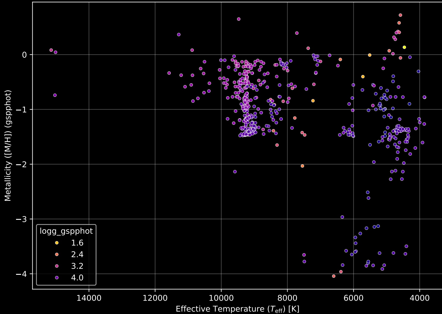
Gaia Cluster: [NGC_6649] Stellar Population Parameters (n= 543)
