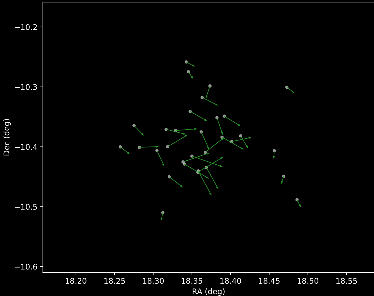
Gaia DR3 Cluster 24 Proper Motion Vectors (n=31)
