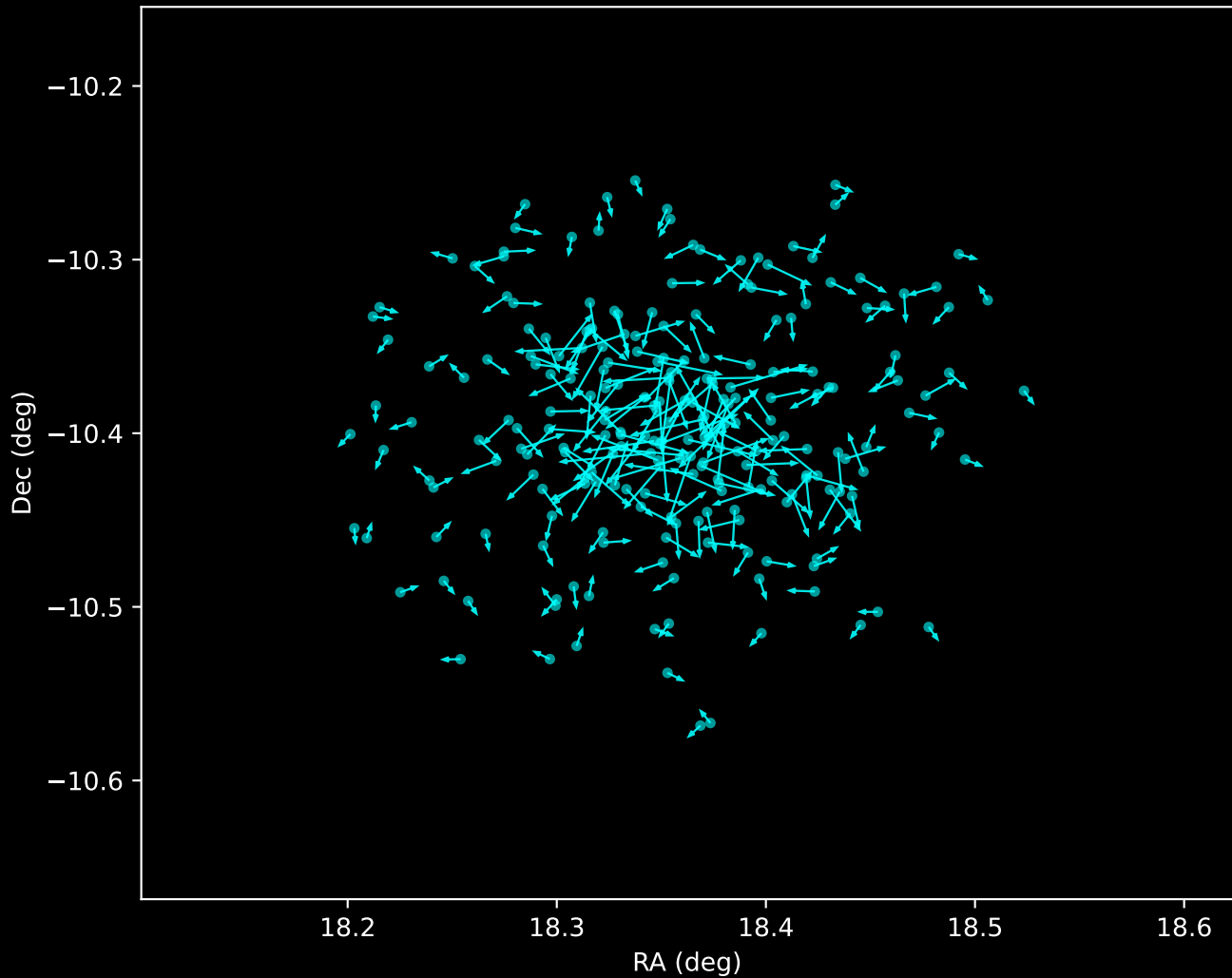
Gaia DR3 Noise Stream Proper Motion Vectors (n=231)
