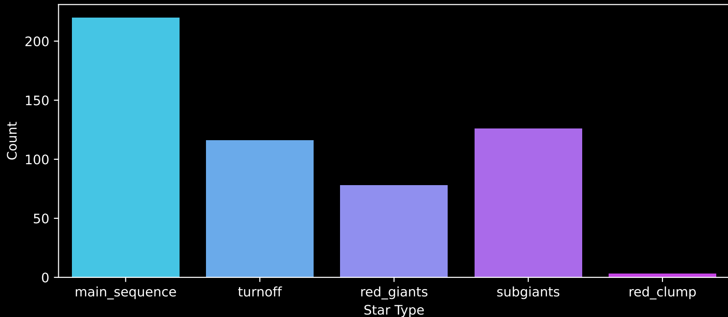
Gaia Cluster: [NGC_6649] Count plot of Star Type
