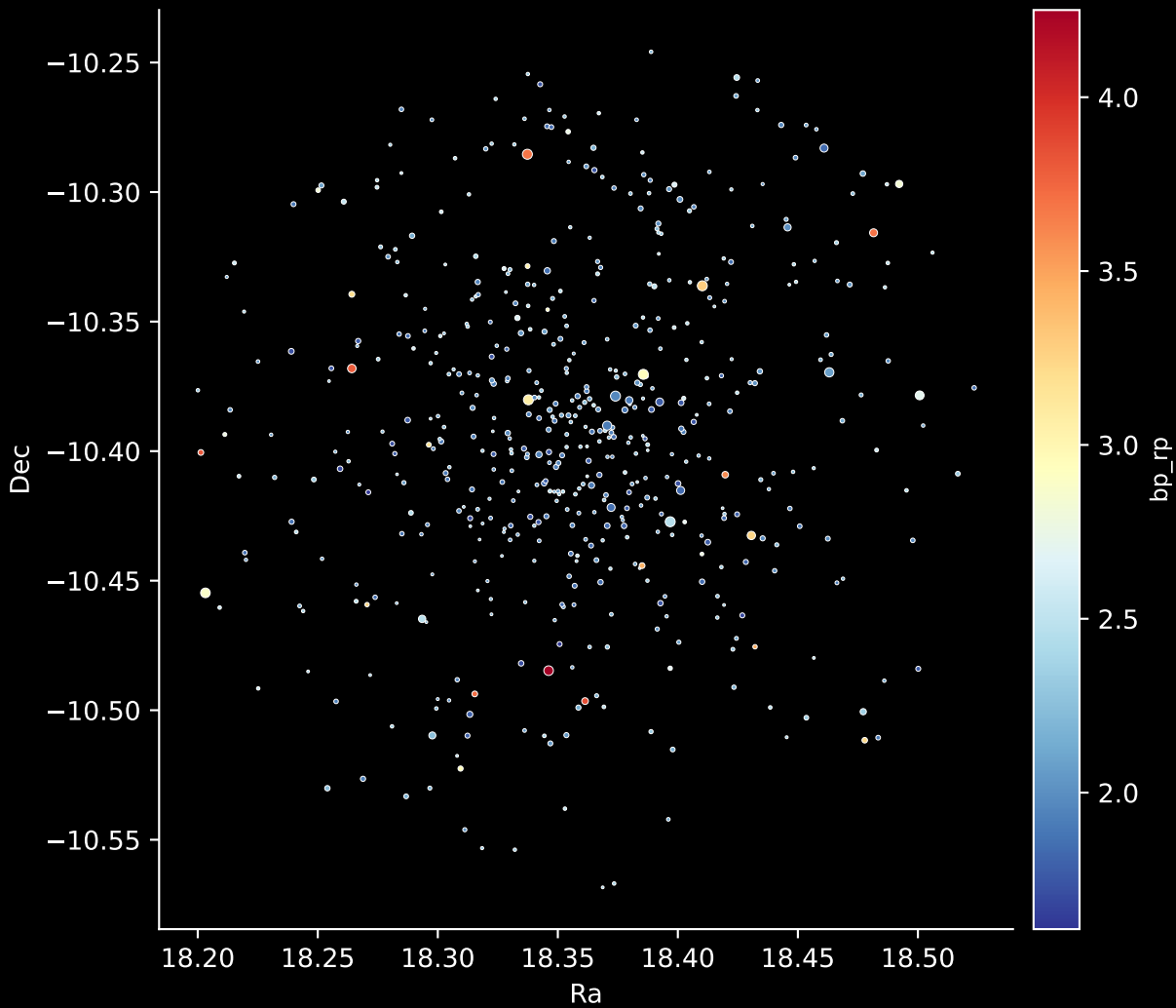
Gaia Cluster: [NGC_6649] Stars: 543
