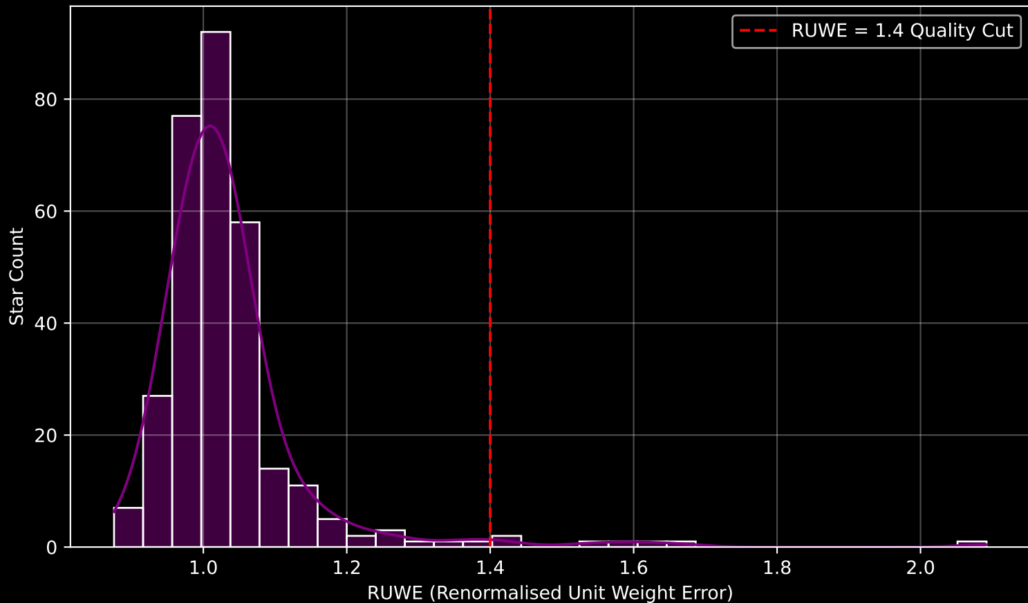
Gaia Cluster: [NGC_6756] RUWE Distribution (n= 306)
