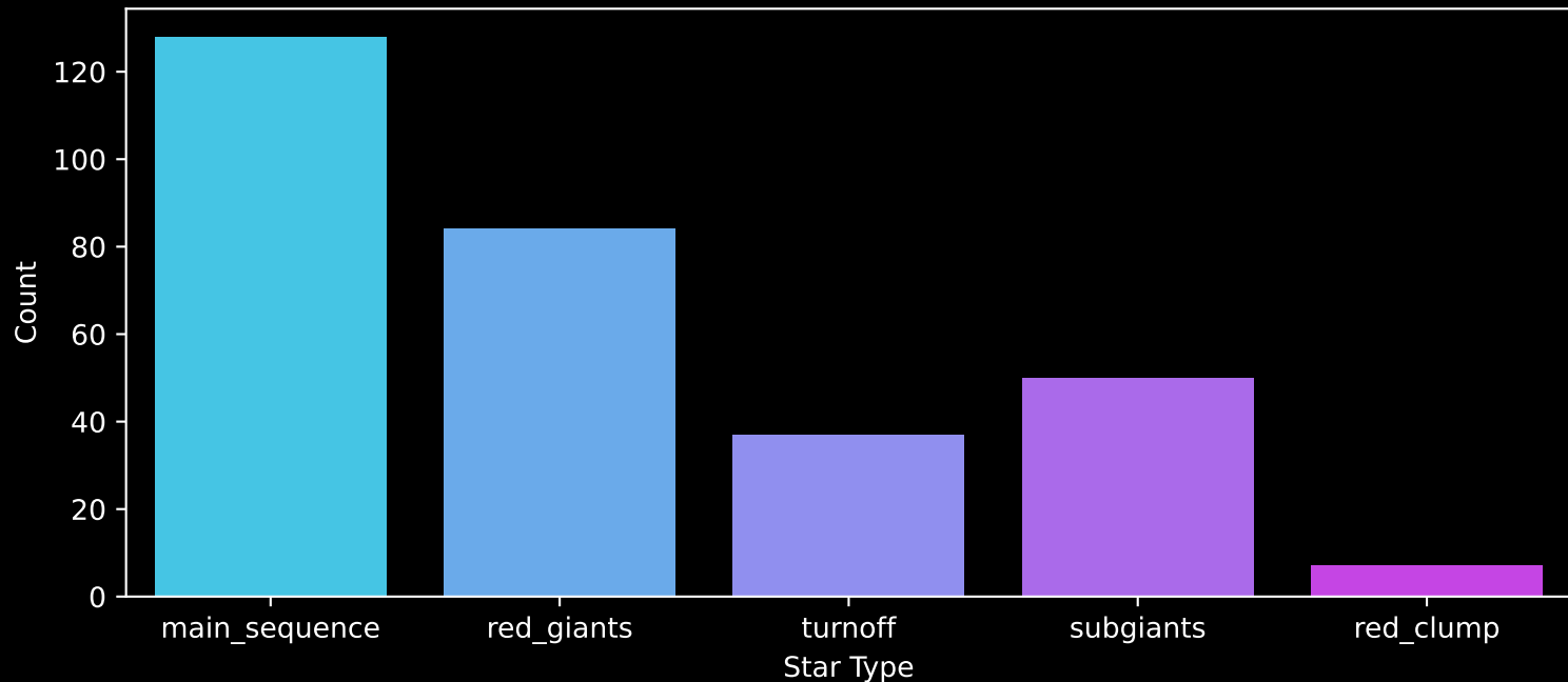
Gaia Cluster: [NGC_6756] Count plot of Star Type
