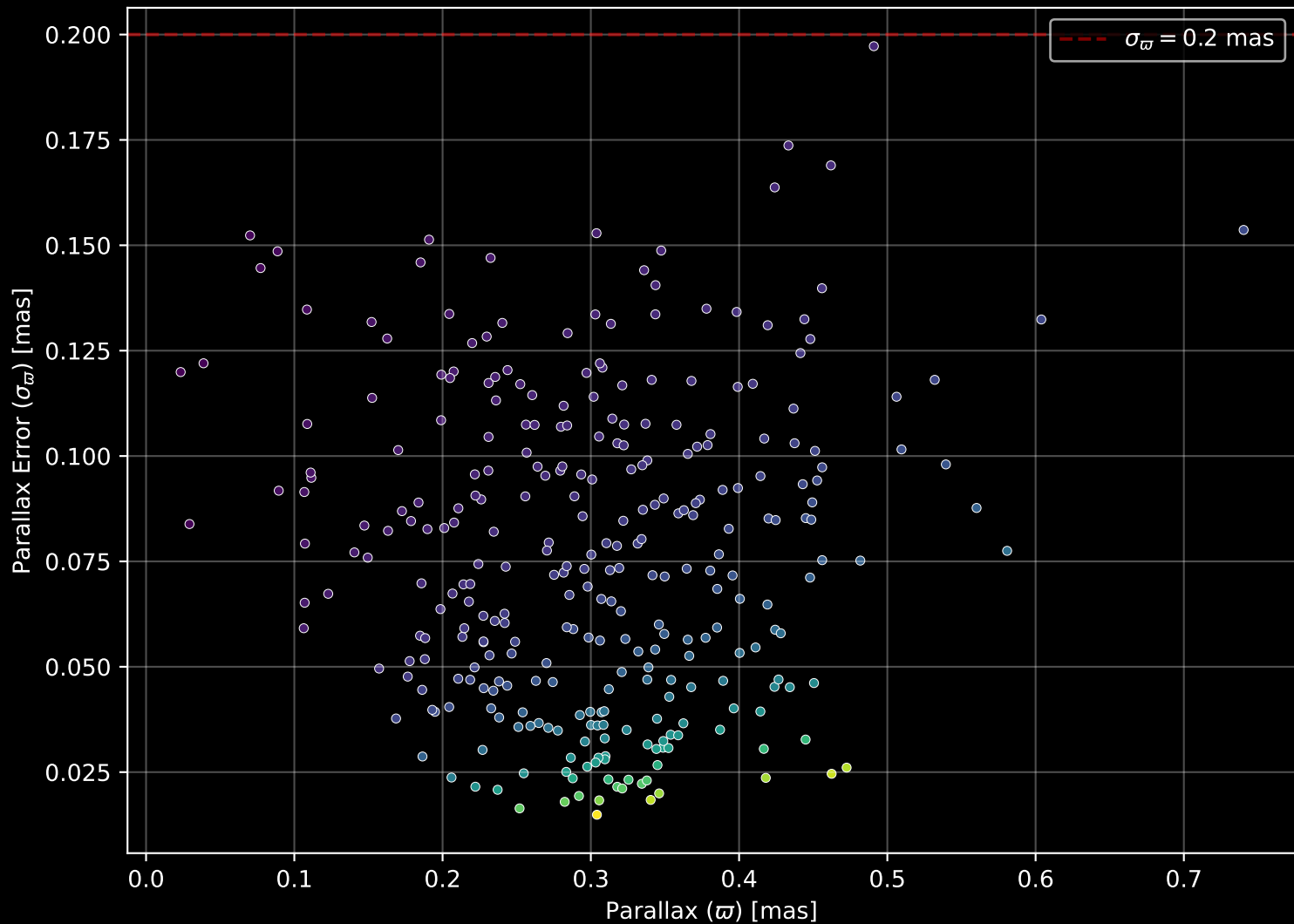
Gaia Cluster: [NGC_6756] Parallax Quality (n= 306)
