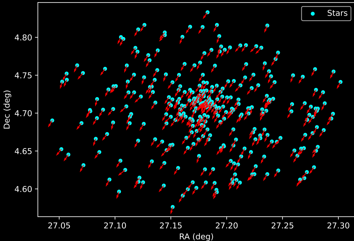
Gaia Cluster: [NGC_6756] Proper Motion Vectors for Gaia Star Field (n= 306)
