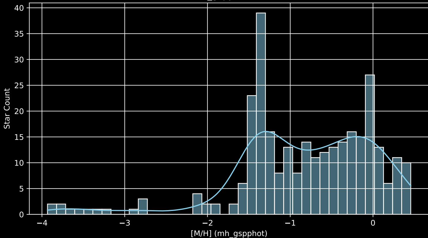
Gaia Cluster: [NGC_6756 [M/H] (mh_gspphot) (n= 298)
