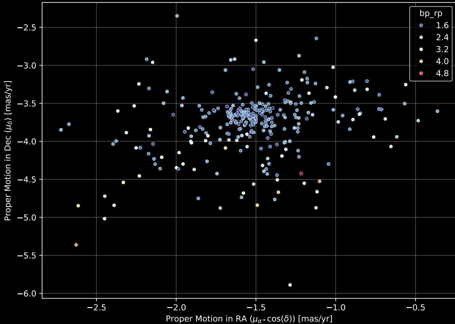
Gaia Cluster: [NGC_6756] Proper Motion Diagram (n= 306)
