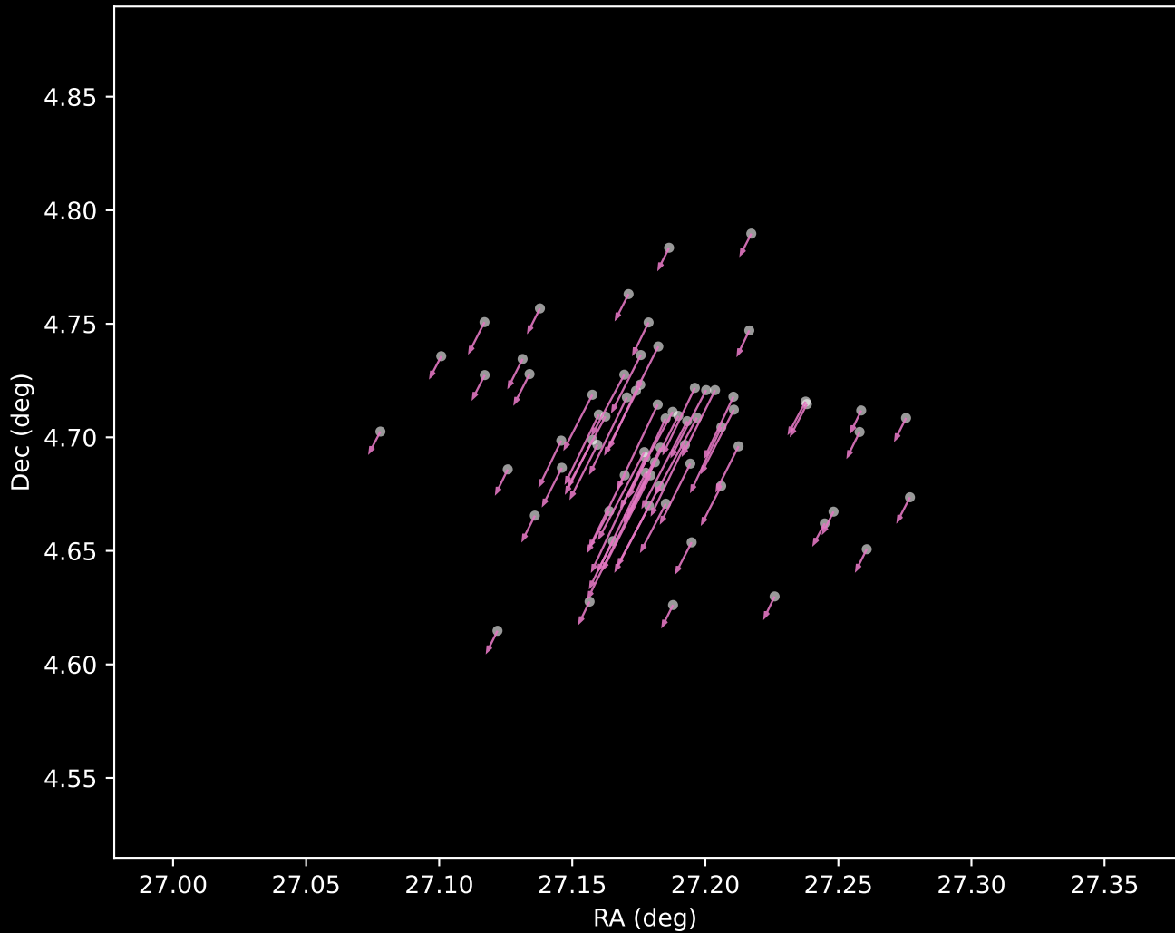
Gaia DR3 Cluster 12 Proper Motion Vectors (n=69)
