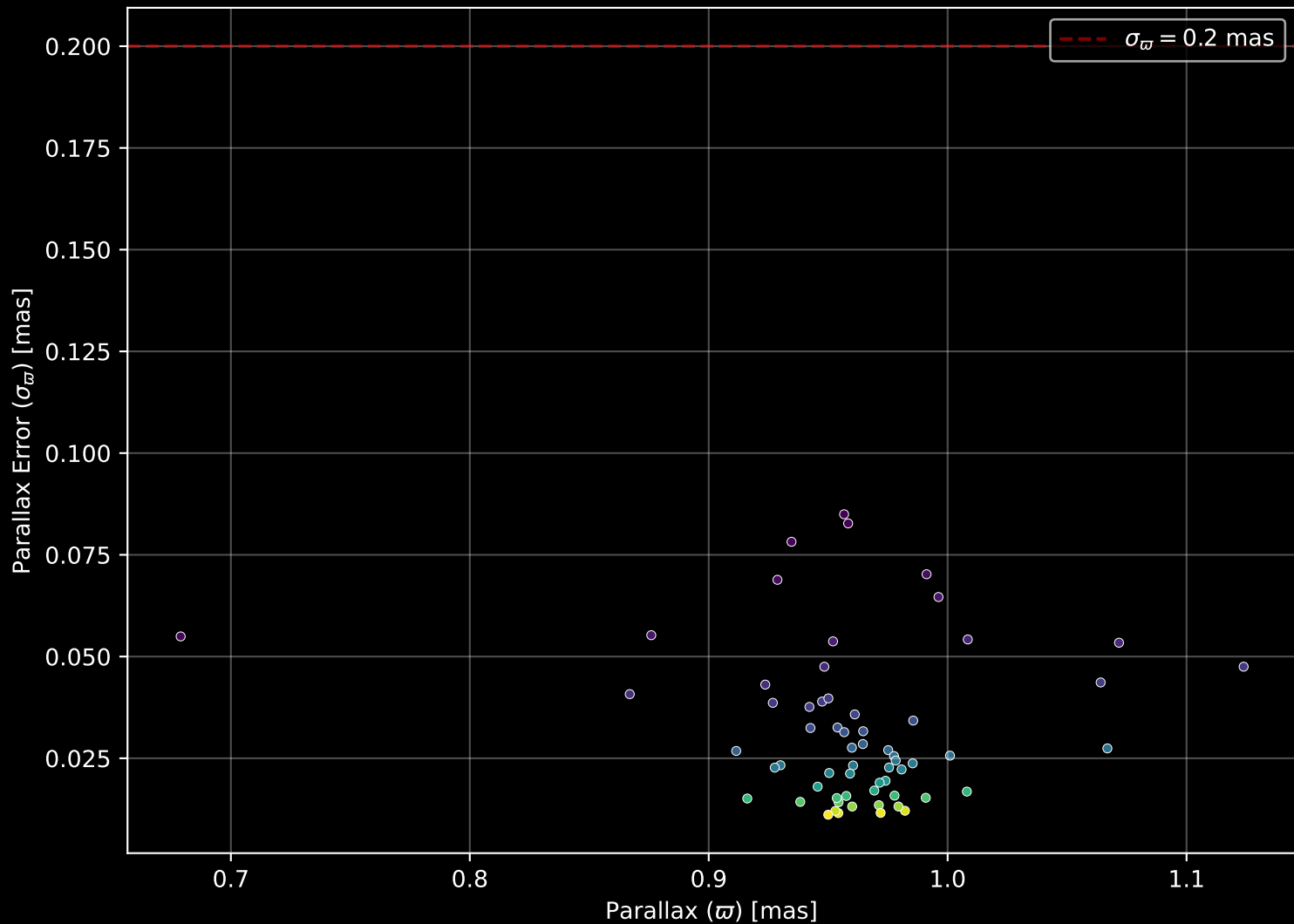
Gaia Cluster: [NGC_6800] Parallax Quality (n= 62)
