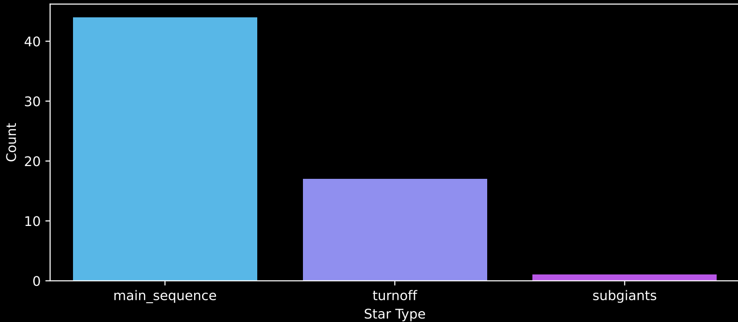
Gaia Cluster: [NGC_6800] Count plot of Star Type
