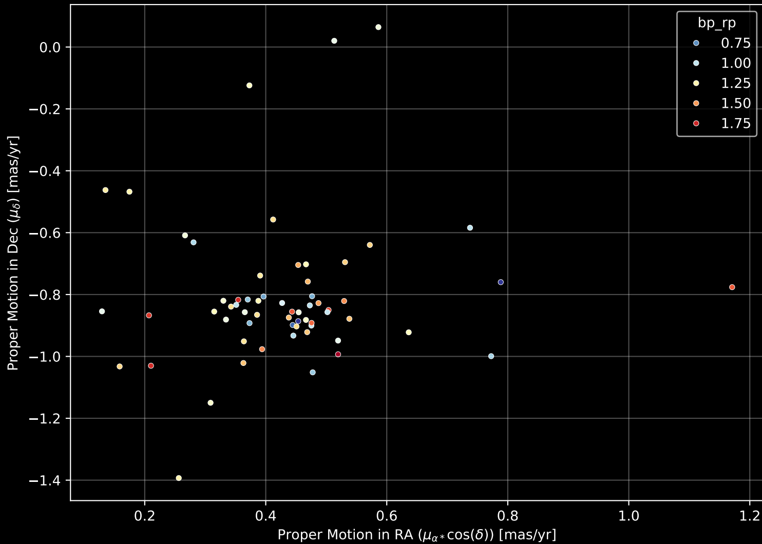
Gaia Cluster: [NGC_6800] Proper Motion Diagram (n= 62)
