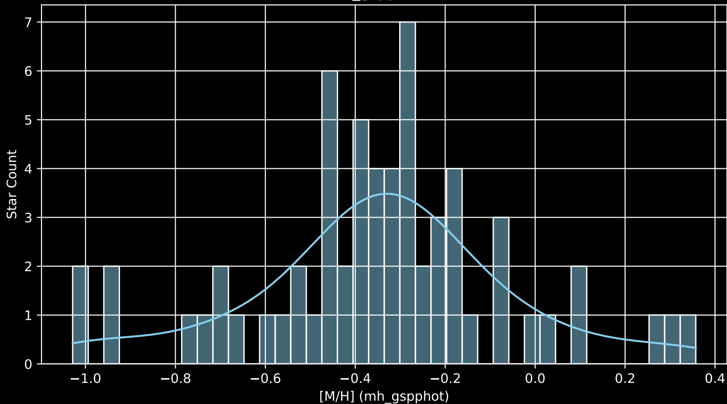
Gaia Cluster: [NGC_6800 [M/H] (mh_gspphot) (n= 62)
