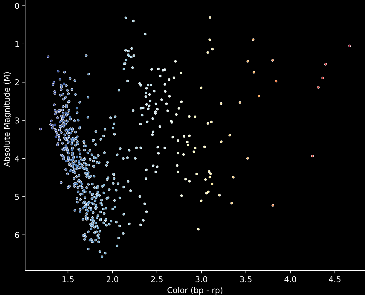
Gaia Cluster: [NGC 6802] Stars (n= 547) Hertzsprung-Russell Diagram
