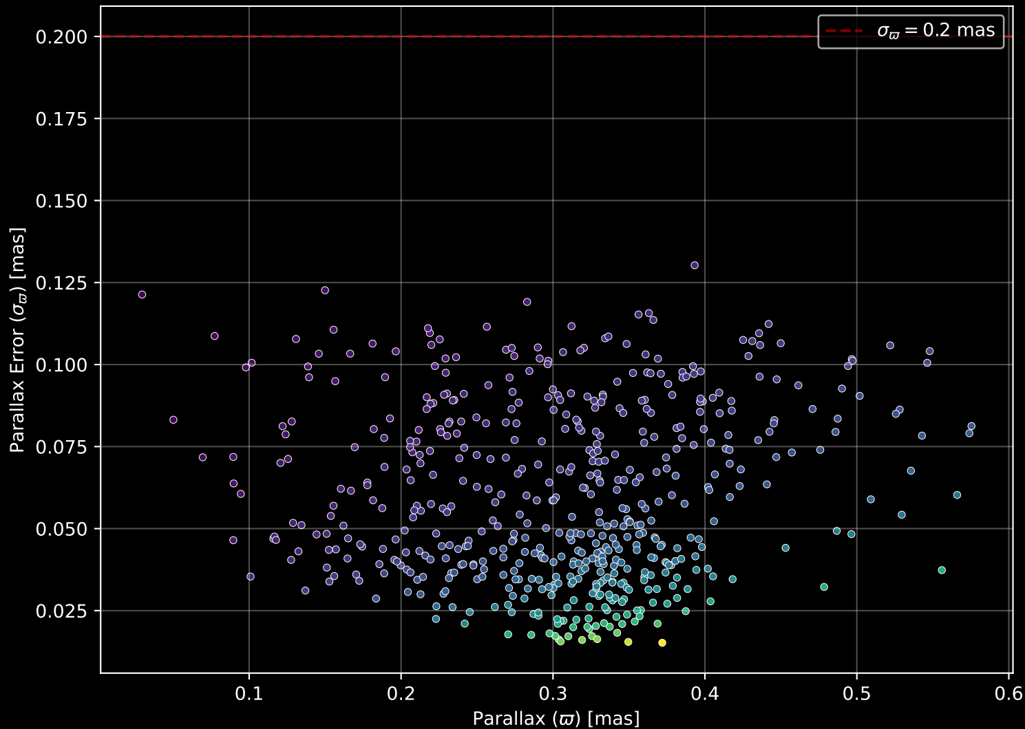
Gaia Cluster: [NGC_6802] Parallax Quality (n= 547)
