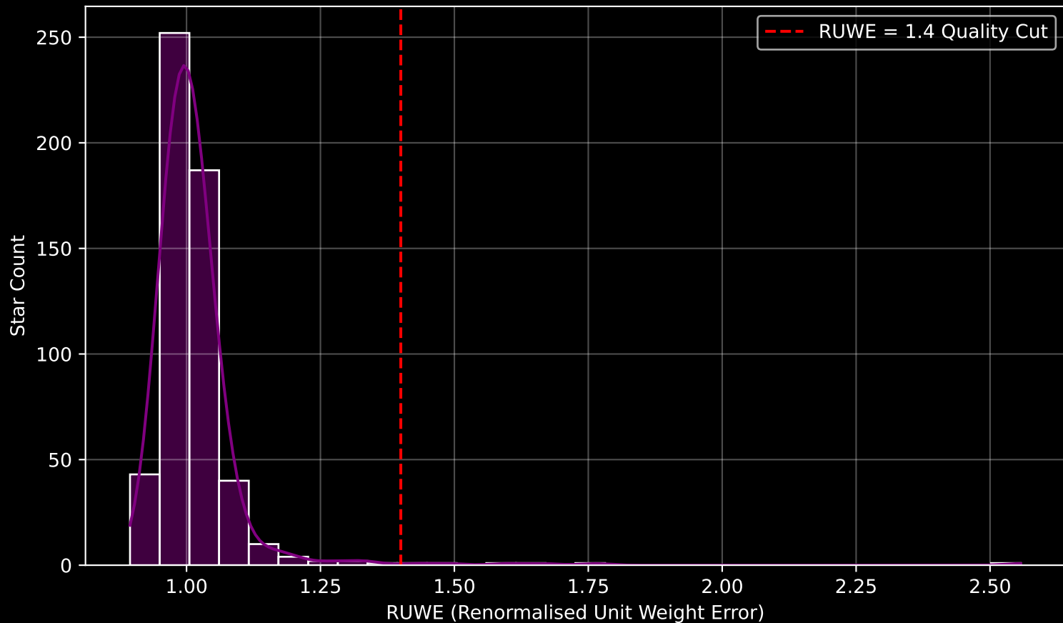
Gaia Cluster: [NGC_6802] RUWE Distribution (n= 547)
