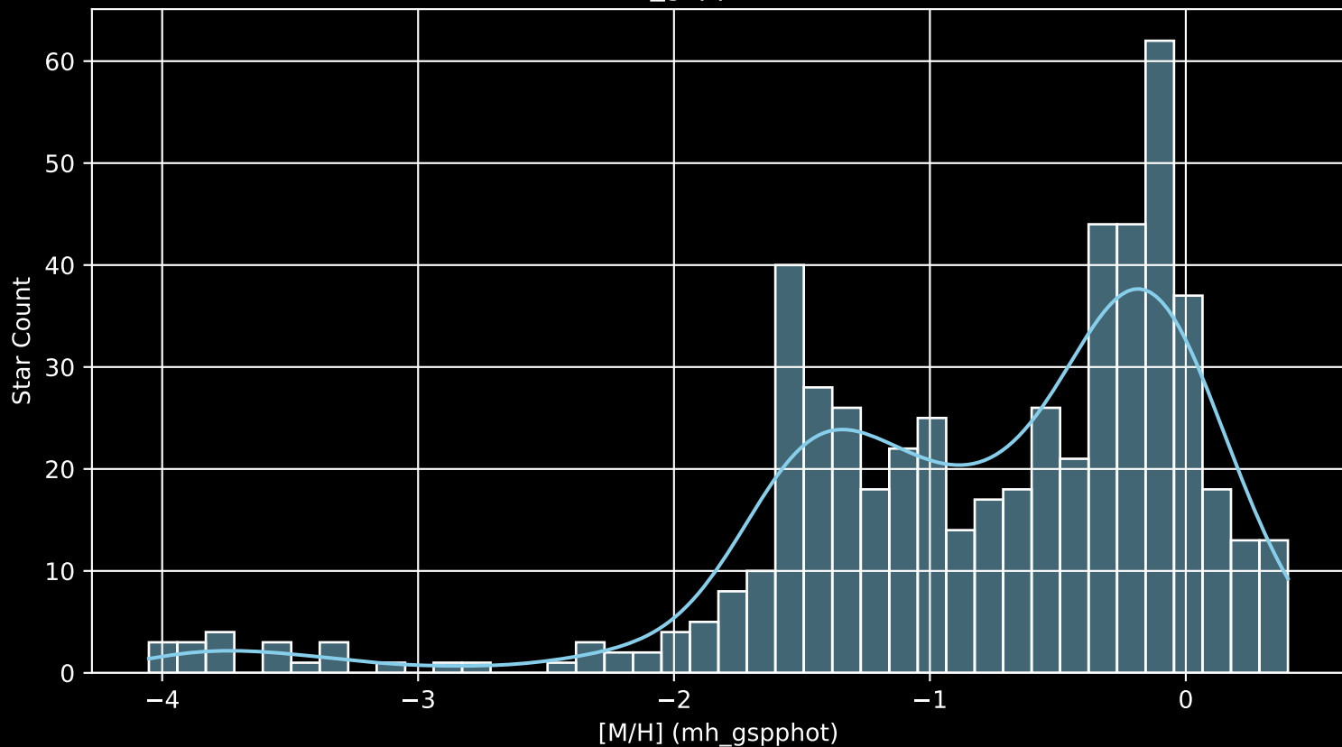
Gaia Cluster: [NGC_6802 [M/H] (mh_gspphot) (n= 541)
