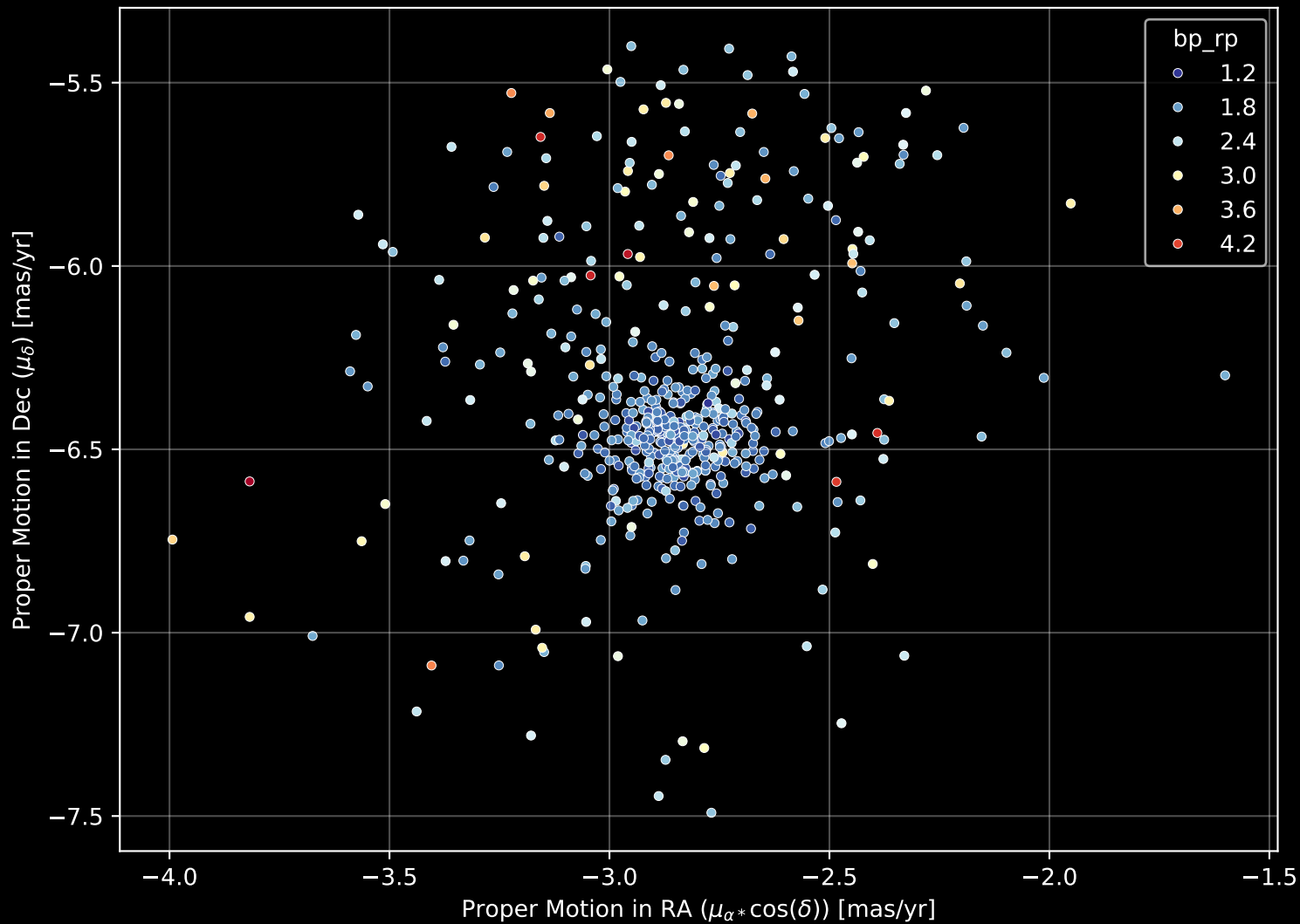
Gaia Cluster: [NGC_6802] Proper Motion Diagram (n= 547)
