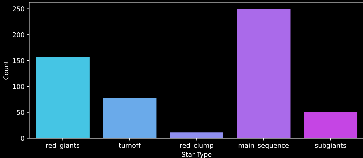
Gaia Cluster: [NGC_6802] Count plot of Star Type
