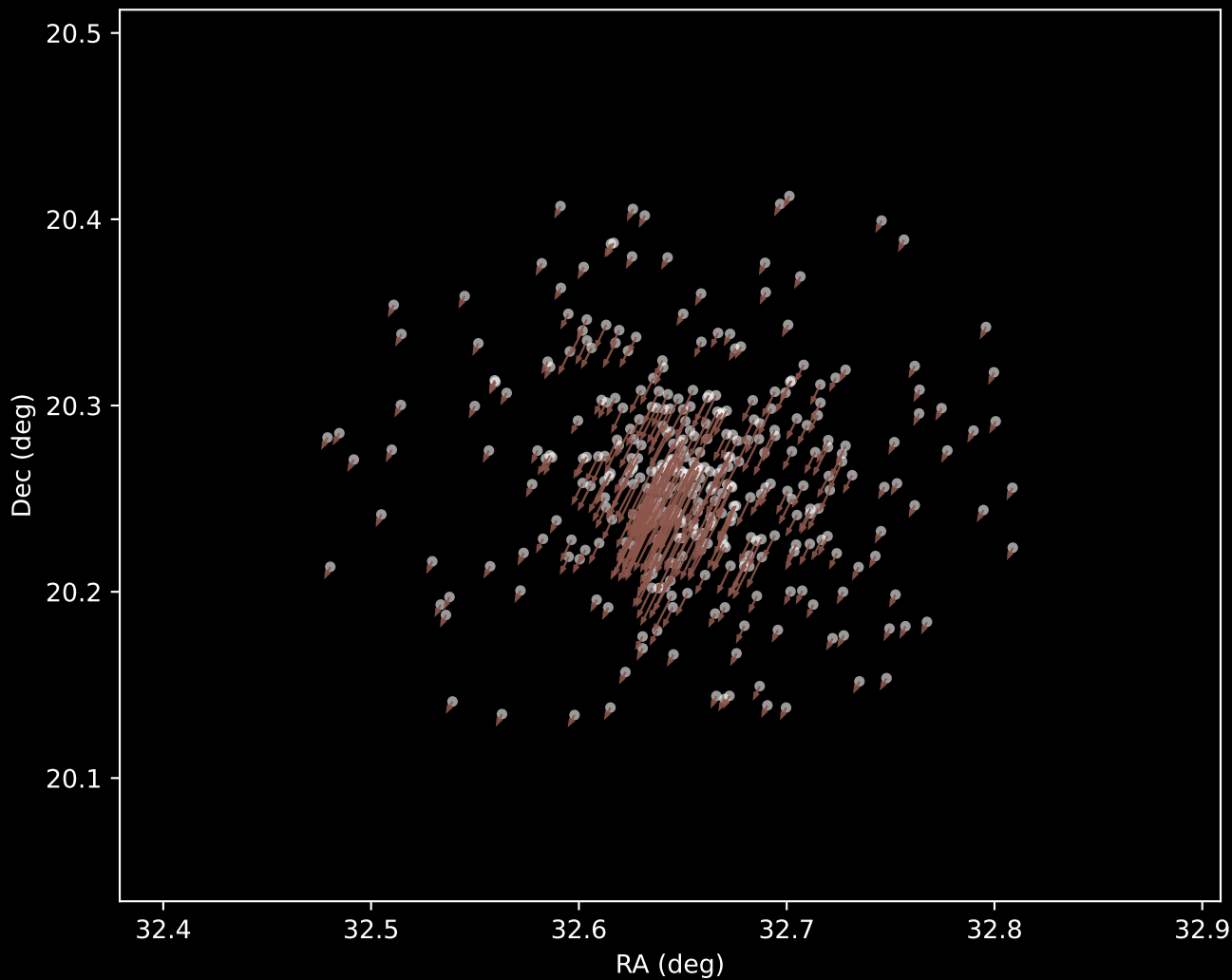
Gaia DR3 Cluster 10 Proper Motion Vectors (n=365)
