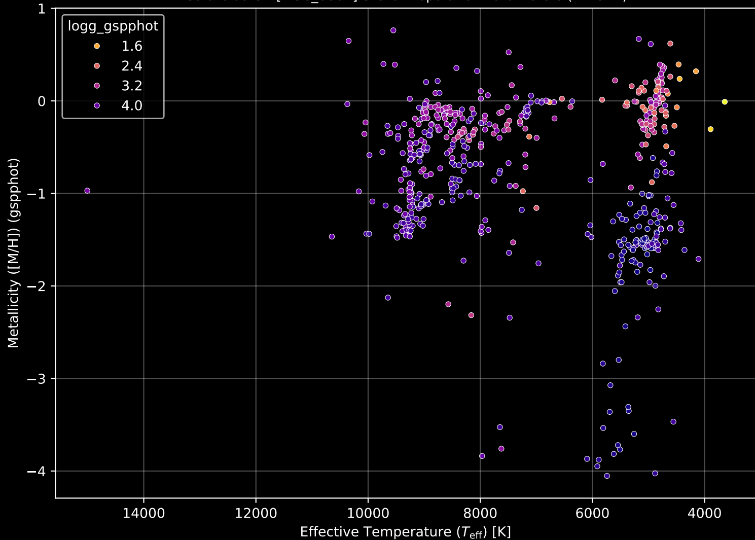
Gaia Cluster: [NGC_6802] Stellar Population Parameters (n= 547)
