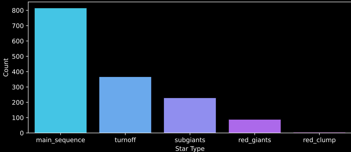
Gaia Cluster: [NGC_6871] Count plot of Star Type
