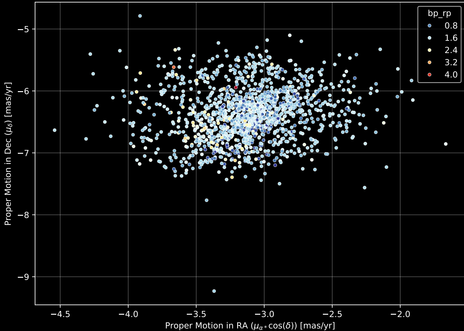
Gaia Cluster: [NGC_6871] Proper Motion Diagram (n= 1497)
