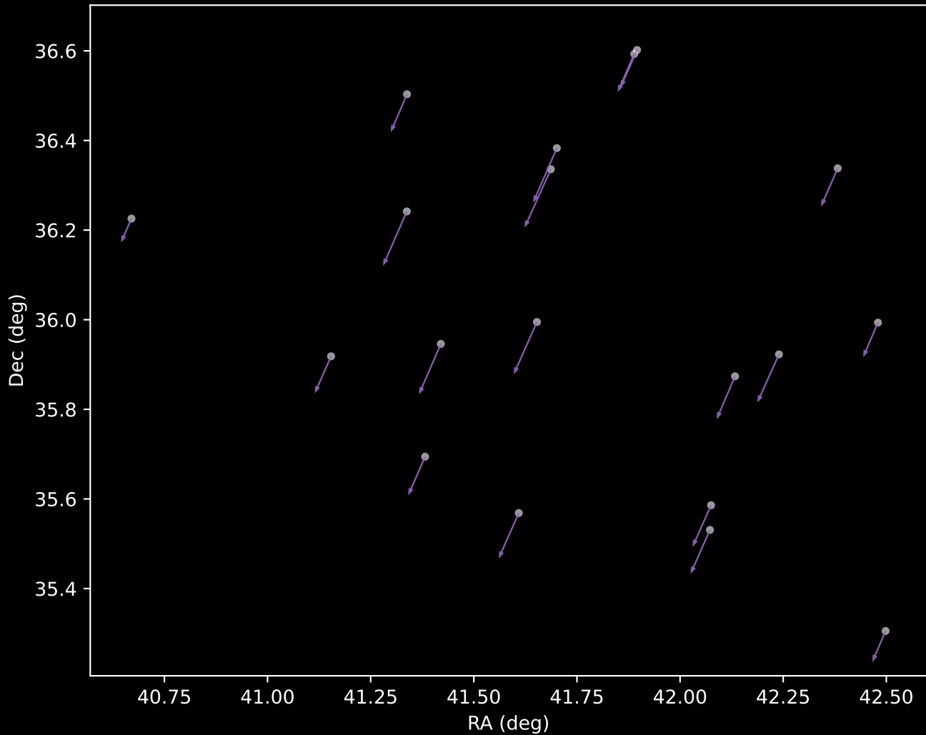
Gaia DR3 Cluster 48 Proper Motion Vectors (n=19)
