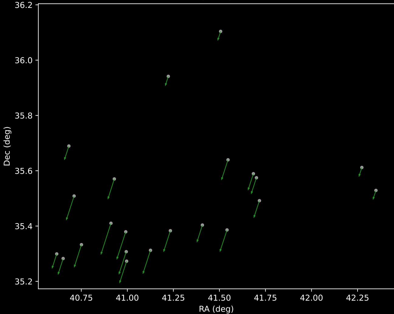
Gaia DR3 Cluster 44 Proper Motion Vectors (n=22)
