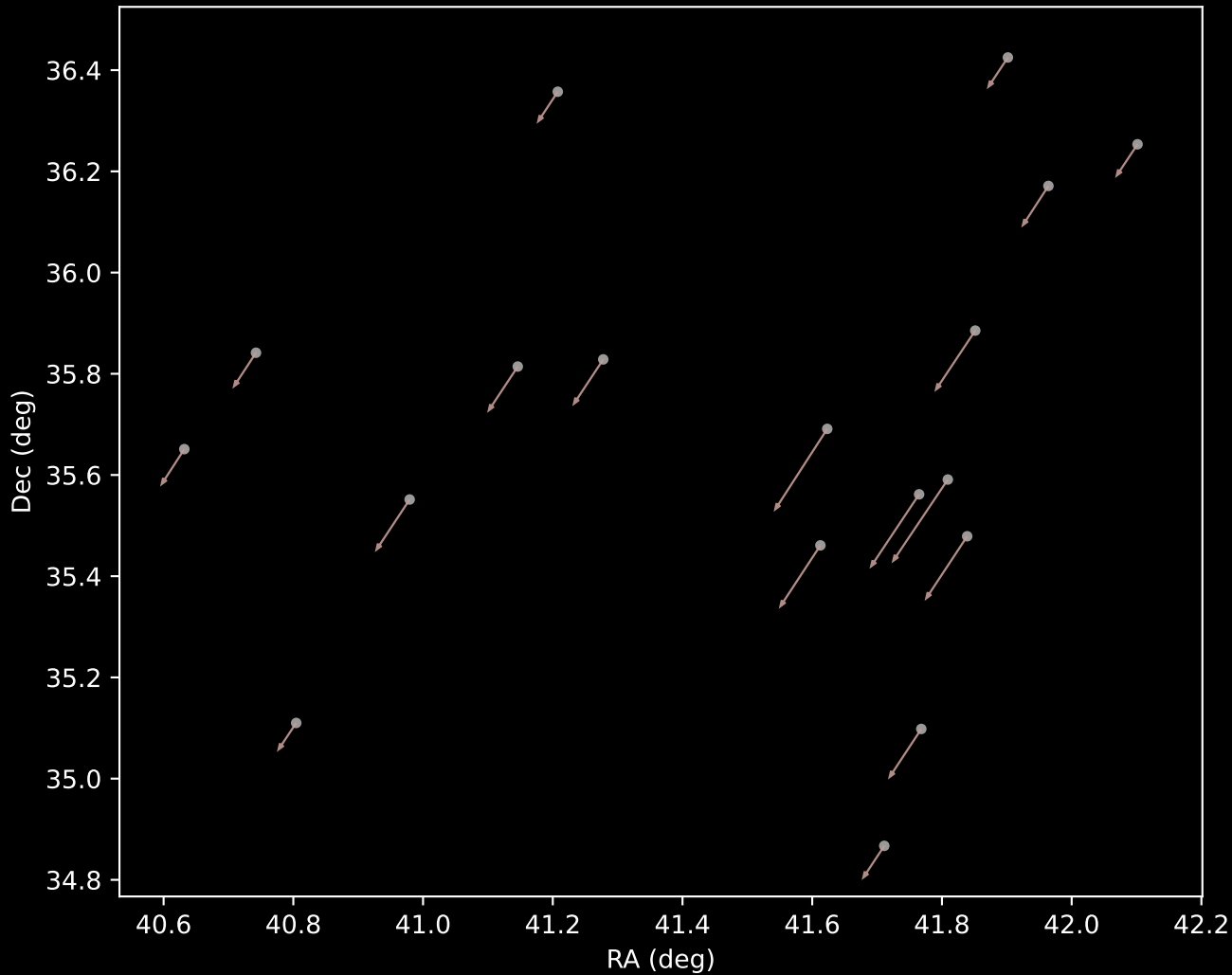
Gaia DR3 Cluster 71 Proper Motion Vectors (n=18)
