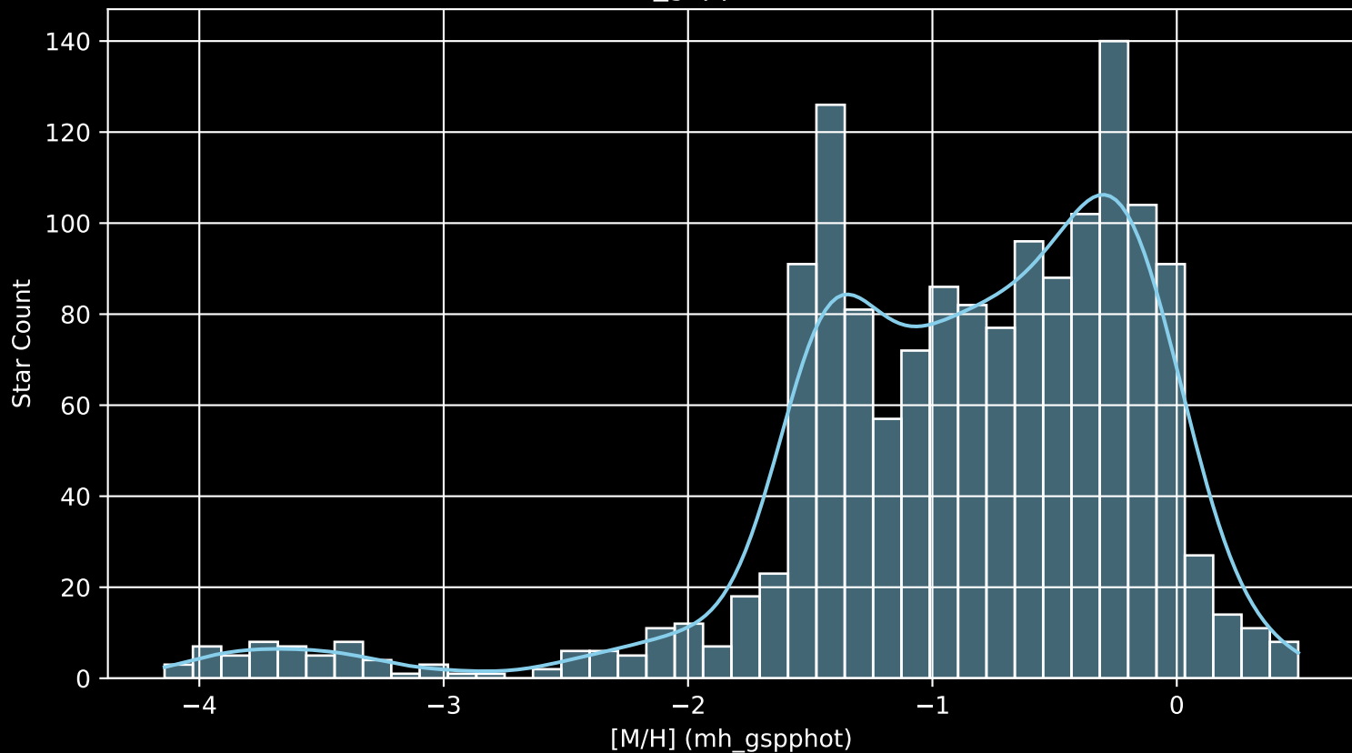
Gaia Cluster: [NGC_6871 [M/H] (mh_gspphot) (n= 1496)
