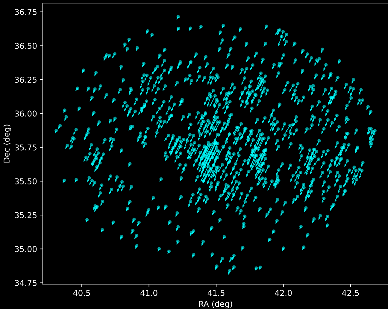
Gaia DR3 Noise Stream Proper Motion Vectors (n=658)
