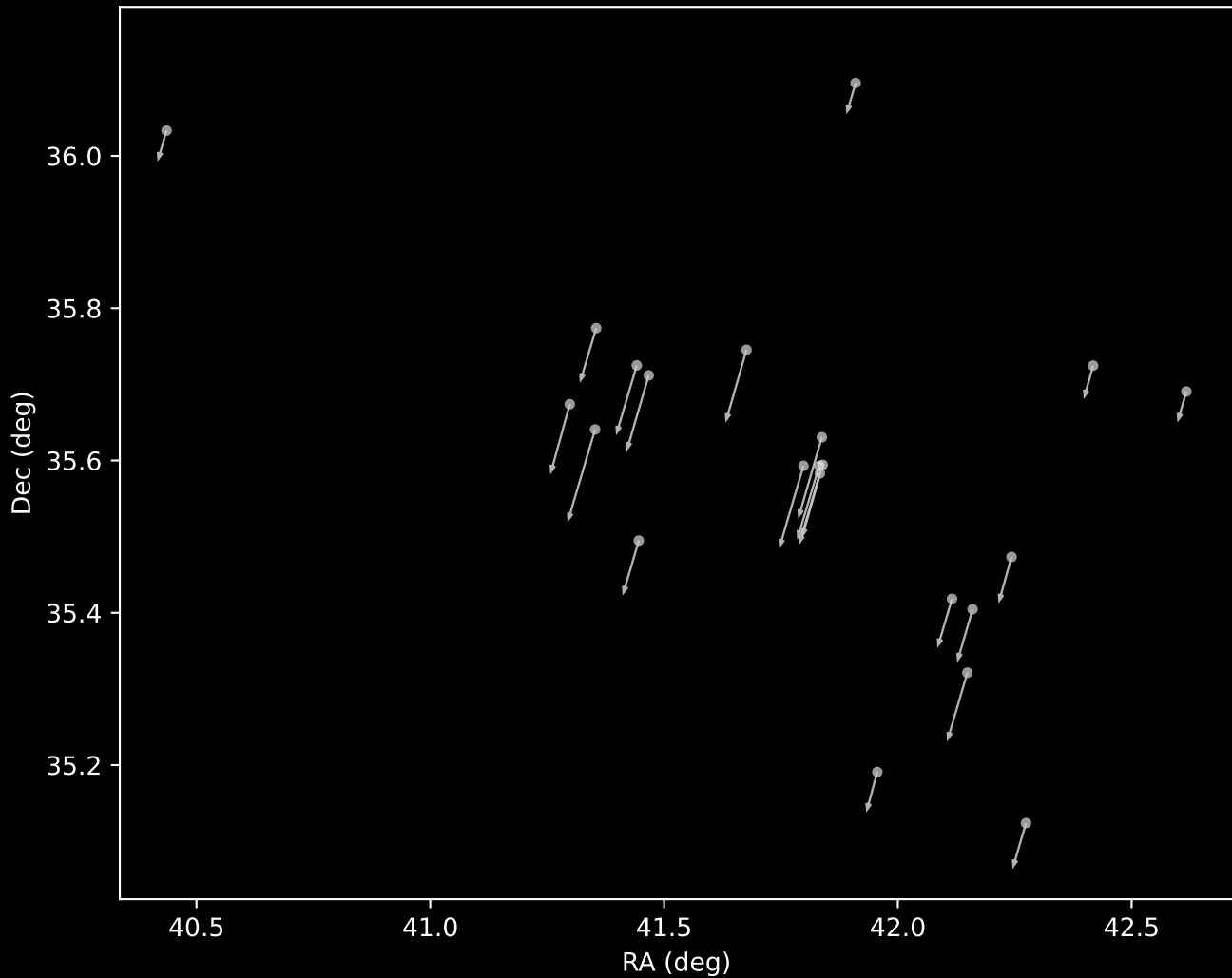
Gaia DR3 Cluster 15 Proper Motion Vectors (n=22)
