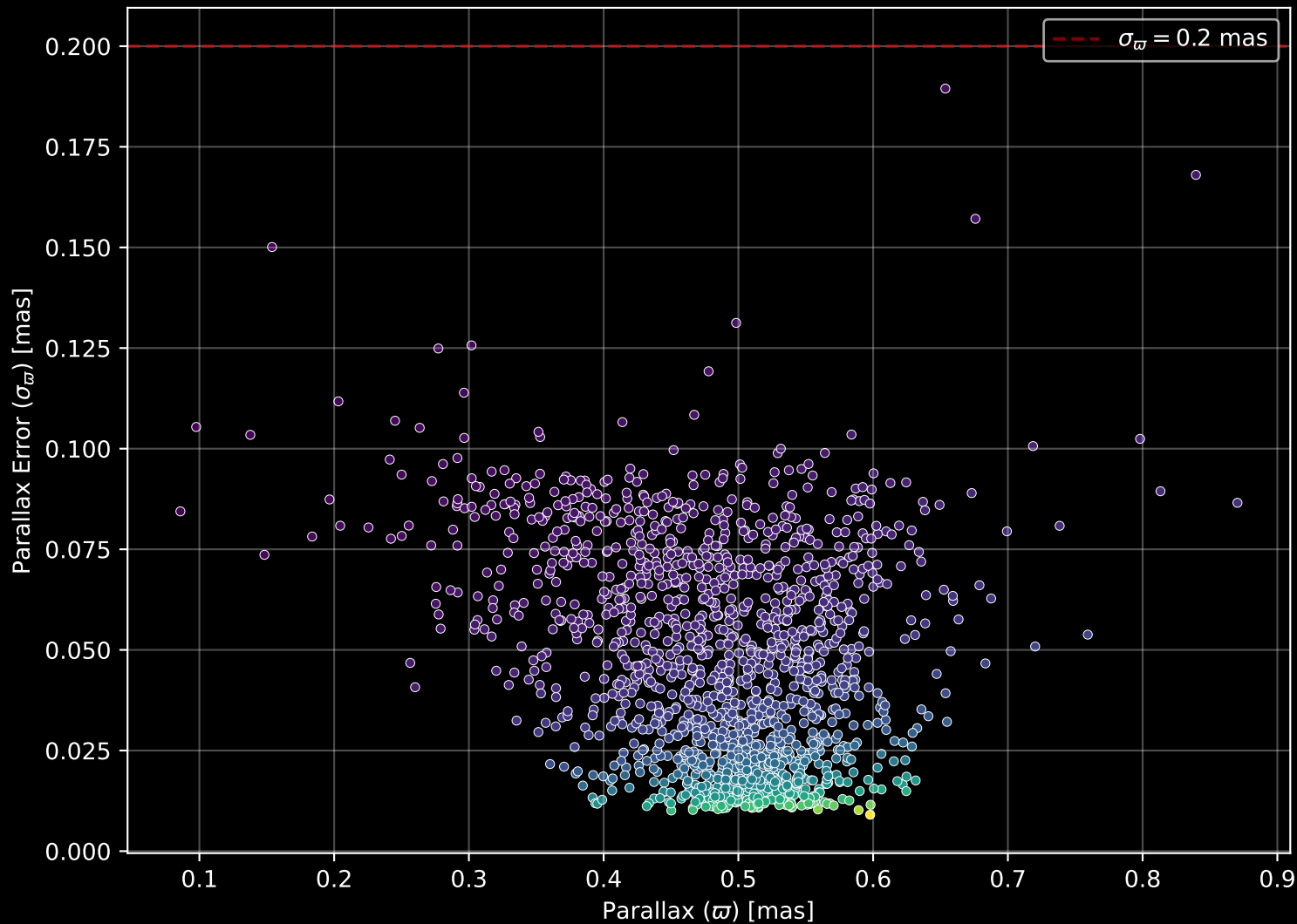
Gaia Cluster: [NGC_6871] Parallax Quality (n= 1497)
