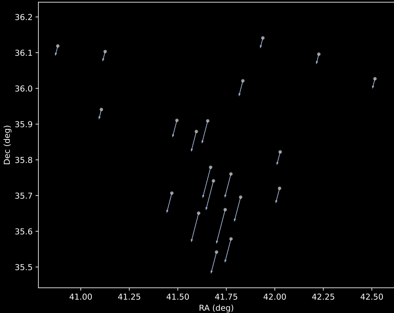
Gaia DR3 Cluster 81 Proper Motion Vectors (n=21)
