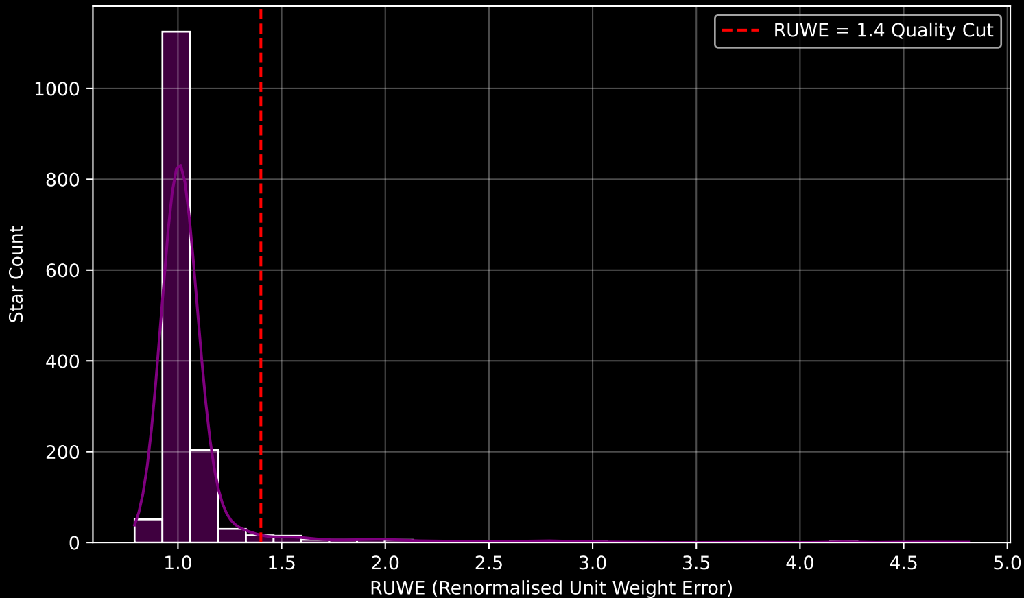
Gaia Cluster: [NGC_6871] RUWE Distribution (n= 1493)
