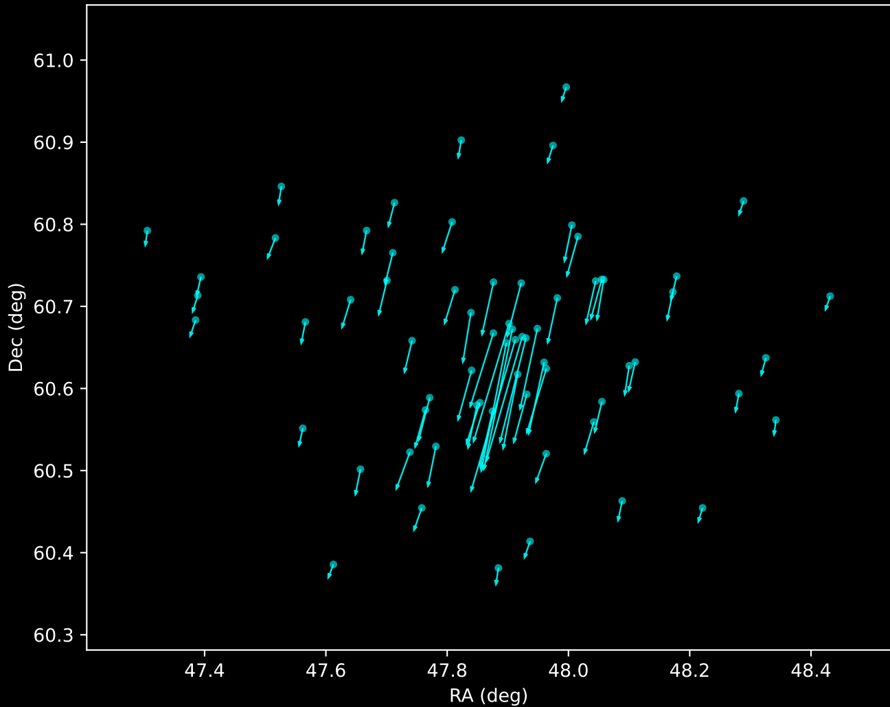
Gaia DR3 Noise Stream Proper Motion Vectors (n=67)
