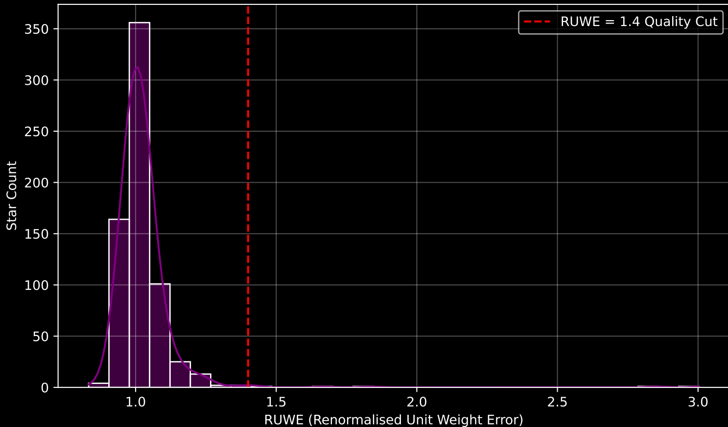
Gaia Cluster: [NGC_6939] RUWE Distribution (n= 672)
