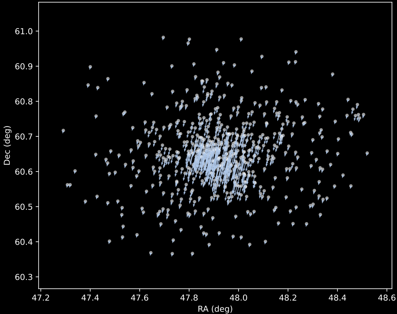
Gaia DR3 Cluster 1 Proper Motion Vectors (n=595)
