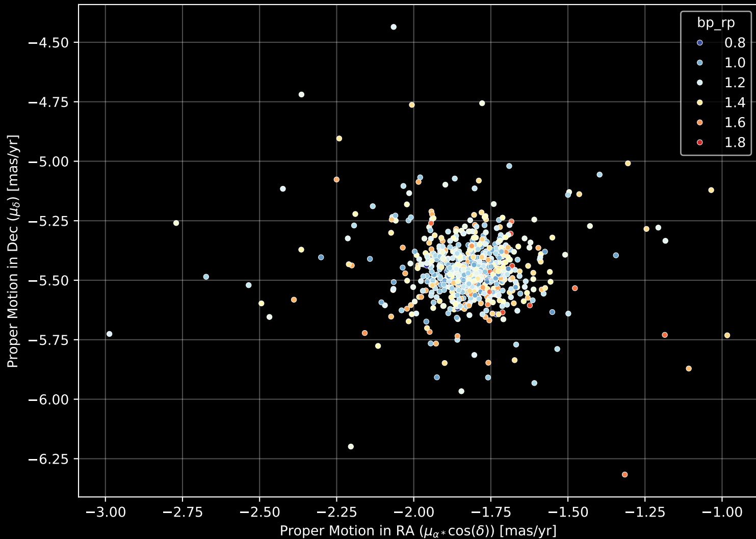
Gaia Cluster: [NGC_6939] Proper Motion Diagram (n= 673)
