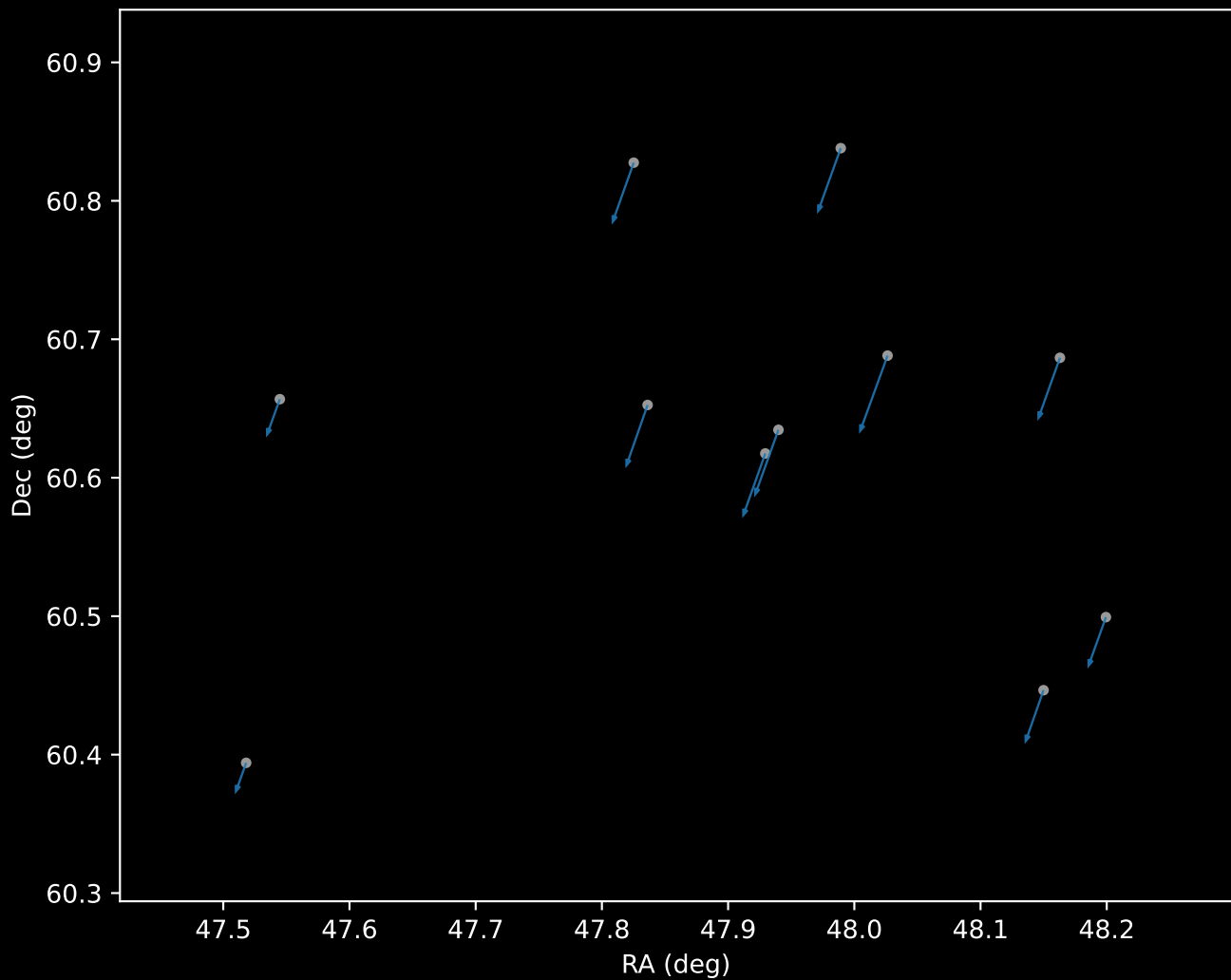
Gaia DR3 Cluster 0 Proper Motion Vectors (n=11)
