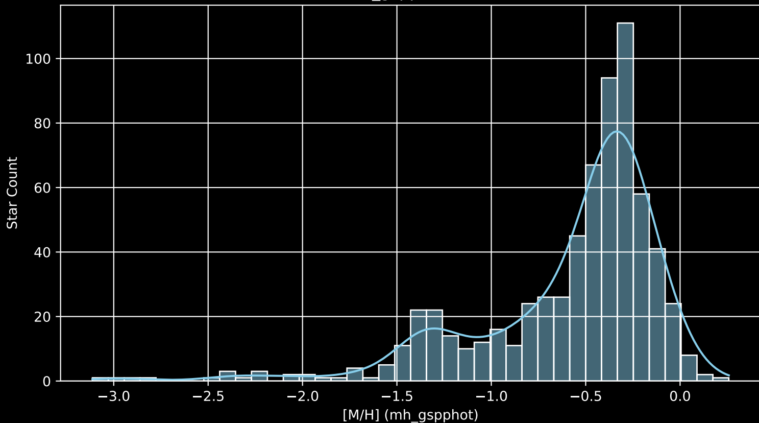
Gaia Cluster: [NGC_6939 [M/H] (mh_gspphot) (n= 673)
