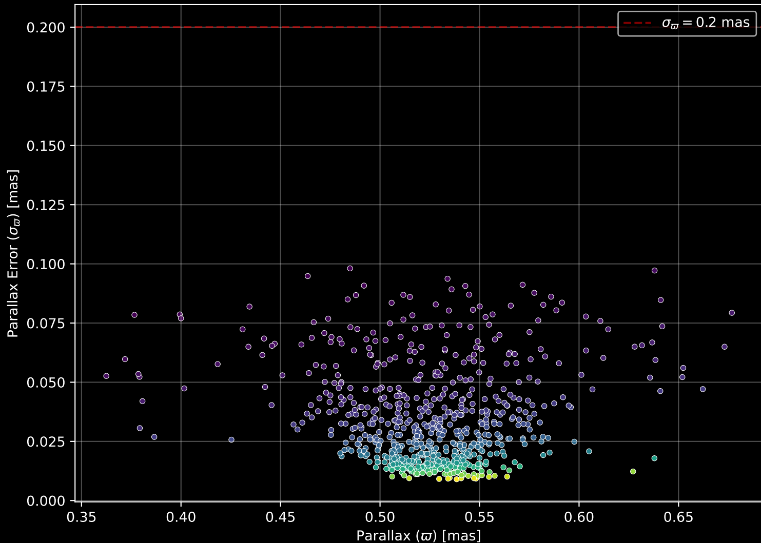
Gaia Cluster: [NGC_6939] Parallax Quality (n= 673)
