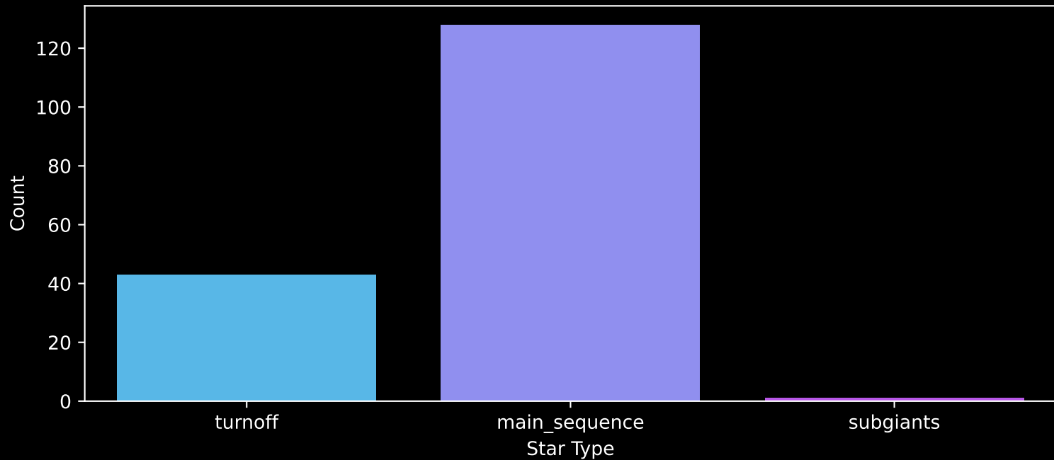
Gaia Cluster: [NGC_6997] Count plot of Star Type
