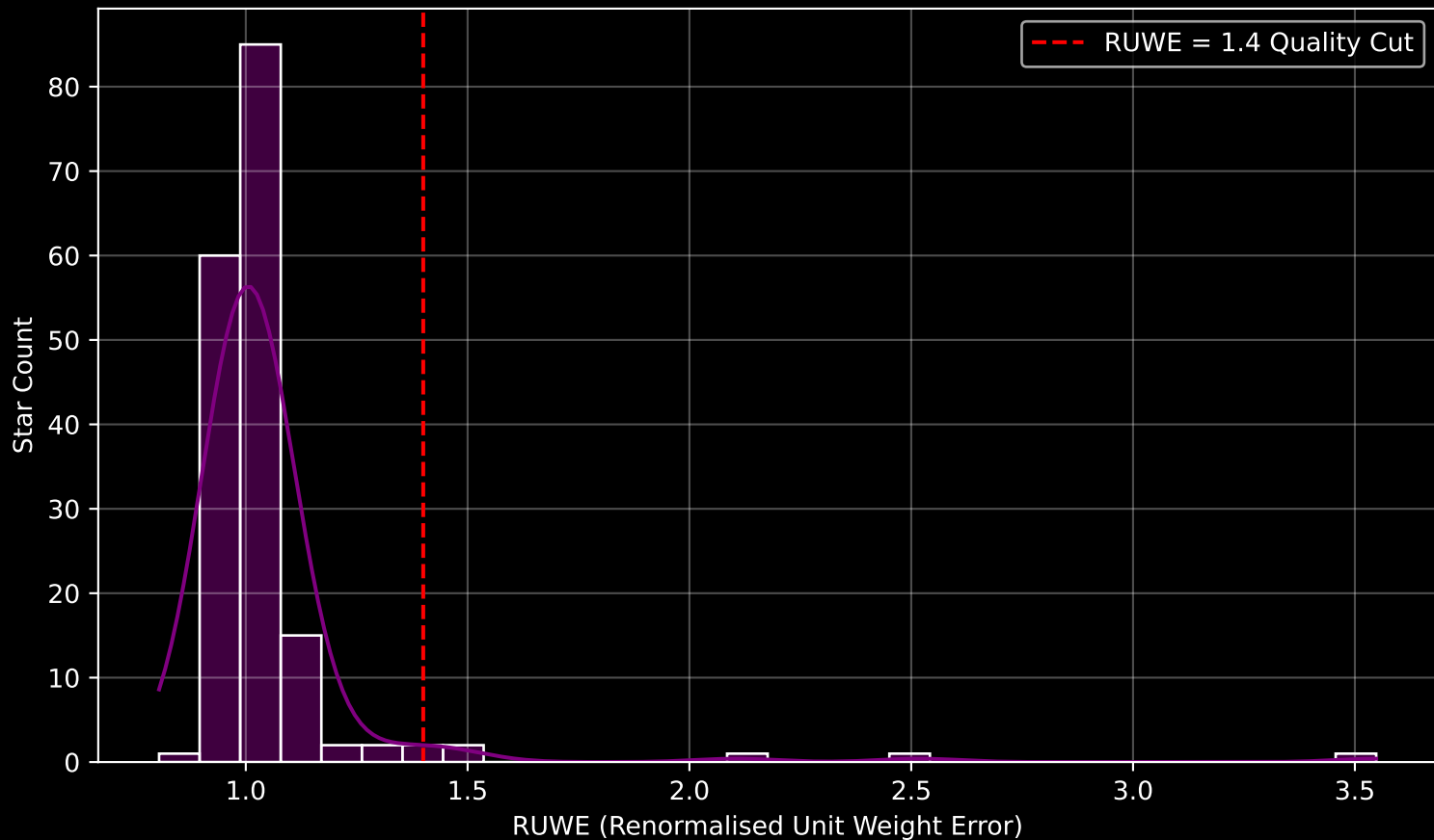
Gaia Cluster: [NGC_6997] RUWE Distribution (n= 172)
