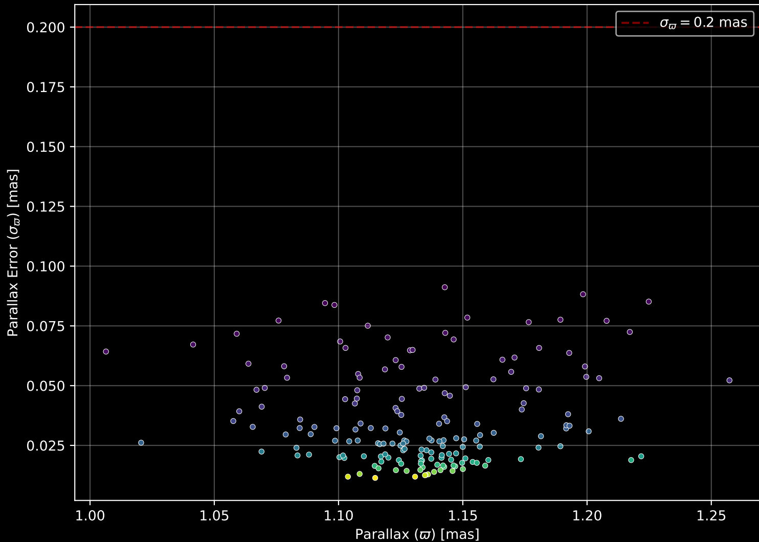
Gaia Cluster: [NGC_6997] Parallax Quality (n= 172)
