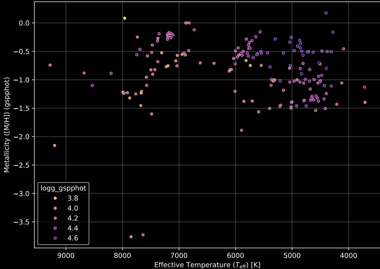
Gaia Cluster: [NGC_6997] Stellar Population Parameters (n= 172)
