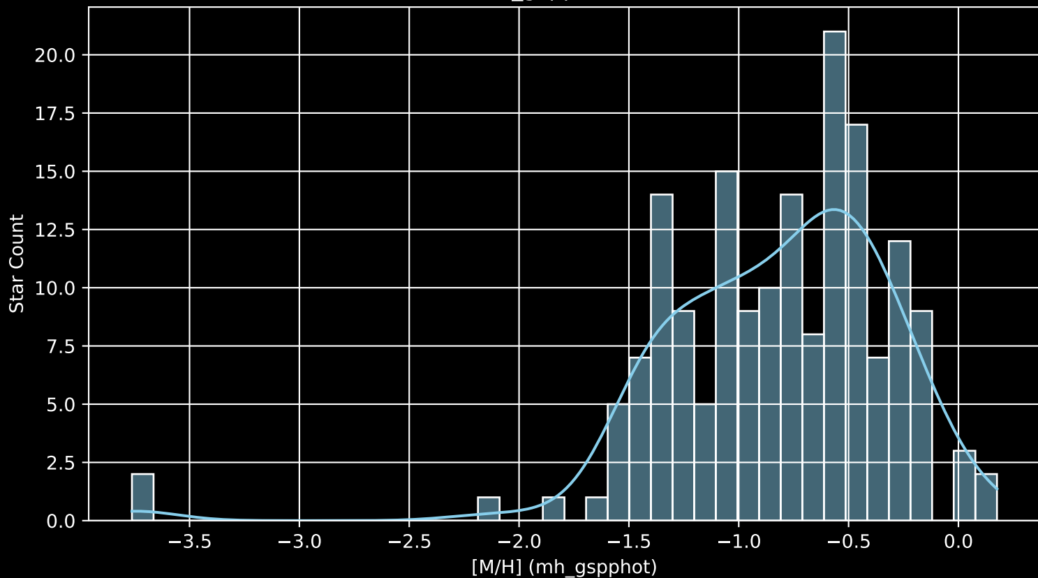
Gaia Cluster: [NGC_6997 [M/H] (mh_gspphot) (n= 172)
