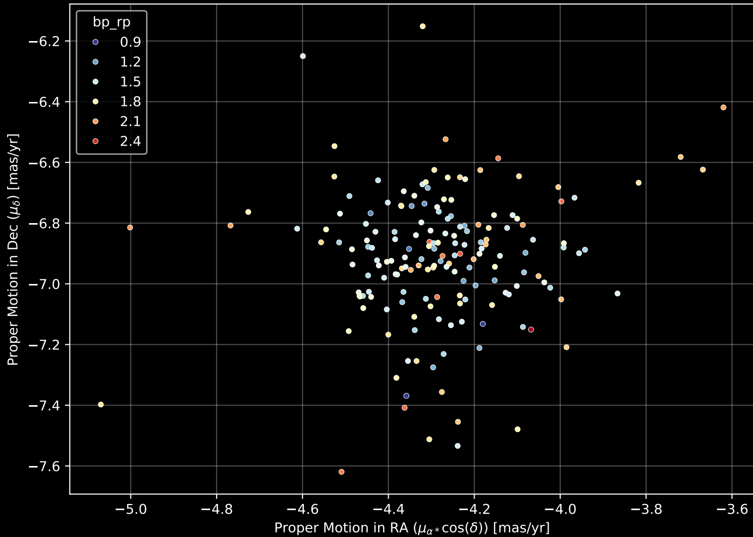
Gaia Cluster: [NGC_6997] Proper Motion Diagram (n= 172)
