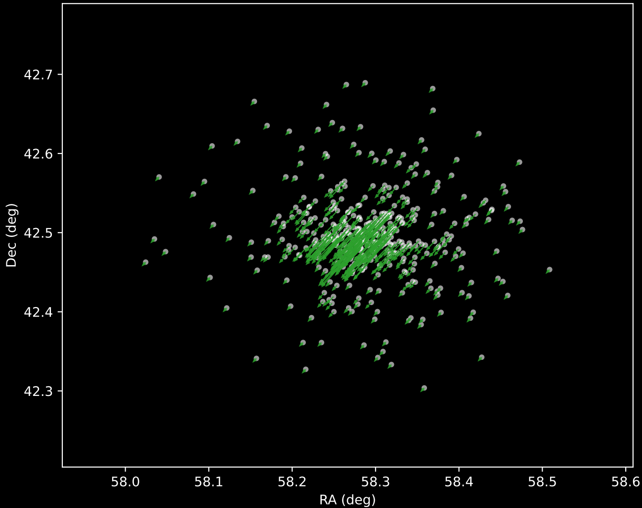
Gaia DR3 Cluster 4 Proper Motion Vectors (n=426)
