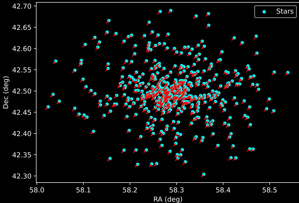
Gaia Cluster: [NGC_7044] Proper Motion Vectors for Gaia Star Field (n= 515)
