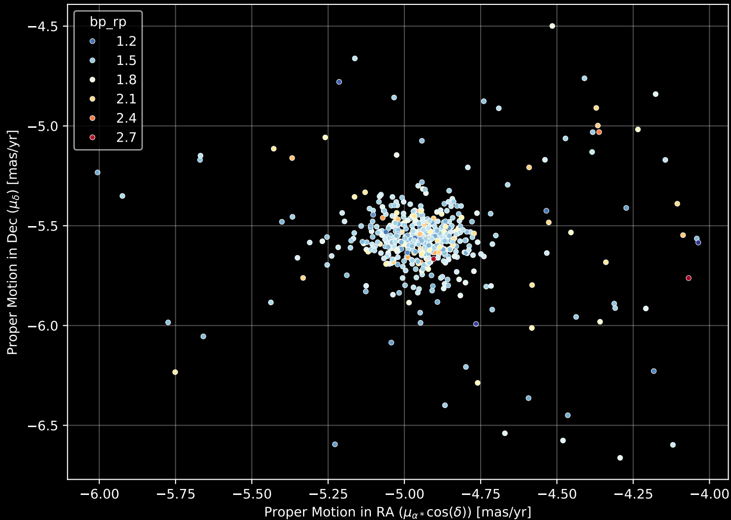
Gaia Cluster: [NGC_7044] Proper Motion Diagram (n= 515)
