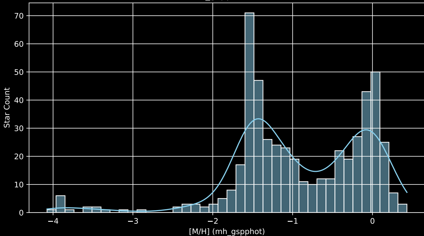
Gaia Cluster: [NGC_7044 [M/H] (mh_gspphot) (n= 509)
