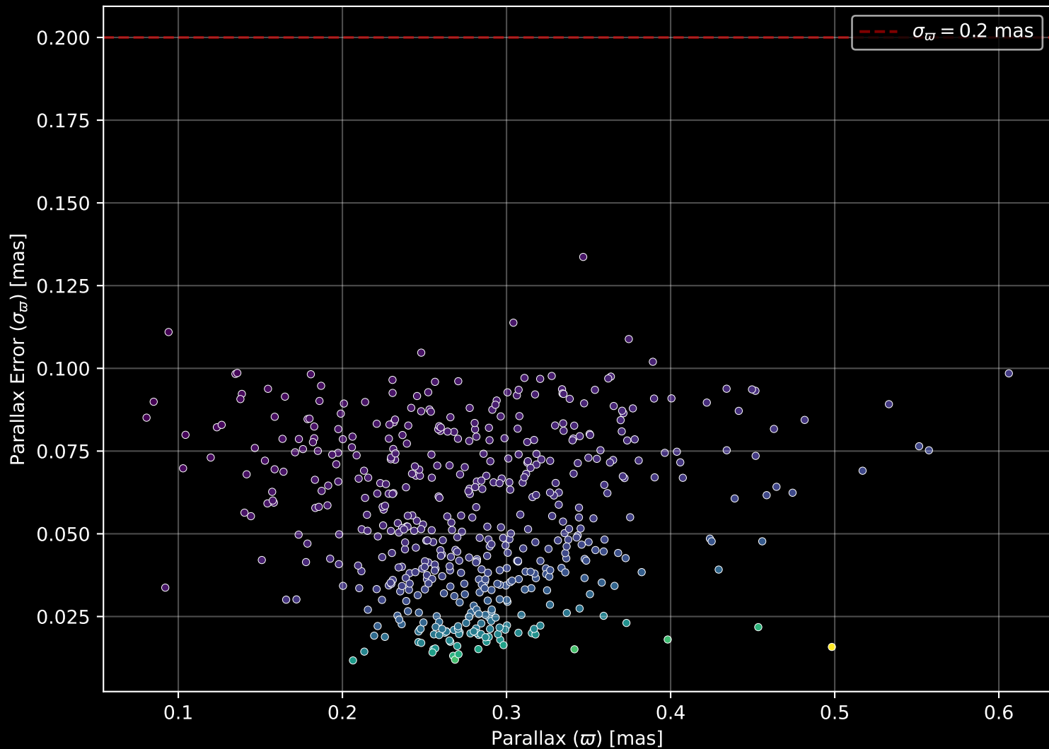
Gaia Cluster: [NGC_7044] Parallax Quality (n= 515)
