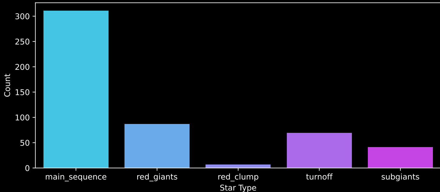
Gaia Cluster: [NGC_7044] Count plot of Star Type
