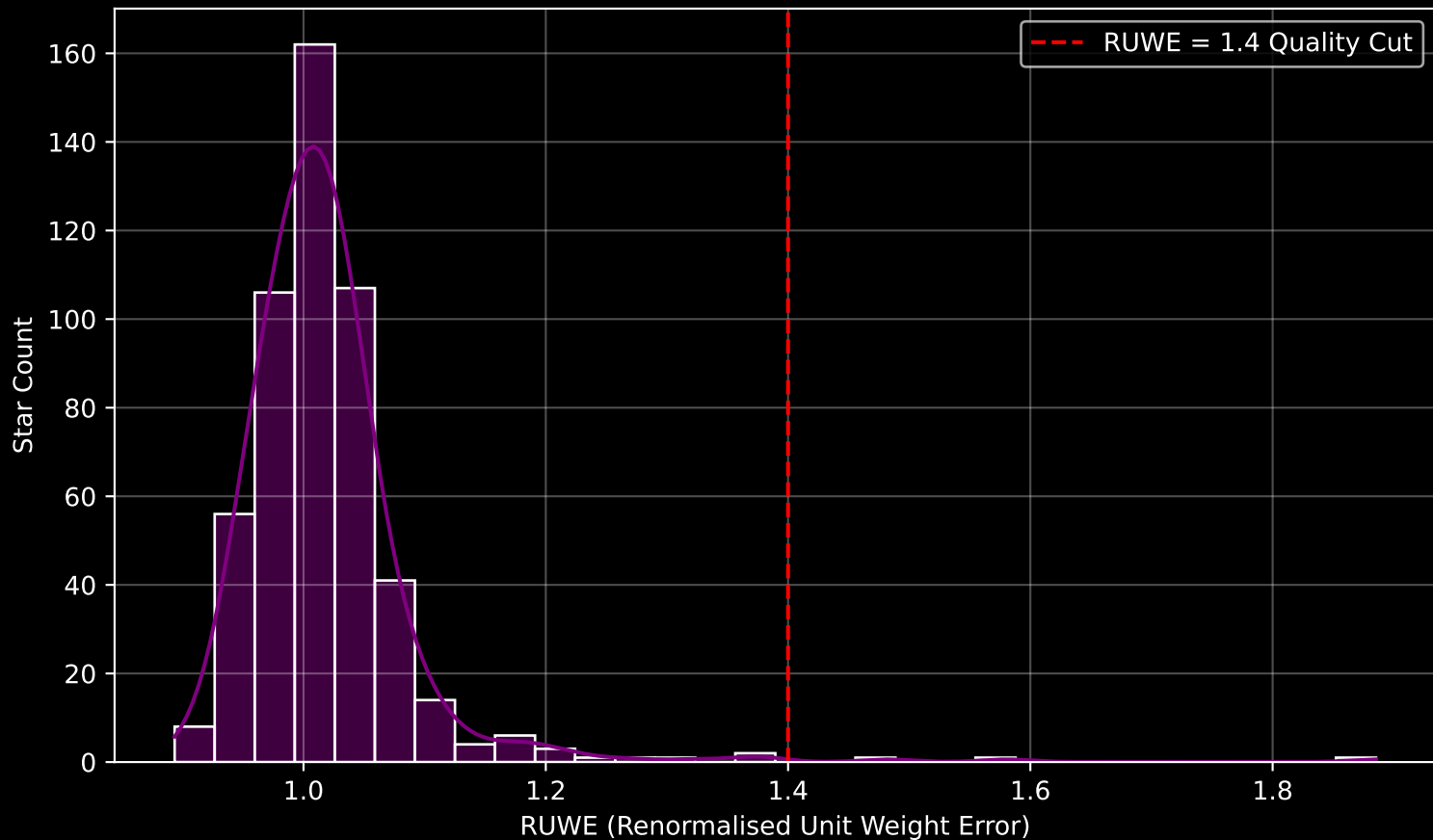
Gaia Cluster: [NGC_7044] RUWE Distribution (n= 515)
