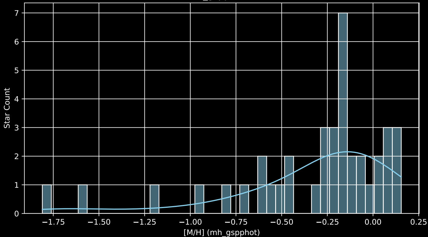
Gaia Cluster: [NGC_7058 [M/H] (mh_gspphot) (n= 39)
