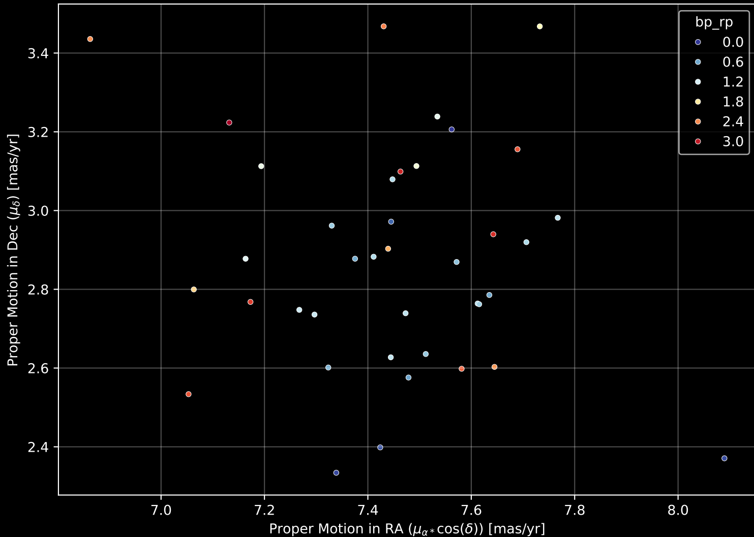
Gaia Cluster: [NGC_7058] Proper Motion Diagram (n= 39)
