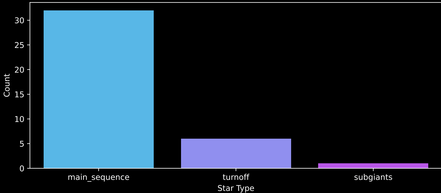
Gaia Cluster: [NGC_7058] Count plot of Star Type
