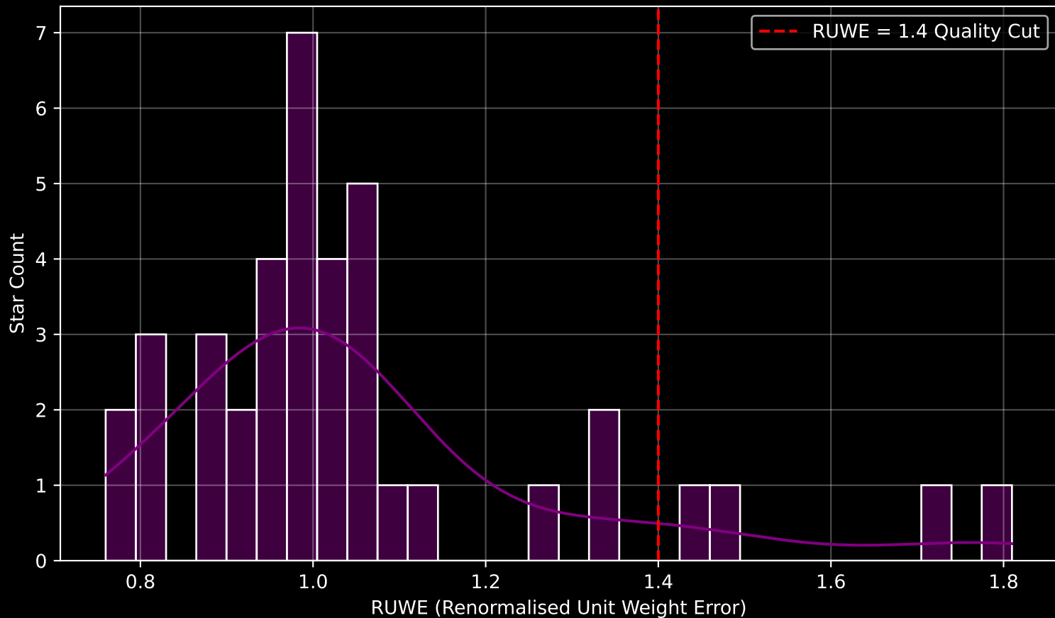
Gaia Cluster: [NGC_7058] RUWE Distribution (n= 39)
