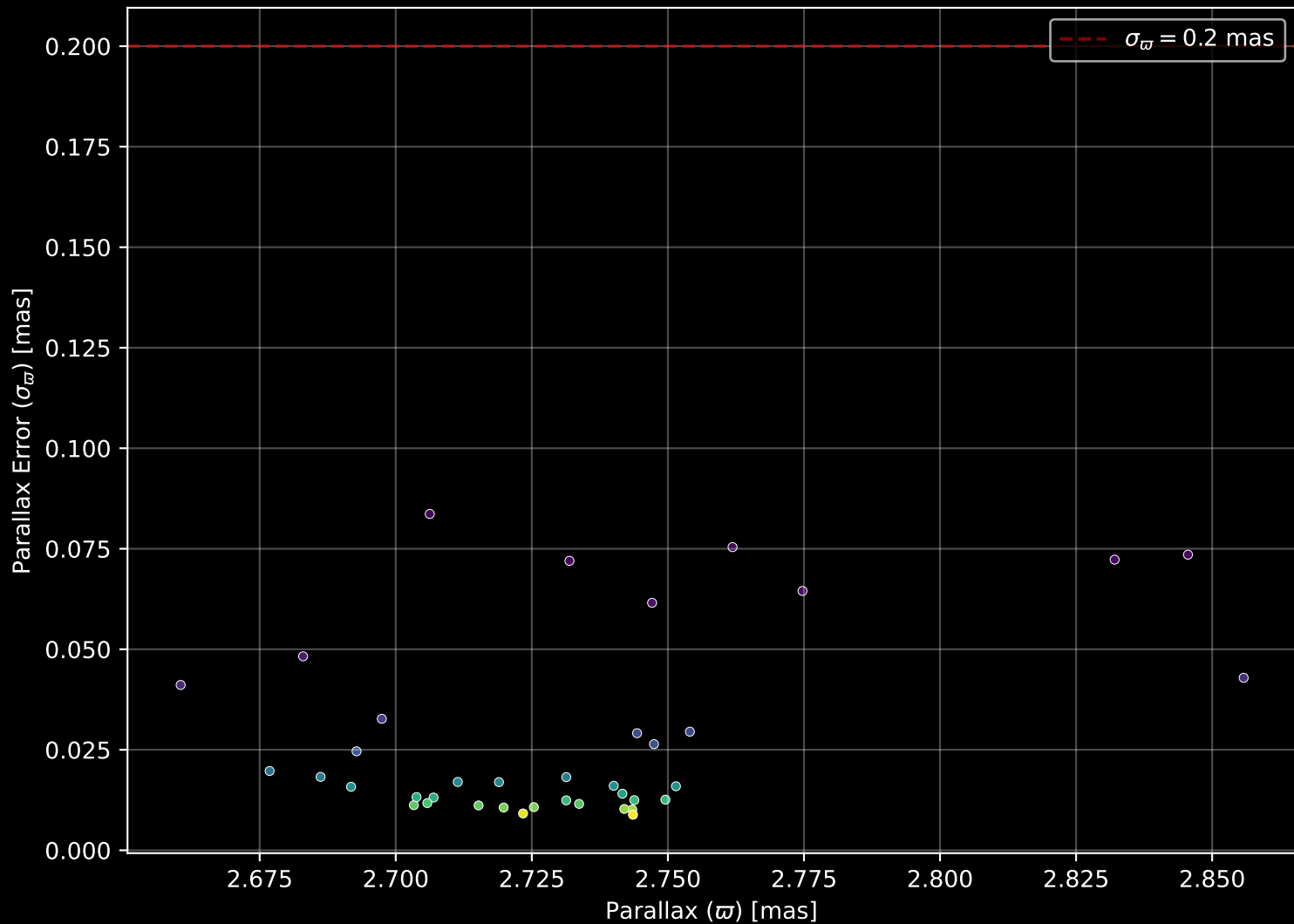
Gaia Cluster: [NGC_7058] Parallax Quality (n= 39)
