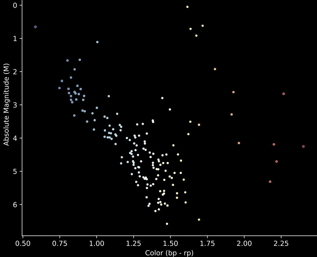
Gaia Cluster: [NGC_7062] Stars (n= 162) Hertzsprung-Russel Diagram
