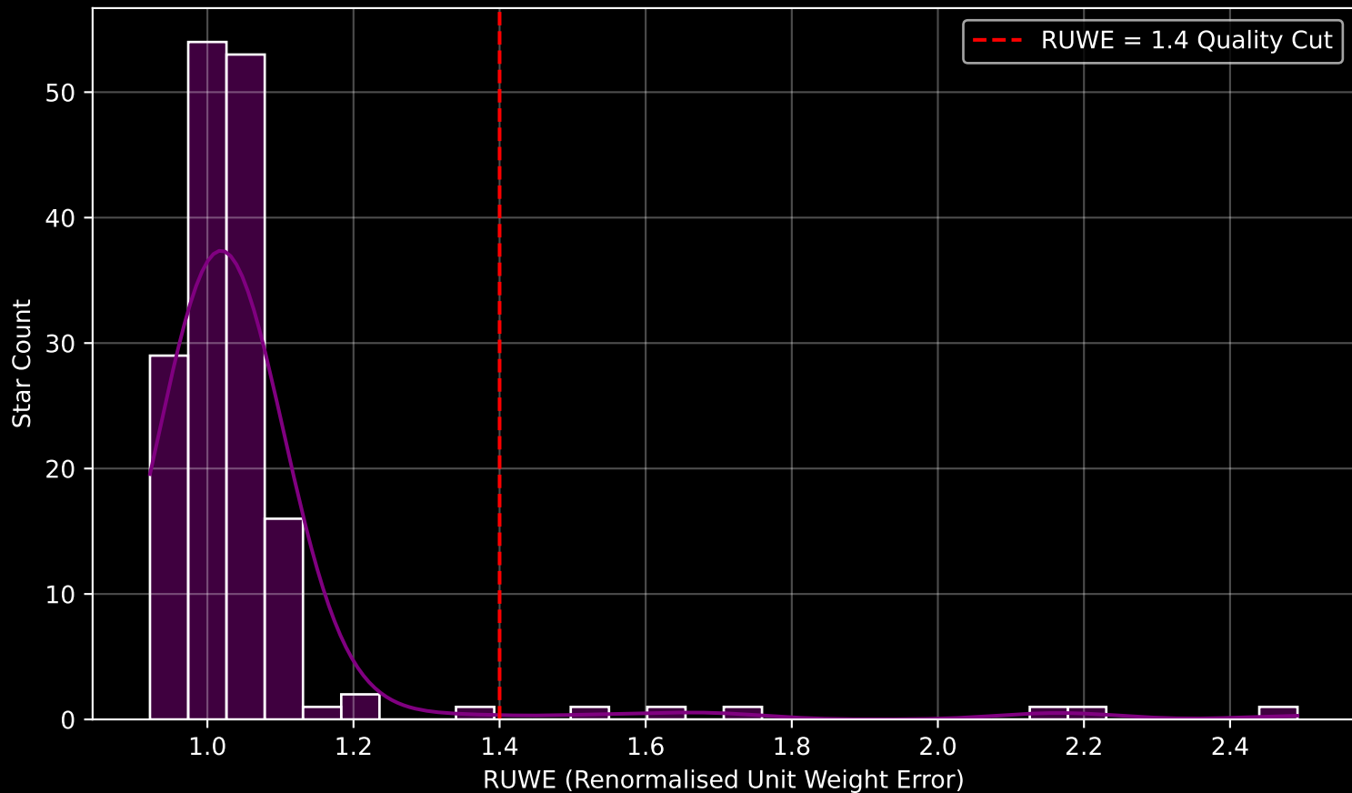
Gaia Cluster: [NGC_7062] RUWE Distribution (n= 162)
