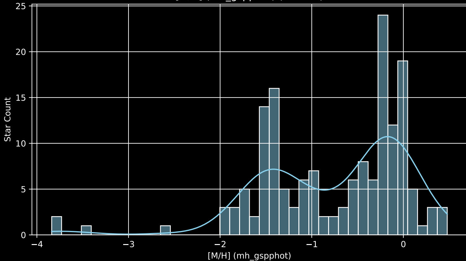
Gaia Cluster: [NGC_7062 [M/H] (mh_gspphot) (n= 162)
