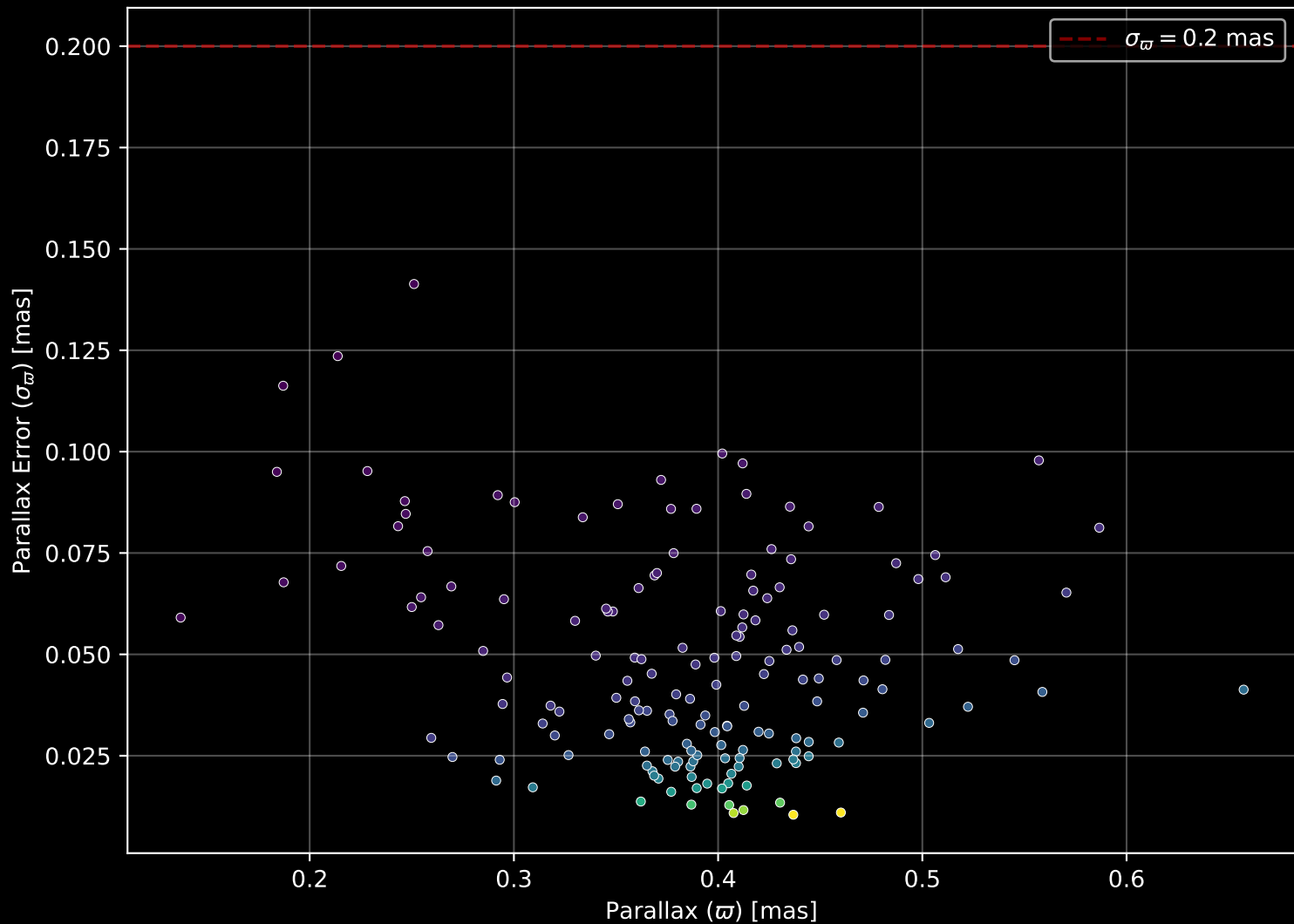
Gaia Cluster: [NGC_7062] Parallax Quality (n= 162)
