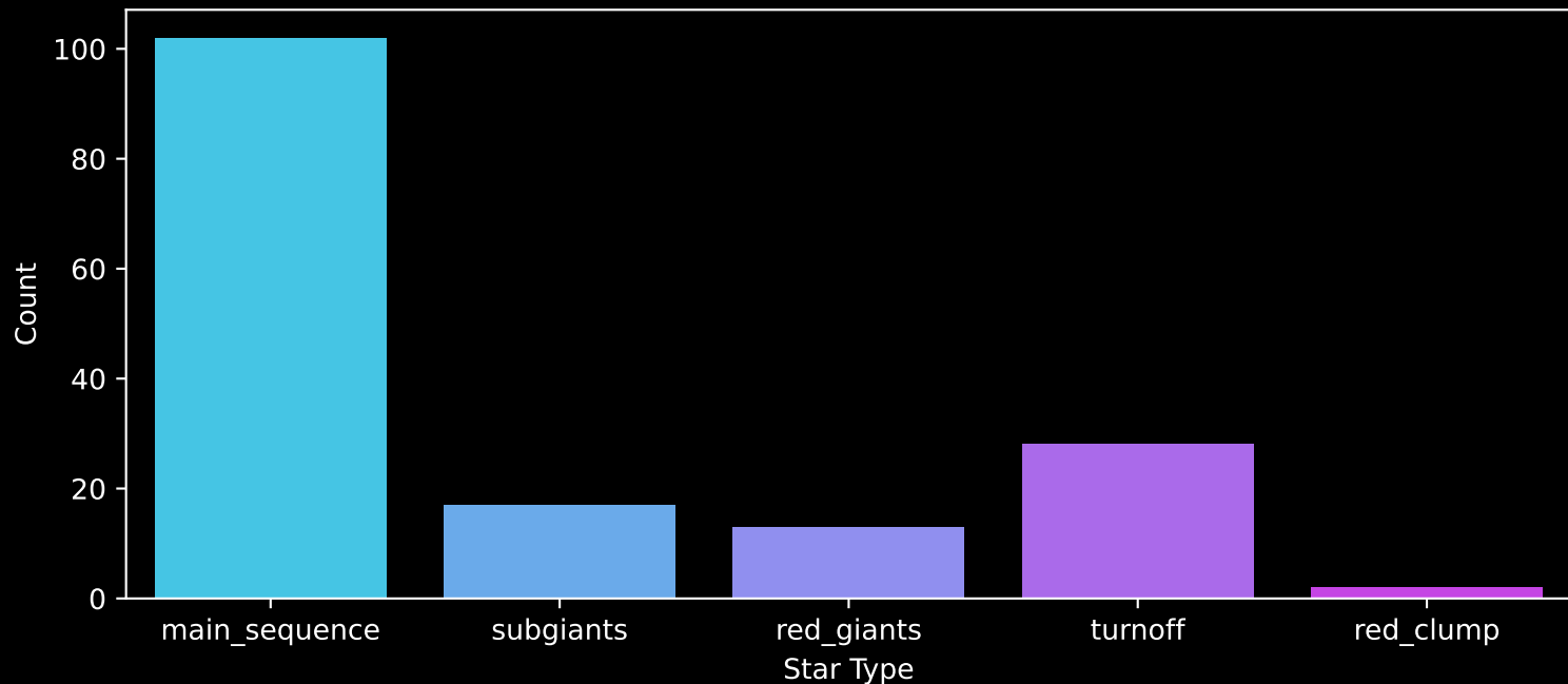
Gaia Cluster: [NGC_7062] Count plot of Star Type
