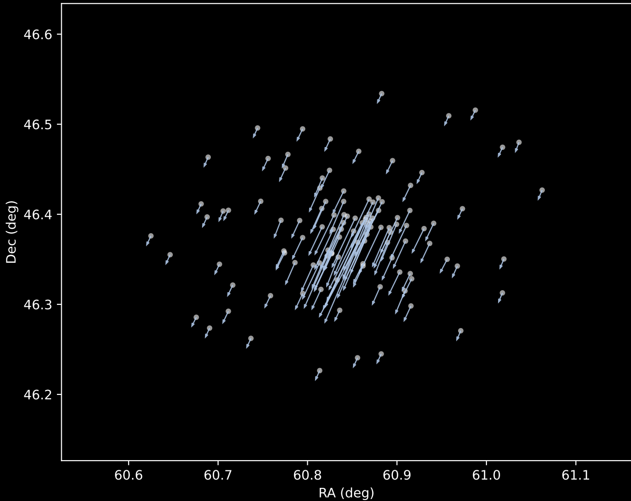
Gaia DR3 Cluster 1 Proper Motion Vectors (n=111)
