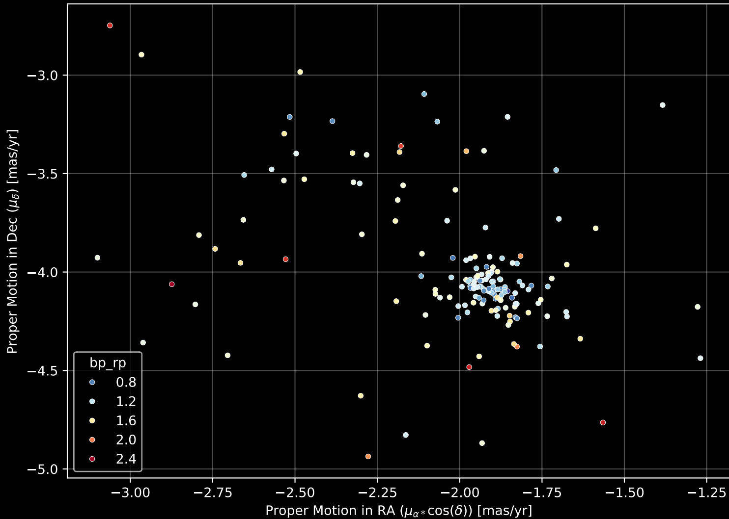
Gaia Cluster: [NGC_7062] Proper Motion Diagram (n= 162)
