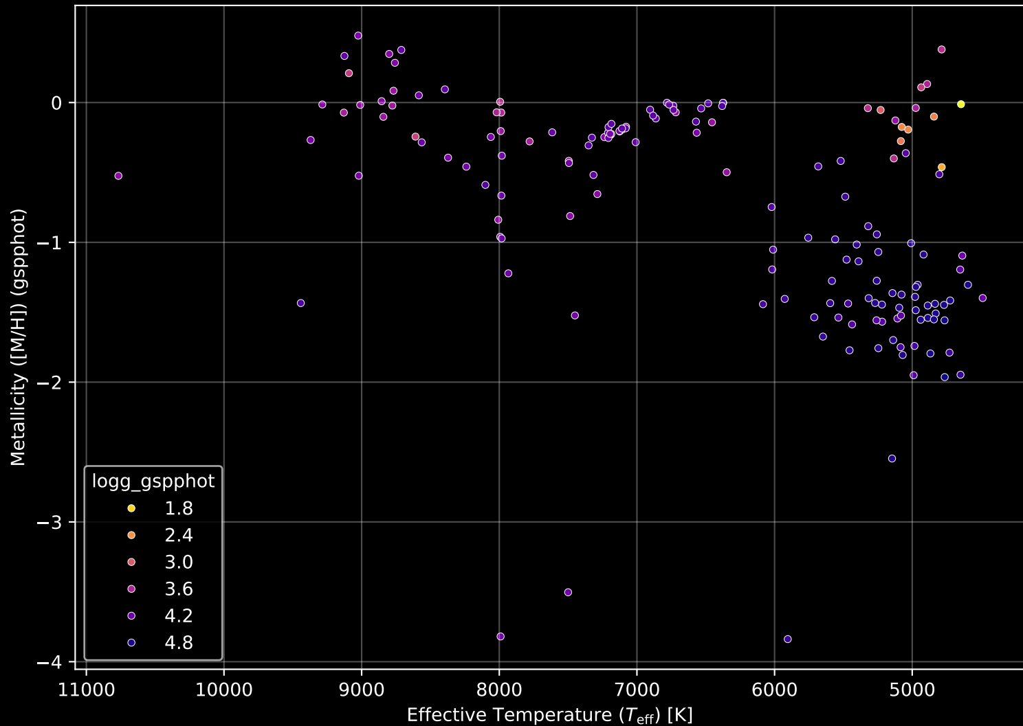
Gaia Cluster: [NGC_7062] Stellar Population Parameters (n= 162)
