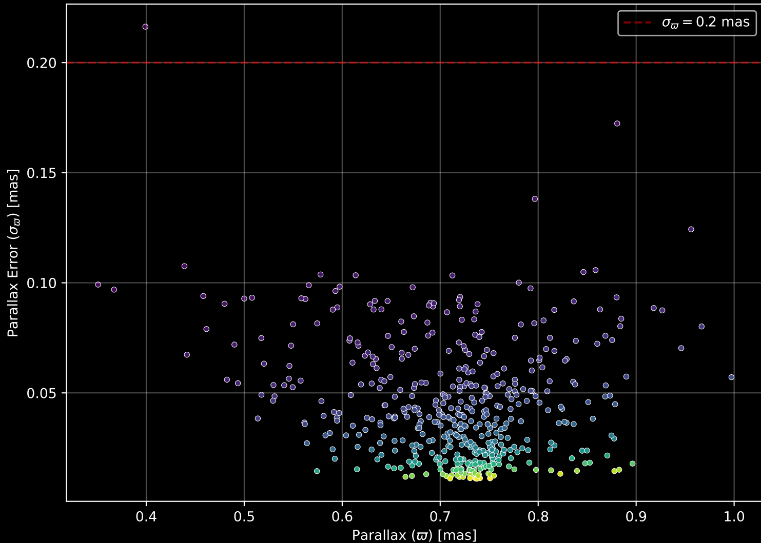
Gaia Cluster: [NGC_7082] Parallax Quality (n= 474)
