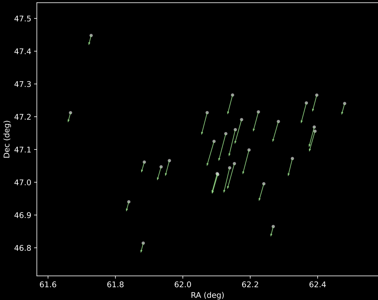
Gaia DR3 Cluster 25 Proper Motion Vectors (n=28)
