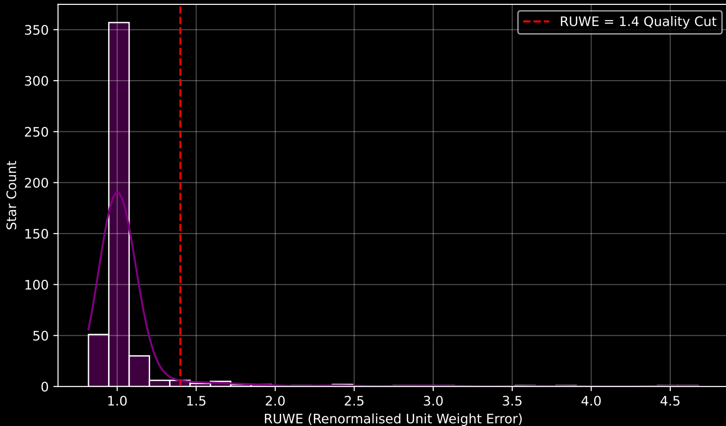
Gaia Cluster: [NGC_7082] RUWE Distribution (n= 472)
