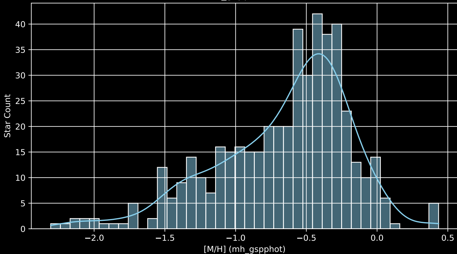
Gaia Cluster: [NGC_7082 [M/H] (mh_gspphot) (n= 474)
