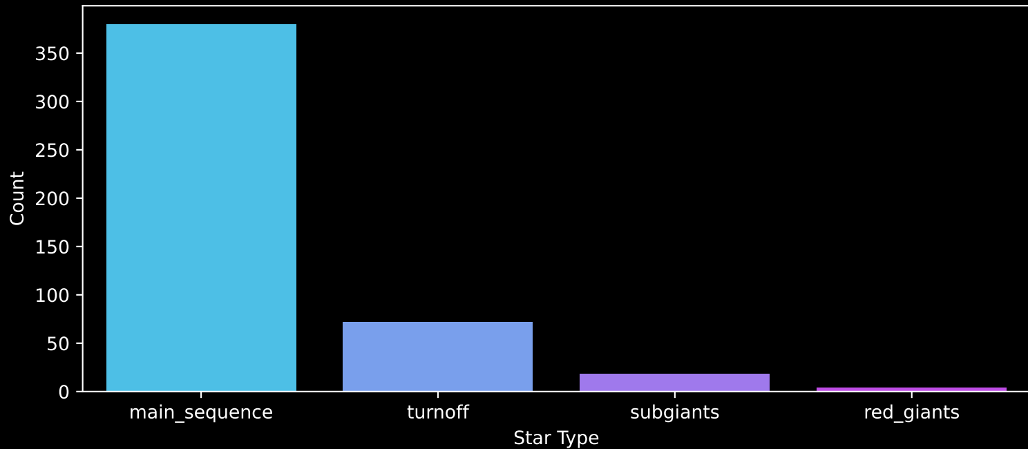
Gaia Cluster: [NGC_7082] Count plot of Star Type
