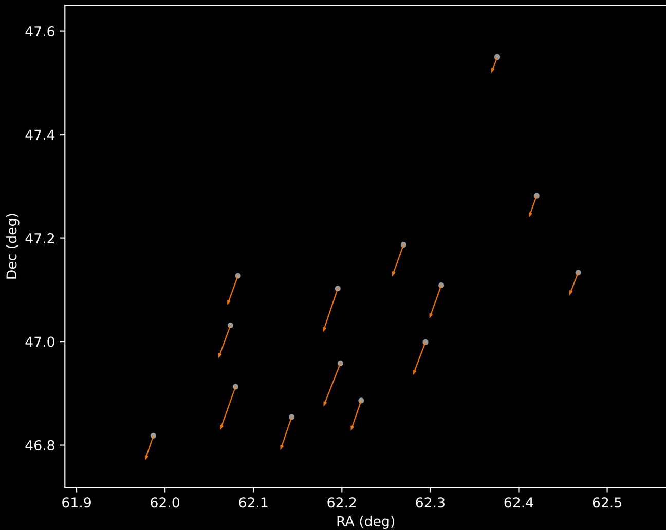
Gaia DR3 Cluster 22 Proper Motion Vectors (n=14)
