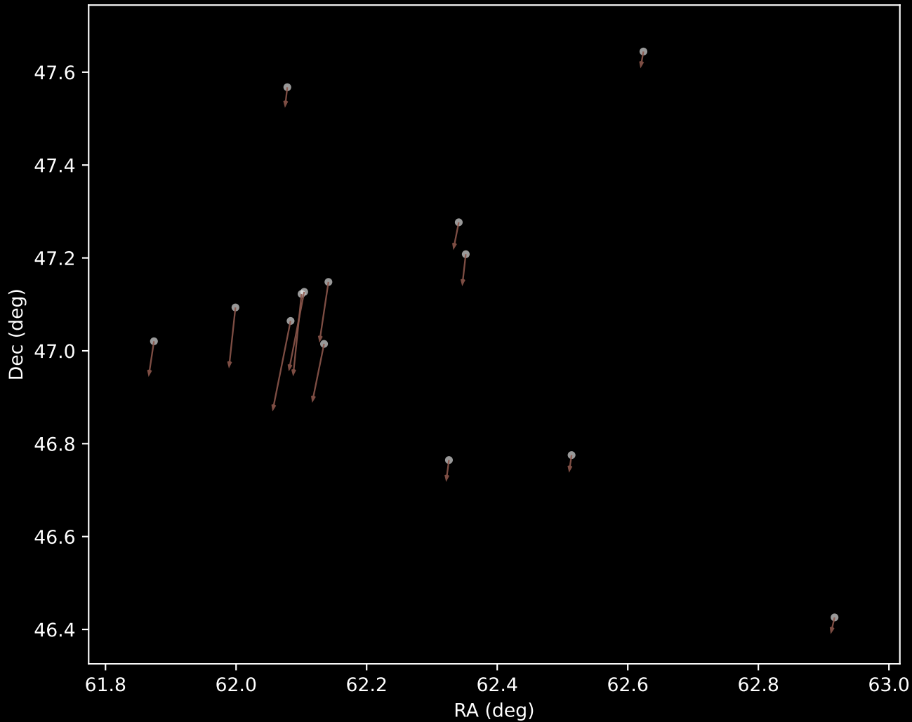
Gaia DR3 Cluster 10 Proper Motion Vectors (n=14)
