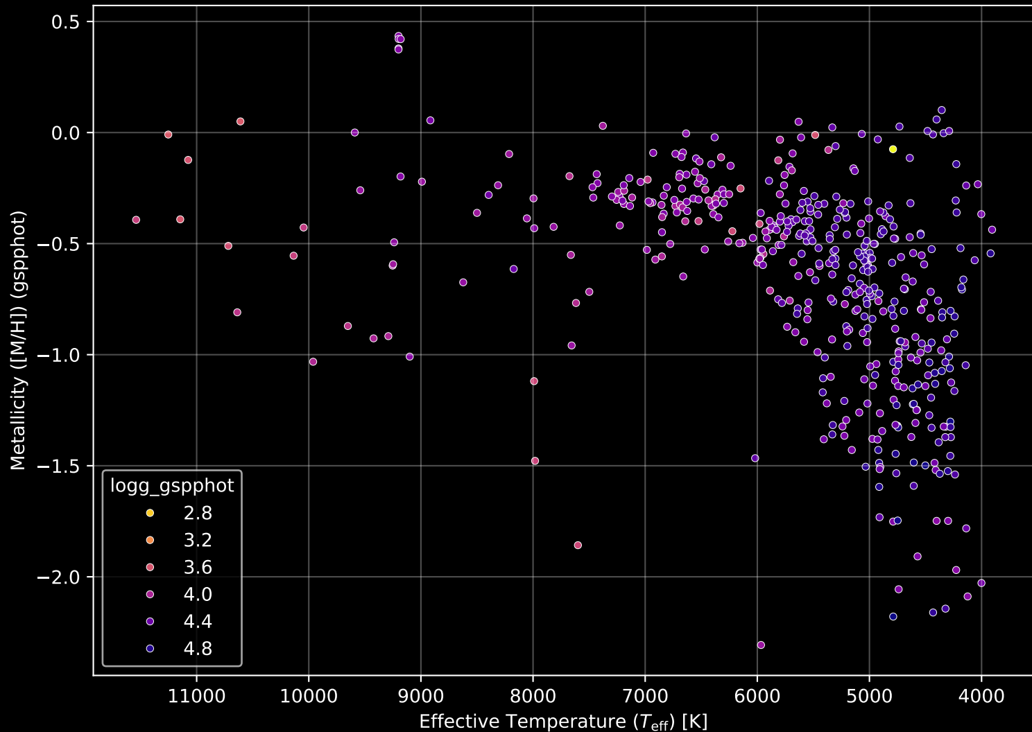
Gaia Cluster: [NGC_7082] Stellar Population Parameters (n= 474)
