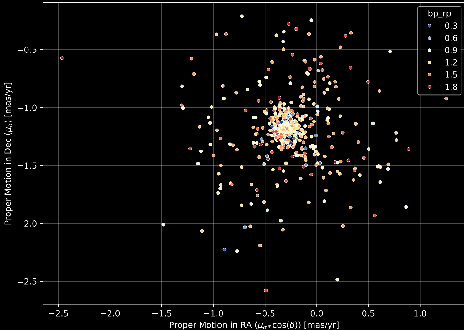
Gaia Cluster: [NGC_7082] Proper Motion Diagram (n= 474)
