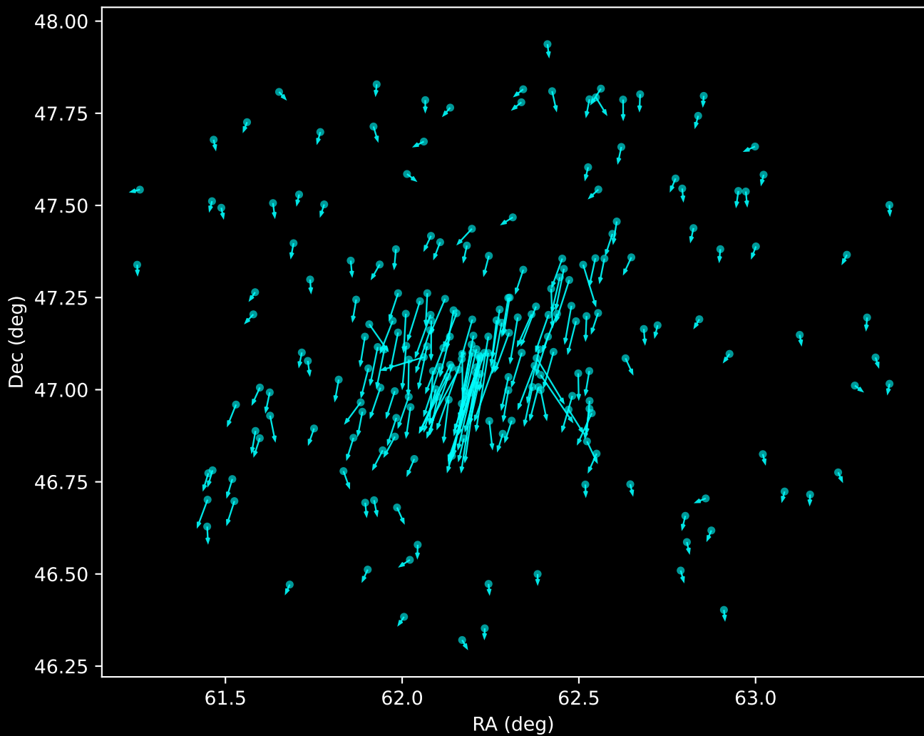
Gaia DR3 Noise Stream Proper Motion Vectors (n=223)
