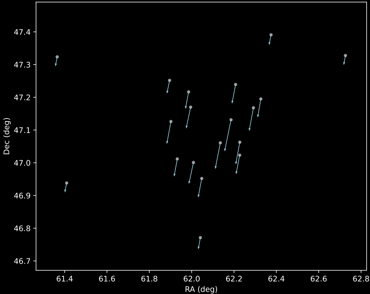
Gaia DR3 Cluster 19 Proper Motion Vectors (n=19)
