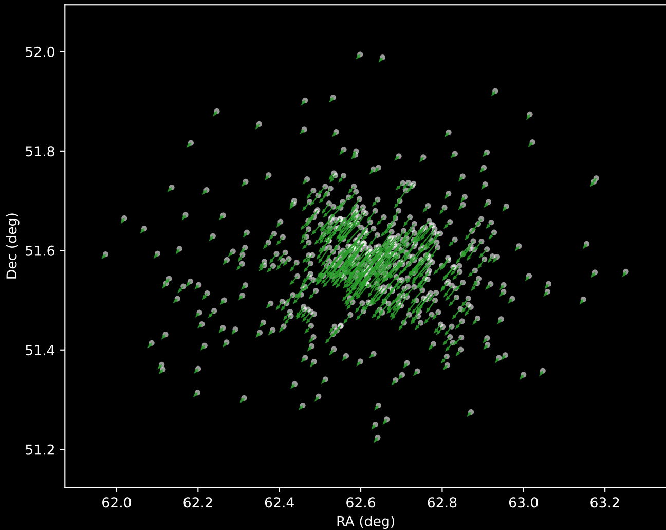
Gaia DR3 Cluster 4 Proper Motion Vectors (n=482)
