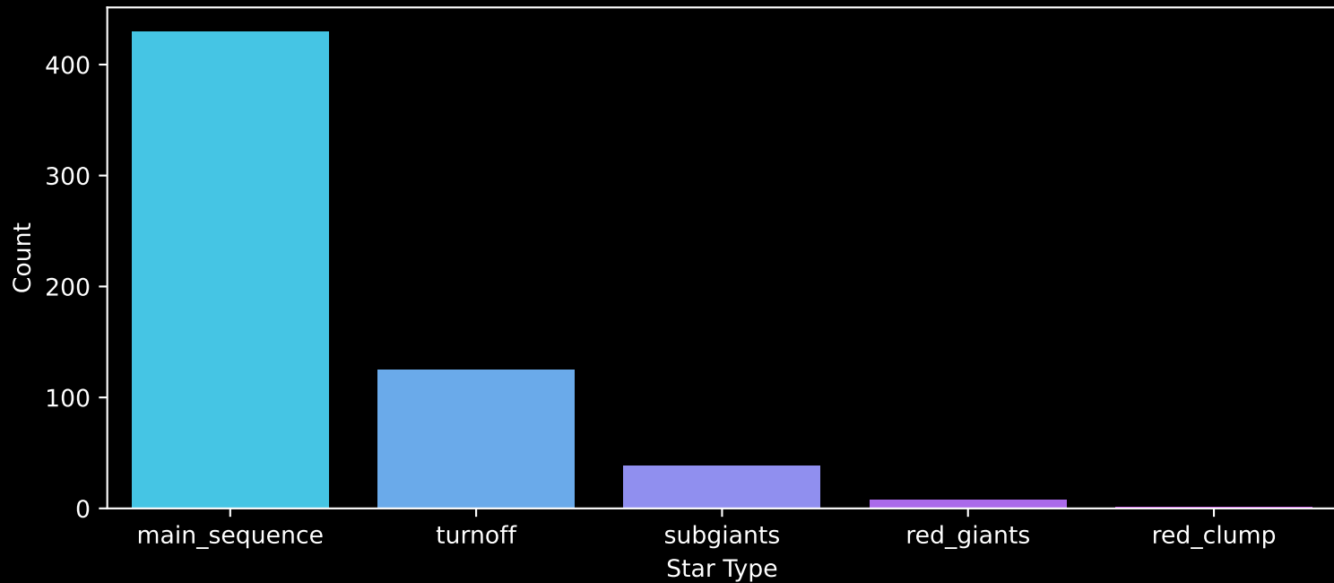
Gaia Cluster: [NGC_7086] Count plot of Star Type
