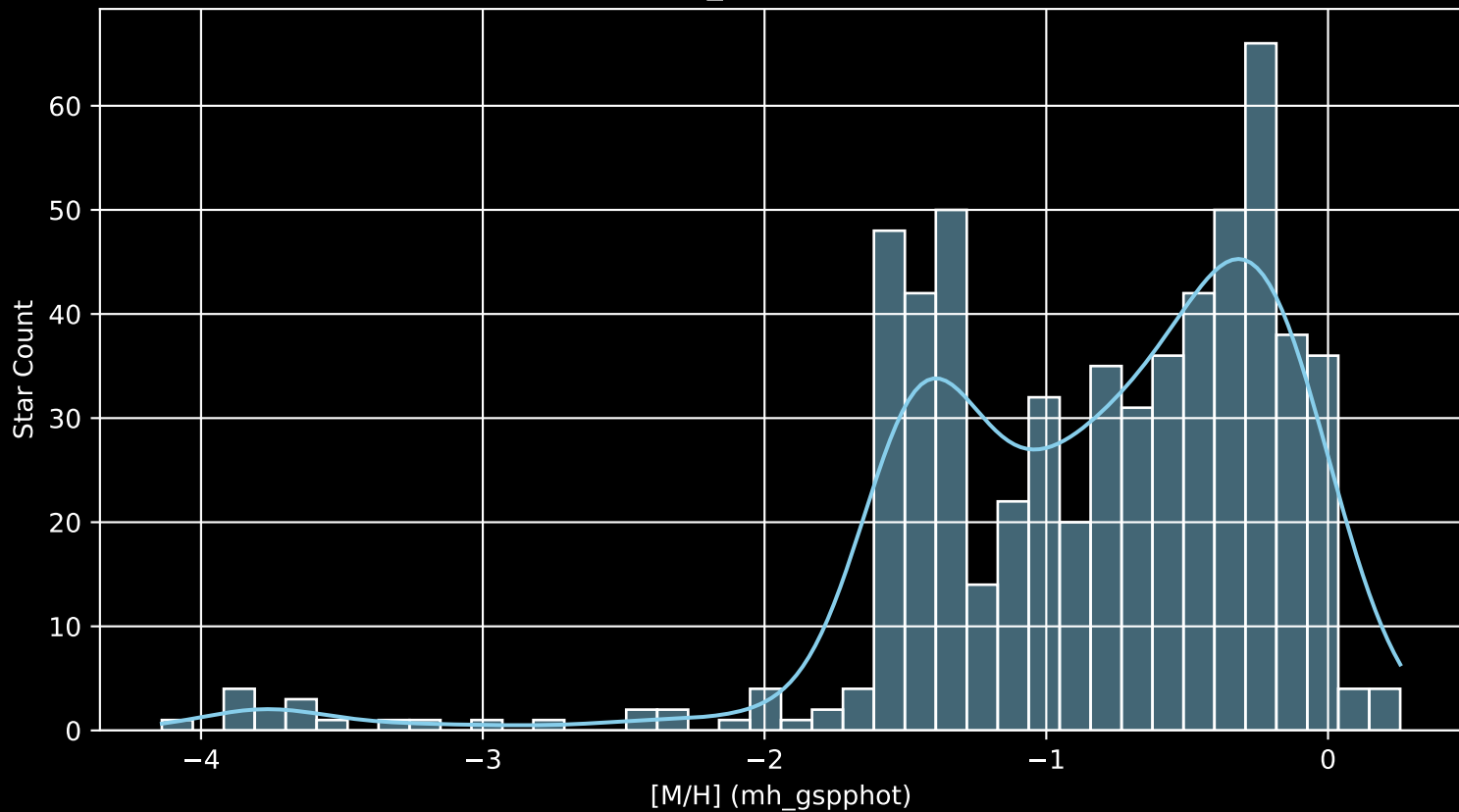
Gaia Cluster: [NGC_7086 [M/H] (mh_gspphot) (n= 601)
