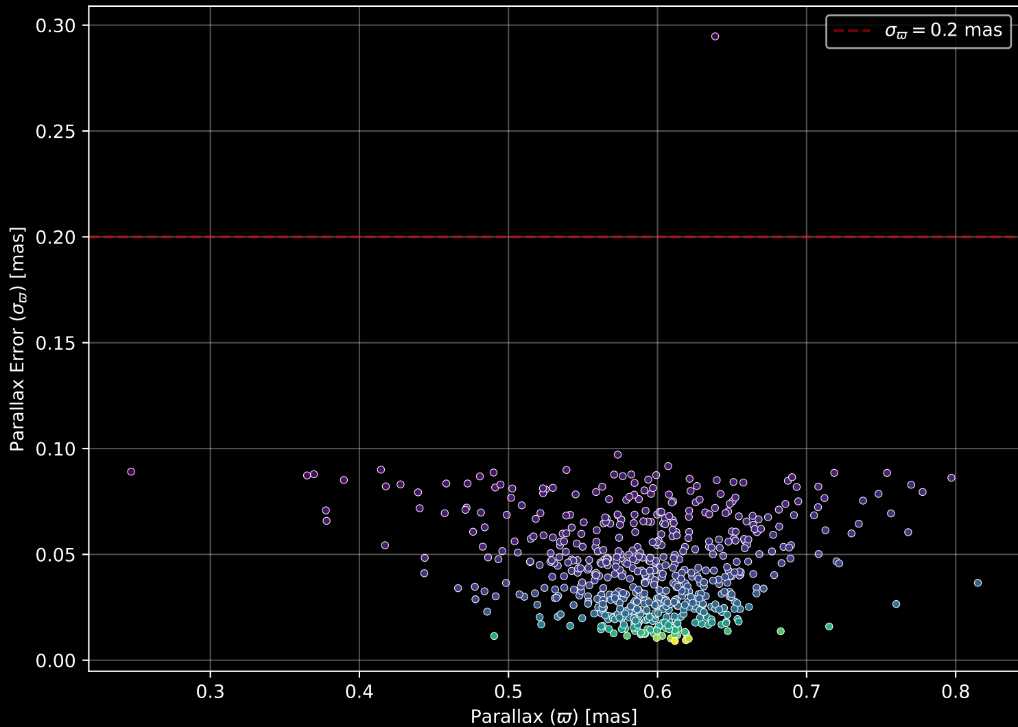
Gaia Cluster: [NGC_7086] Parallax Quality (n= 602)
