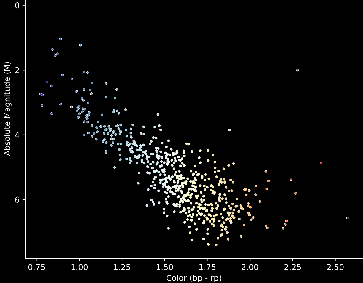
Gaia Cluster: [NGC_7086] Stars (n= 602) Hertzsprung-Russel Diagram
