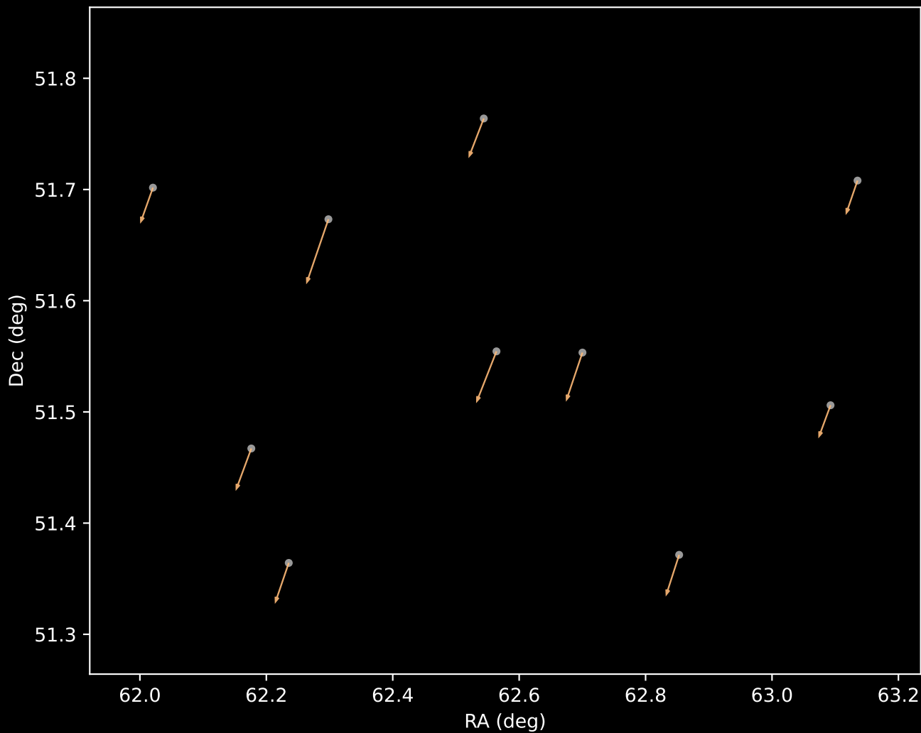
Gaia DR3 Cluster 3 Proper Motion Vectors (n=10)
