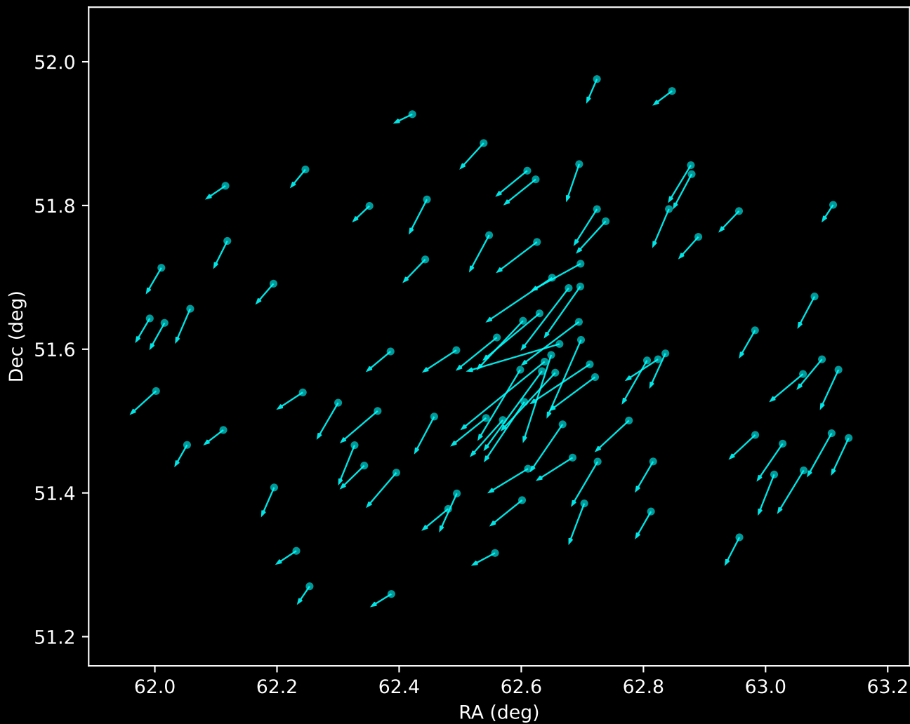
Gaia DR3 Noise Stream Proper Motion Vectors (n=91)
