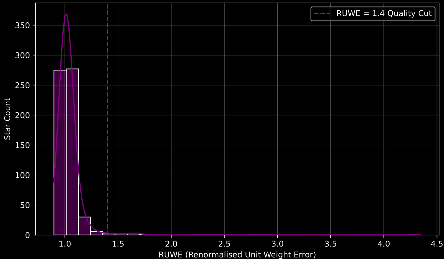
Gaia Cluster: [NGC_7086] RUWE Distribution (n= 601)
