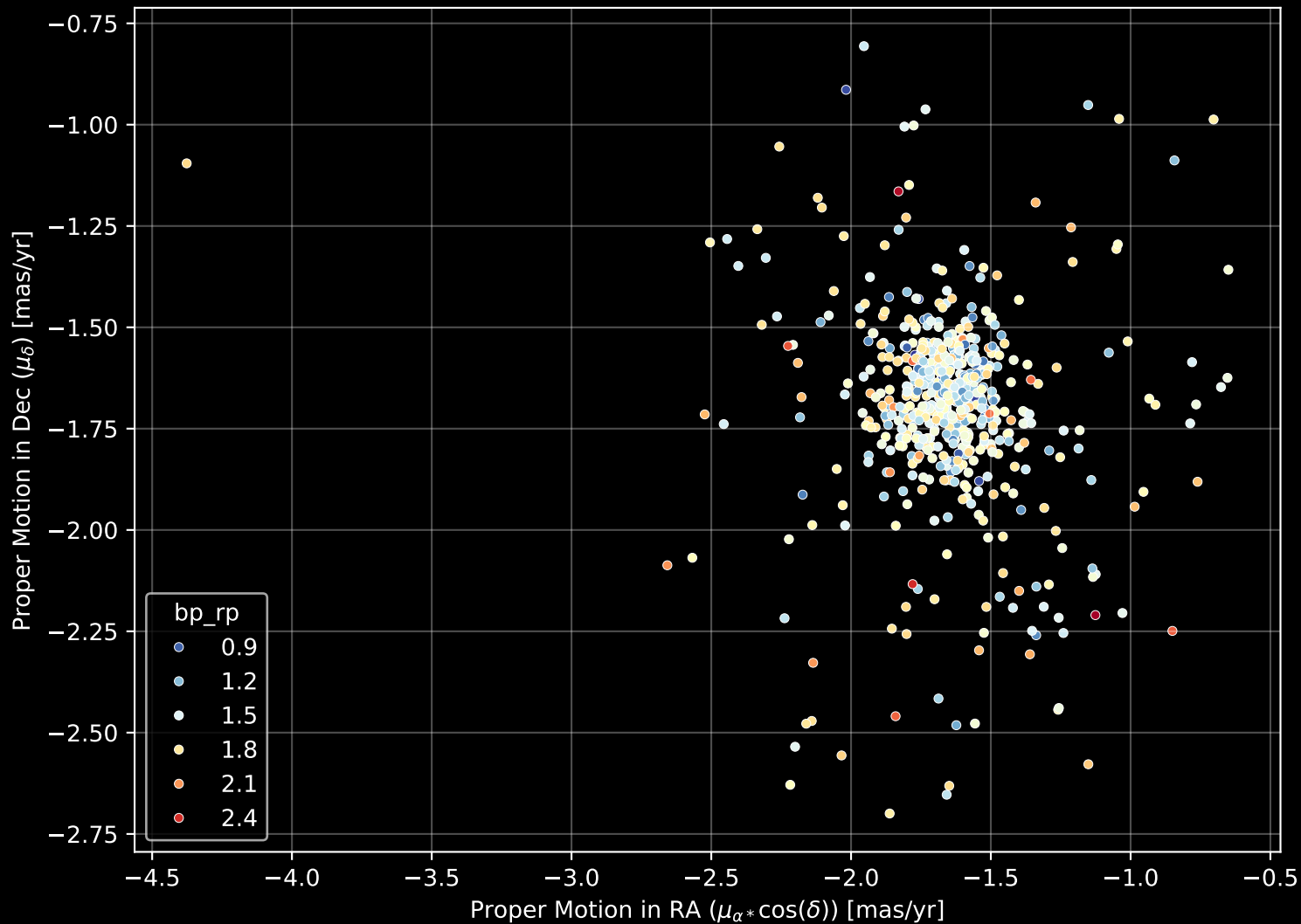
Gaia Cluster: [NGC_7086] Proper Motion Diagram (n= 602)
