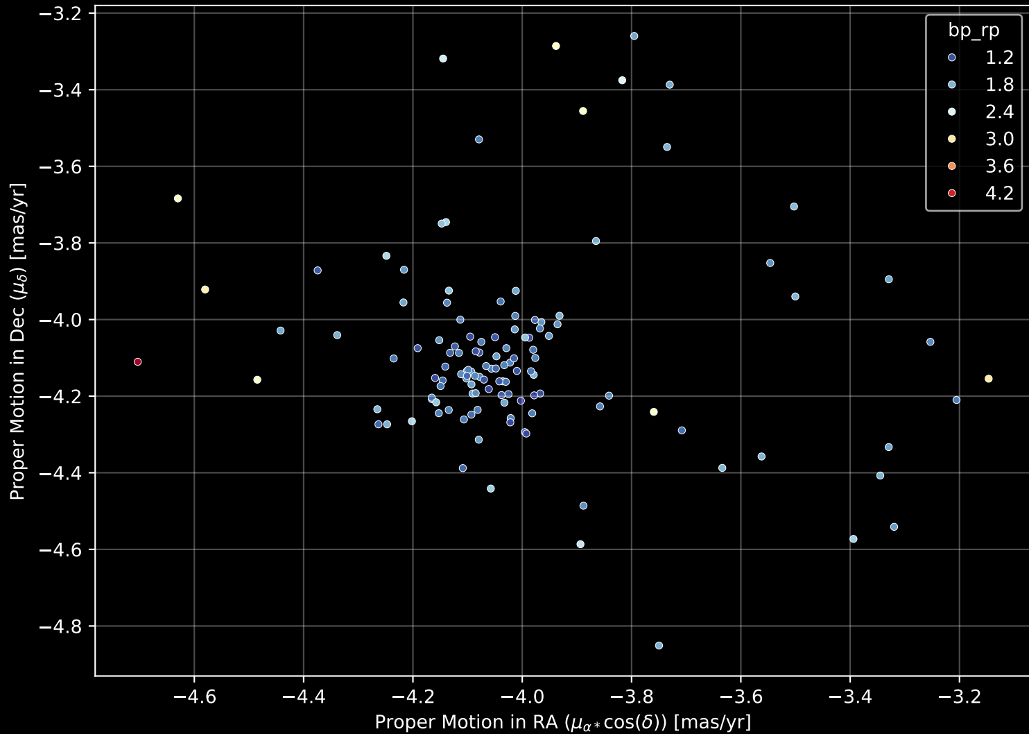
Gaia Cluster: [NGC_7128] Proper Motion Diagram (n= 126)
