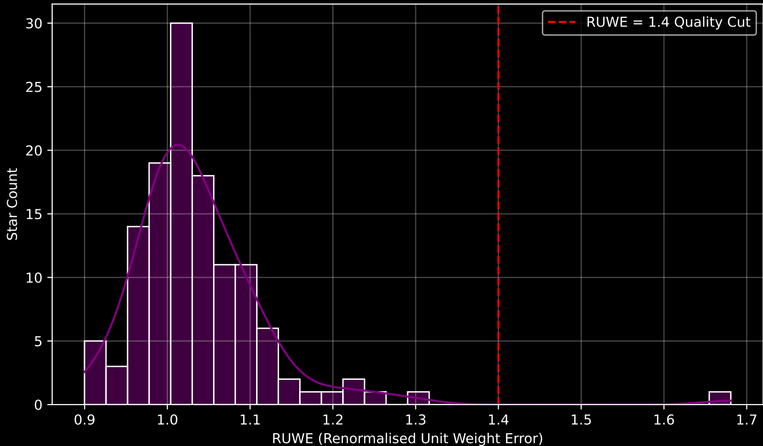
Gaia Cluster: [NGC_7128] RUWE Distribution (n= 126)
