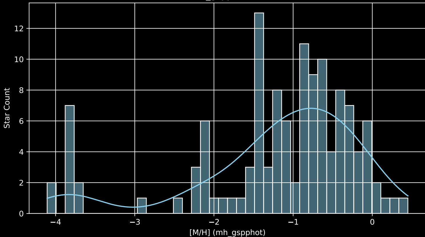
Gaia Cluster: [NGC_7128 [M/H] (mh_gspphot) (n= 125)
