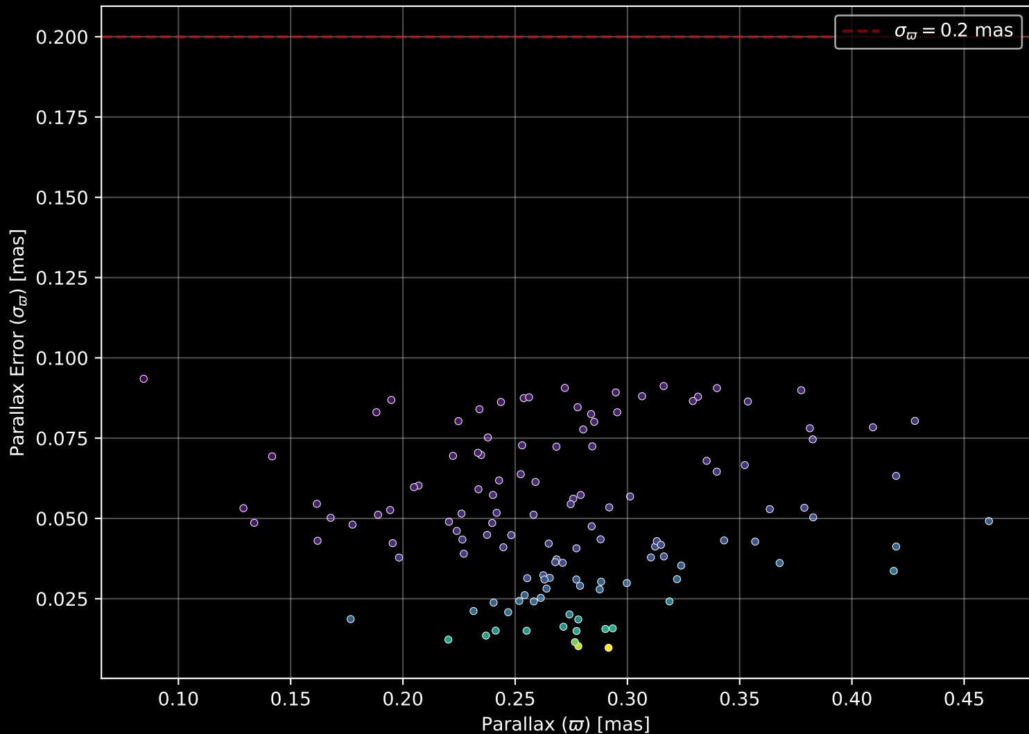
Gaia Cluster: [NGC_7128] Parallax Quality (n= 126)
