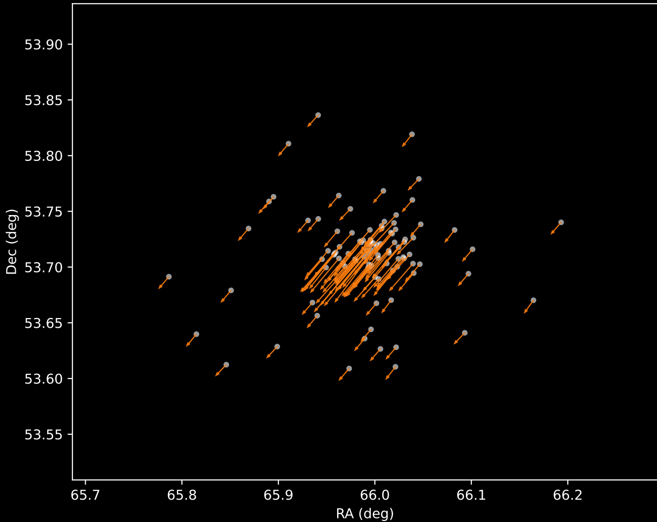
Gaia DR3 Cluster 2 Proper Motion Vectors (n=99)
