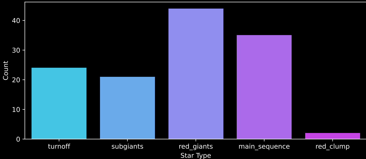
Gaia Cluster: [NGC_7128] Count plot of Star Type
