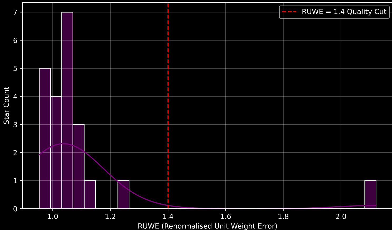
Gaia Cluster: [NGC_7129] RUWE Distribution (n= 22)
