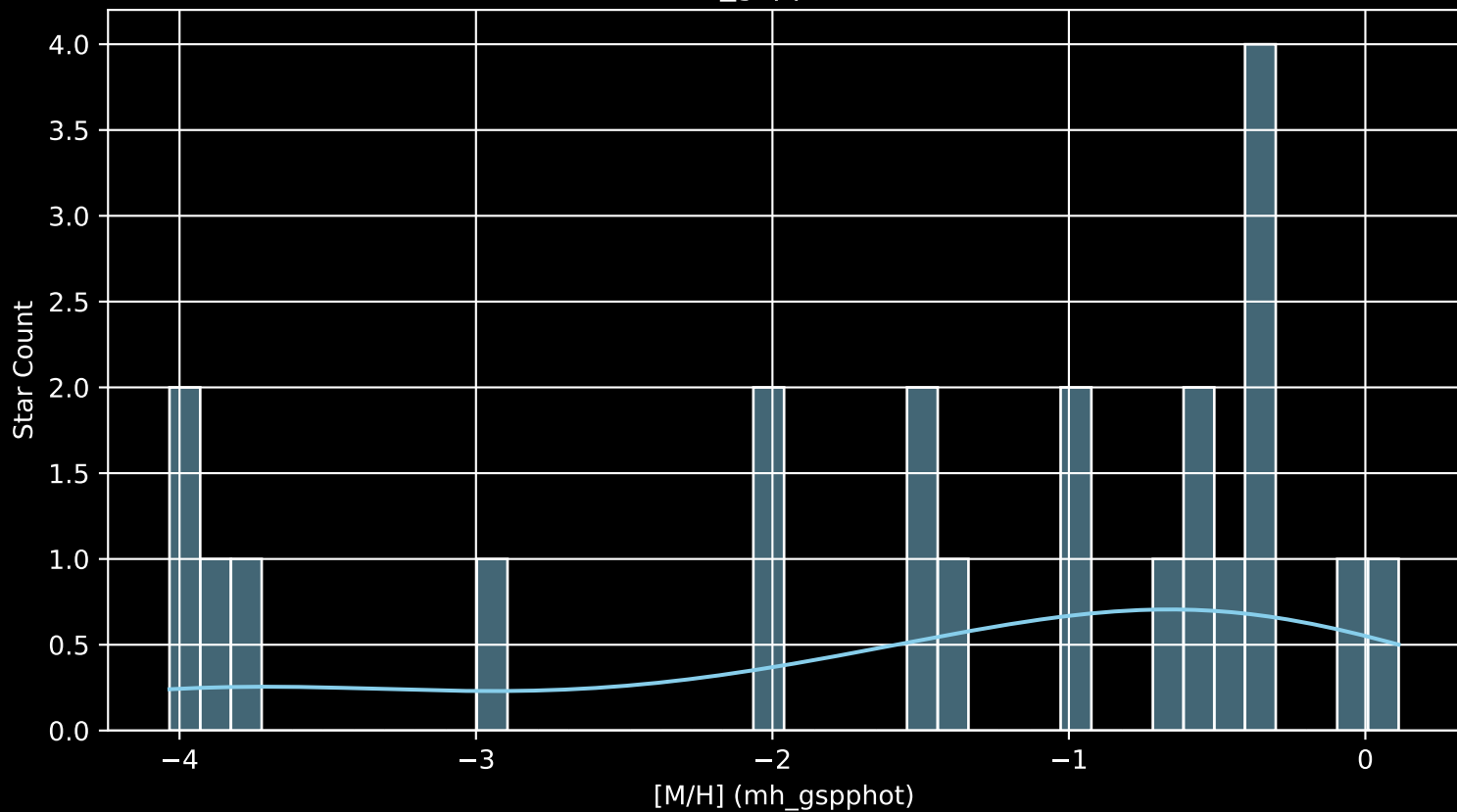
Gaia Cluster: [NGC_7129 [M/H] (mh_gspphot) (n= 22)
