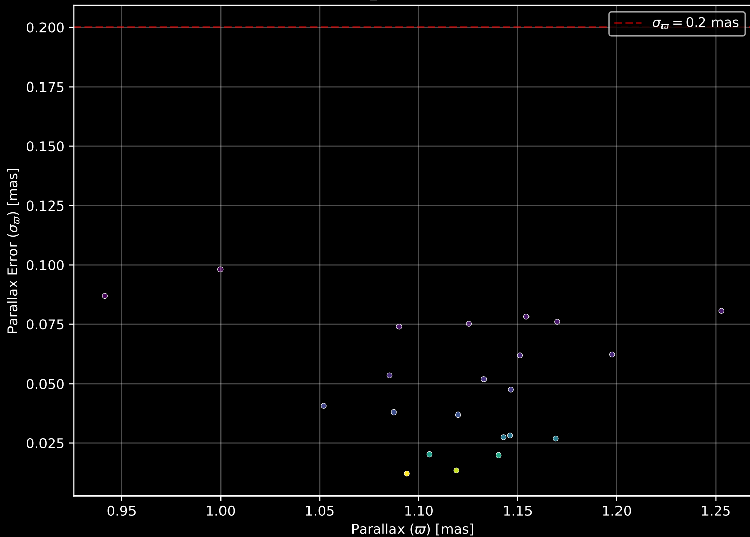
Gaia Cluster: [NGC_7129] Parallax Quality (n= 22)
