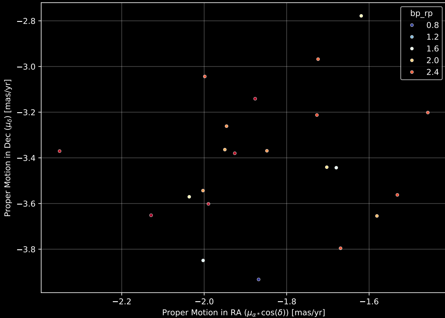
Gaia Cluster: [NGC_7129] Proper Motion Diagram (n= 22)
