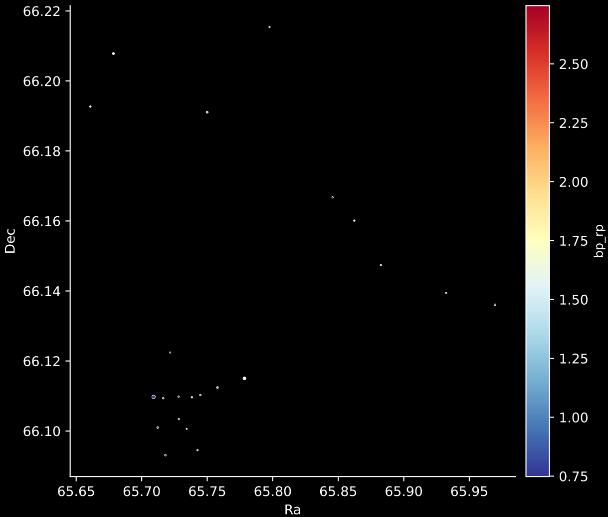
Gaia Cluster: [NGC_7129] Stars: 22
