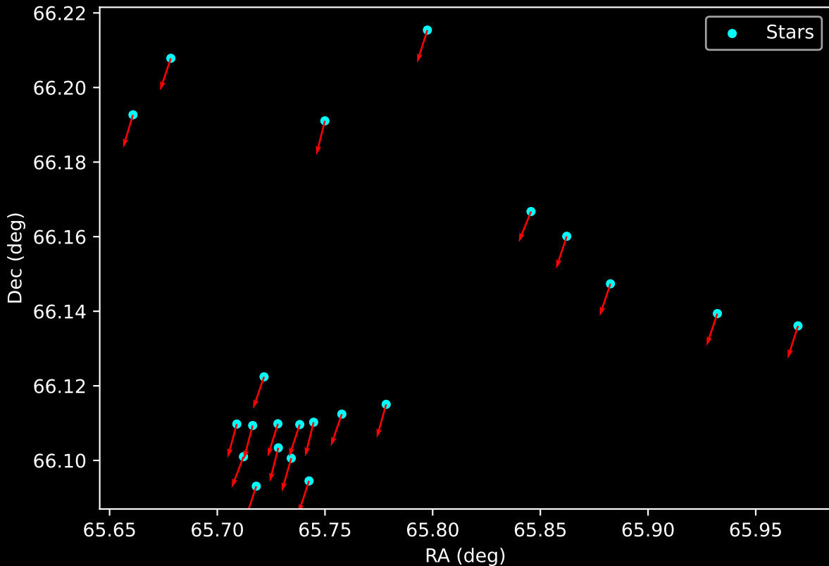
Gaia Cluster: [NGC_7129] Proper Motion Vectors for Gaia Star Field (n= 22)
