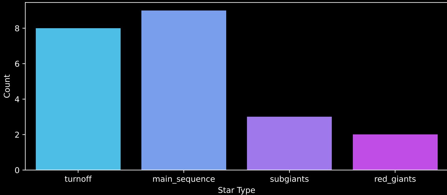
Gaia Cluster: [NGC_7129] Count plot of Star Type
