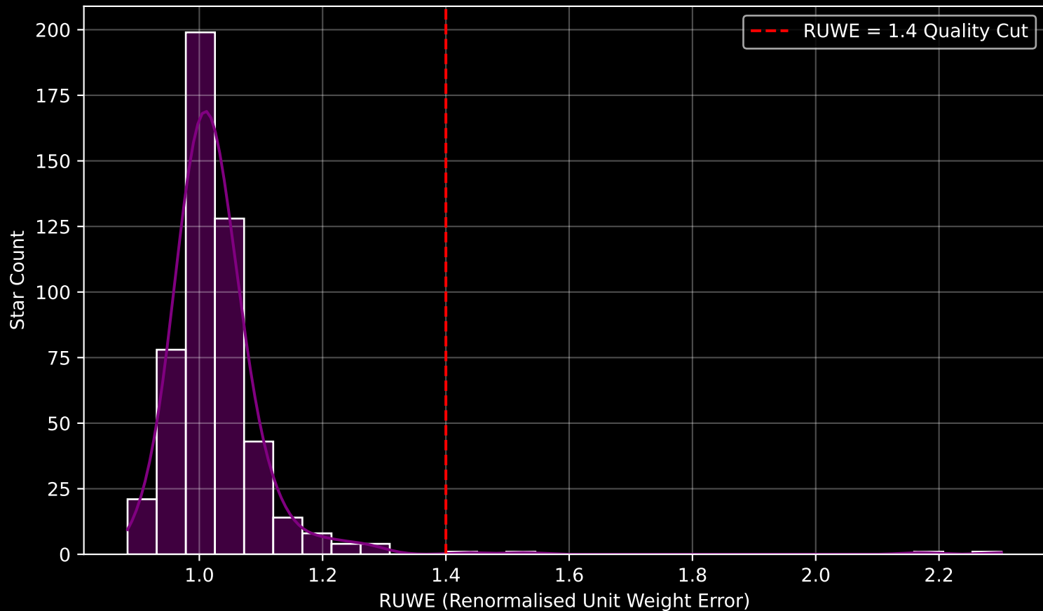
Gaia Cluster: [NGC_7142] RUWE Distribution (n= 503)
