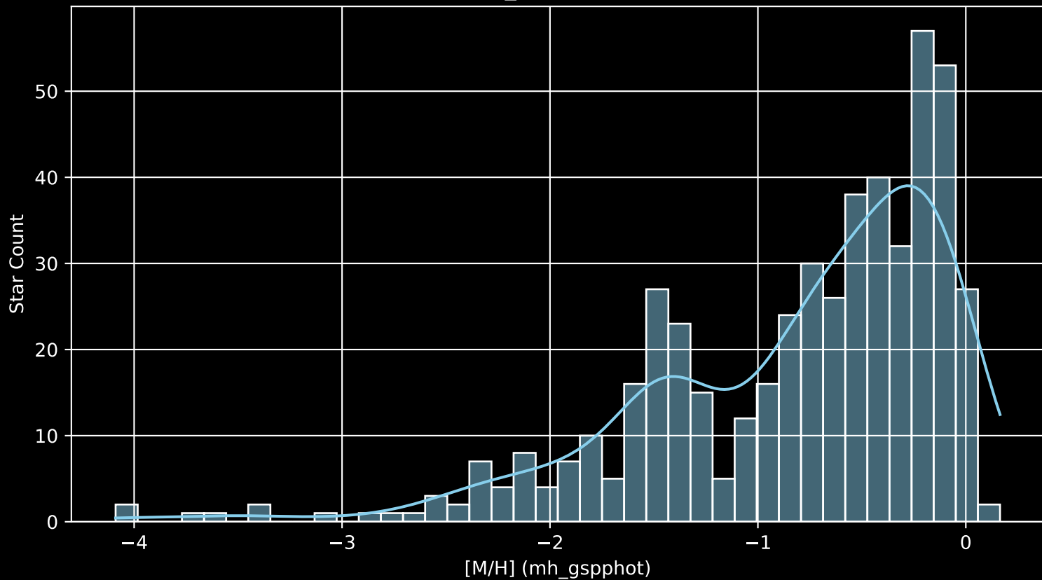
Gaia Cluster: [NGC_7142 [M/H] (mh_gspphot) (n= 503)
