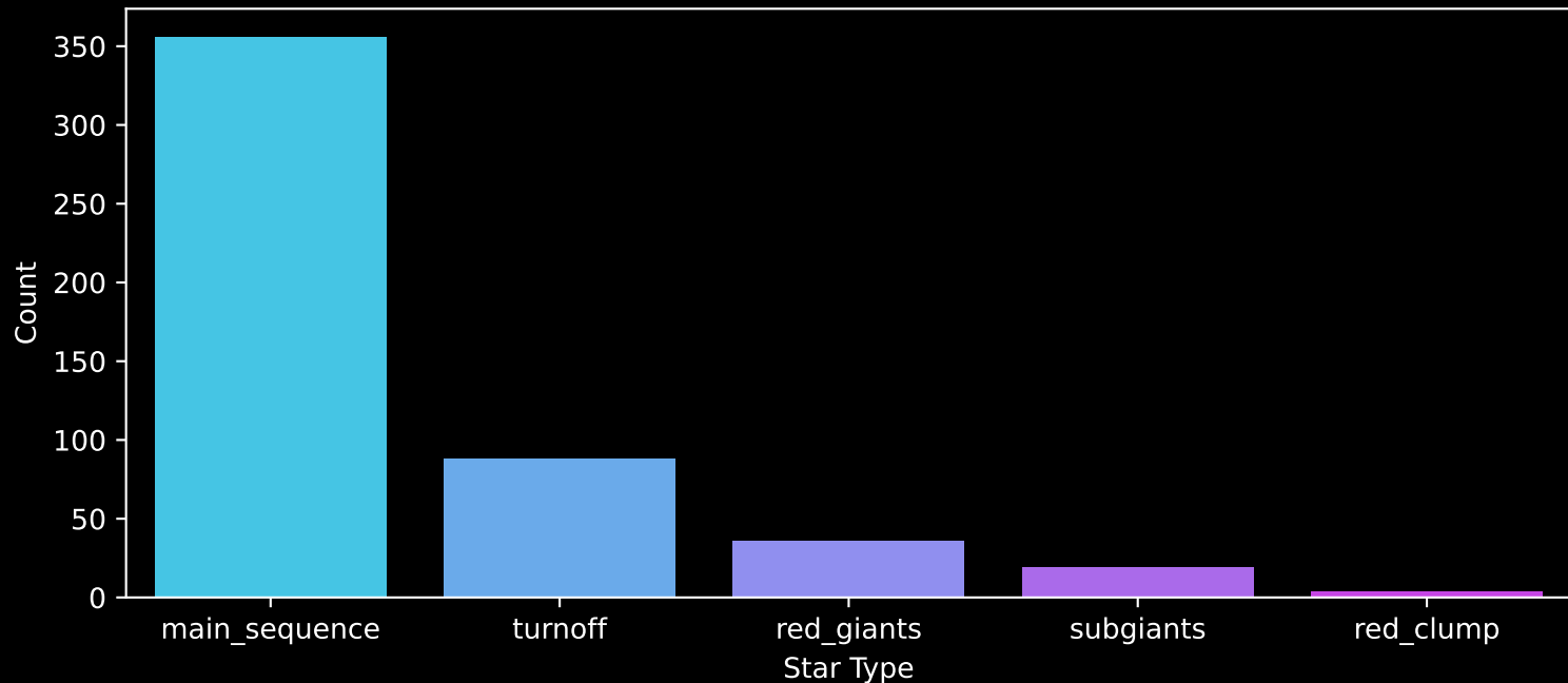
Gaia Cluster: [NGC_7142] Count plot of Star Type
