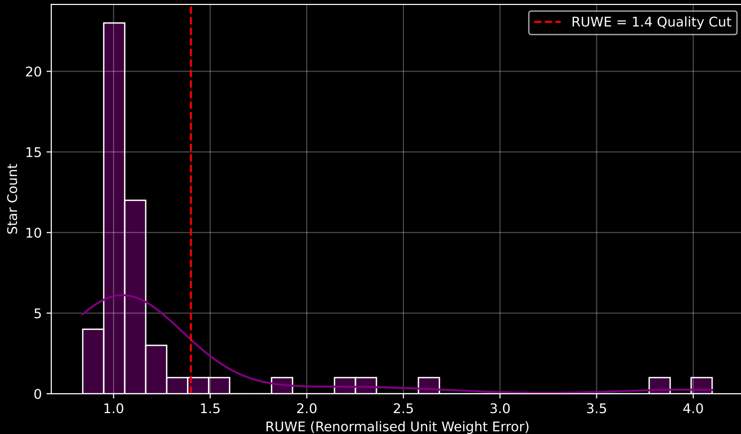
Gaia Cluster: [NGC_7160] RUWE Distribution (n= 51)
