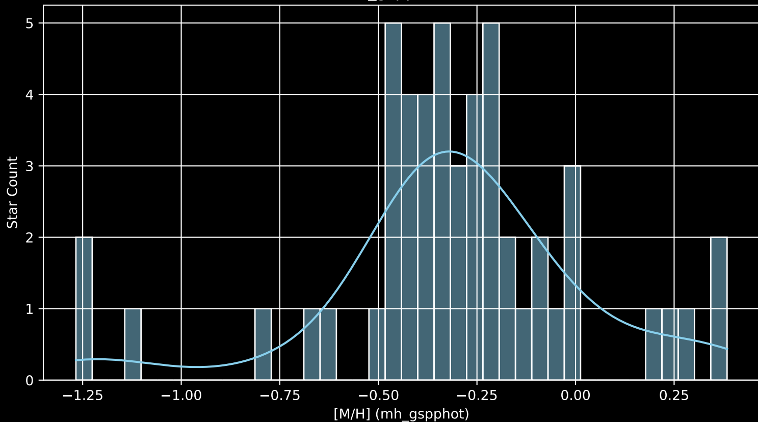
Gaia Cluster: [NGC_7160 [M/H] (mh_gspphot) (n= 51)
