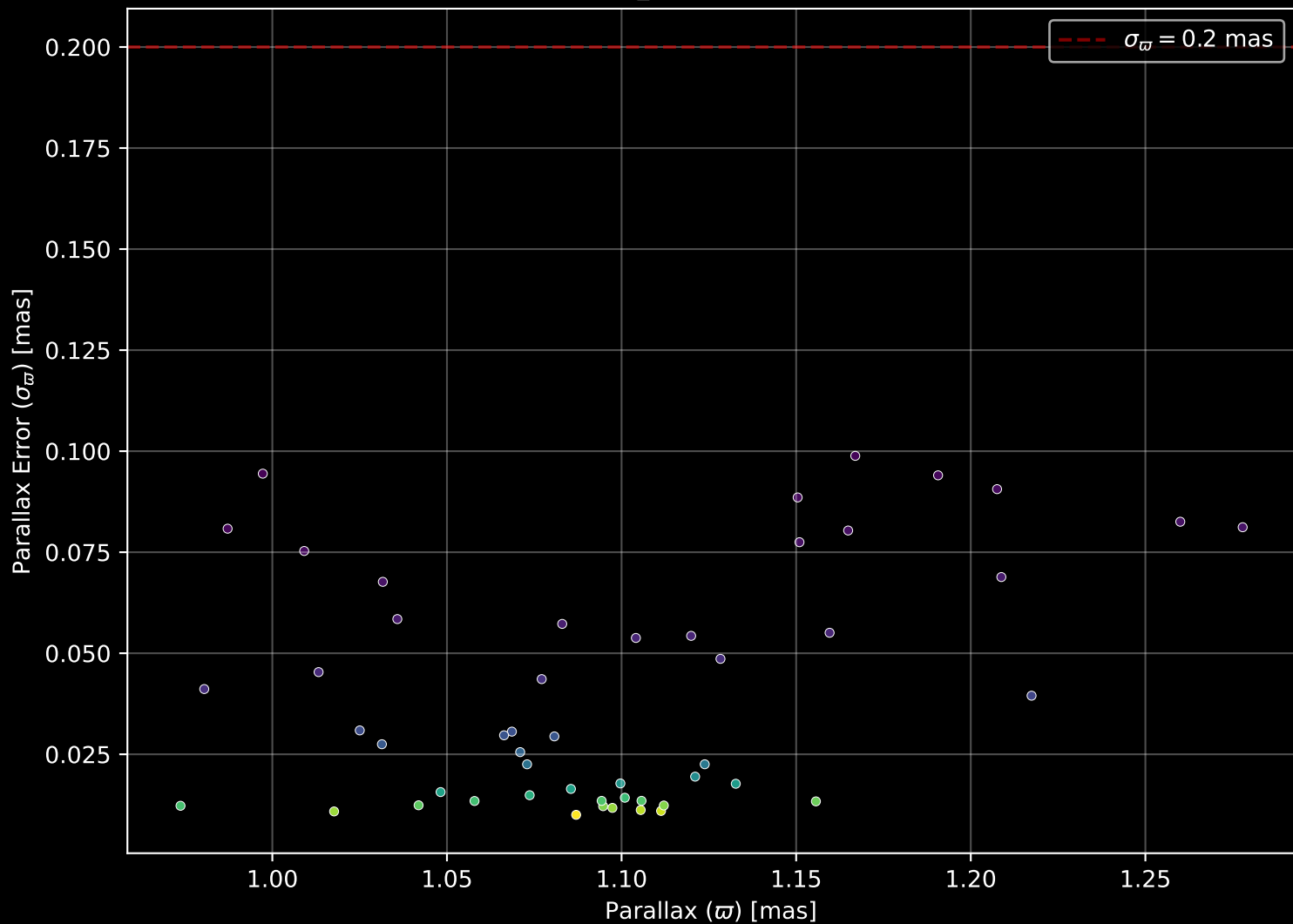
Gaia Cluster: [NGC_7160] Parallax Quality (n= 51)
