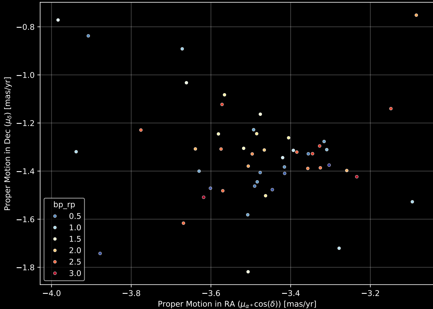
Gaia Cluster: [NGC_7160] Proper Motion Diagram (n= 51)
