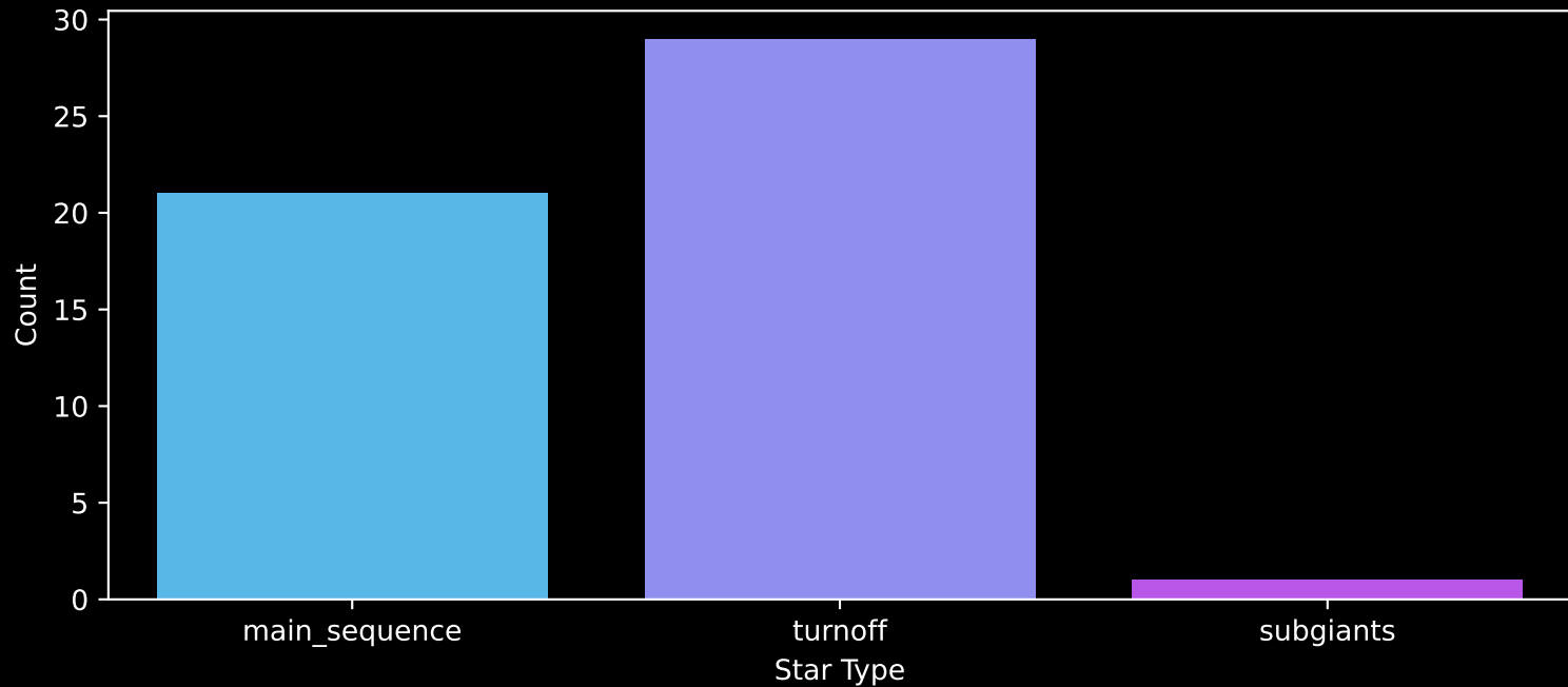
Gaia Cluster: [NGC_7160] Count plot of Star Type
