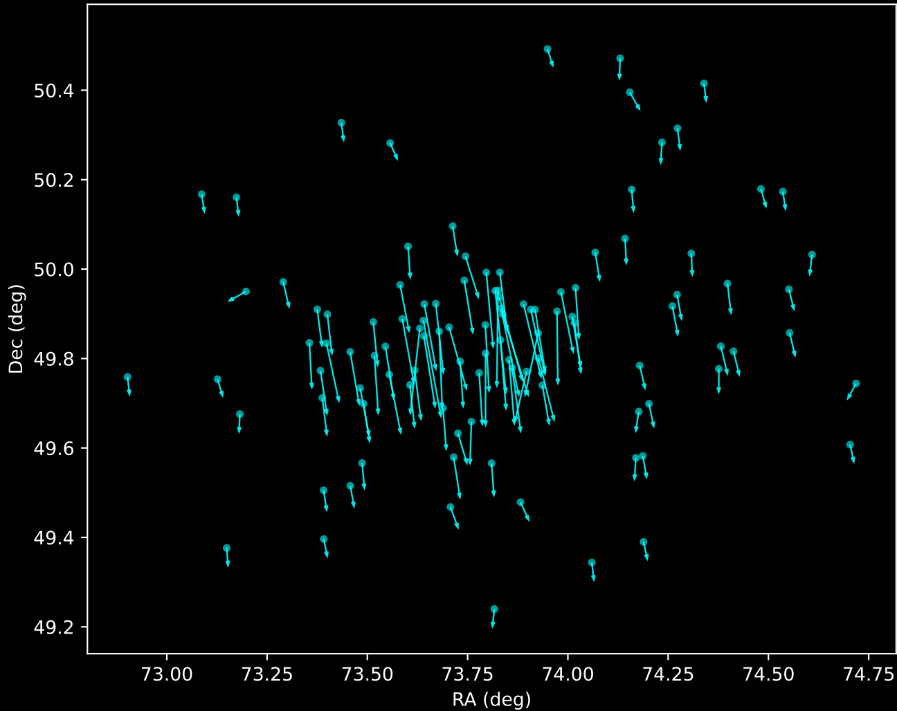
Gaia DR3 Noise Stream Proper Motion Vectors (n=106)
