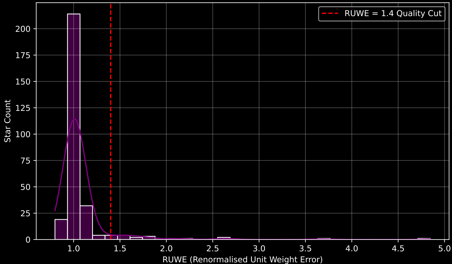
Gaia Cluster: [NGC_7243] RUWE Distribution (n= 288)
