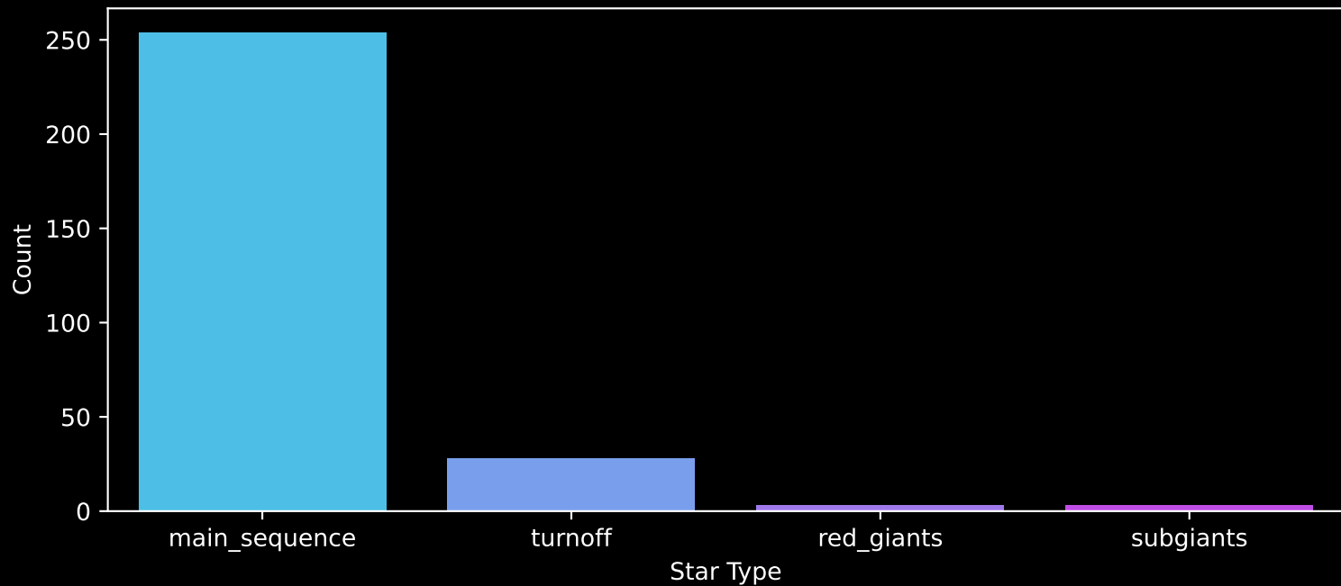
Gaia Cluster: [NGC_7243] Count plot of Star Type
