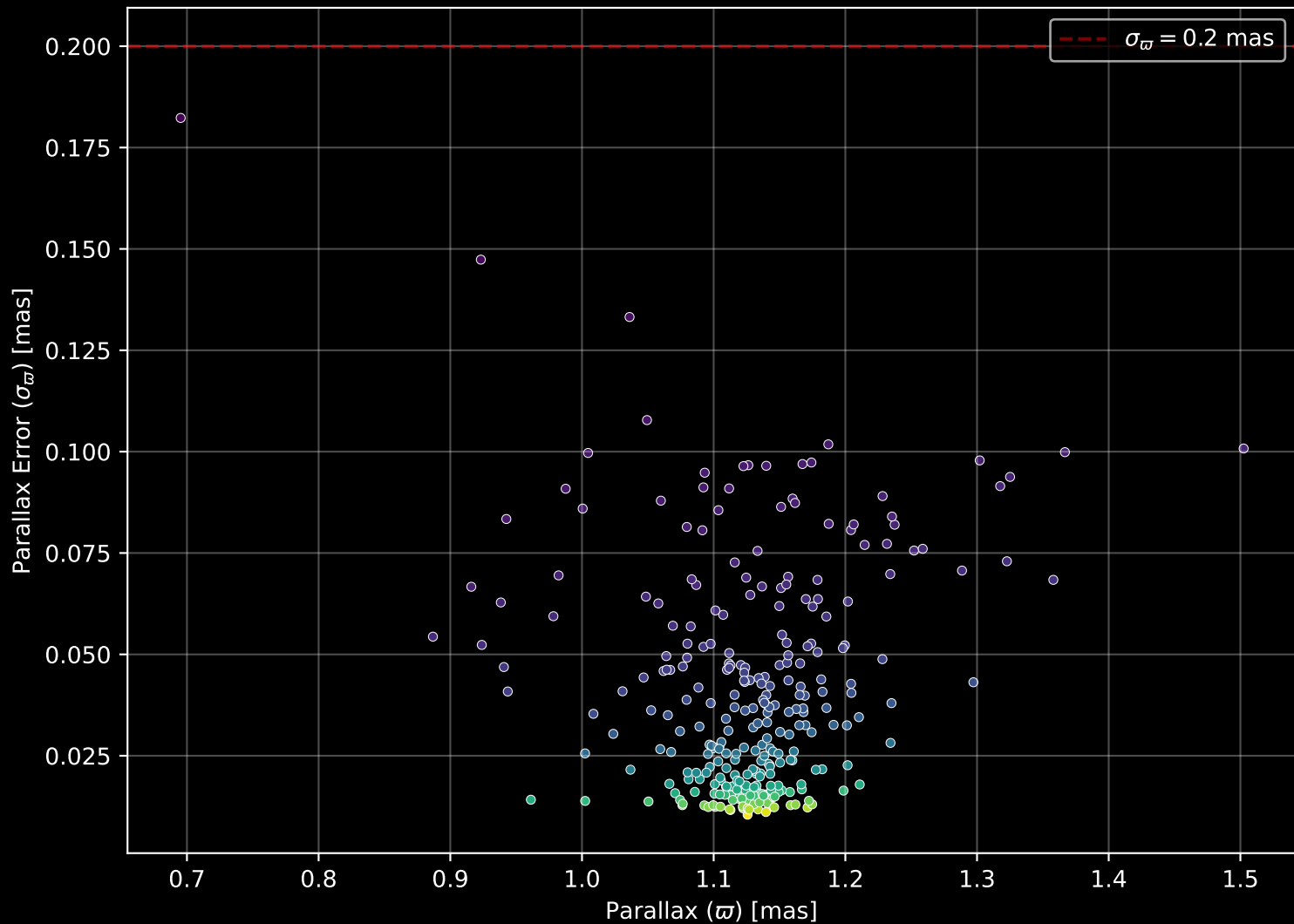
Gaia Cluster: [NGC_7243] Parallax Quality (n= 288)
