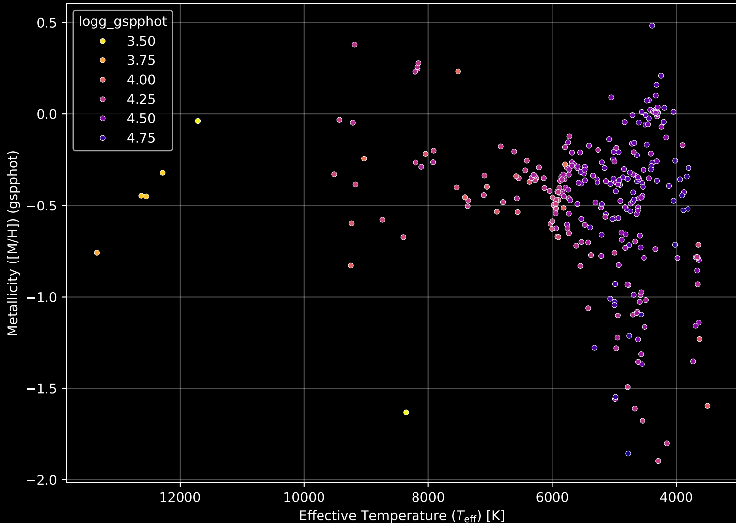
Gaia Cluster: [NGC_7243] Stellar Population Parameters (n= 288)
