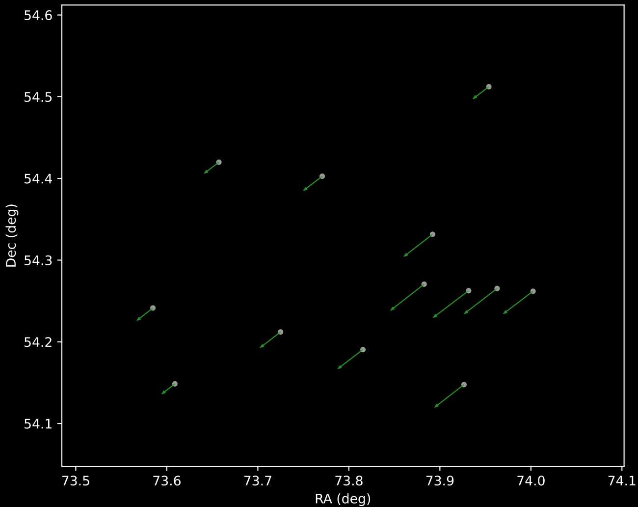
Gaia DR3 Cluster 24 Proper Motion Vectors (n=13)
