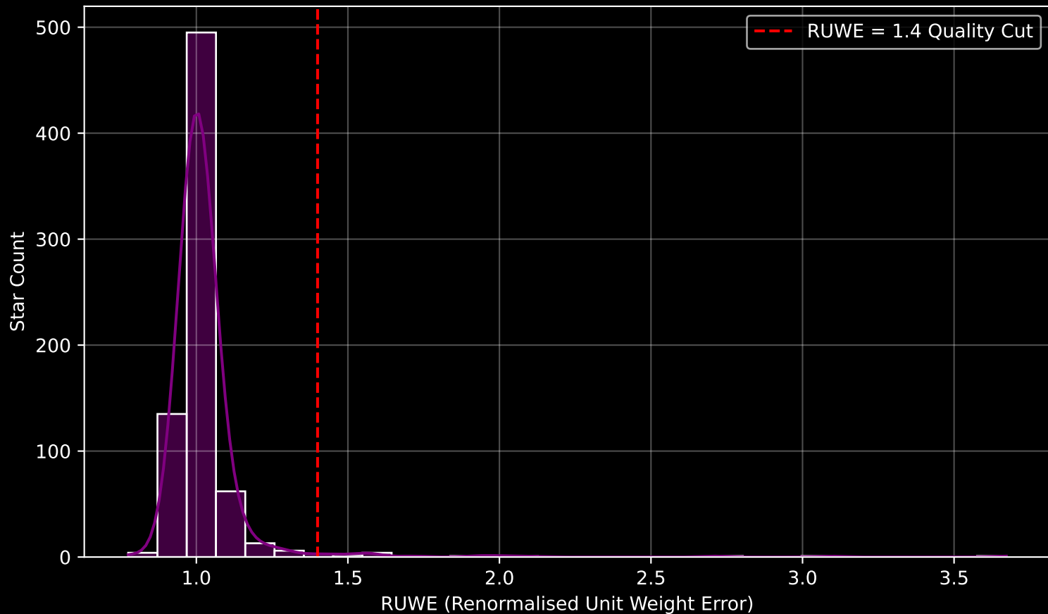
Gaia Cluster: [NGC_7245] RUWE Distribution (n= 731)
