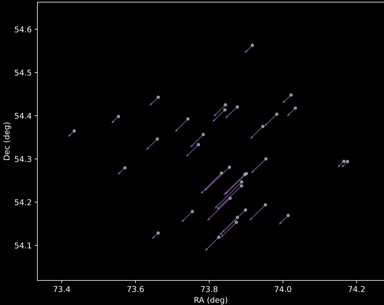
Gaia DR3 Cluster 28 Proper Motion Vectors (n=34)
