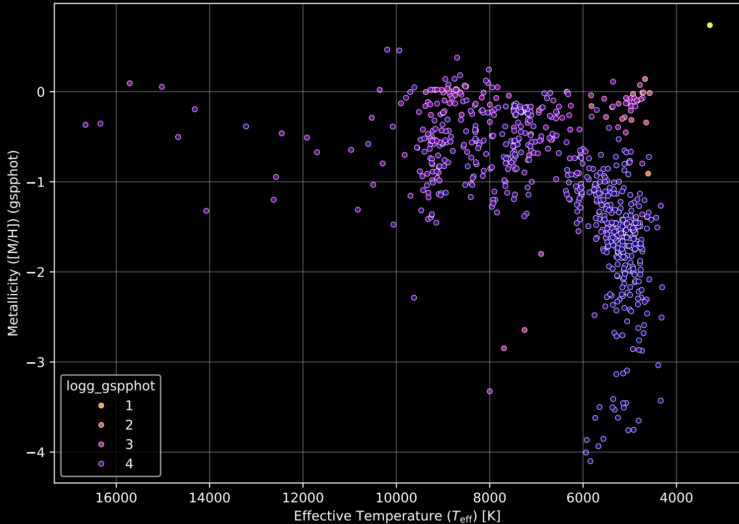
Gaia Cluster: [NGC_7245] Stellar Population Parameters (n= 732)
