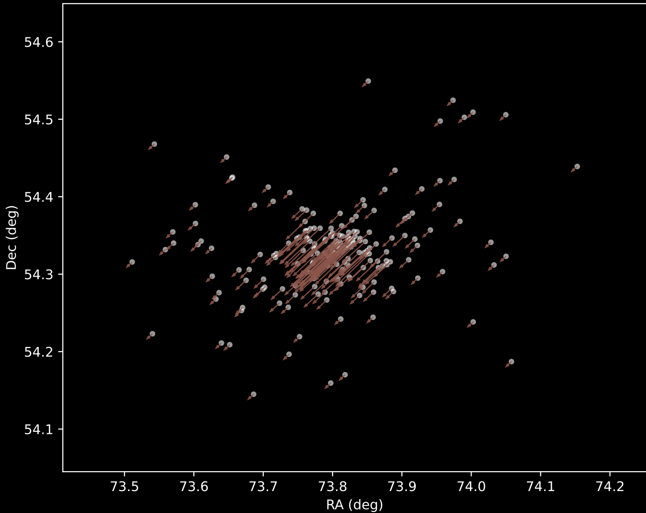
Gaia DR3 Cluster 30 Proper Motion Vectors (n=186)
