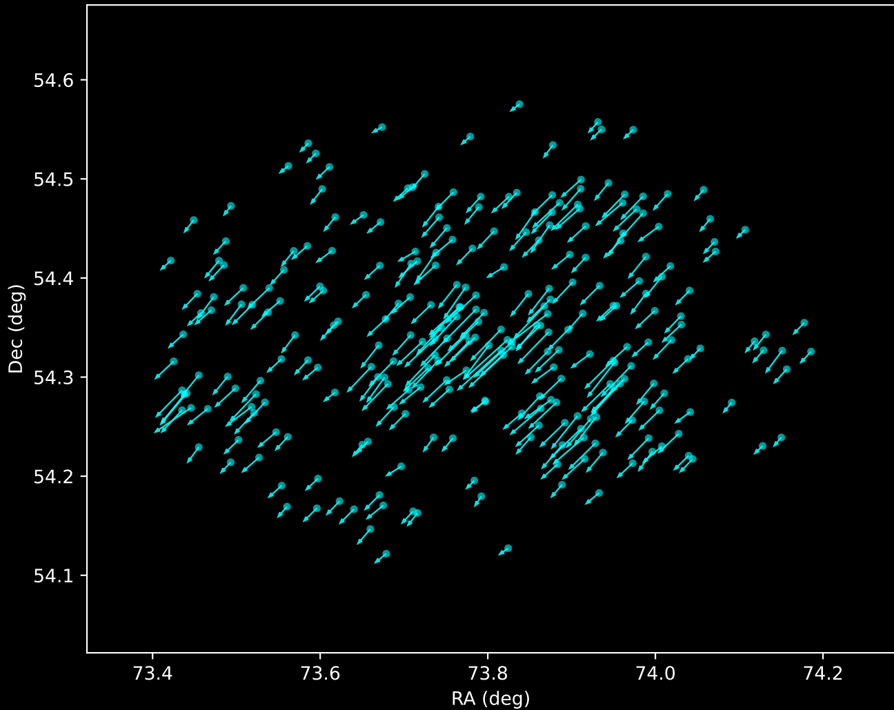
Gaia DR3 Noise Stream Proper Motion Vectors (n=266)
