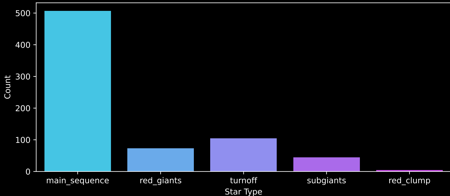
Gaia Cluster: [NGC_7245] Count plot of Star Type
