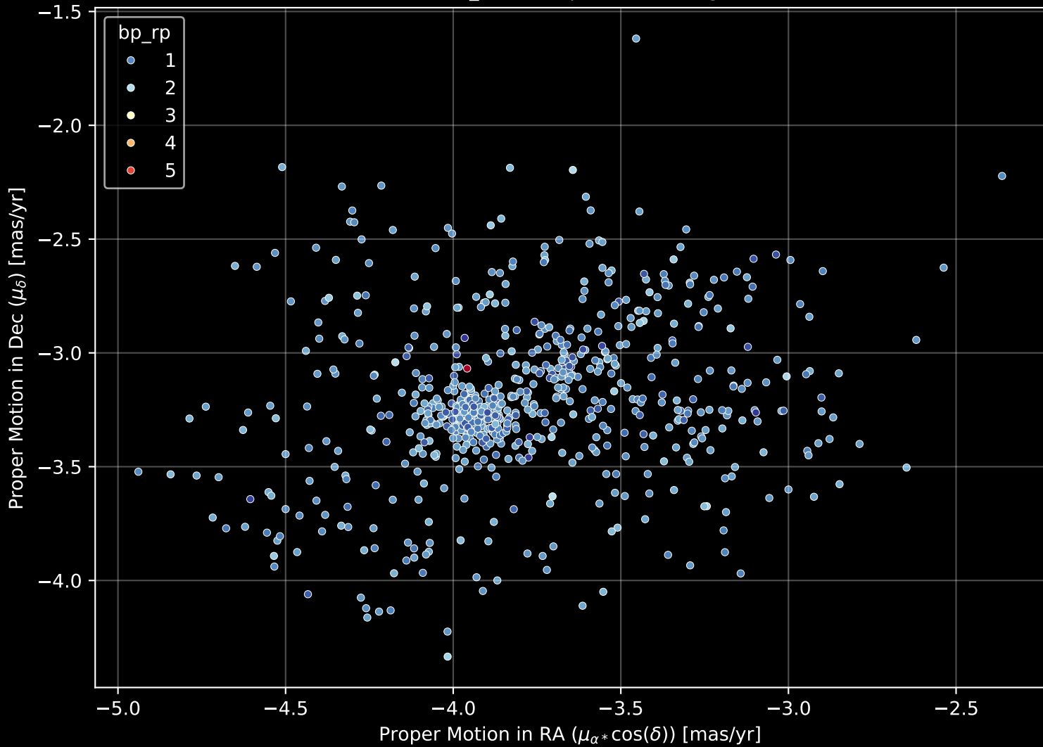
Gaia Cluster: [NGC_7245] Proper Motion Diagram (n= 732)
