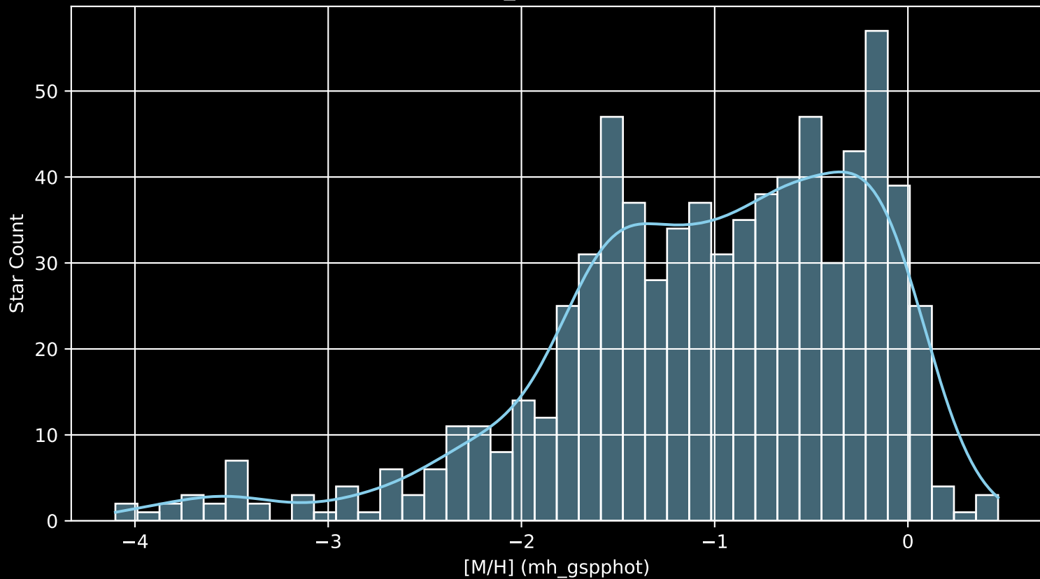
Gaia Cluster: [NGC_7245 [M/H] (mh_gspphot) (n= 731)
