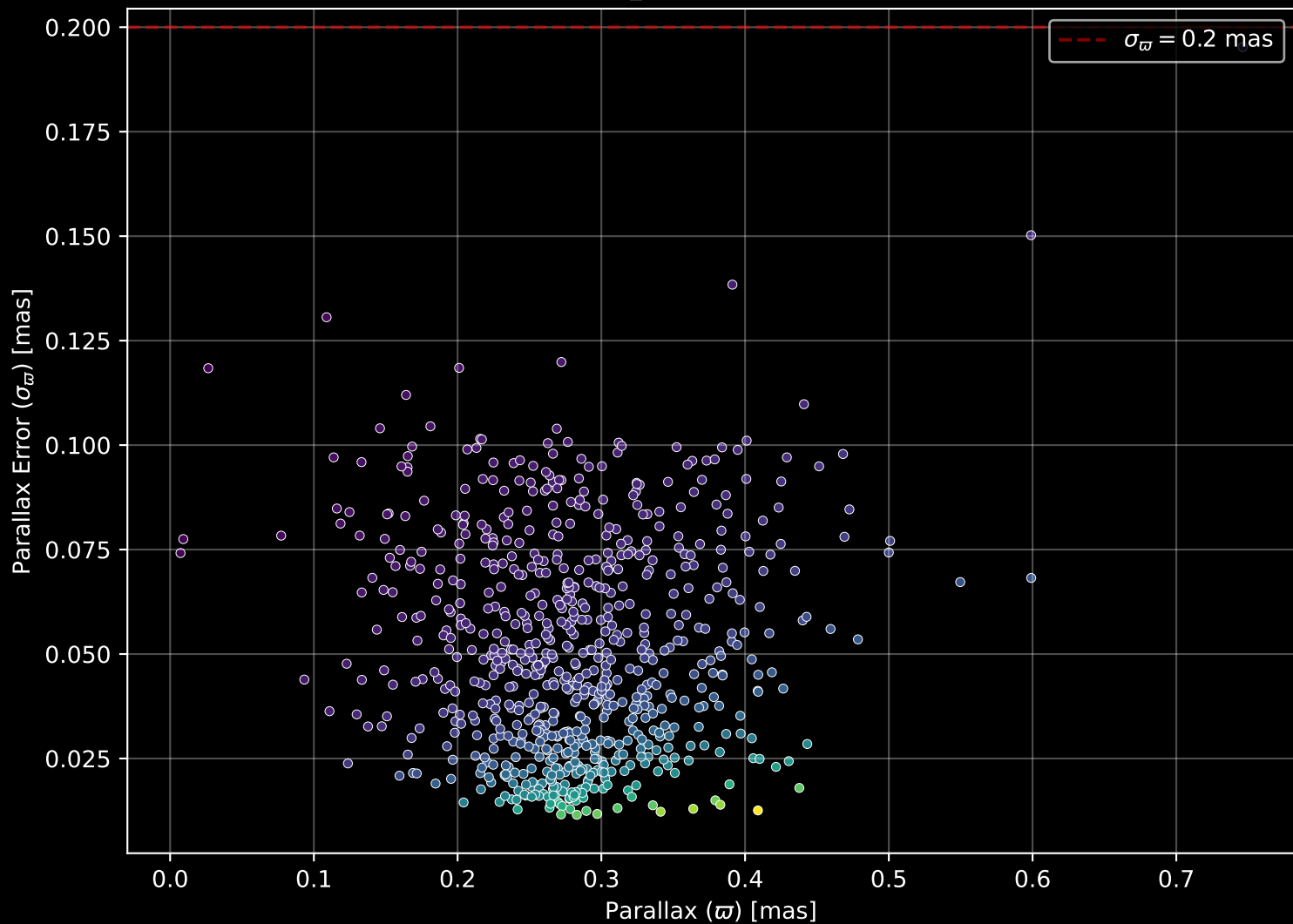
Gaia Cluster: [NGC_7245] Parallax Quality (n= 732)
