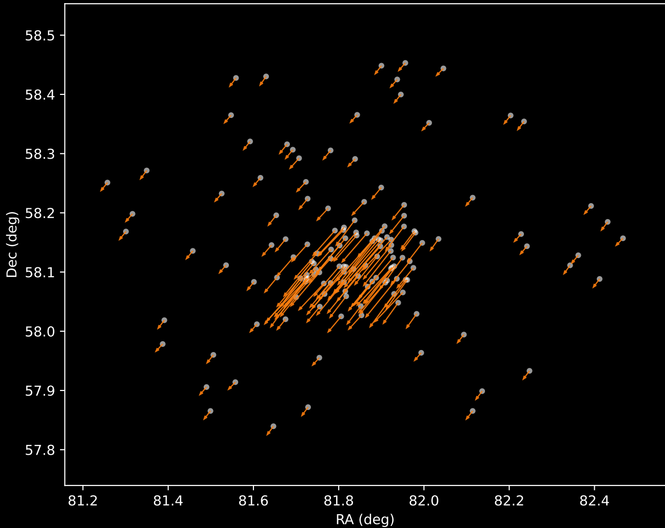
Gaia DR3 Cluster 2 Proper Motion Vectors (n=141)
