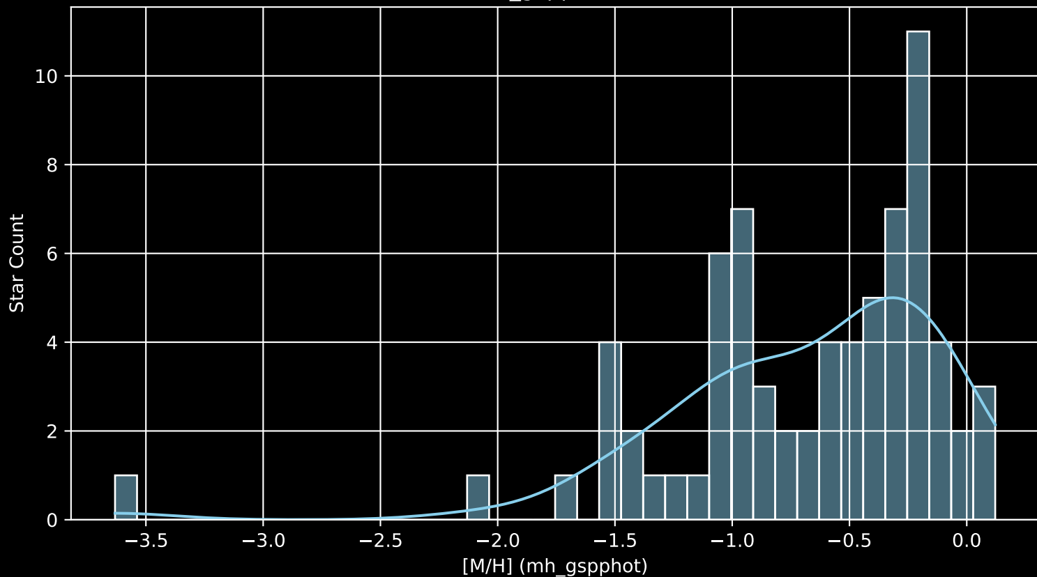
Gaia Cluster: [NGC_743 [M/H] (mh_gspphot) (n= 72)
