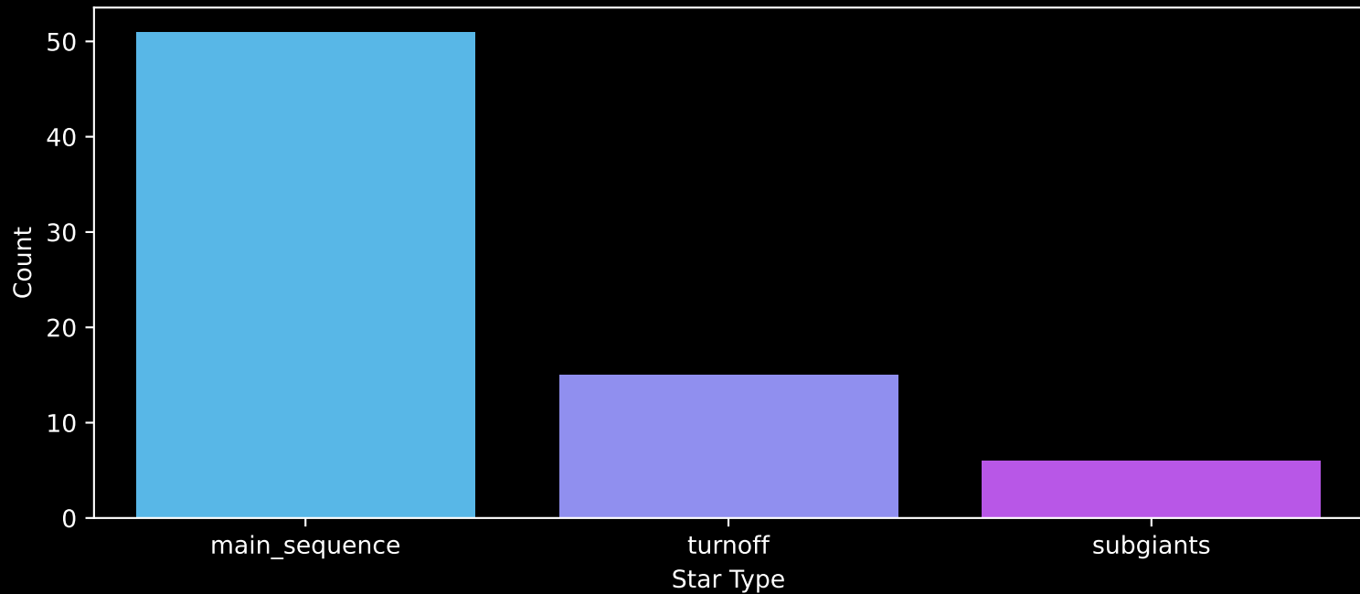
Gaia Cluster: [NGC_743] Count plot of Star Type
