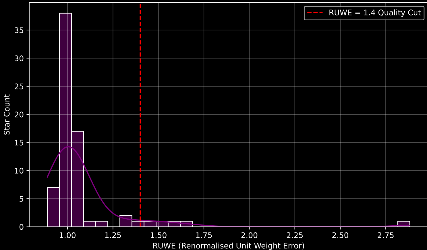
Gaia Cluster: [NGC_743] RUWE Distribution (n= 72)
