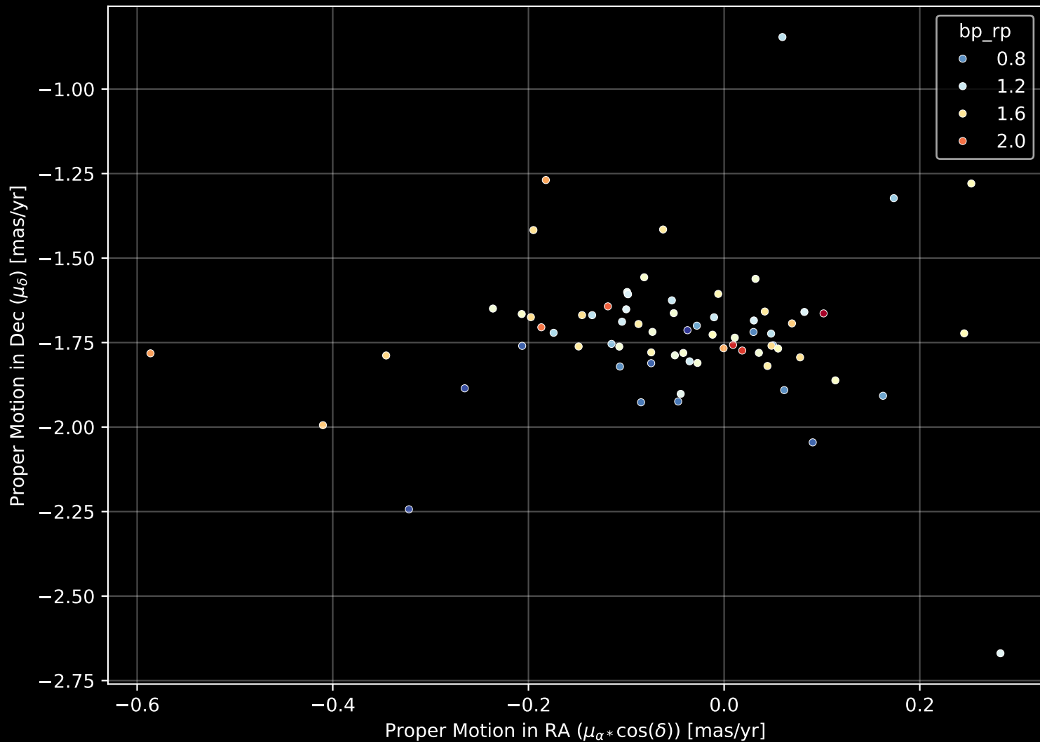
Gaia Cluster: [NGC_743] Proper Motion Diagram (n= 72)
