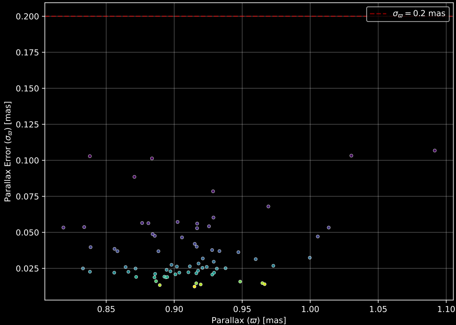
Gaia Cluster: [NGC_743] Parallax Quality (n= 72)
