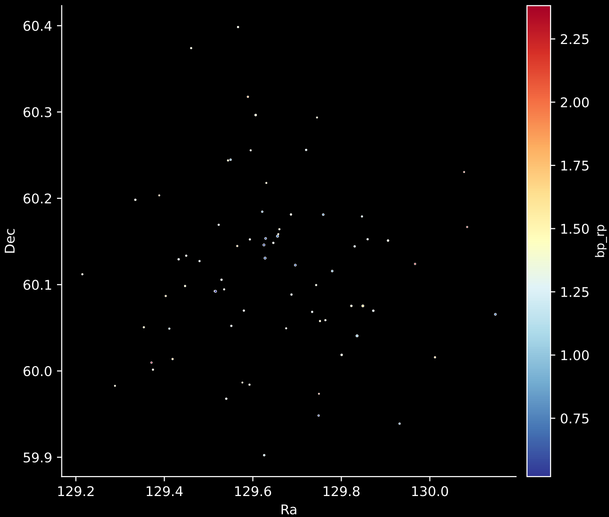
Gaia Cluster: [NGC_743] Stars: 72
