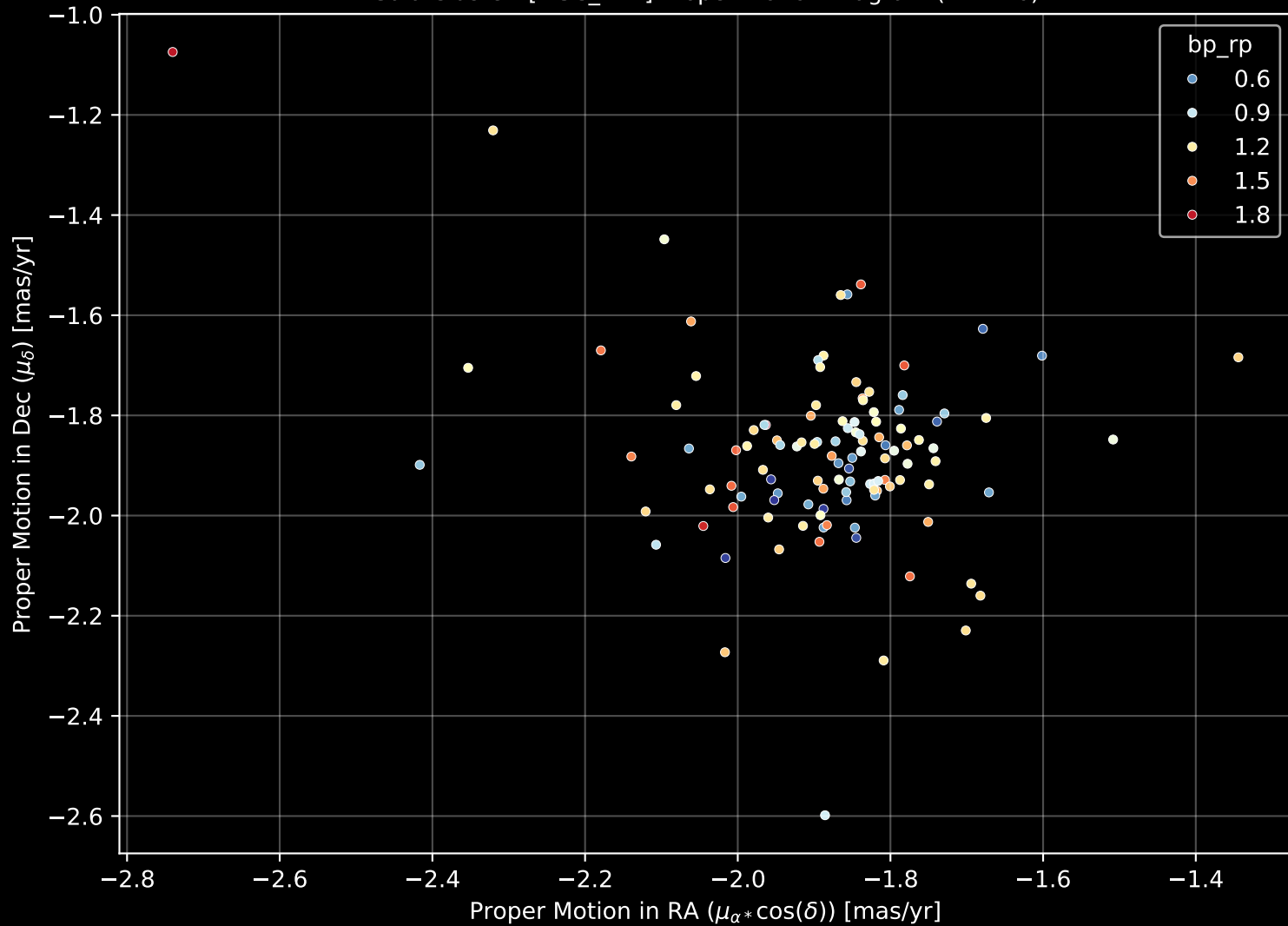
Gaia Cluster: [NGC_744] Proper Motion Diagram (n= 116)
