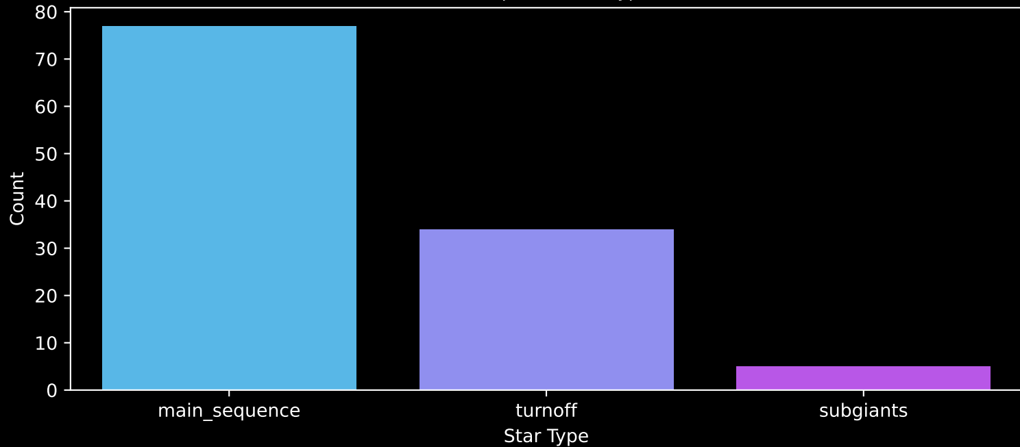
Gaia Cluster: [NGC_744] Count plot of Star Type
