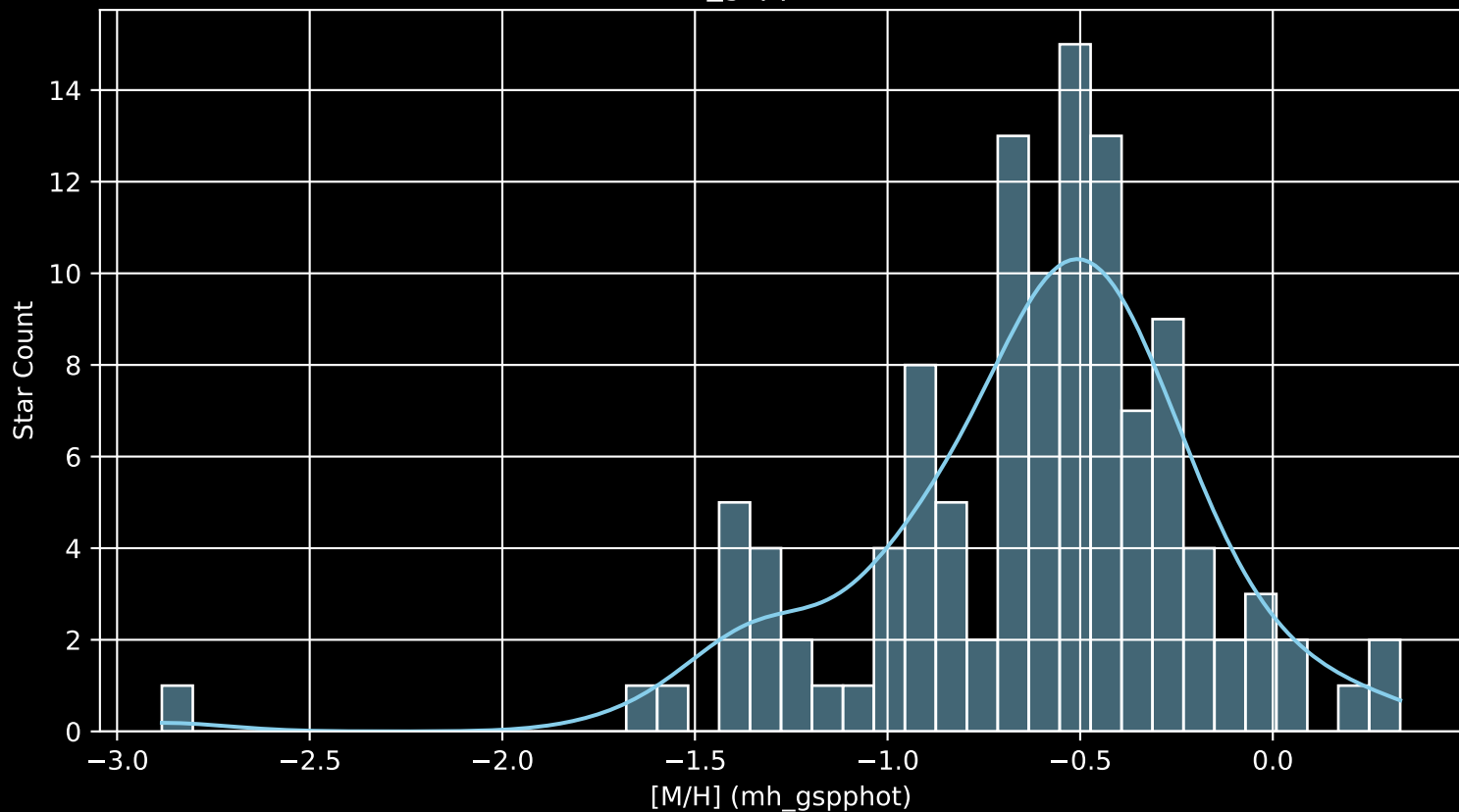
Gaia Cluster: [NGC_744 [M/H] (mh_gspphot) (n= 116)
