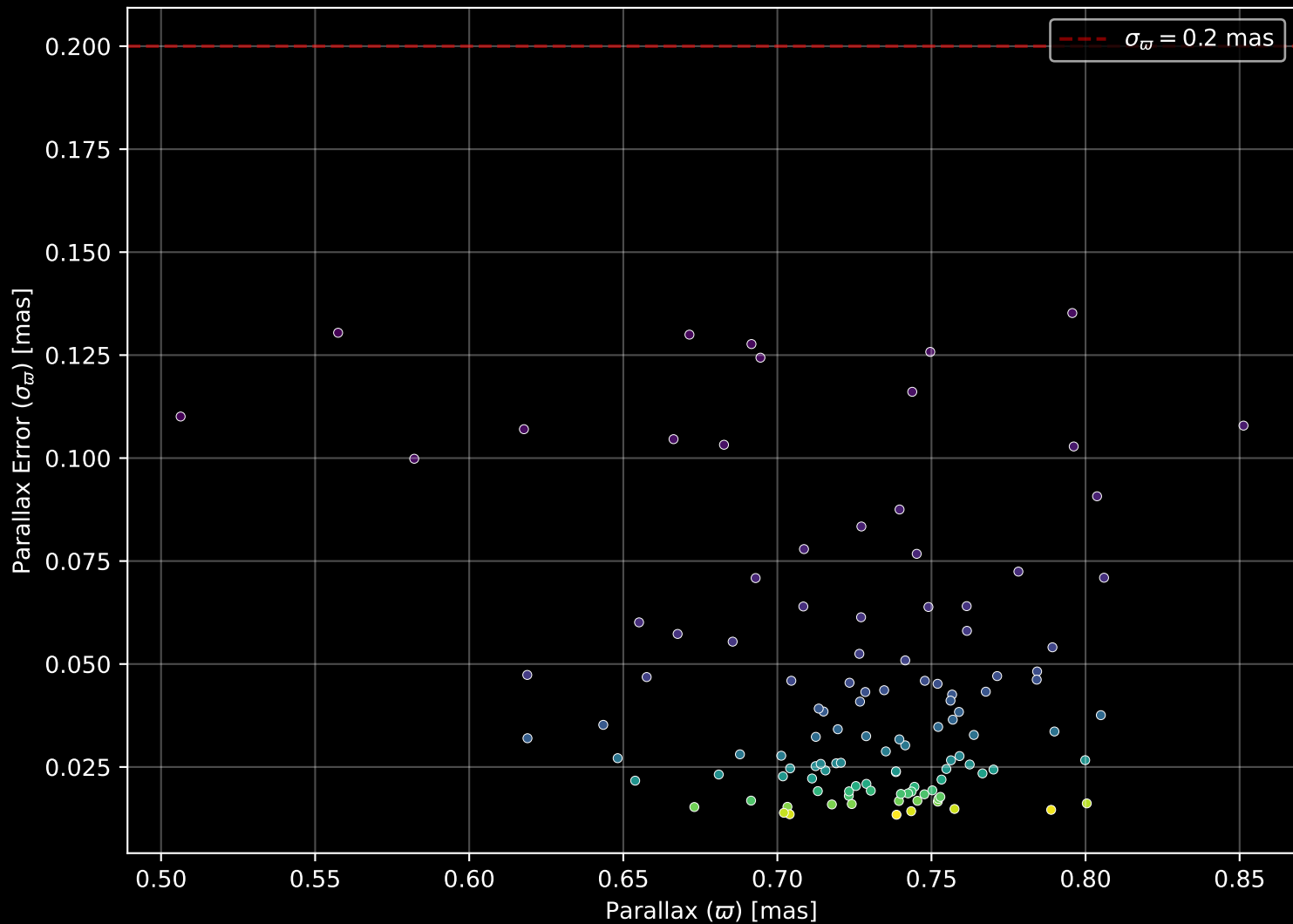
Gaia Cluster: [NGC_744] Parallax Quality (n= 116)
