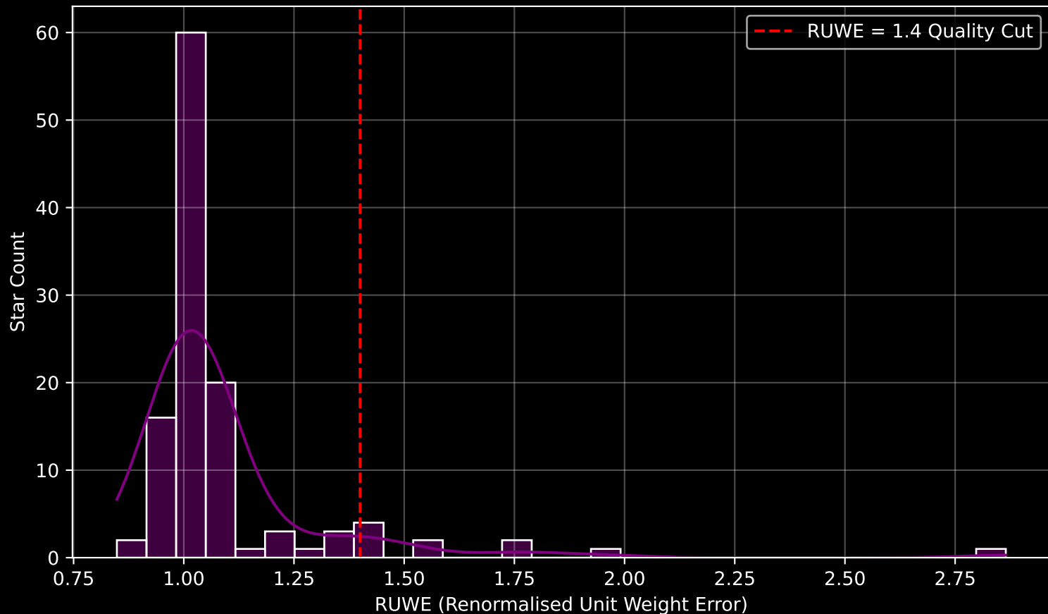
Gaia Cluster: [NGC_744] RUWE Distribution (n= 116)
