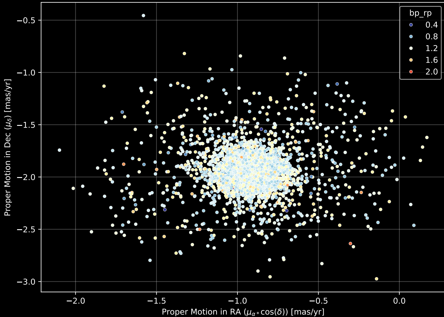
Gaia Cluster: [NGC_7789] Proper Motion Diagram (n= 3347)
