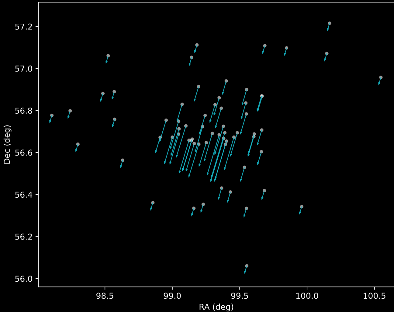
Gaia DR3 Cluster 178 Proper Motion Vectors (n=64)
