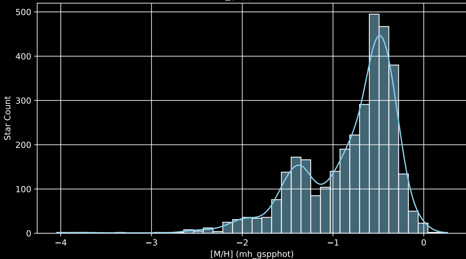
Gaia Cluster: [NGC_7789 [M/H] (mh_gspphot) (n= 3346)
