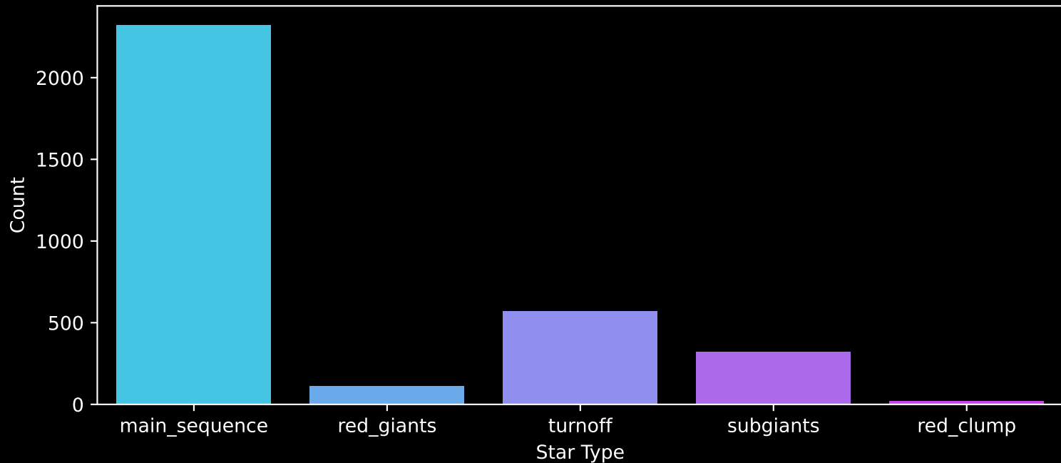
Gaia Cluster: [NGC_7789] Count plot of Star Type
