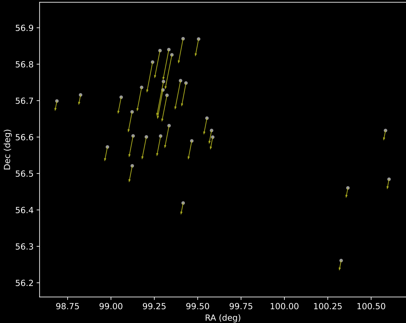
Gaia DR3 Cluster 116 Proper Motion Vectors (n=31)
