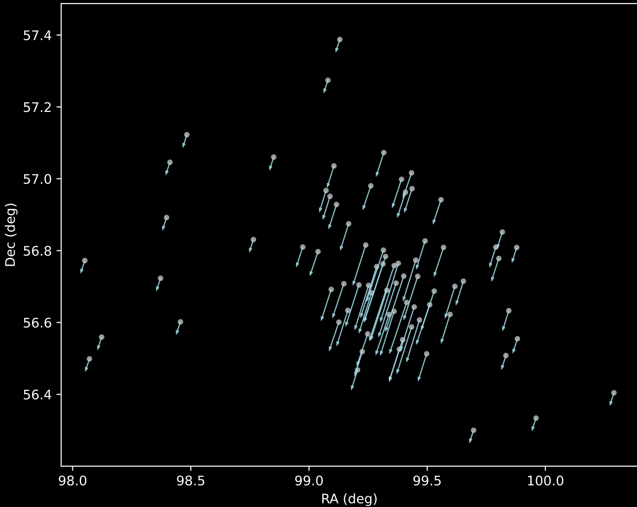
Gaia DR3 Cluster 159 Proper Motion Vectors (n=74)
