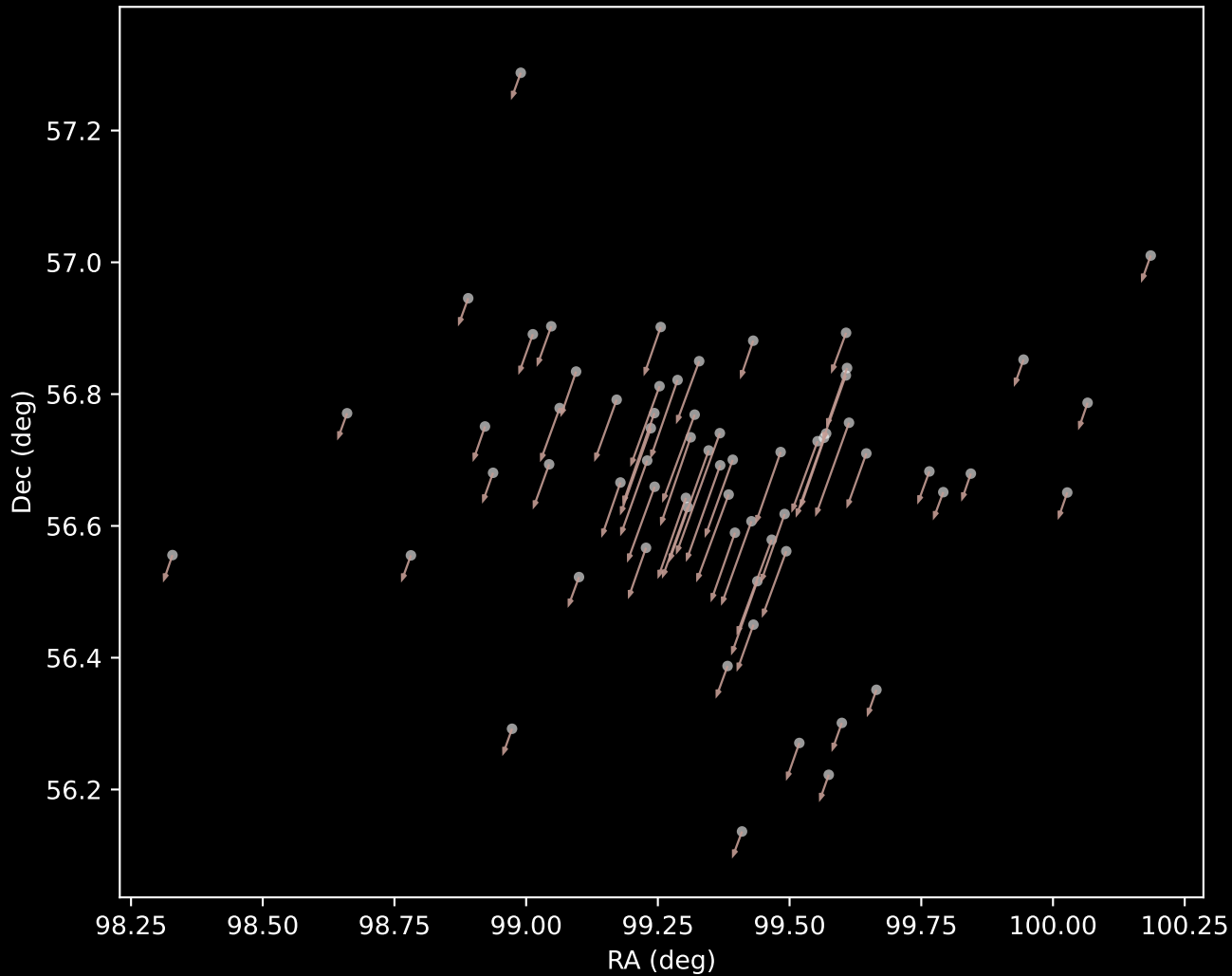
Gaia DR3 Cluster 151 Proper Motion Vectors (n=64)
