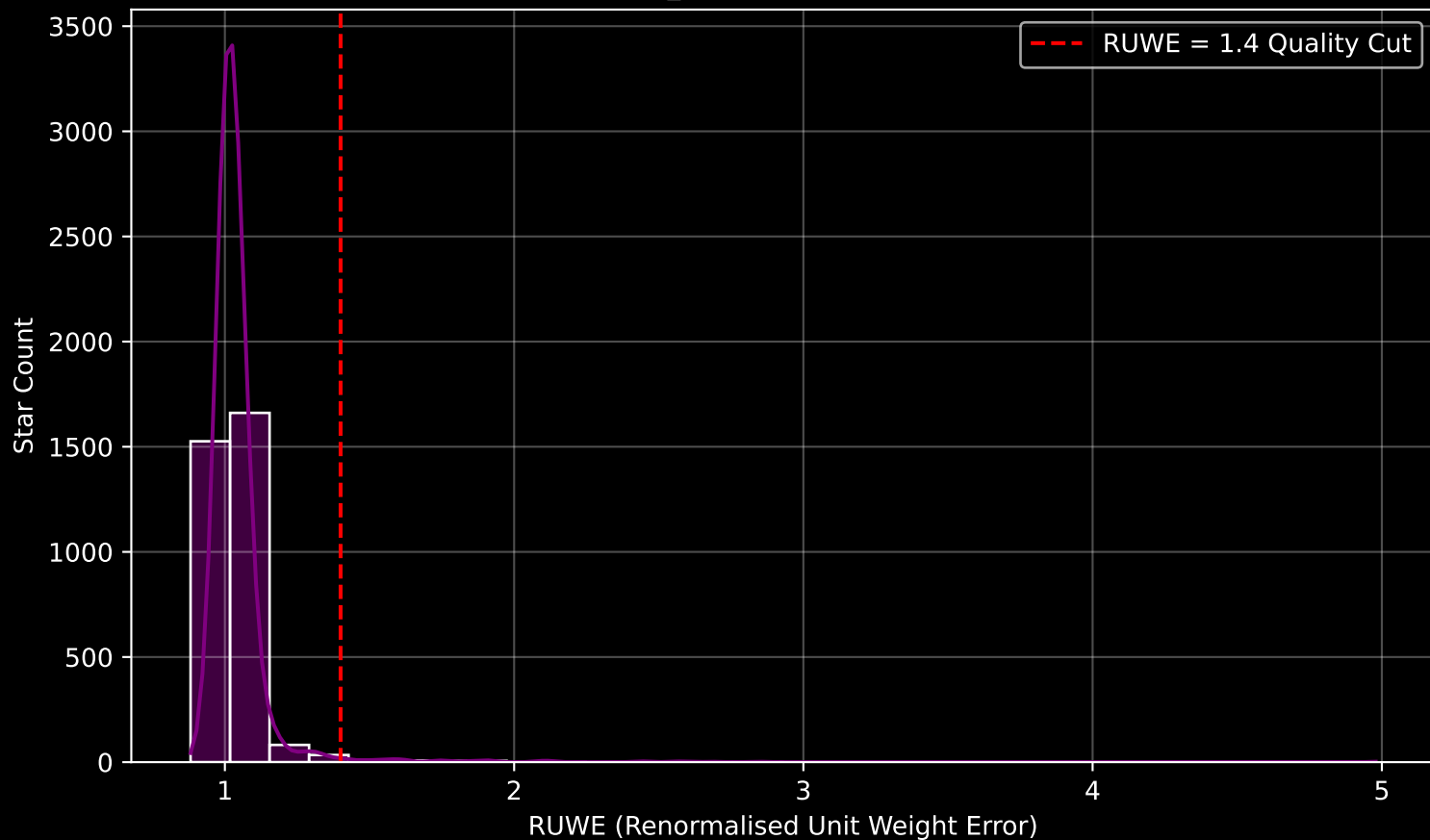
Gaia Cluster: [NGC_7789] RUWE Distribution (n= 3344)
