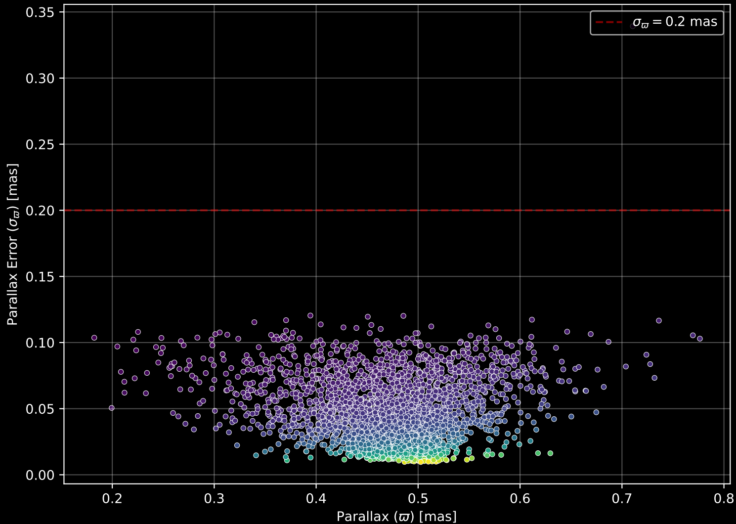
Gaia Cluster: [NGC_7789] Parallax Quality (n= 3347)
