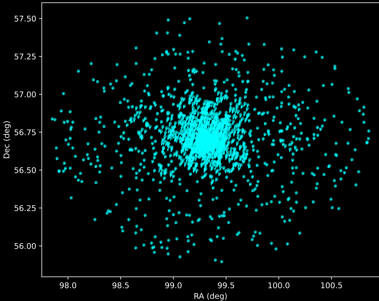
Gaia DR3 Noise Stream Proper Motion Vectors (n=1264)
