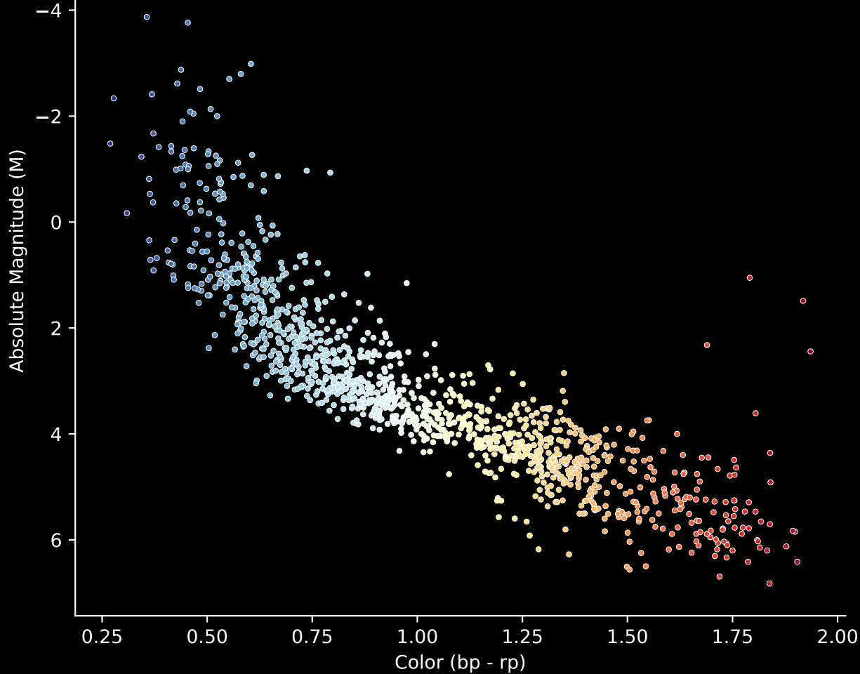
Gaia Cluster: [NGC_869] Stars (n= 1262) Hertzsprung-Russel Diagram
