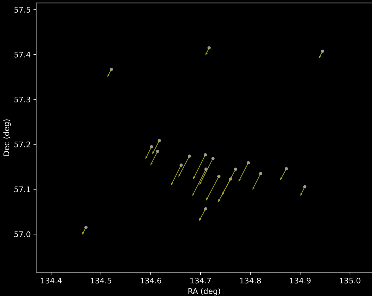
Gaia DR3 Cluster 36 Proper Motion Vectors (n=20)
