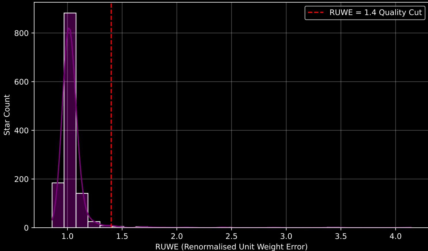
Gaia Cluster: [NGC_869] RUWE Distribution (n= 1260)
