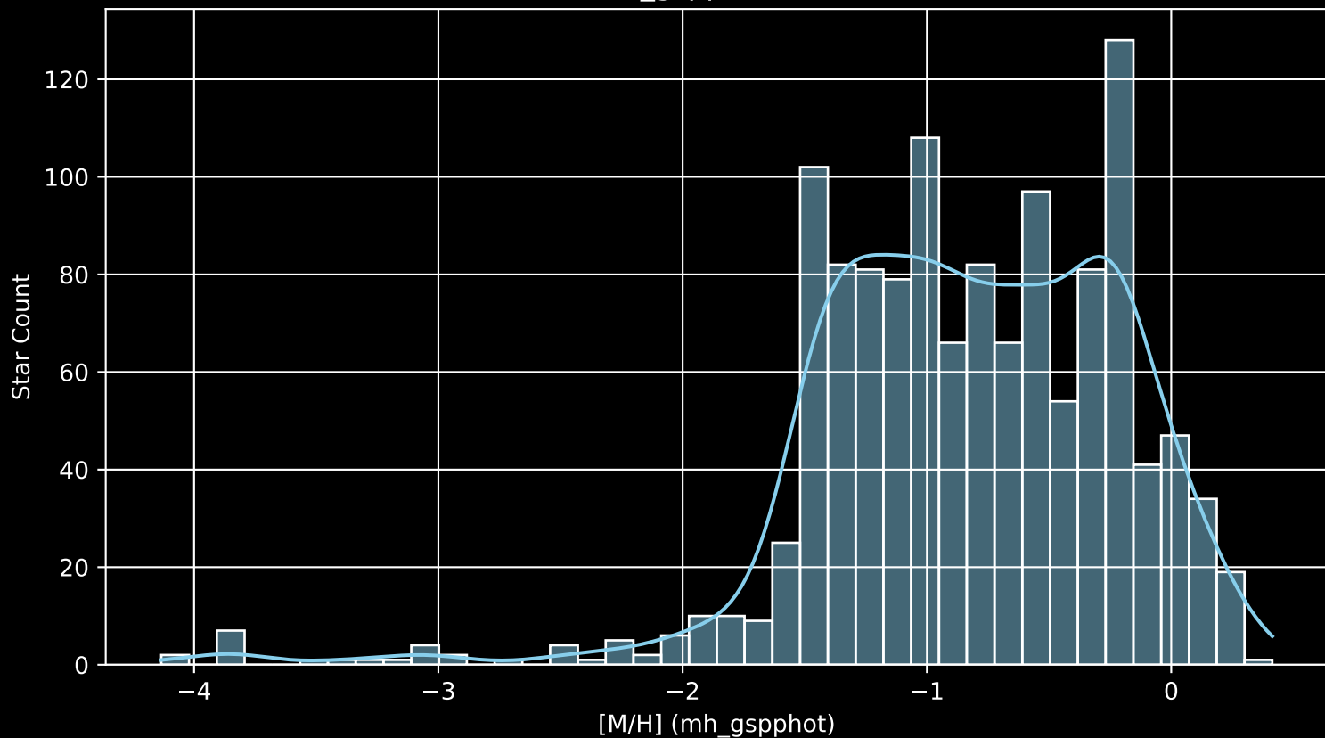
Gaia Cluster: [NGC_869 [M/H] (mh_gspphot) (n= 1260)
