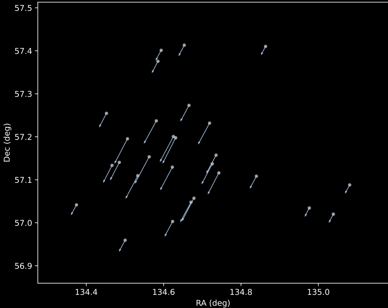
Gaia DR3 Cluster 41 Proper Motion Vectors (n=28)
