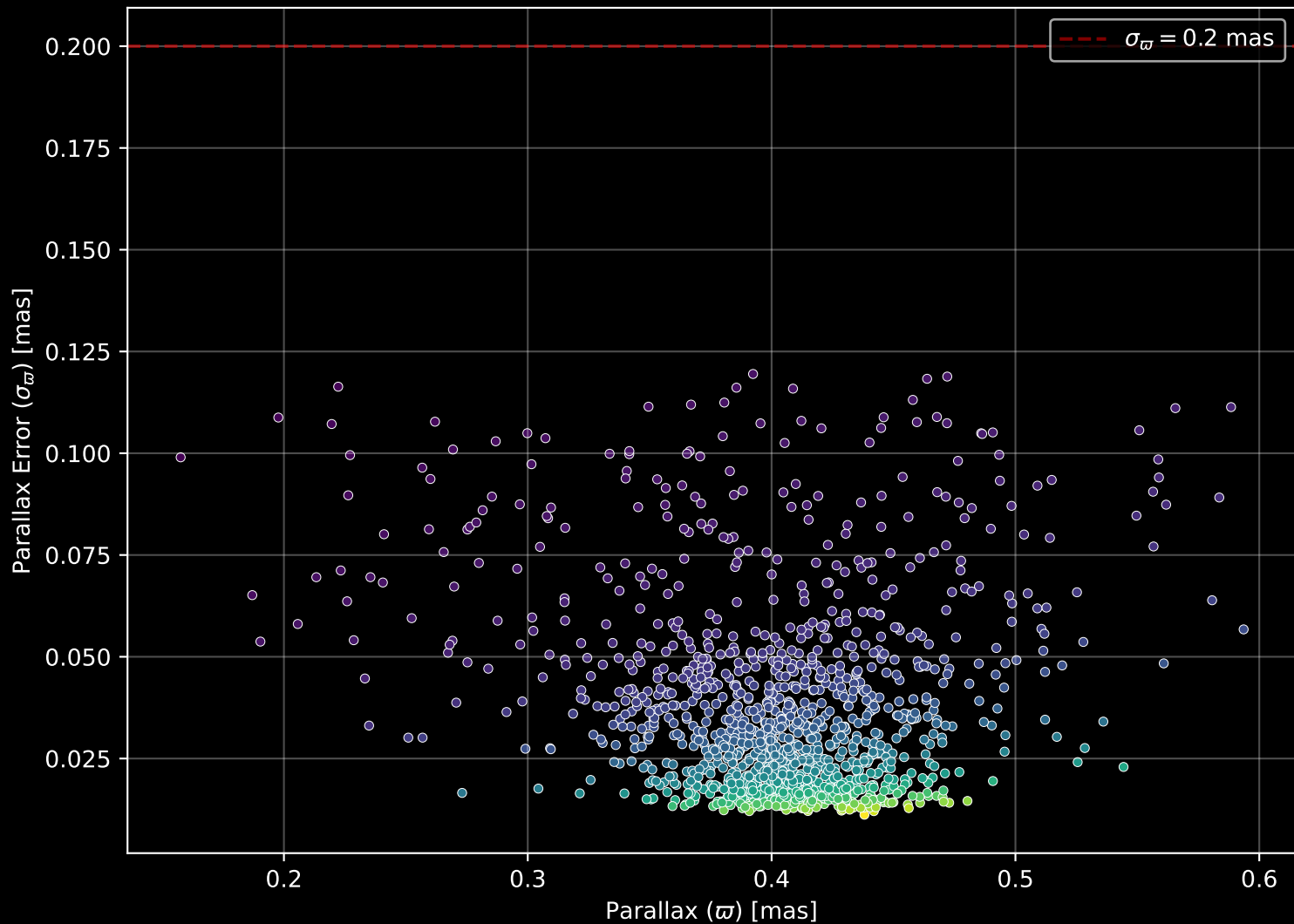
Gaia Cluster: [NGC_869] Parallax Quality (n= 1262)
