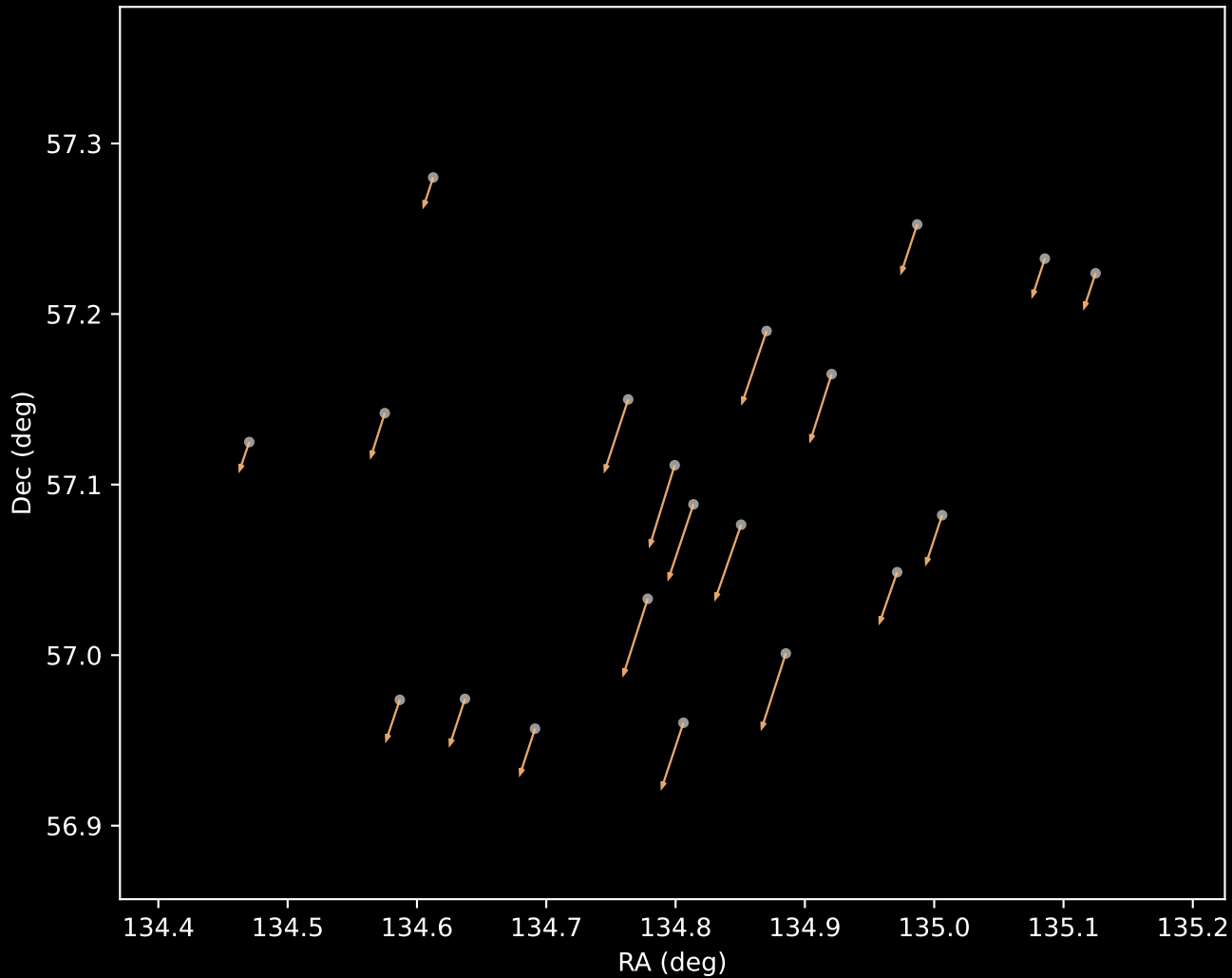
Gaia DR3 Cluster 23 Proper Motion Vectors (n=20)
