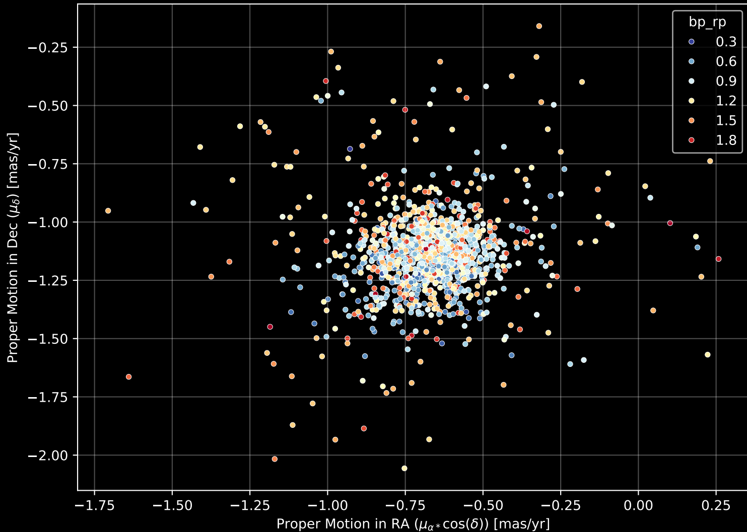
Gaia Cluster: [NGC_869] Proper Motion Diagram (n= 1262)
