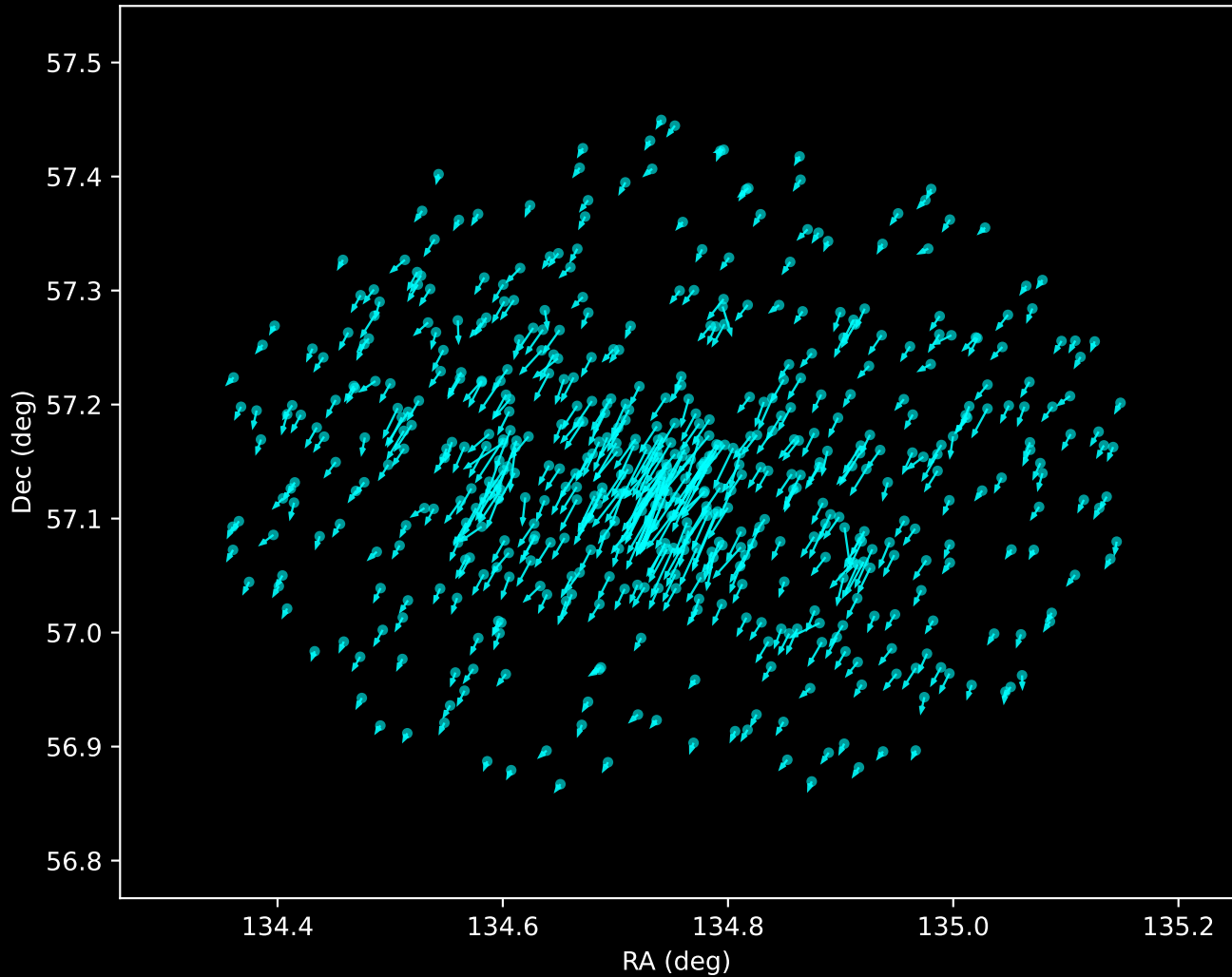
Gaia DR3 Noise Stream Proper Motion Vectors (n=544)
