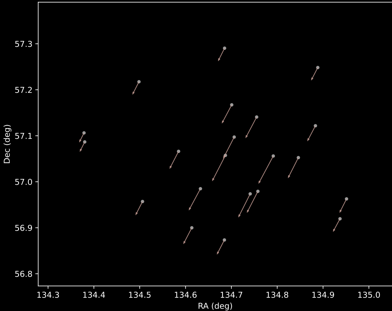
Gaia DR3 Cluster 71 Proper Motion Vectors (n=21)
