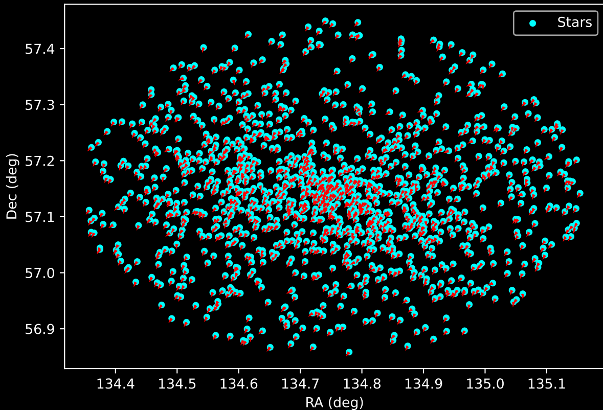
Gaia Cluster: [NGC_869] Proper Motion Vectors for Gaia Star Field (n= 1262)
