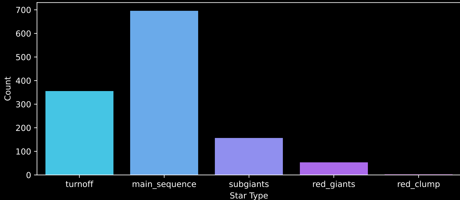
Gaia Cluster: [NGC_869] Count plot of Star Type
