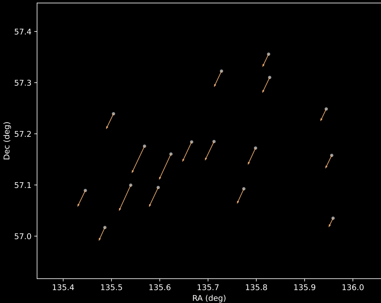
Gaia DR3 Cluster 43 Proper Motion Vectors (n=17)
