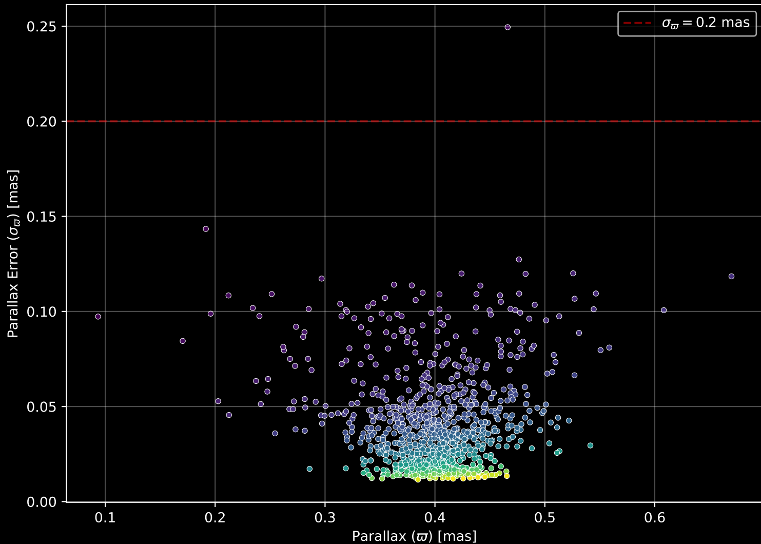
Gaia Cluster: [NGC_884] Parallax Quality (n= 981)
