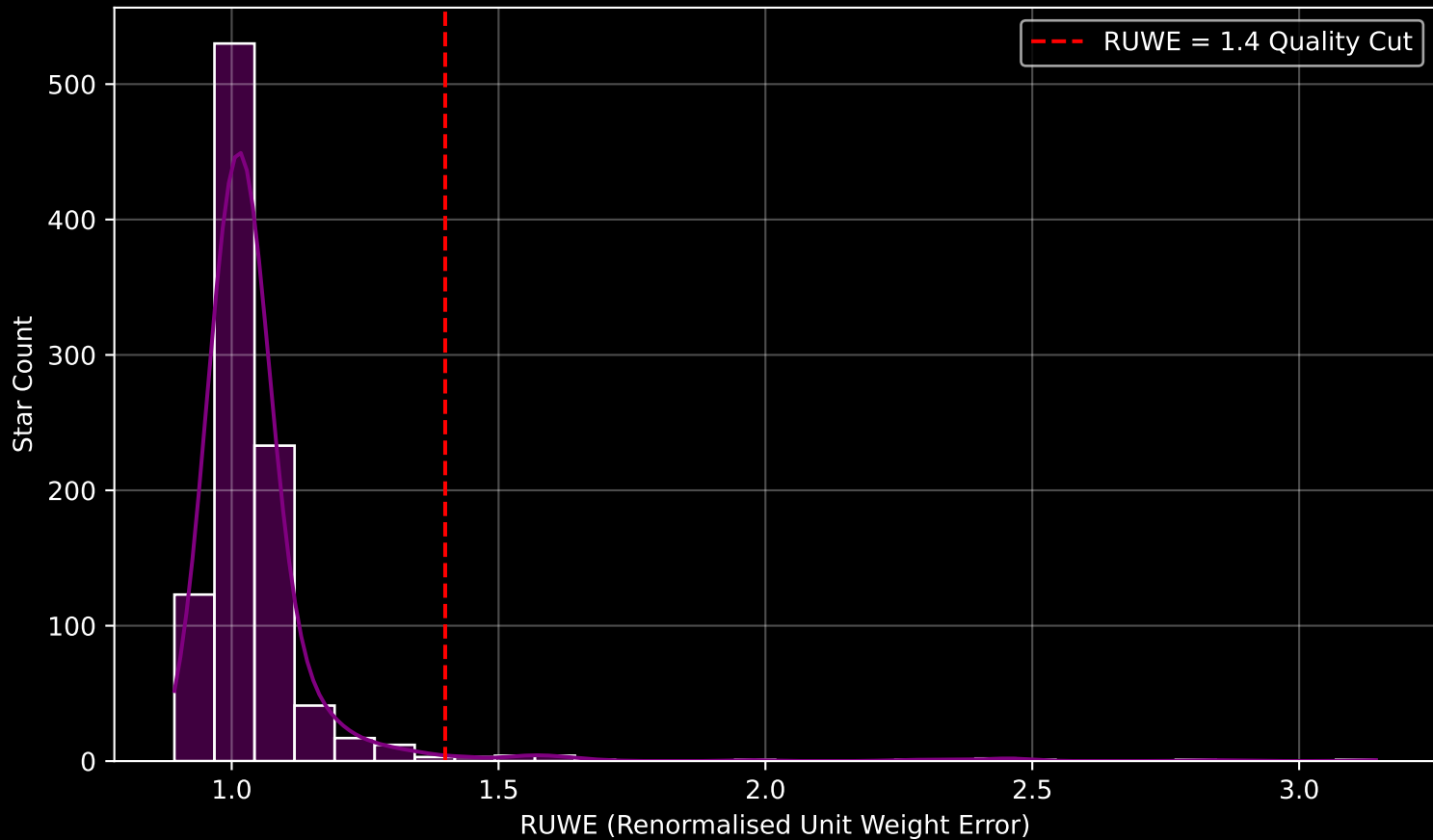
Gaia Cluster: [NGC_884] RUWE Distribution (n= 979)
