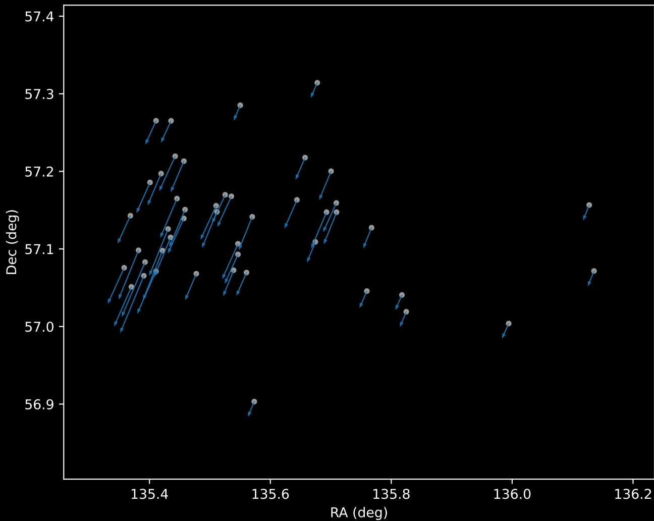
Gaia DR3 Cluster 20 Proper Motion Vectors (n=46)
