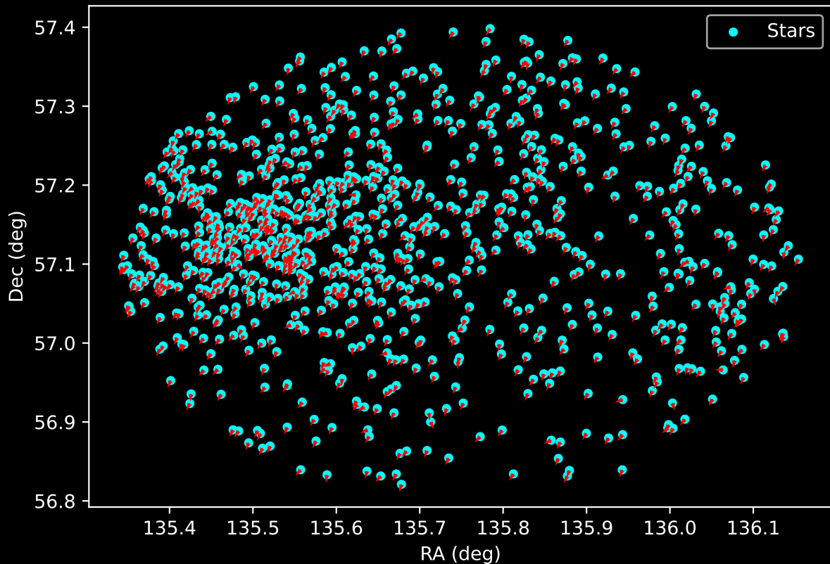
Gaia Cluster: [NGC_884] Proper Motion Vectors for Gaia Star Field (n= 981)
