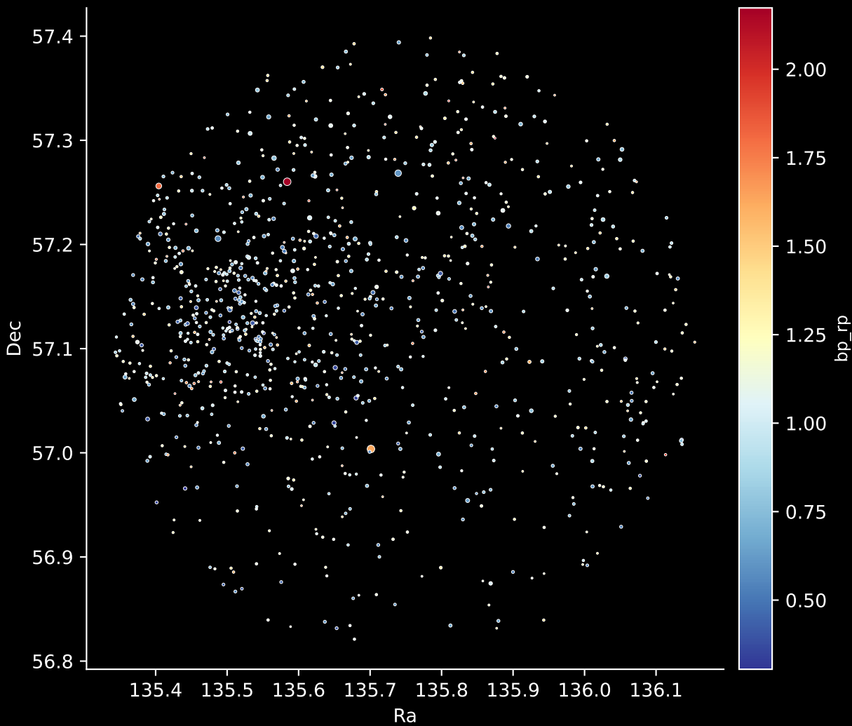
Gaia Cluster: [NGC_884] Stars: 981
