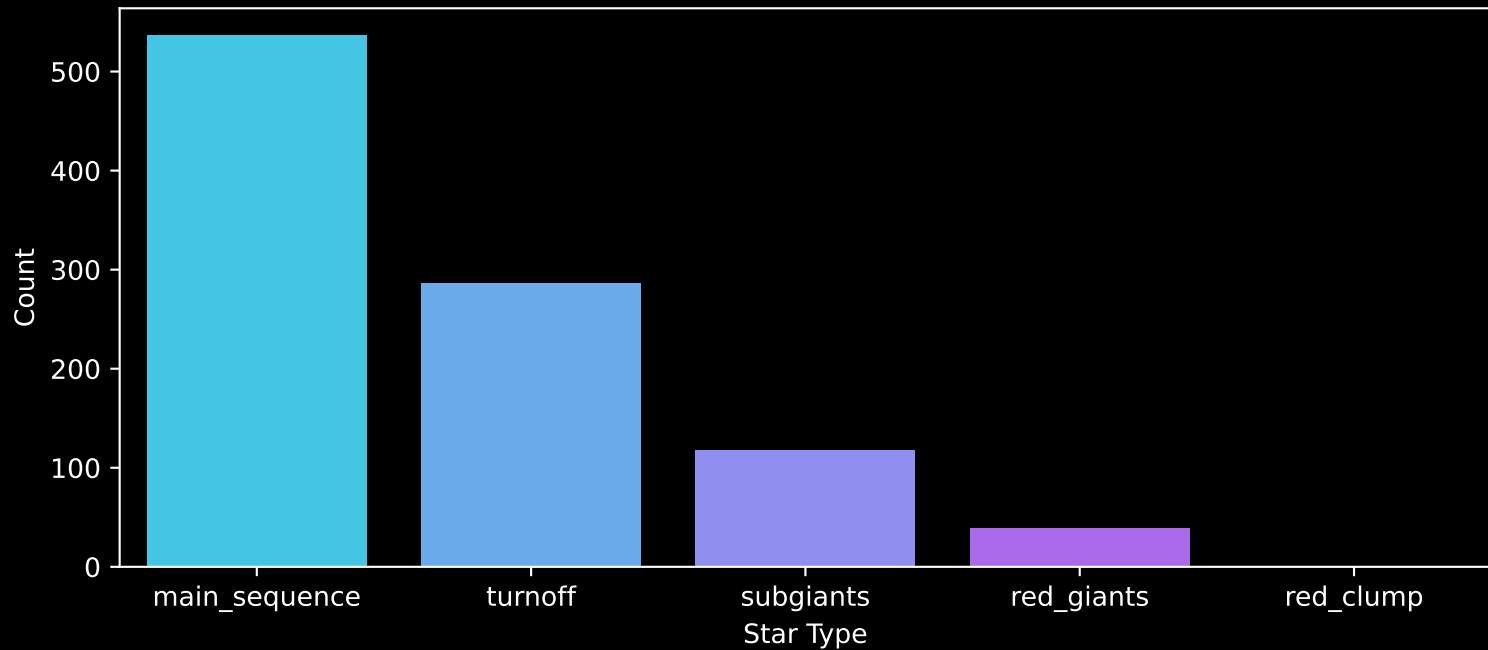
Gaia Cluster: [NGC_884] Count plot of Star Type
