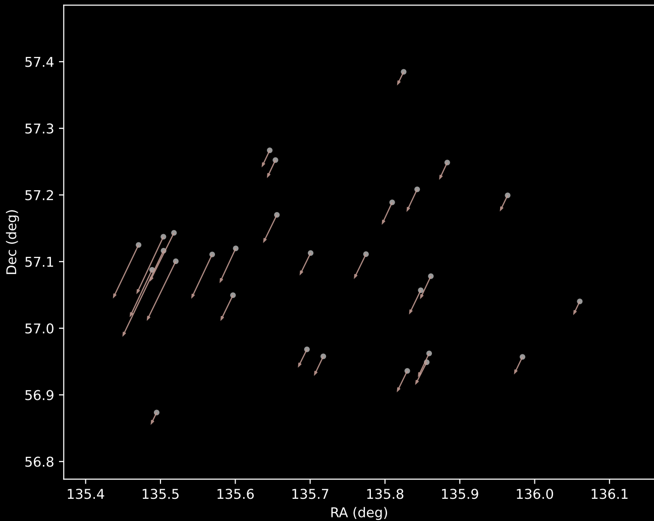
Gaia DR3 Cluster 11 Proper Motion Vectors (n=29)
