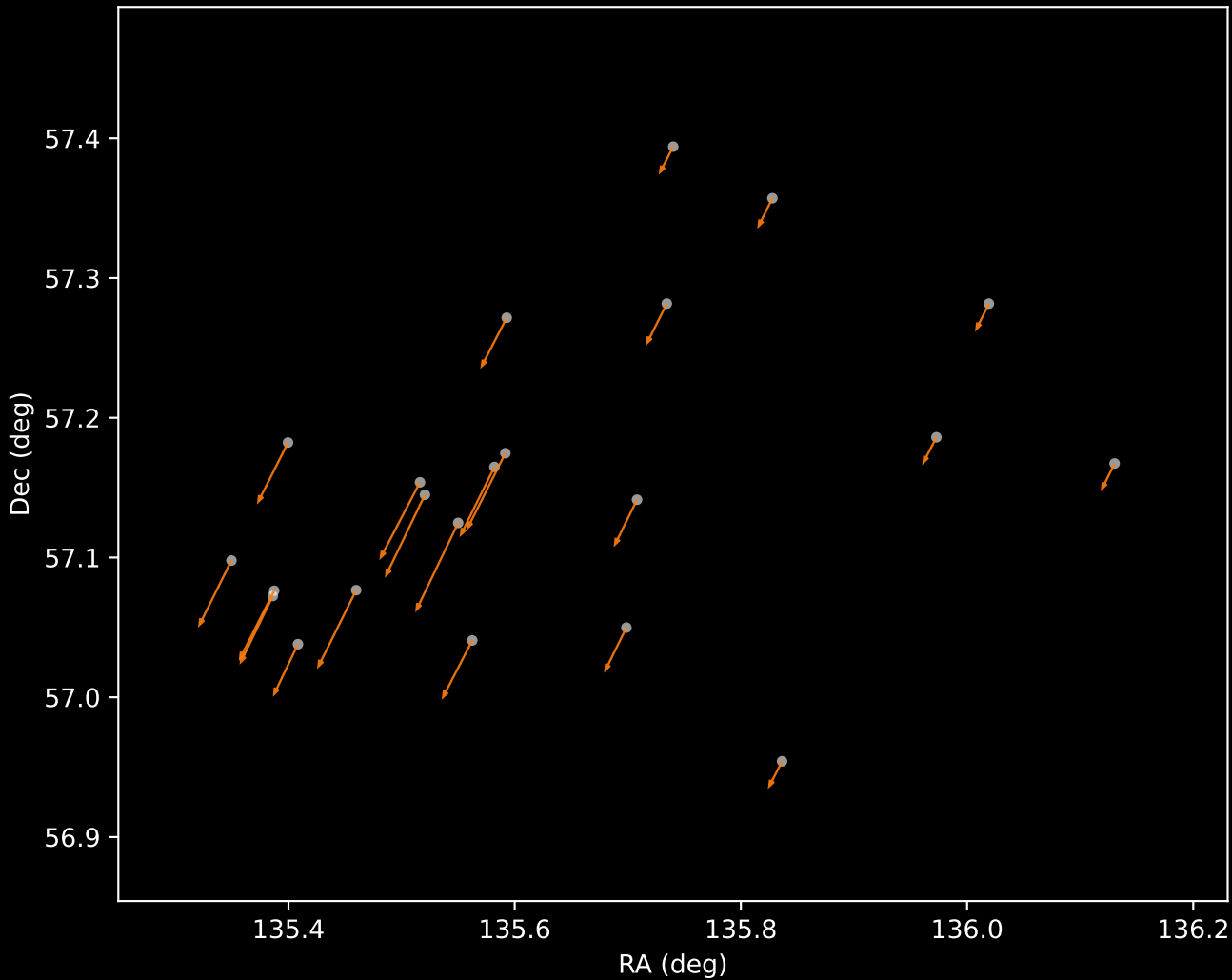
Gaia DR3 Cluster 22 Proper Motion Vectors (n=22)
