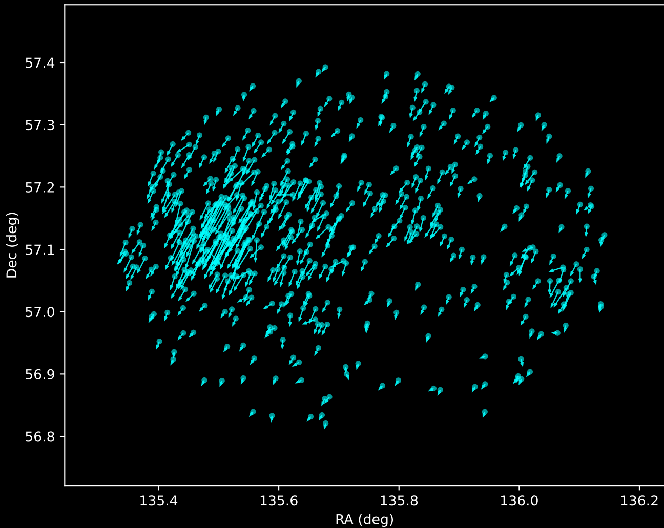
Gaia DR3 Noise Stream Proper Motion Vectors (n=511)
