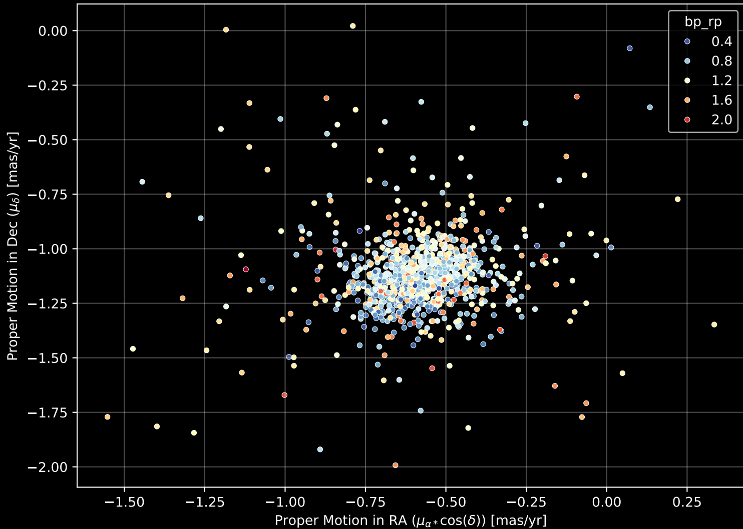
Gaia Cluster: [NGC_884] Proper Motion Diagram (n= 981)
