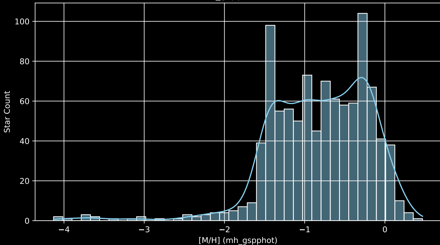
Gaia Cluster: [NGC_884 [M/H] (mh_gspphot) ( \bar{n}=980 )
