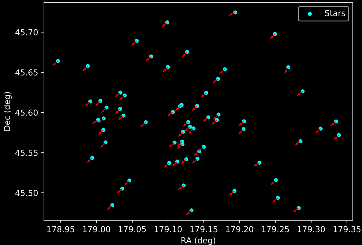
Gaia Cluster: [Patchick_3] Proper Motion Vectors for Gaia Star Field (n= 63)
