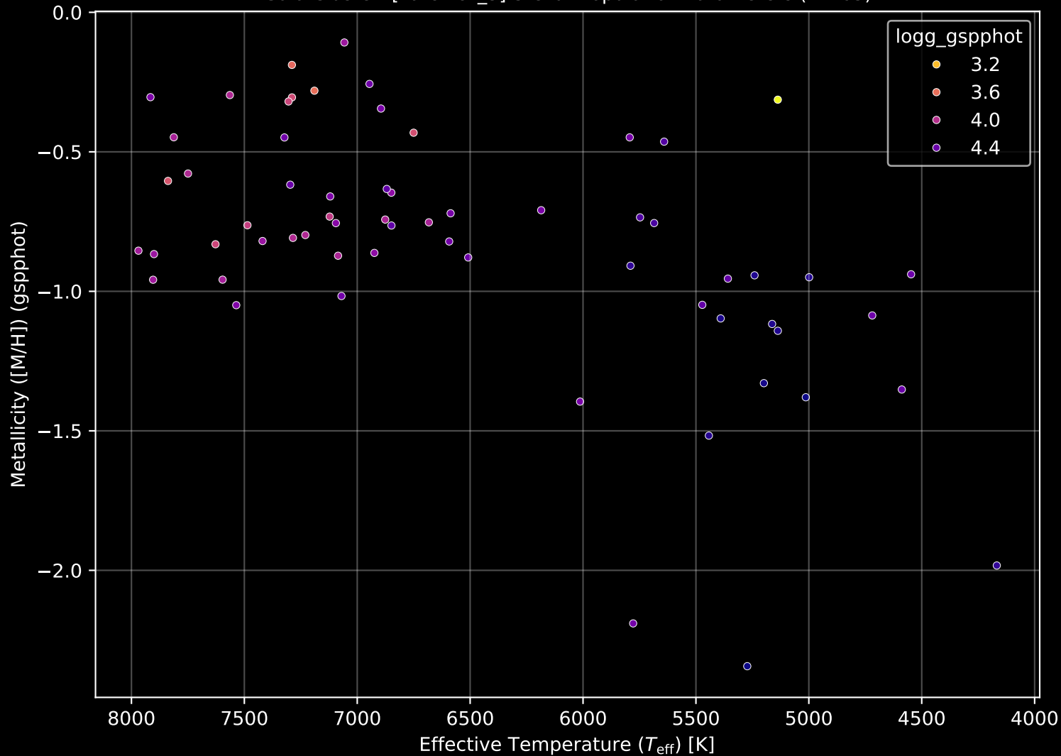
Gaia Cluster: [Patchick_3] Stellar Population Parameters (n= 63)
