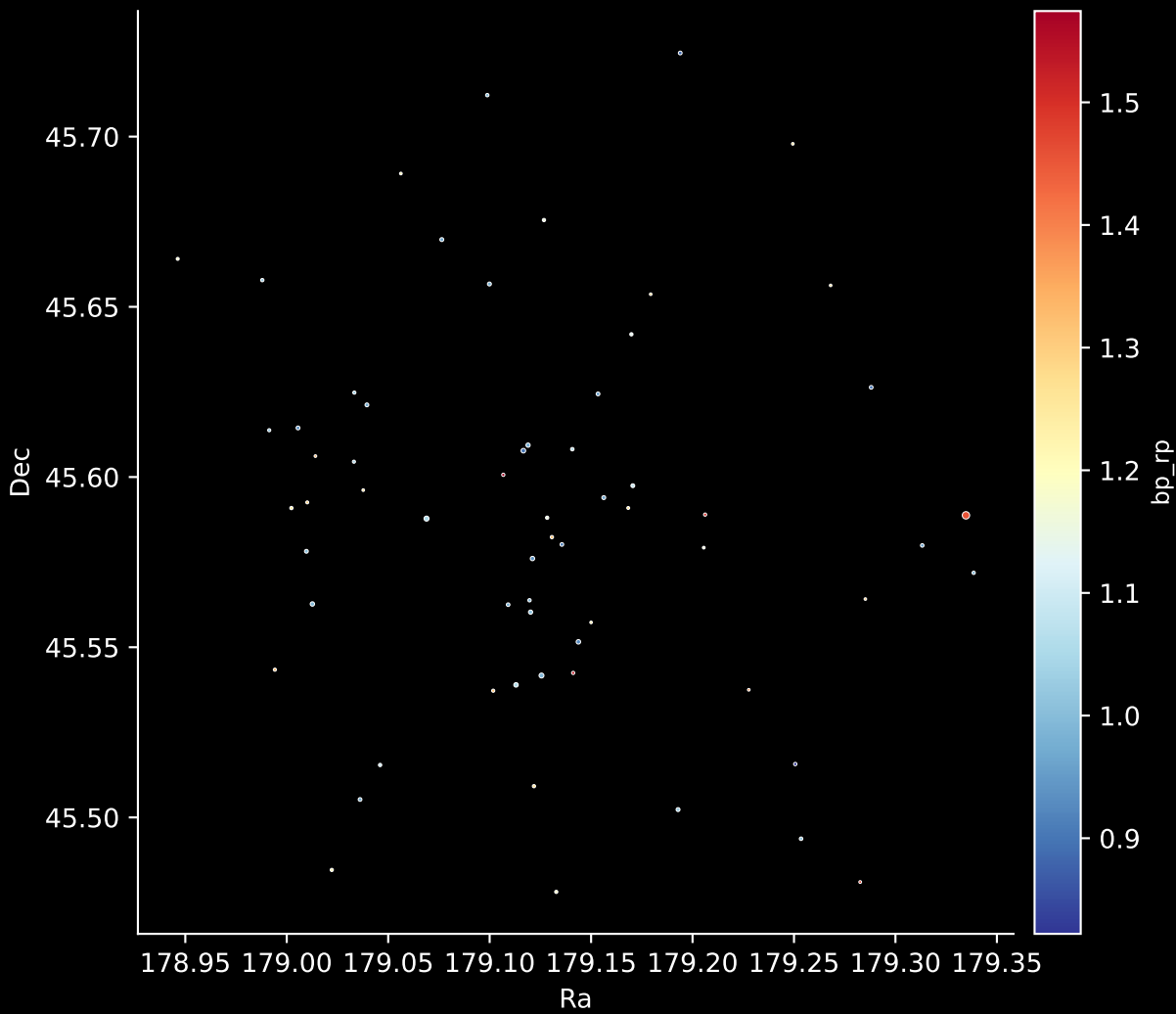
Gaia Cluster: [Patchick_3] Stars: 63
