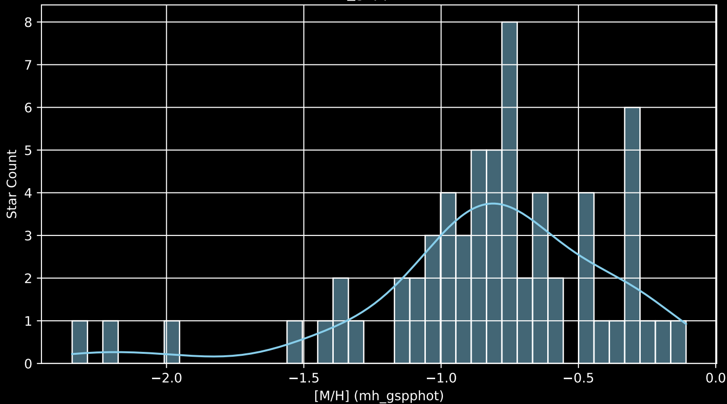
Gaia Cluster: [Patchick_3 [M/H] (mh_gspphot) (n= 63)
