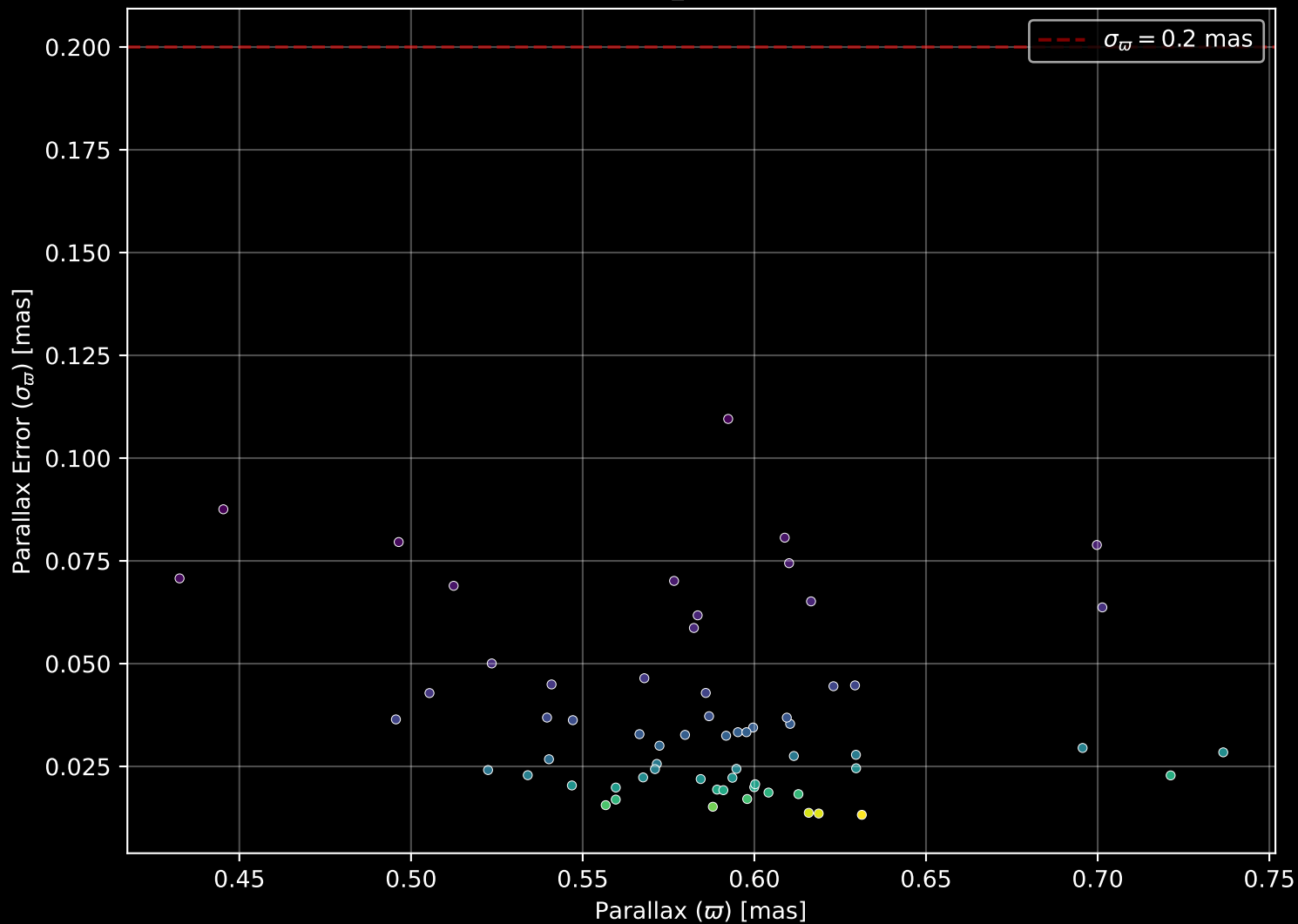
Gaia Cluster: [Patchick_3] Parallax Quality (n= 63)
