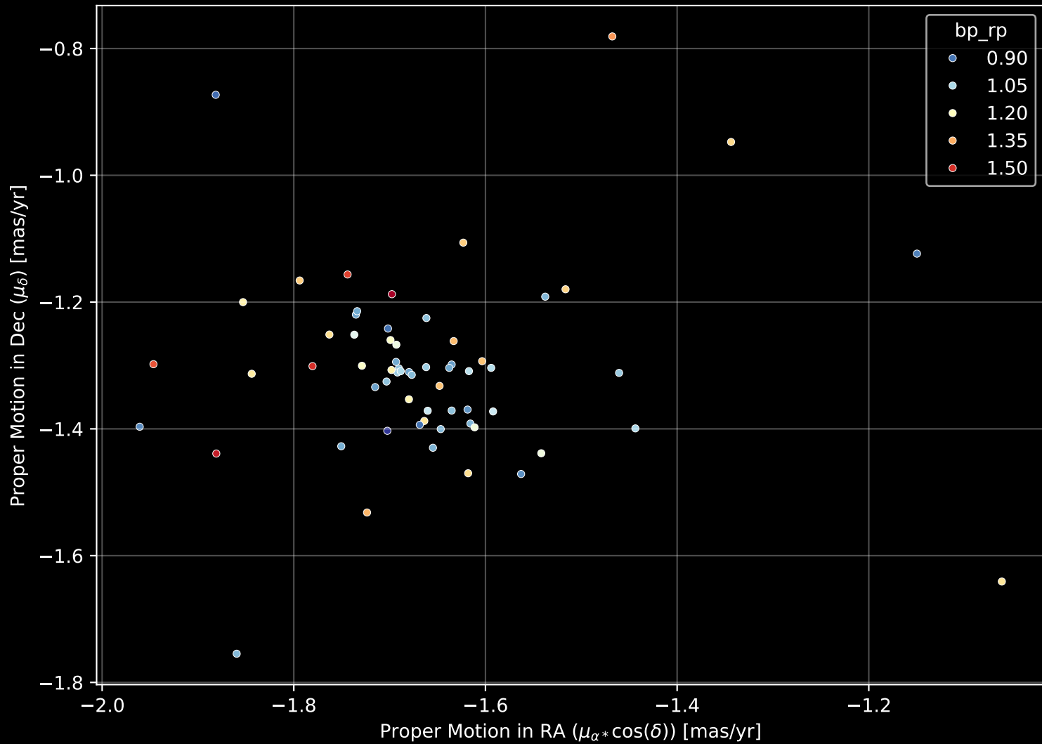
Gaia Cluster: [Patchick_3] Proper Motion Diagram (n= 63)
