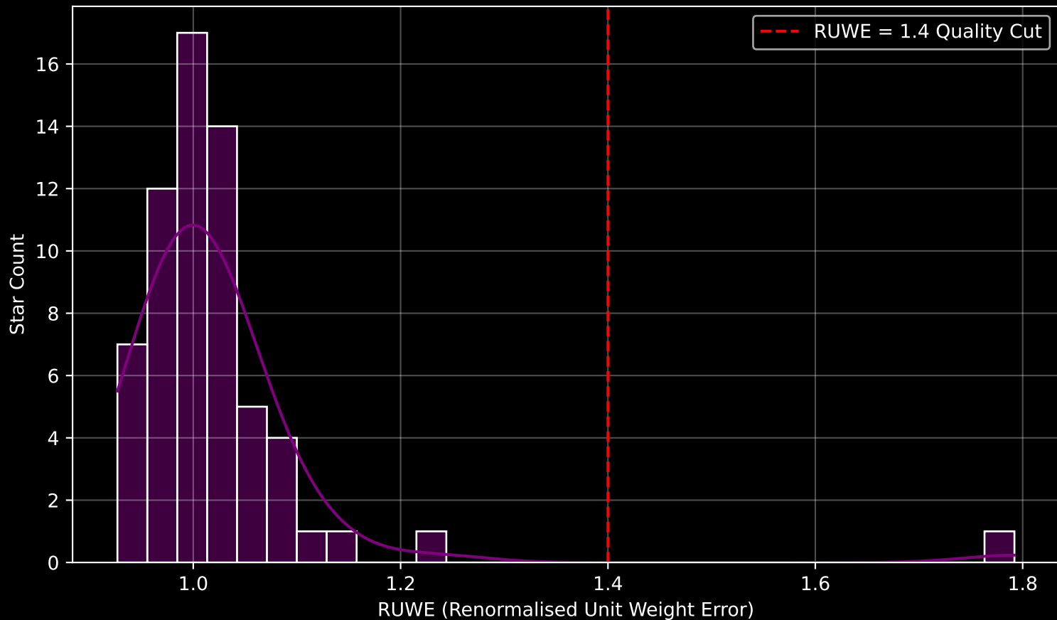
Gaia Cluster: [Patchick_3] RUWE Distribution (n= 63)
