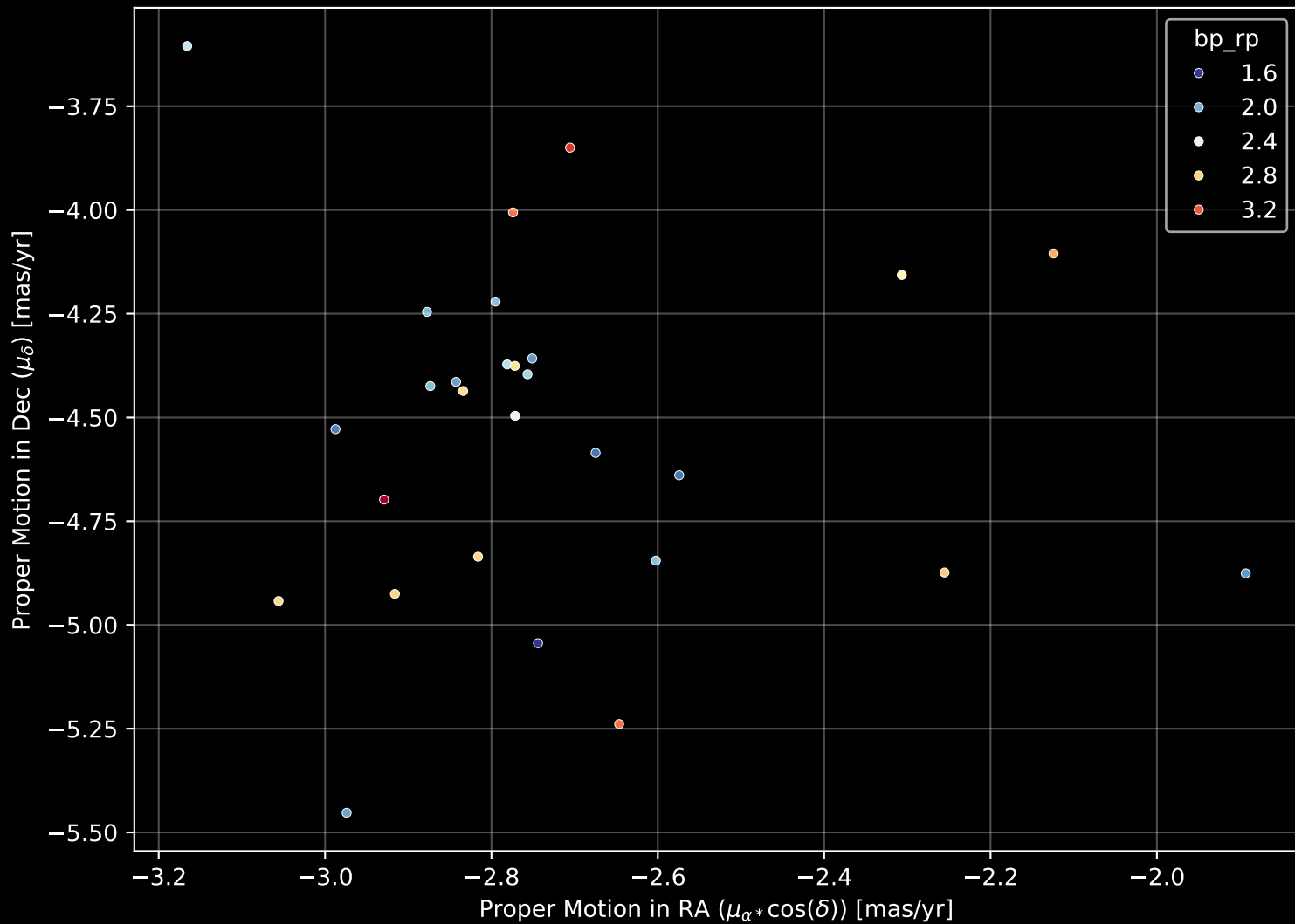
Gaia Cluster: [Patchick_75] Proper Motion Diagram (n= 28)
