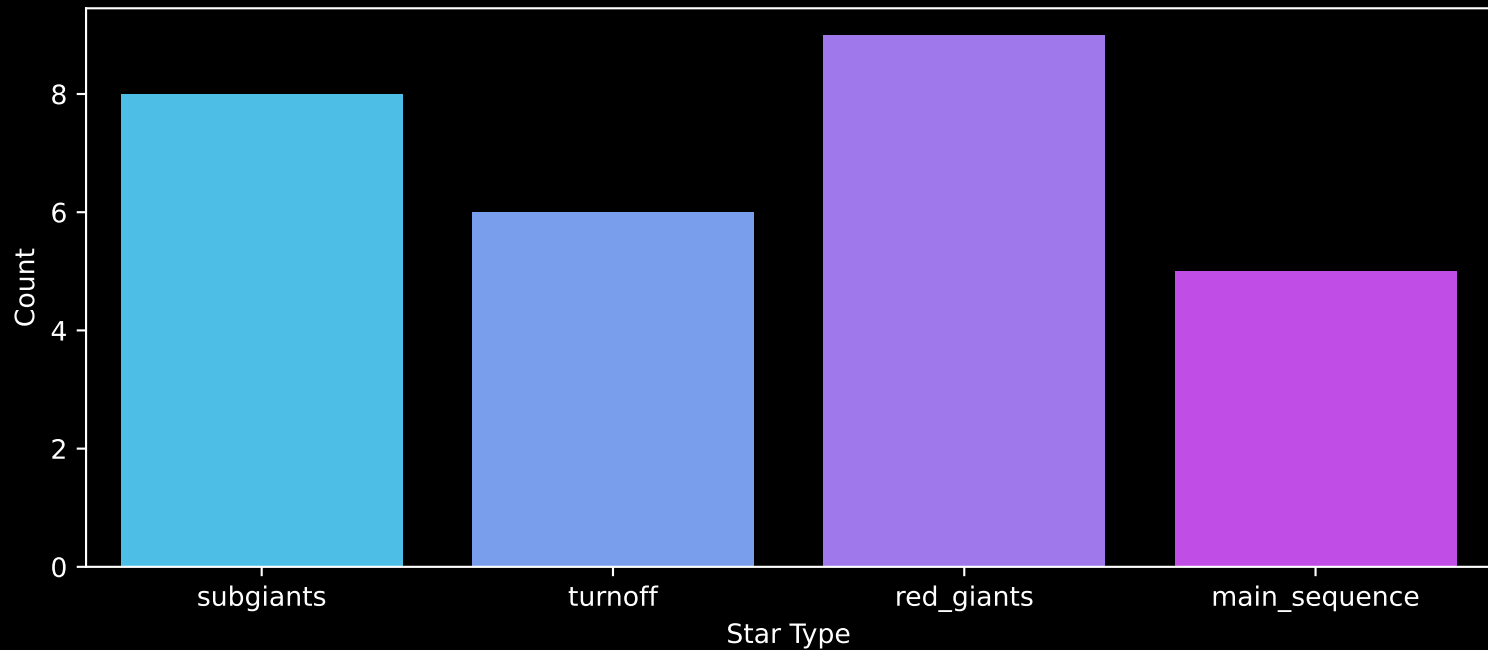
Gaia Cluster: [Patchick_75] Count plot of Star Type
