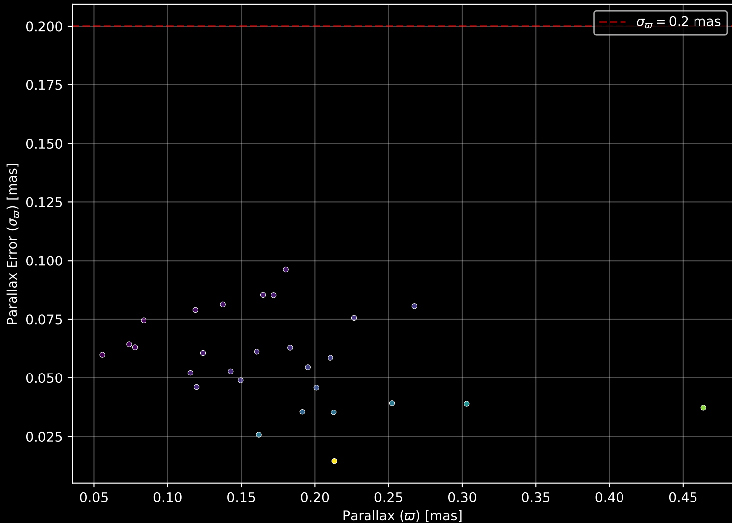
Gaia Cluster: [Patchick_75] Parallax Quality (n= 28)
