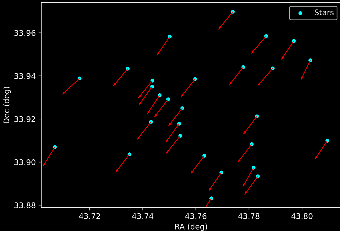
Gaia Cluster: [Patchick_75] Proper Motion Vectors for Gaia Star Field (n= 28)
