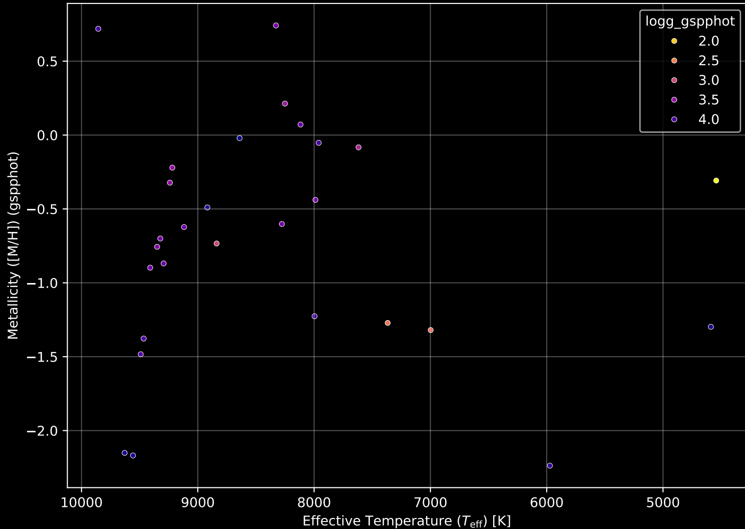
Gaia Cluster: [Patchick_75] Stellar Population Parameters (n= 28)
