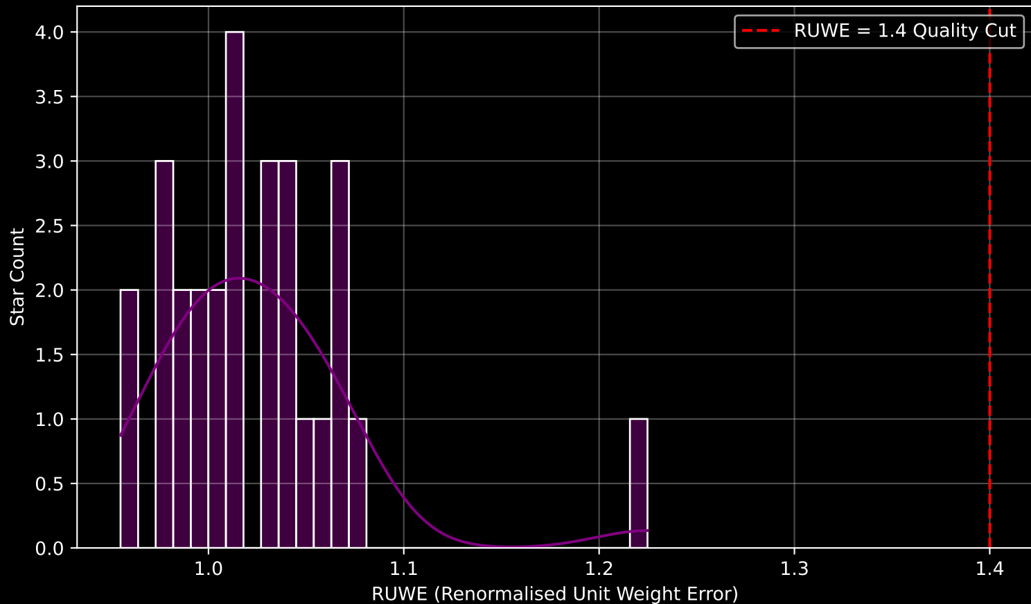
Gaia Cluster: [Patchick_75] RUWE Distribution (n= 28)
