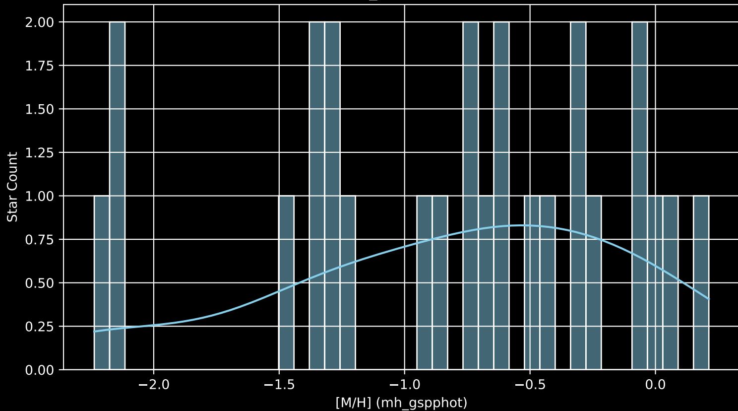
Gaia Cluster: [Patchick_75 [M/H] (mh_gspphot) (n= 26)
