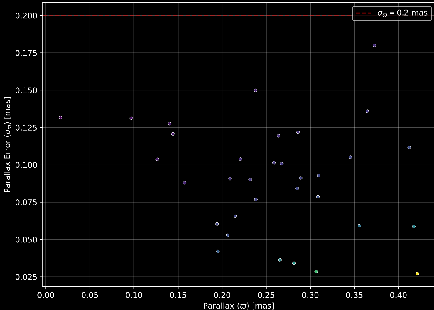
Gaia Cluster: [Patchick_94] Parallax Quality (n= 33)
