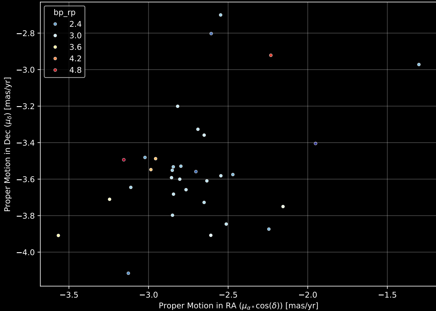
Gaia Cluster: [Patchick_94] Proper Motion Diagram (n= 33)
