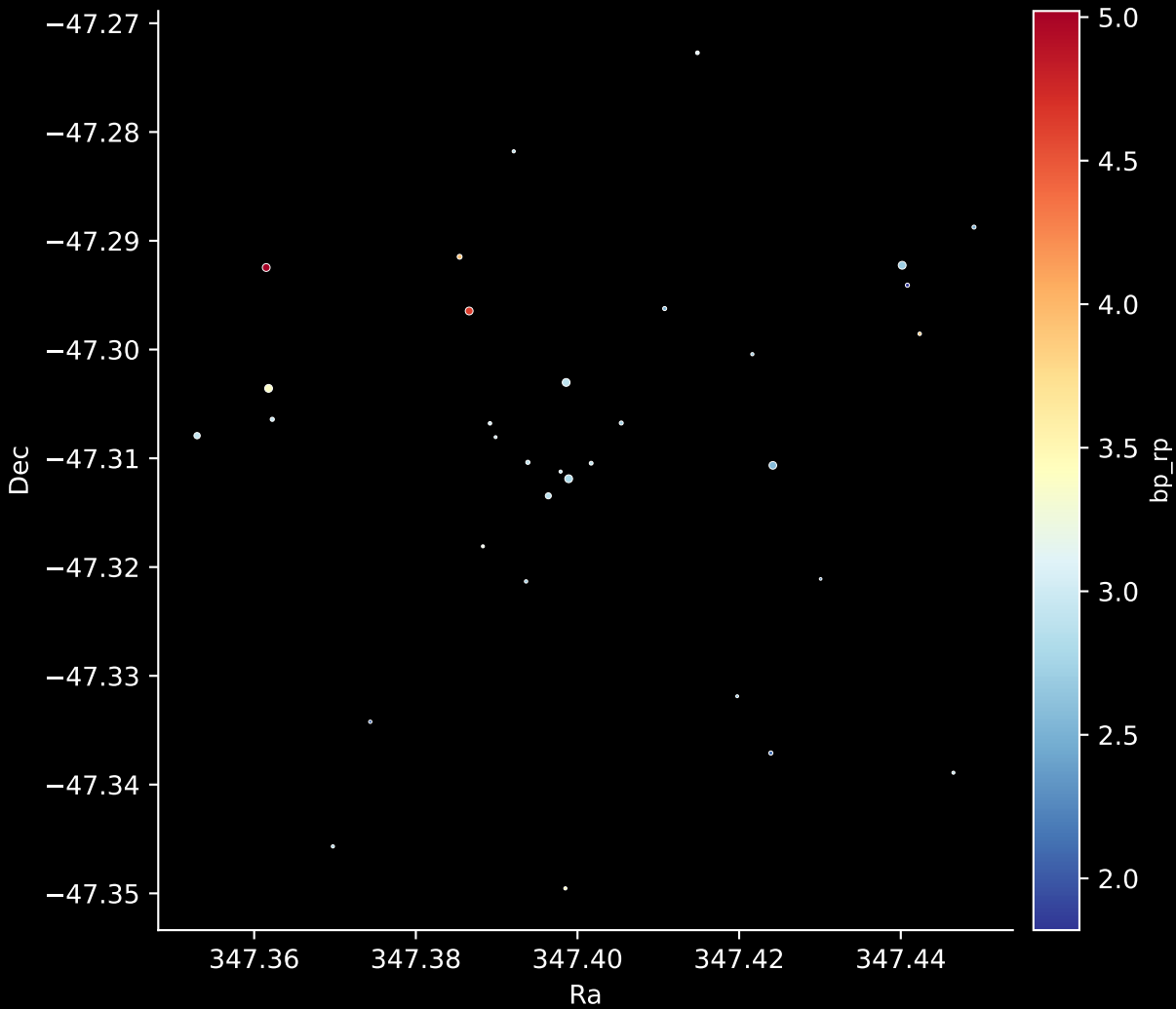
Gaia Cluster: [Patchick_94] Stars: 33
