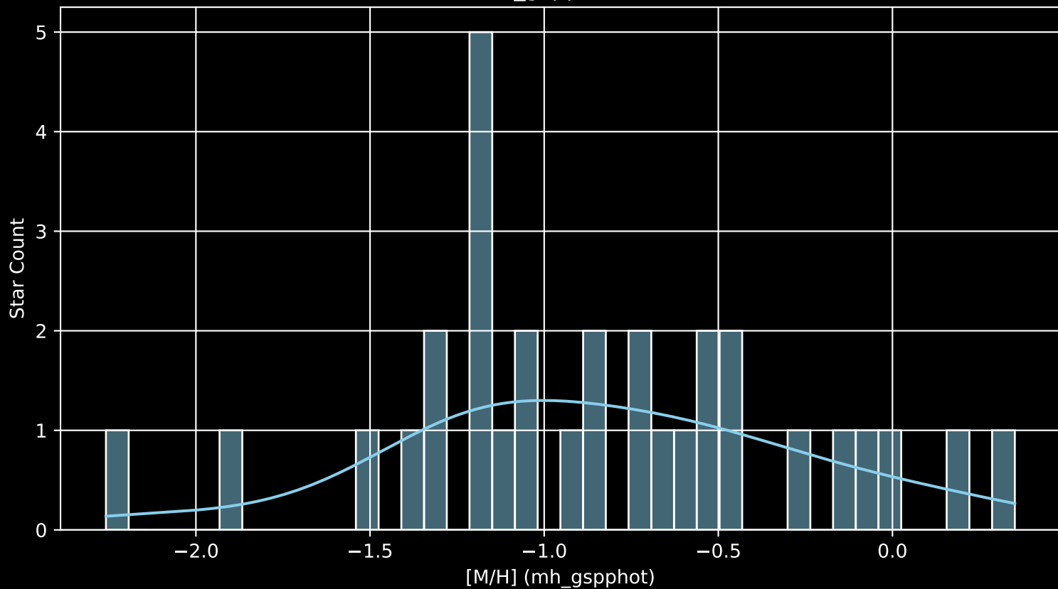
Gaia Cluster: [Patchick_94 [M/H] (mh_gspphot) (n= 31)
