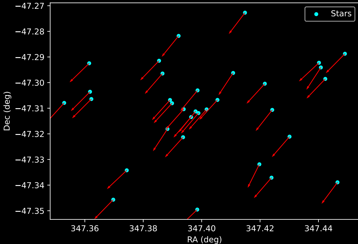
Gaia Cluster: [Patchick_94] Proper Motion Vectors for Gaia Star Field (n= 33)
