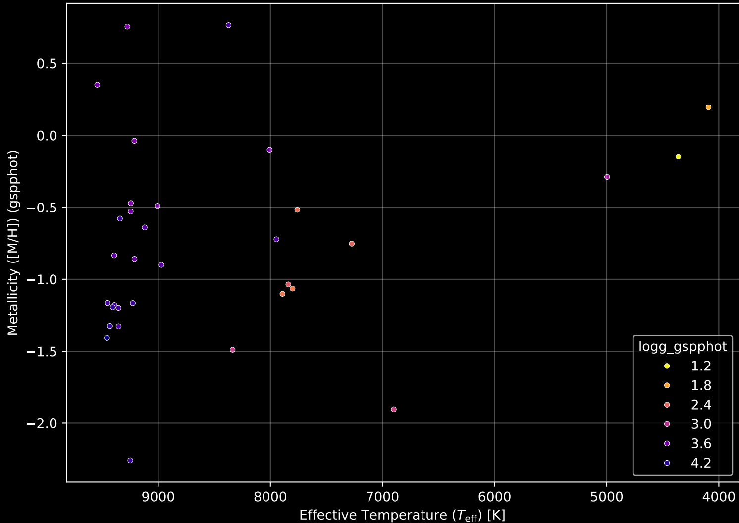
Gaia Cluster: [Patchick_94] Stellar Population Parameters (n= 33)
