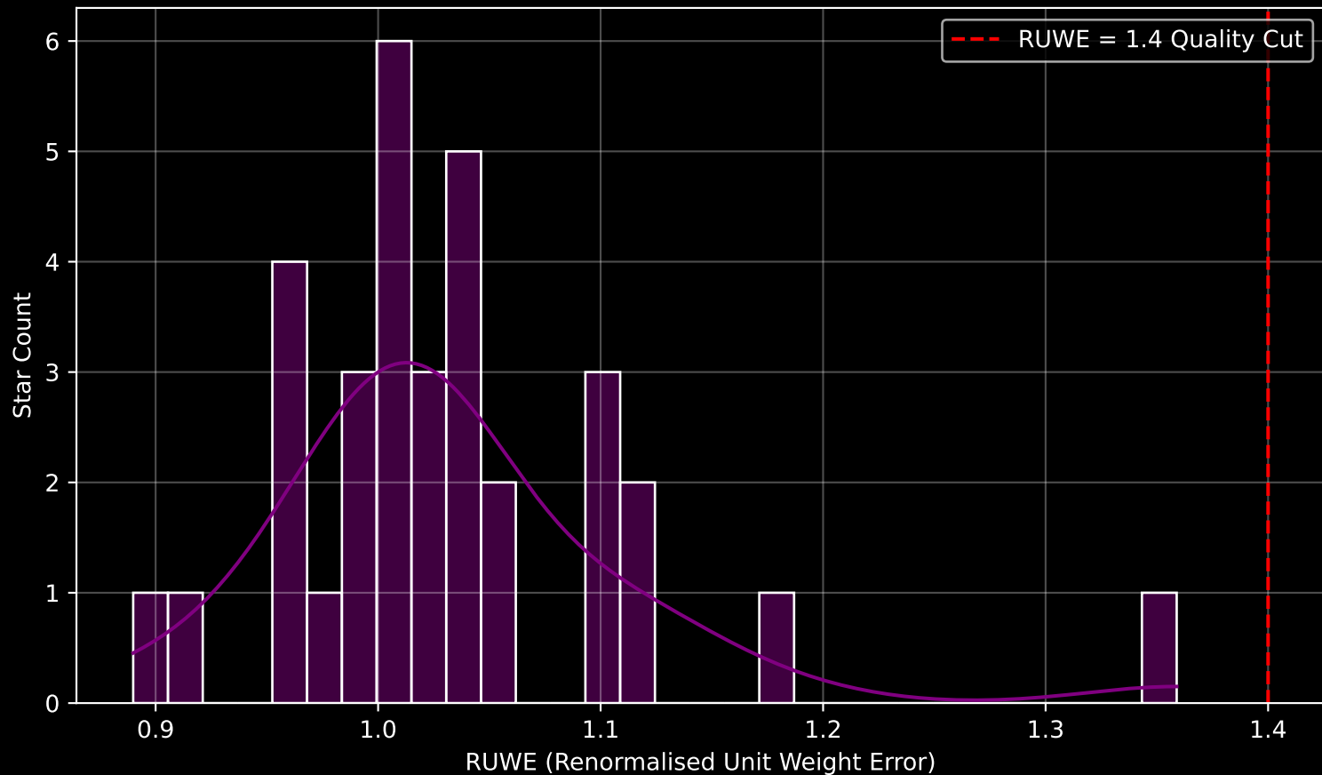
Gaia Cluster: [Patchick_94] RUWE Distribution (n= 33)
