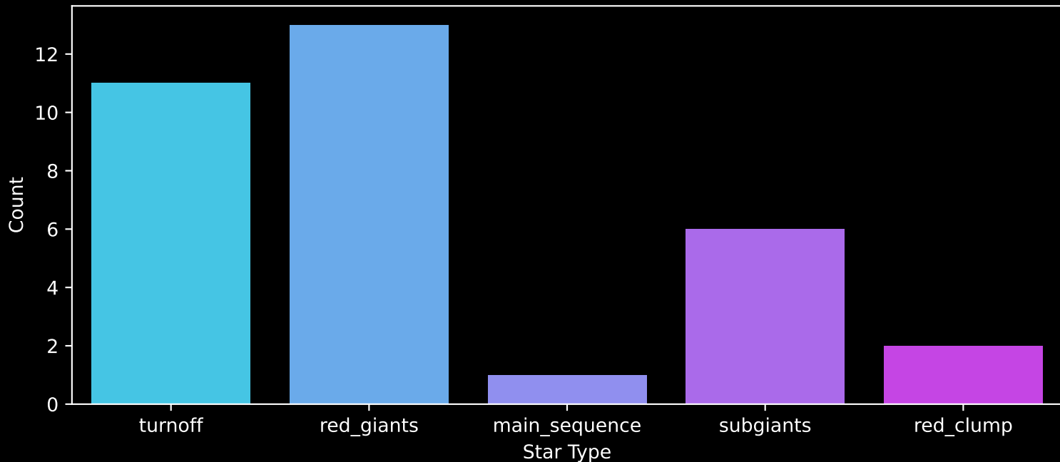
Gaia Cluster: [Patchick_94] Count plot of Star Type
