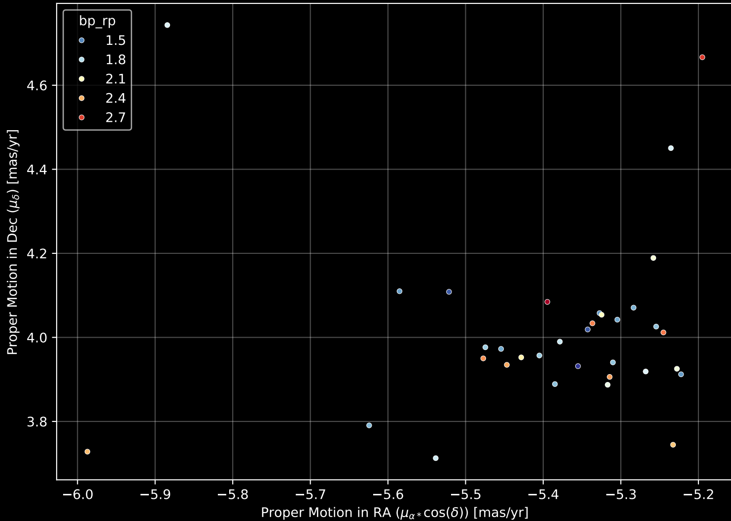
Gaia Cluster: [Pismis_11] Proper Motion Diagram (n= 34)
