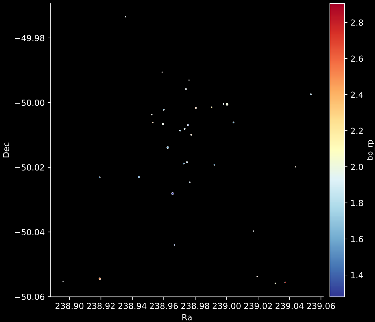
Gaia Cluster: [Pismis_11] Stars: 34
