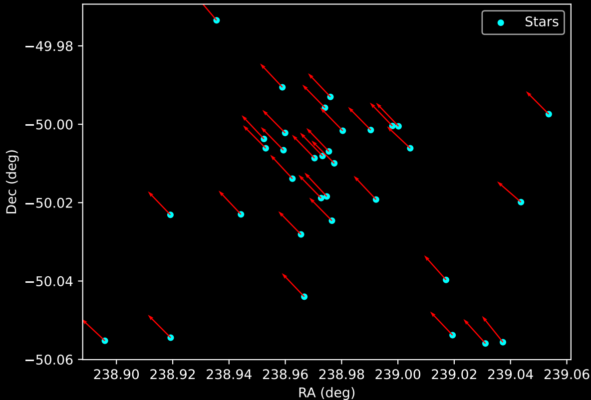
Gaia Cluster: [Pismis_11] Proper Motion Vectors for Gaia Star Field (n= 34)
