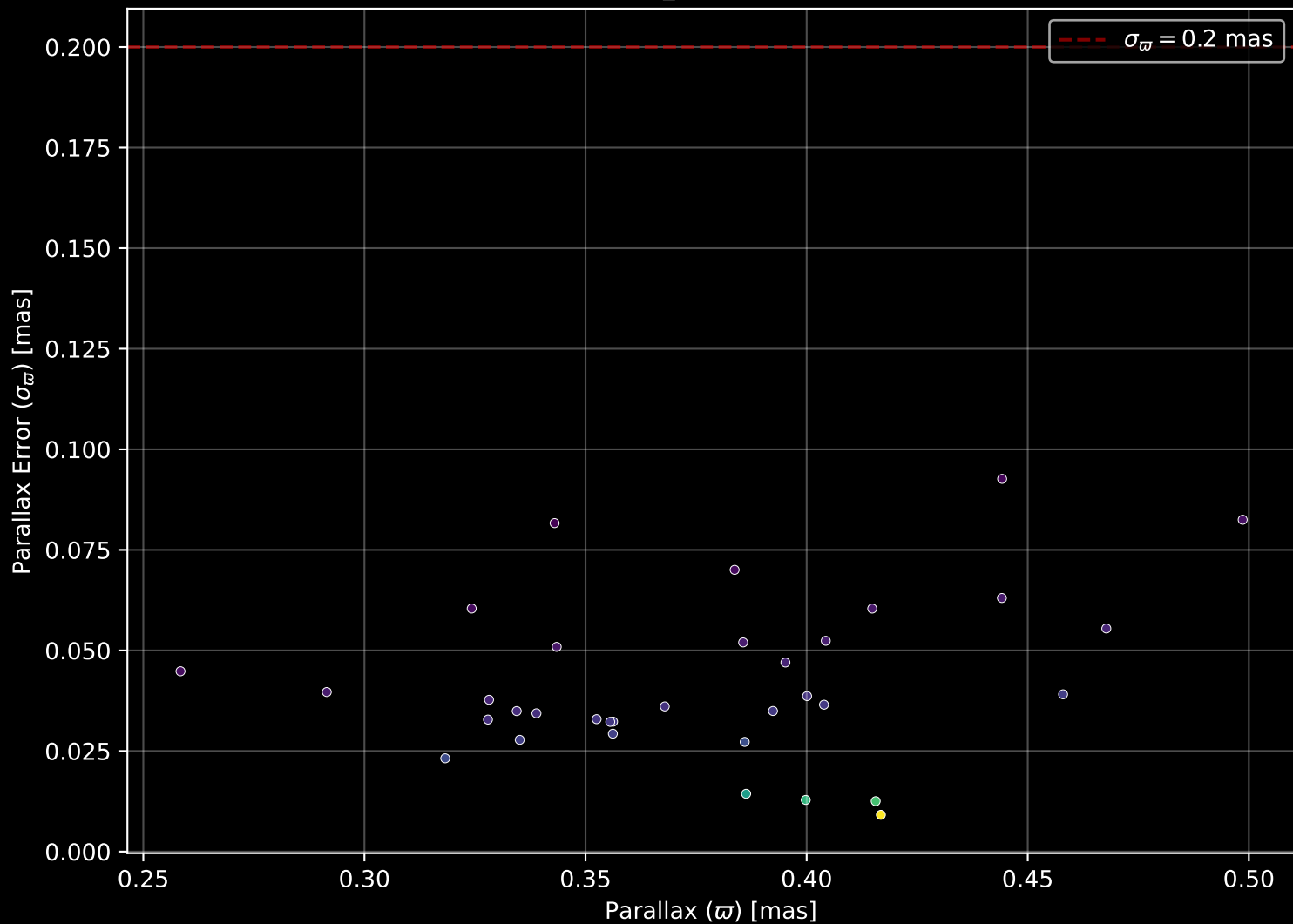
Gaia Cluster: [Pismis_11] Parallax Quality (n= 34)
