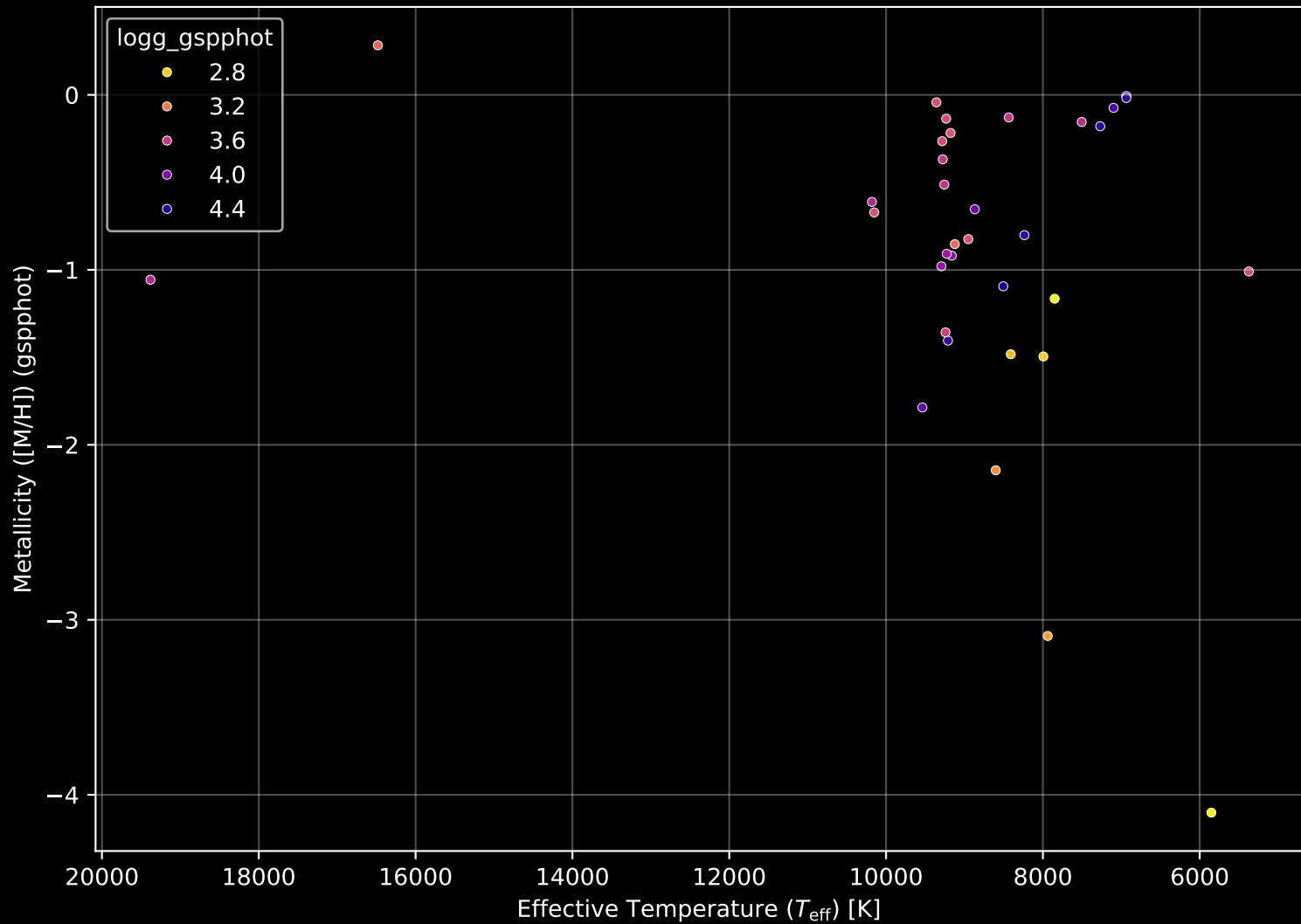
Gaia Cluster: [Pismis_11] Stellar Population Parameters (n= 34)
