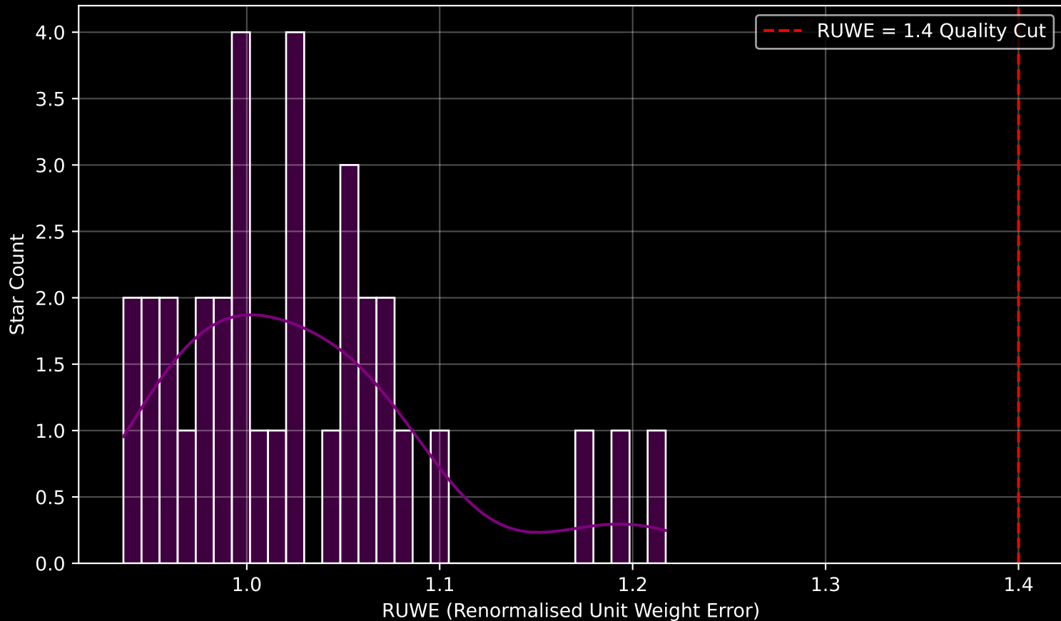
Gaia Cluster: [Pismis_11] RUWE Distribution (n= 34)
