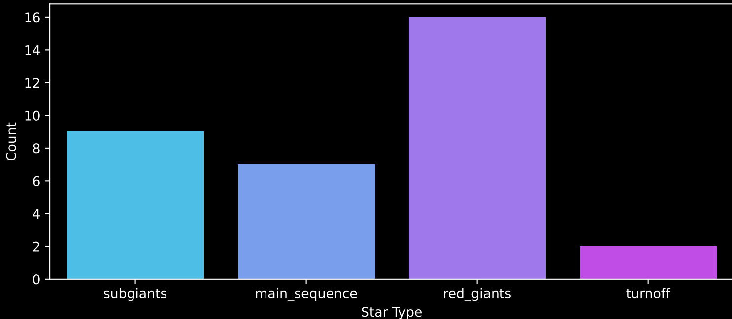
Gaia Cluster: [Pismis_11] Count plot of Star Type
