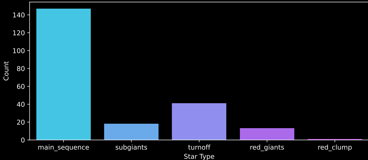
Gaia Cluster: [Pismis_12] Count plot of Star Type
