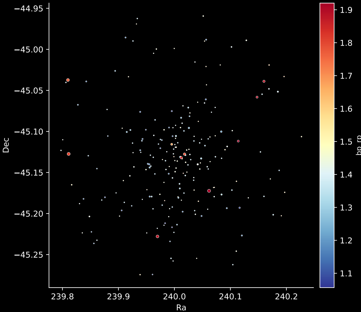
Gaia Cluster: [Pismis_12] Stars: 220
