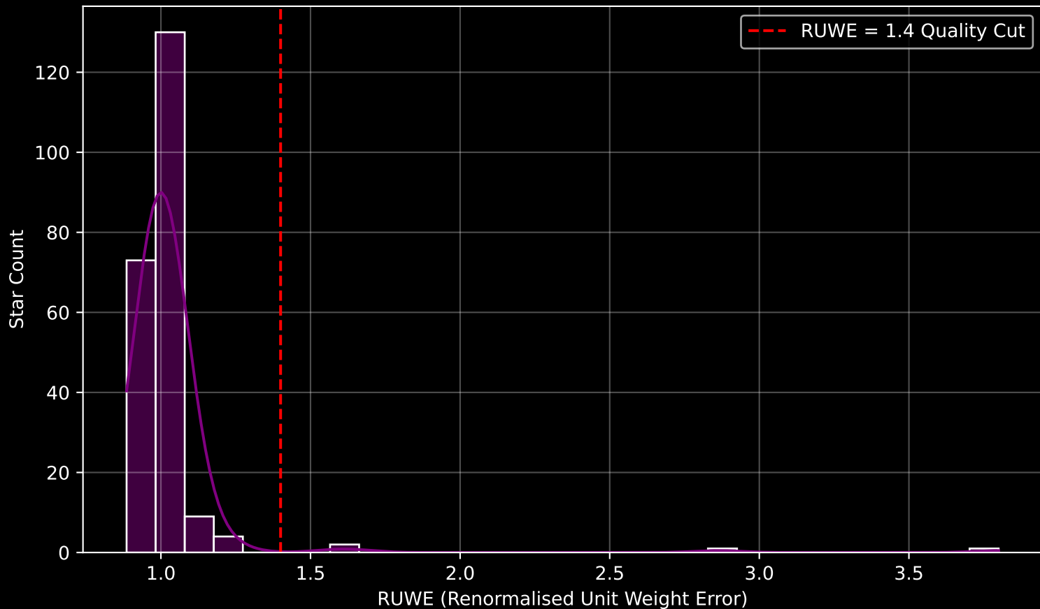
Gaia Cluster: [Pismis_12] RUWE Distribution (n= 220)
