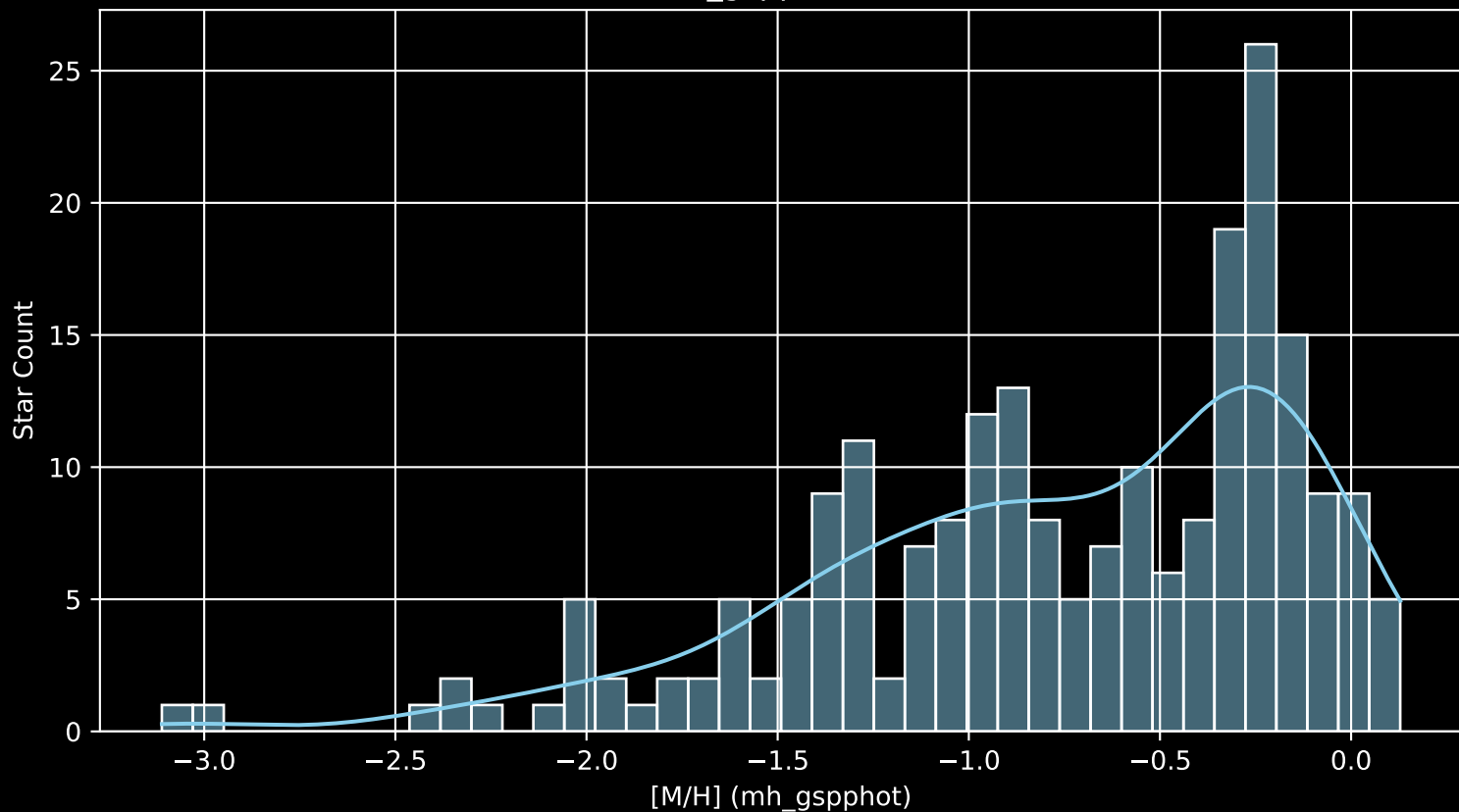
Gaia Cluster: [Pismis_12 [M/H] (mh_gspphot) (n= 220)
