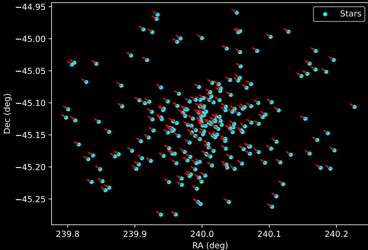
Gaia Cluster: [Pismis_12] Proper Motion Vectors for Gaia Star Field (n= 220)
