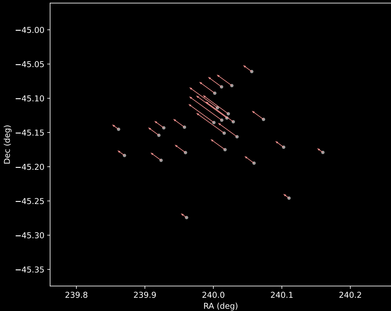
Gaia DR3 Cluster 7 Proper Motion Vectors (n=26)
