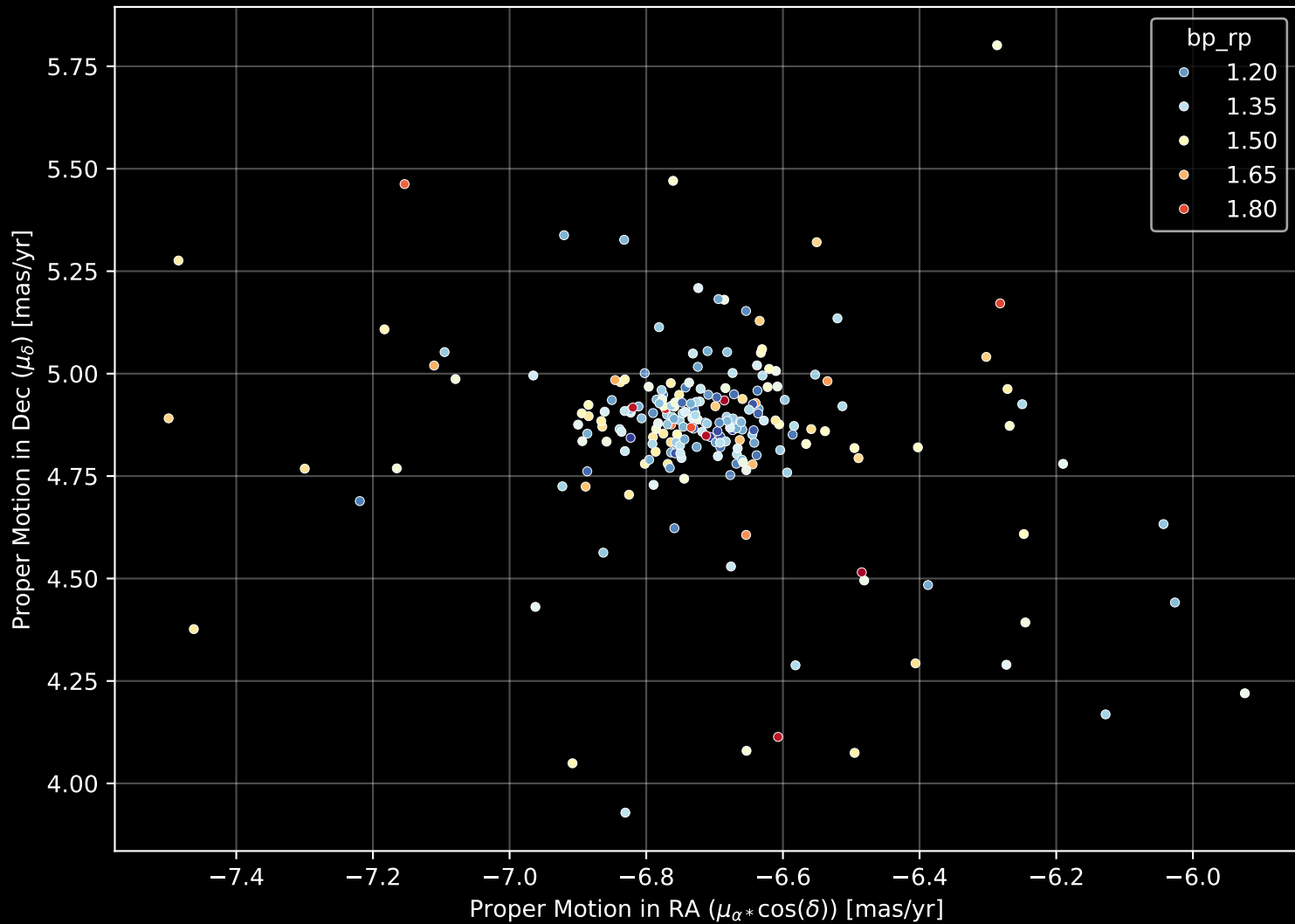
Gaia Cluster: [Pismis_12] Proper Motion Diagram (n= 220)
