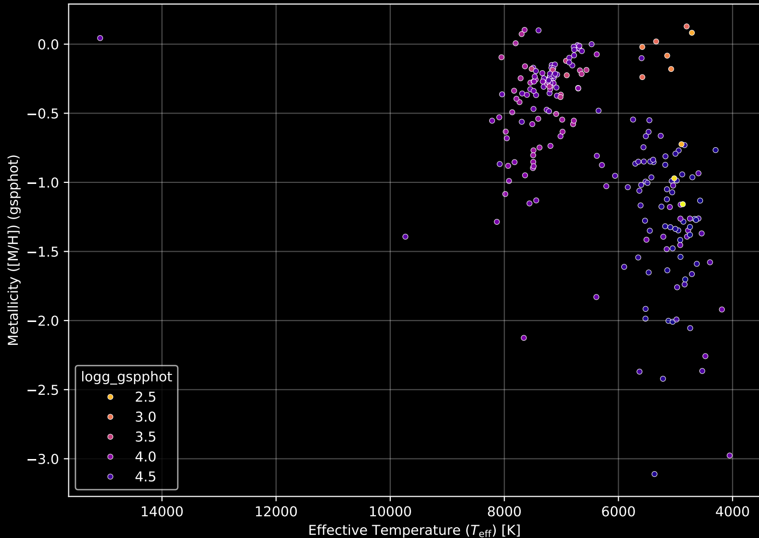
Gaia Cluster: [Pismis_12] Stellar Population Parameters (n= 220)
