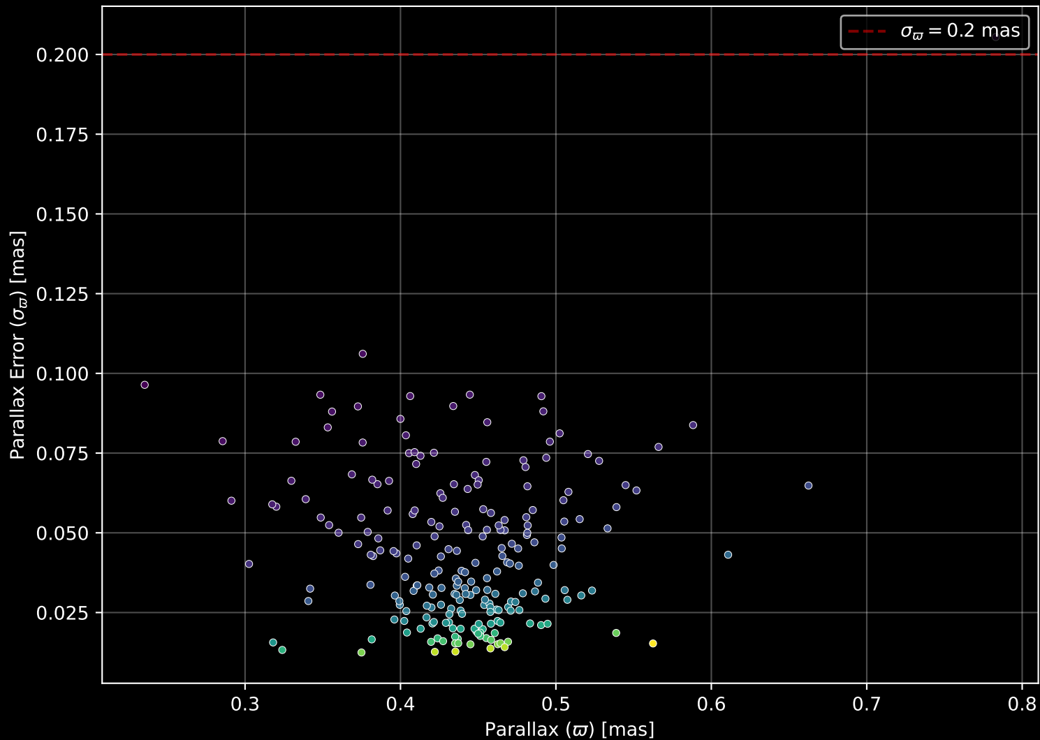
Gaia Cluster: [Pismis_12] Parallax Quality (n= 220)
