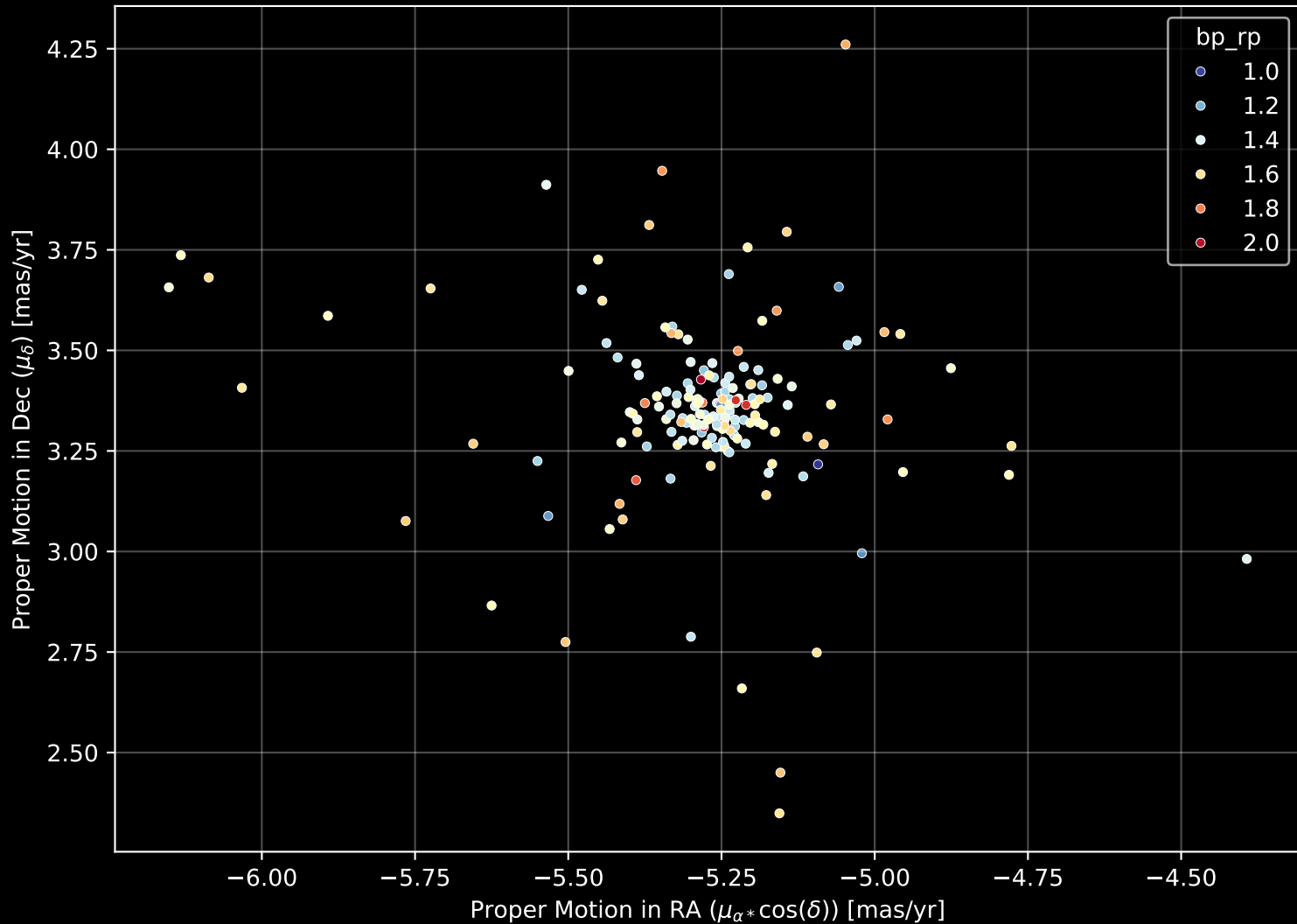
Gaia Cluster: [Pismis_15] Proper Motion Diagram (n= 174)
