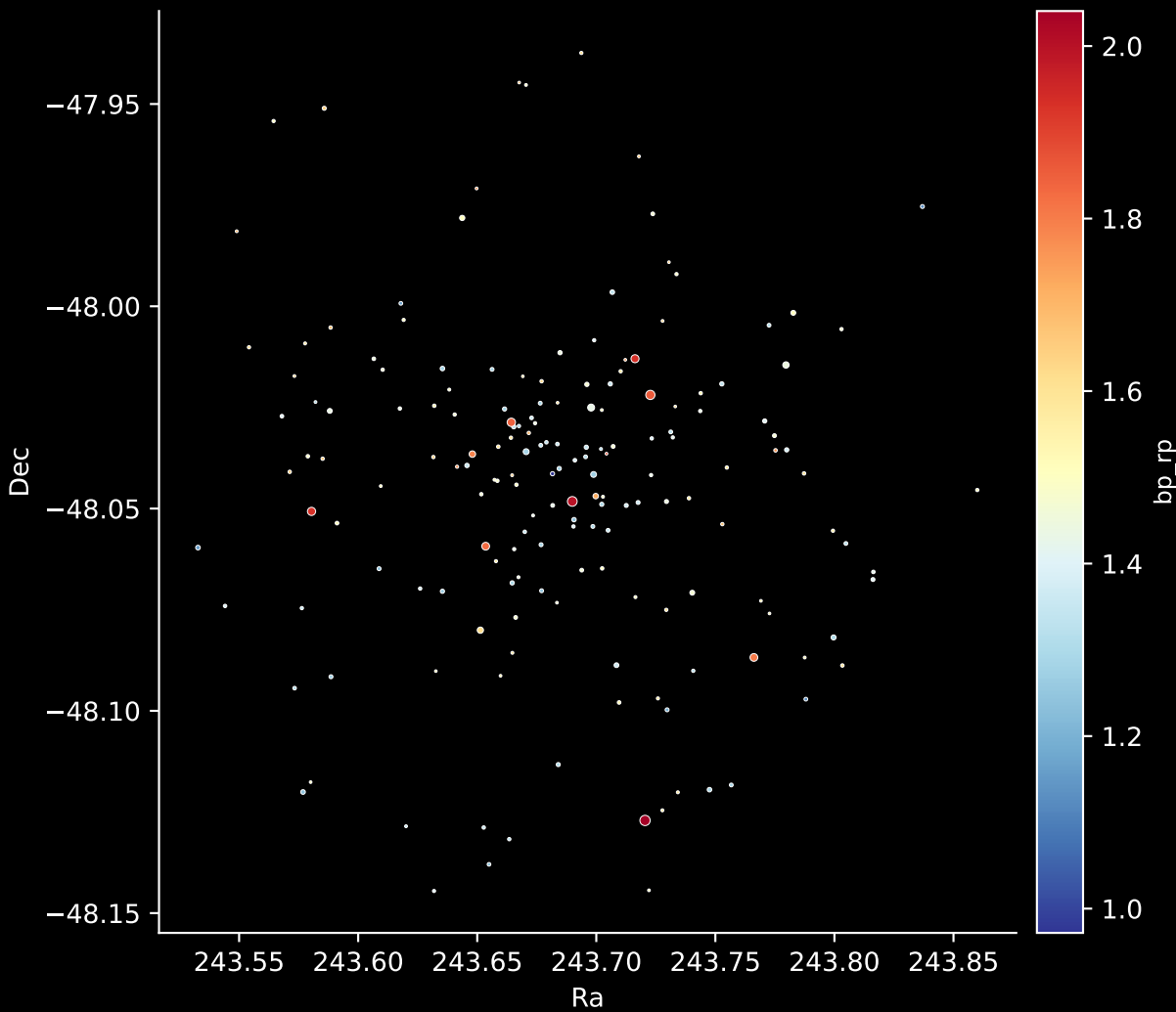
Gaia Cluster: [Pismis_15] Stars: 174
