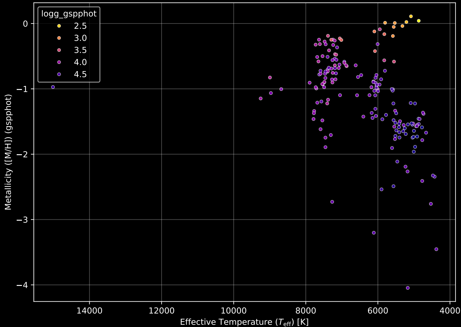
Gaia Cluster: [Pismis_15] Stellar Population Parameters (n= 174)
