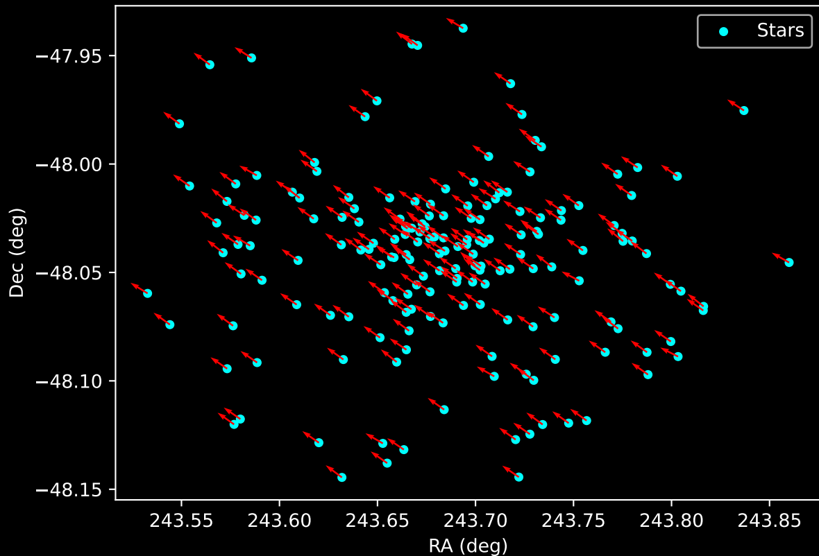
Gaia Cluster: [Pismis_15] Proper Motion Vectors for Gaia Star Field (n= 174)
