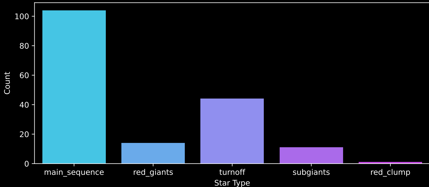
Gaia Cluster: [Pismis_15] Count plot of Star Type
