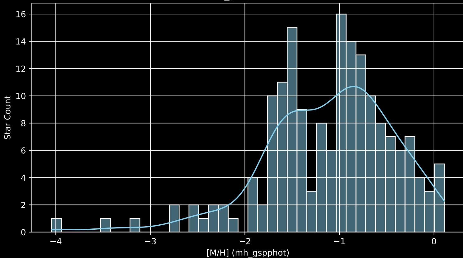
Gaia Cluster: [Pismis_15 [M/H] (mh_gspphot) (n= 174)
