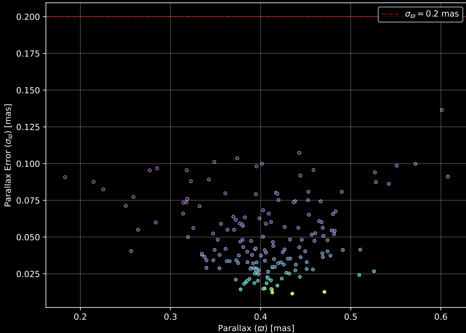
Gaia Cluster: [Pismis_15] Parallax Quality (n= 174)
