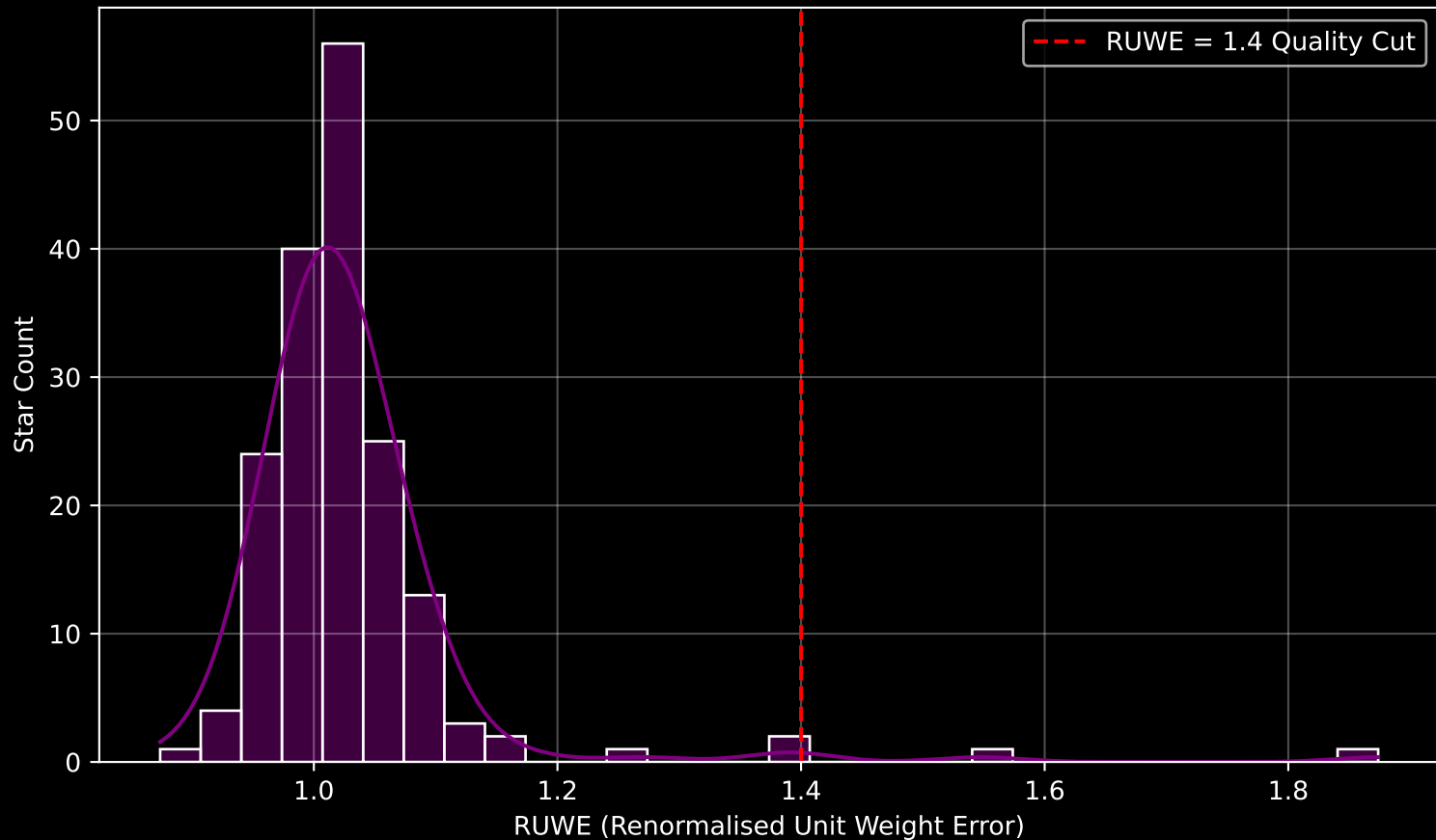
Gaia Cluster: [Pismis_15] RUWE Distribution (n= 173)
