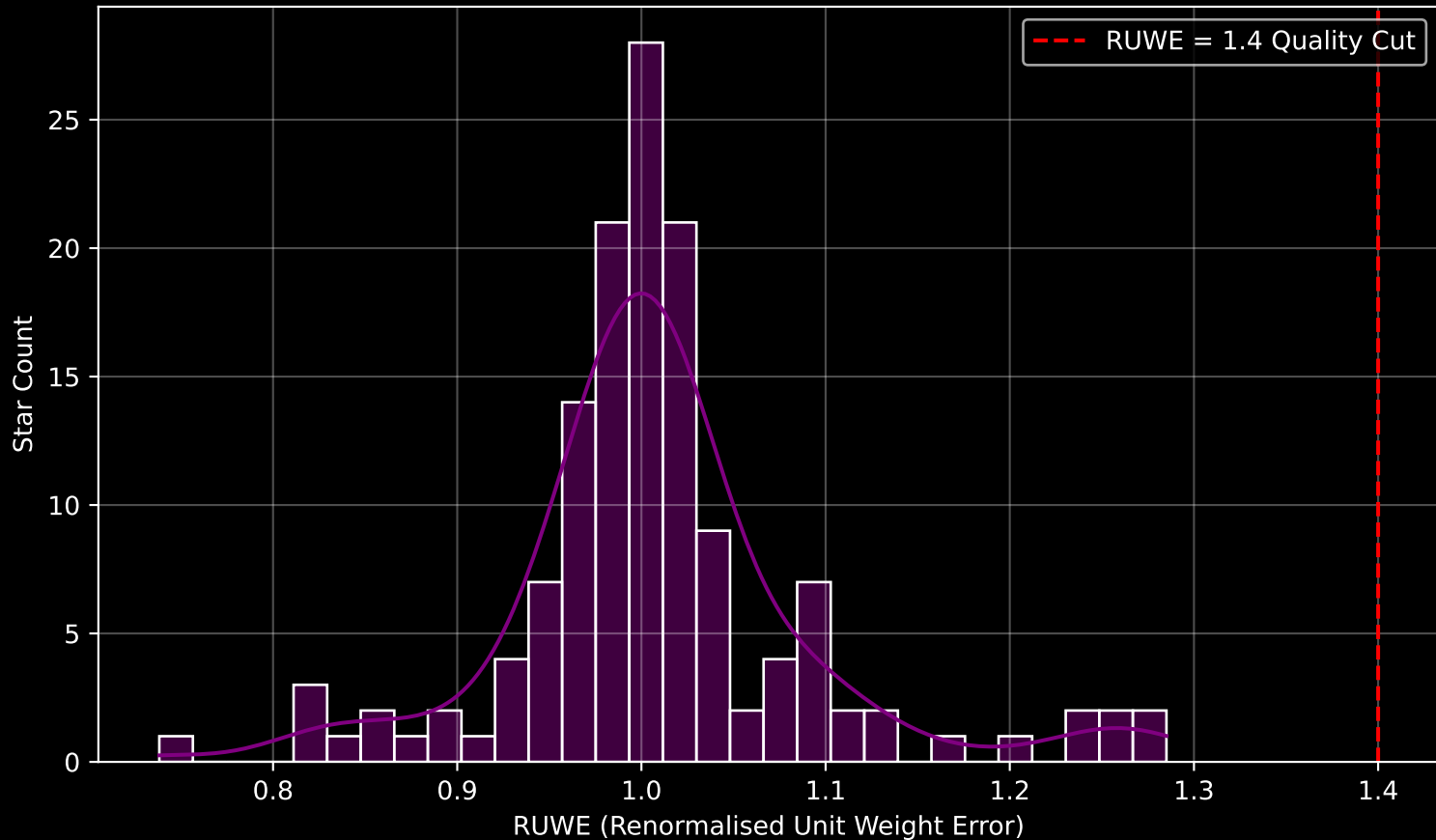
Gaia Cluster: [Pismis_17] RUWE Distribution (n= 140)
