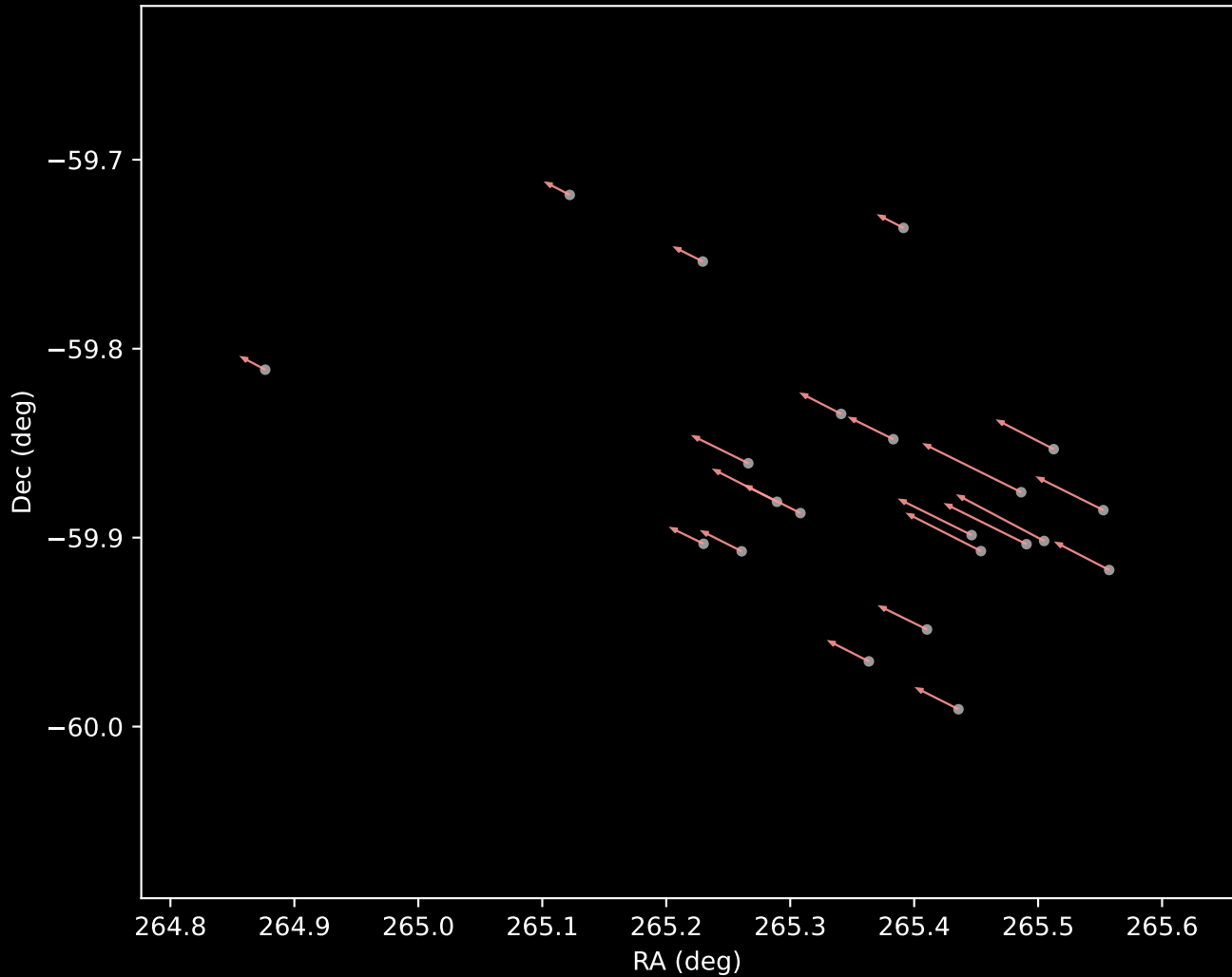
Gaia DR3 Cluster 7 Proper Motion Vectors (n=22)
