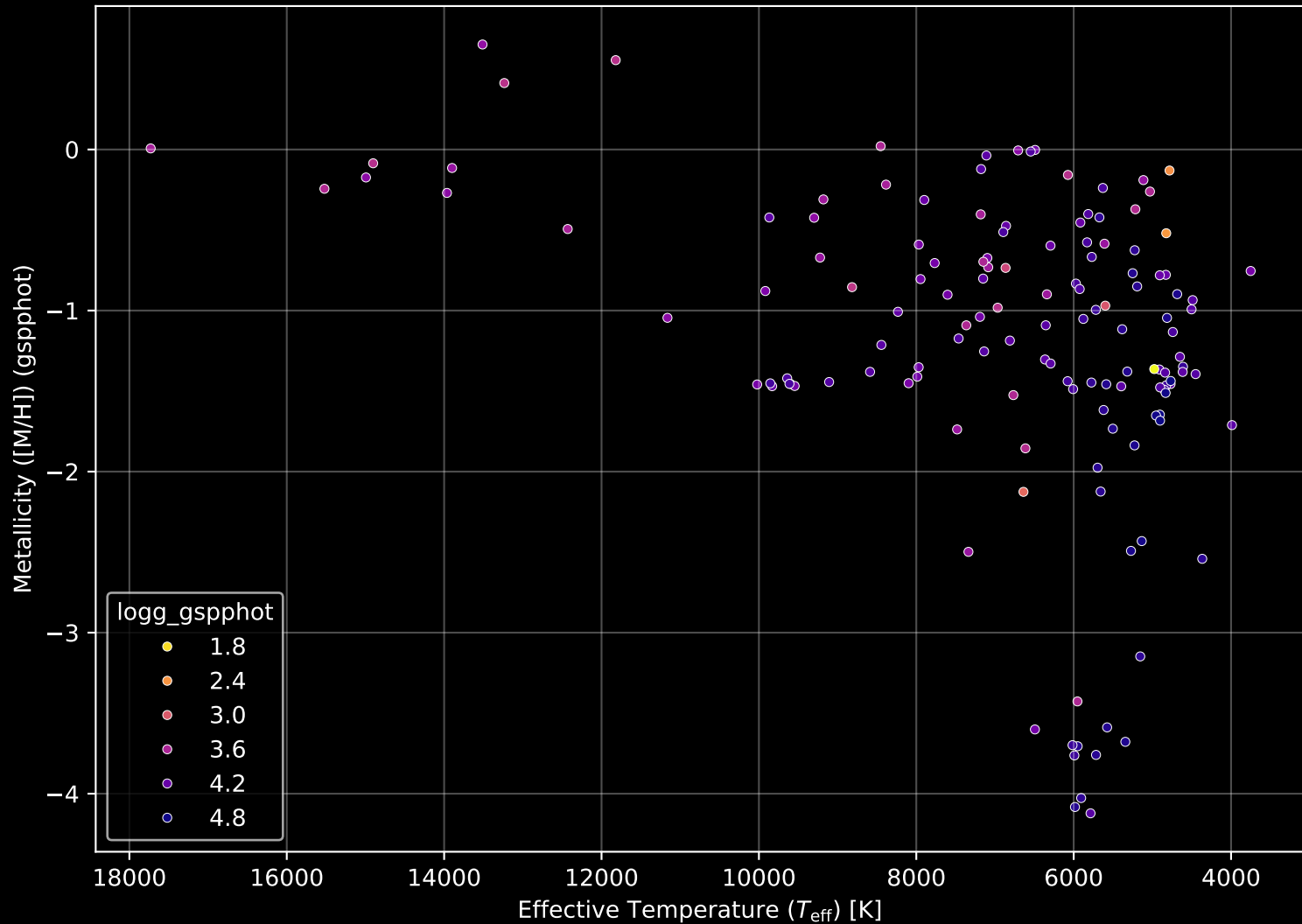
Gaia Cluster: [Pismis_17] Stellar Population Parameters (n= 140)
