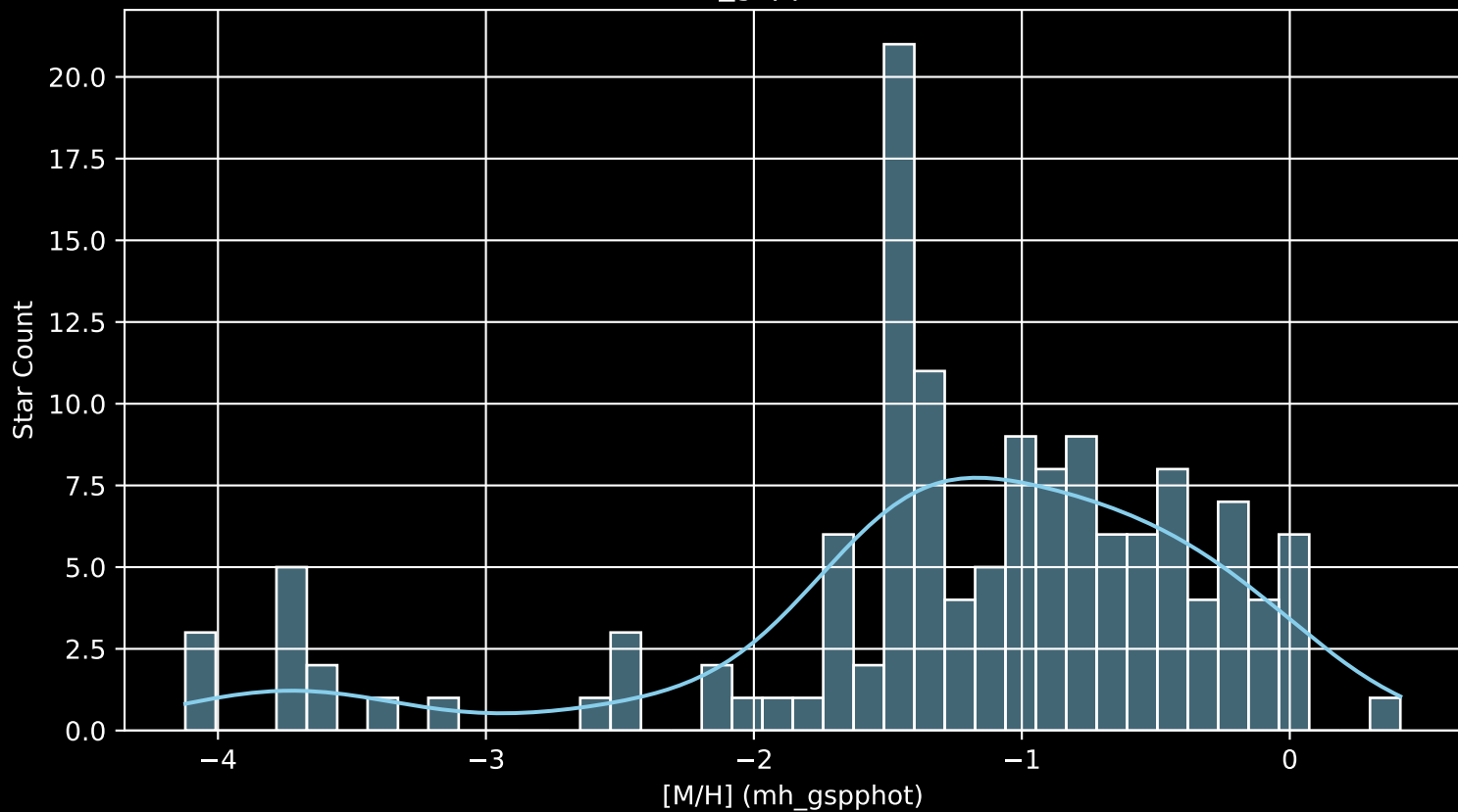
Gaia Cluster: [Pismis_17 [M/H] (mh_gspphot) (n= 138)
