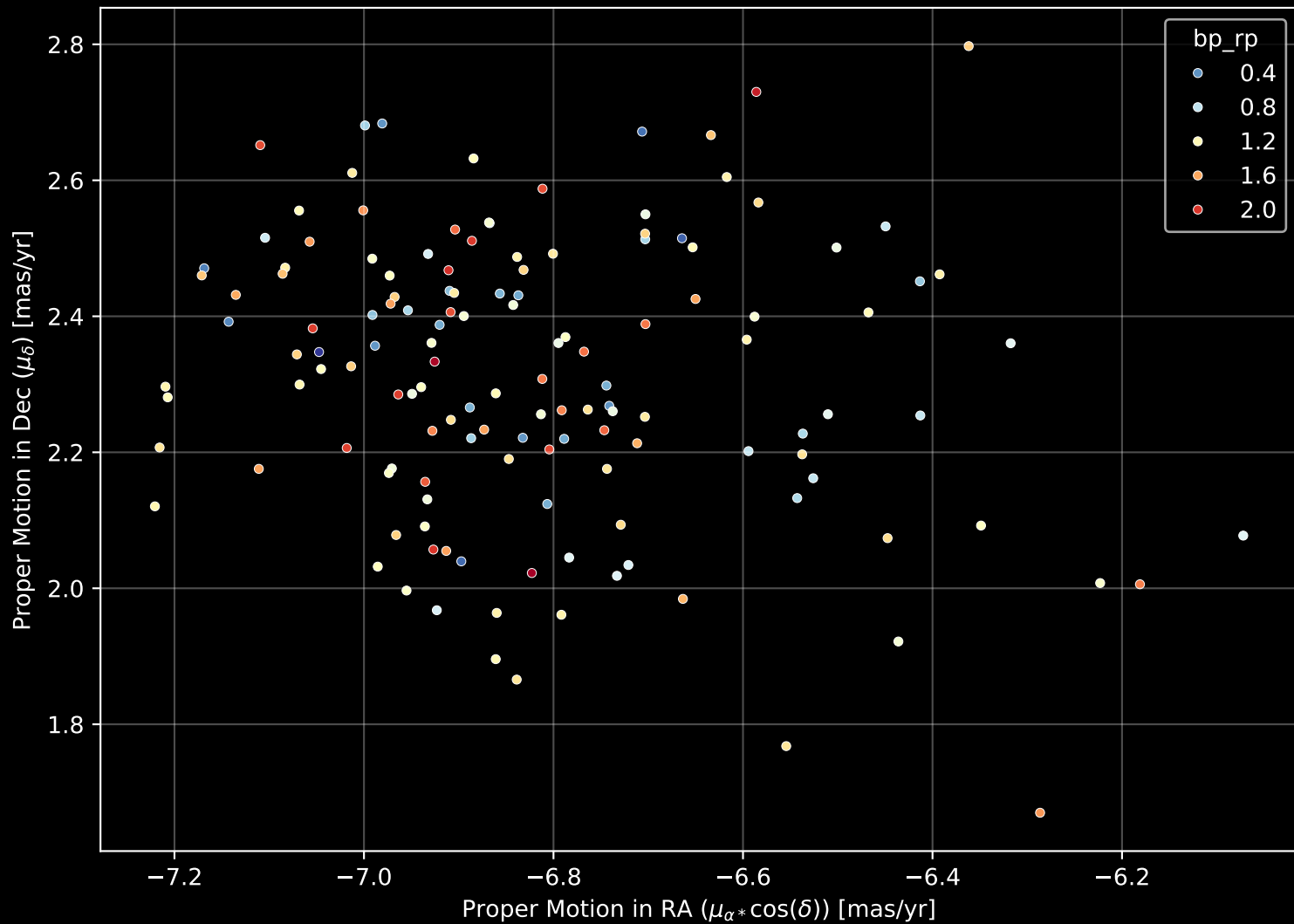
Gaia Cluster: [Pismis_17] Proper Motion Diagram (n= 140)
