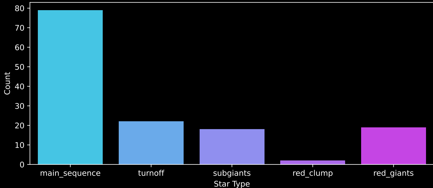
Gaia Cluster: [Pismis_17] Count plot of Star Type
