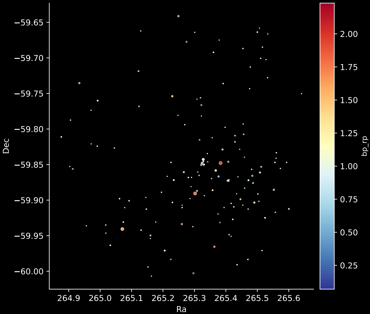
Gaia Cluster: [Pismis_17] Stars: 140
