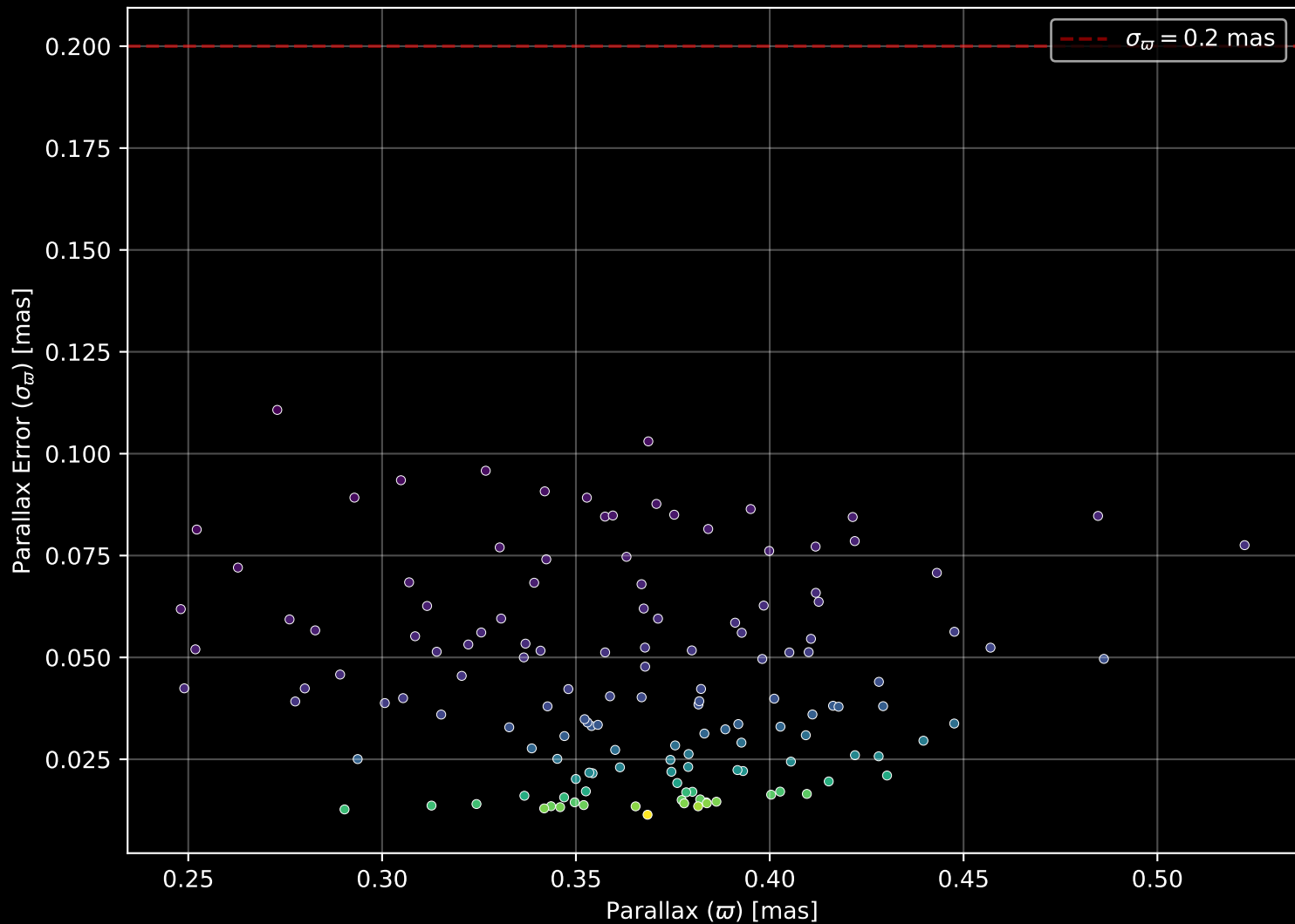
Gaia Cluster: [Pismis_17] Parallax Quality (n= 140)
