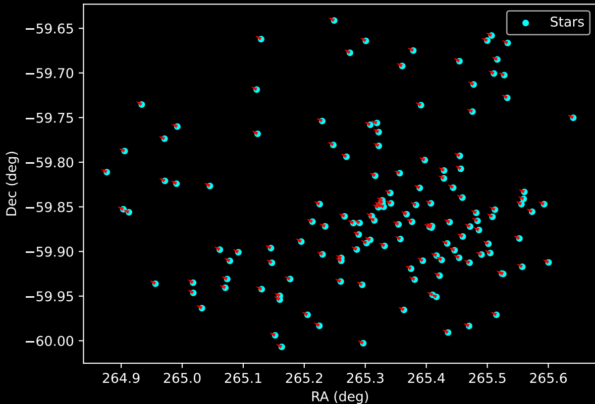
Gaia Cluster: [Pismis_17] Proper Motion Vectors for Gaia Star Field (n= 140)
