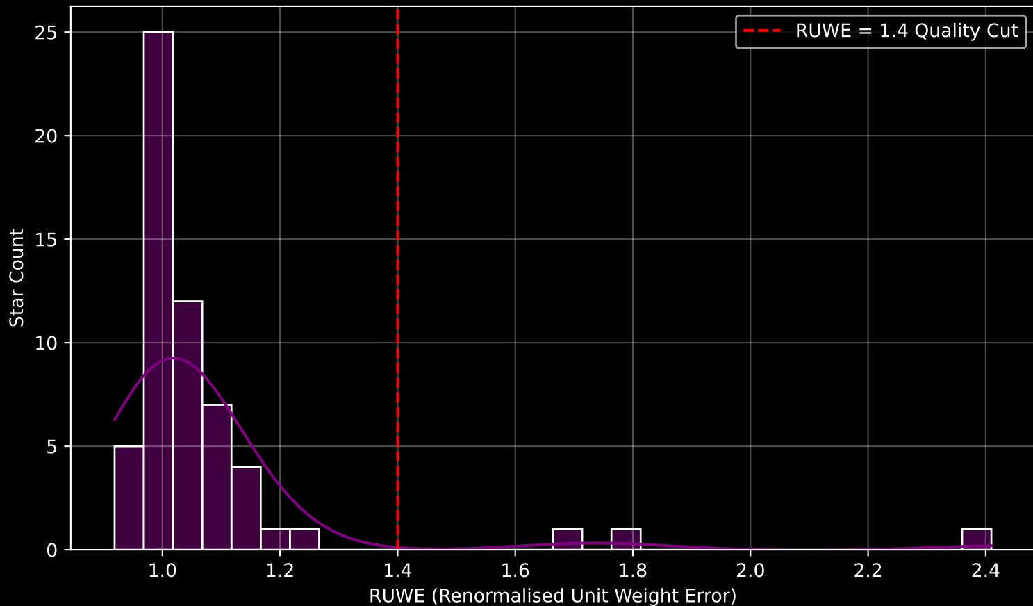
Gaia Cluster: [Pismis_23] RUWE Distribution (n= 58)
