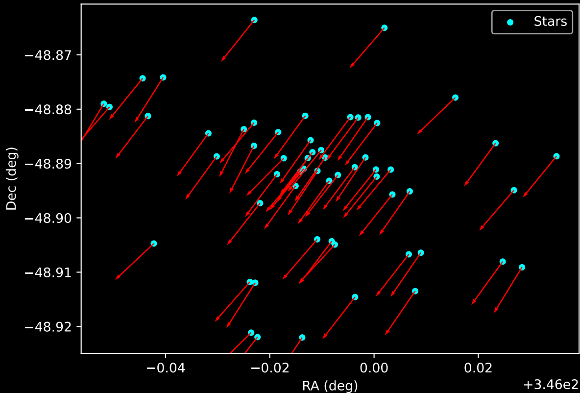
Gaia Cluster: [Pismis_23] Proper Motion Vectors for Gaia Star Field (n= 58)
