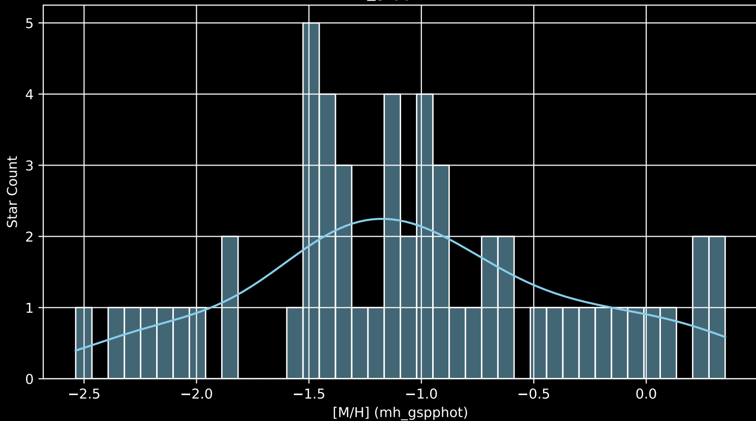
Gaia Cluster: [Pismis_23 [M/H] (mh_gspphot) (n= 56)
