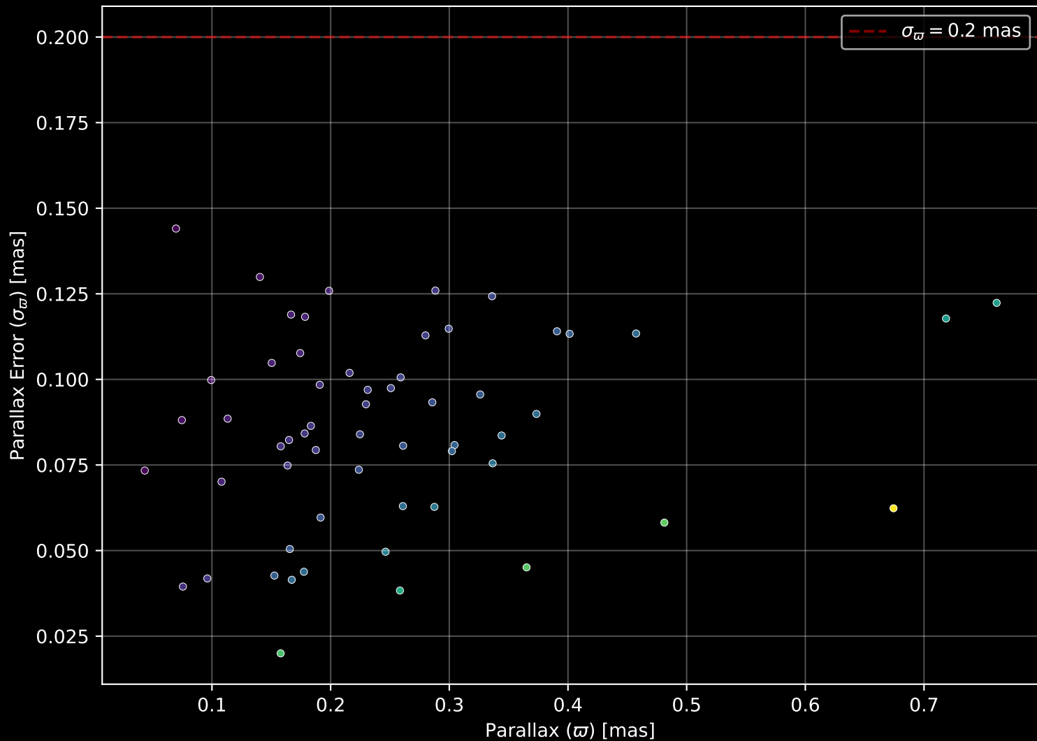
Gaia Cluster: [Pismis_23] Parallax Quality (n= 58)
