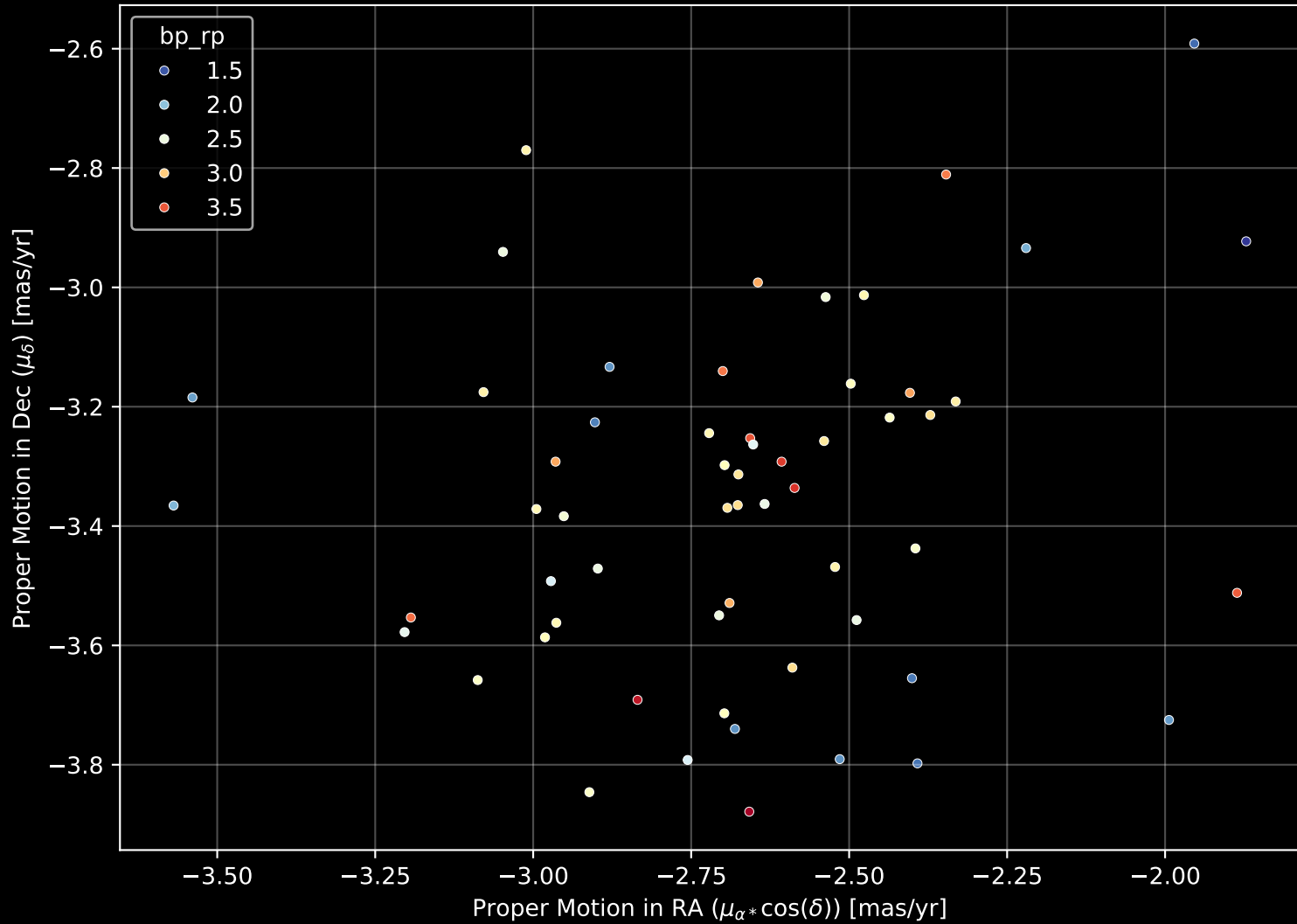
Gaia Cluster: [Pismis_23] Proper Motion Diagram (n= 58)
