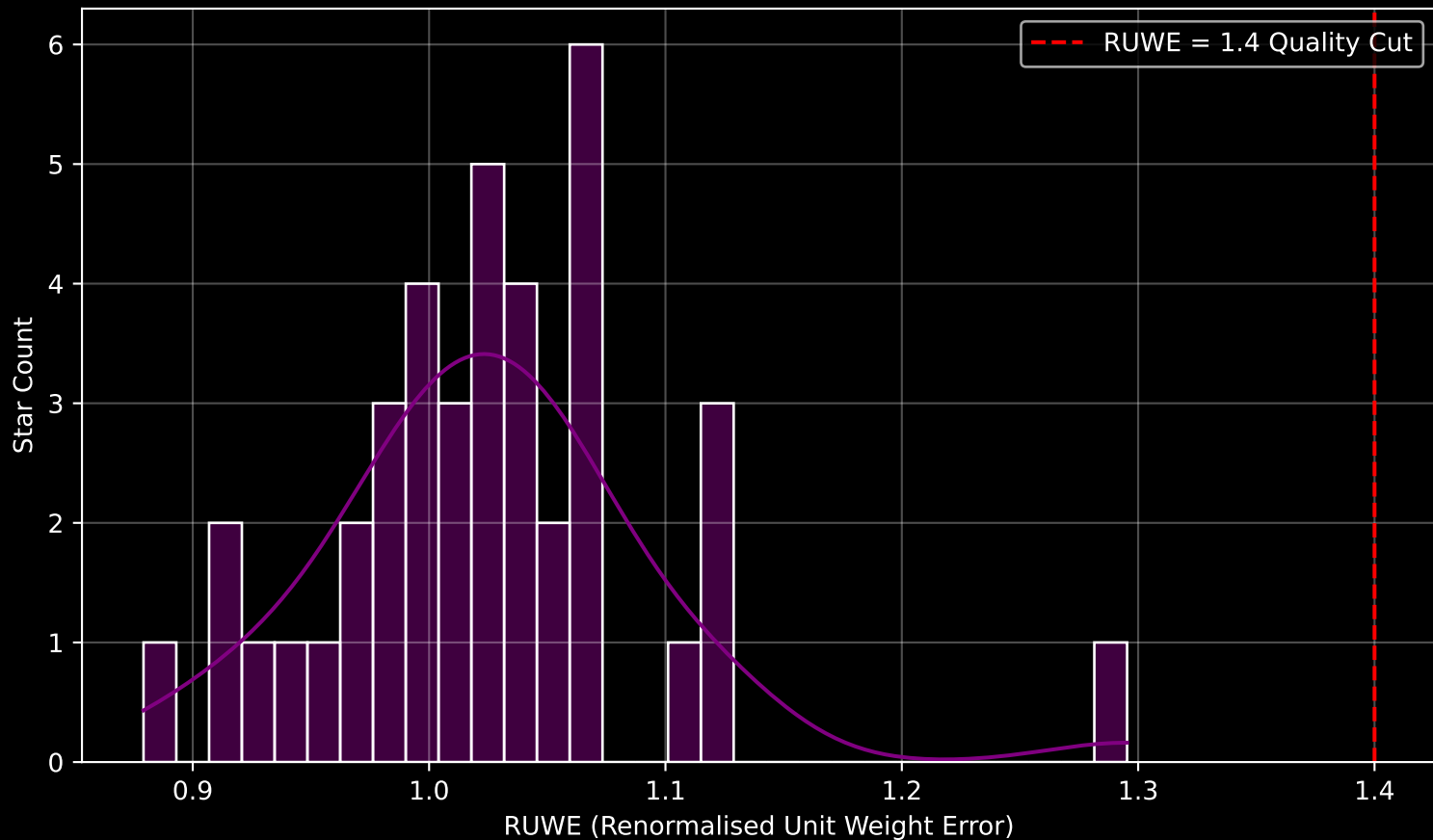
Gaia Cluster: [Pismis_27] RUWE Distribution (n= 40)
