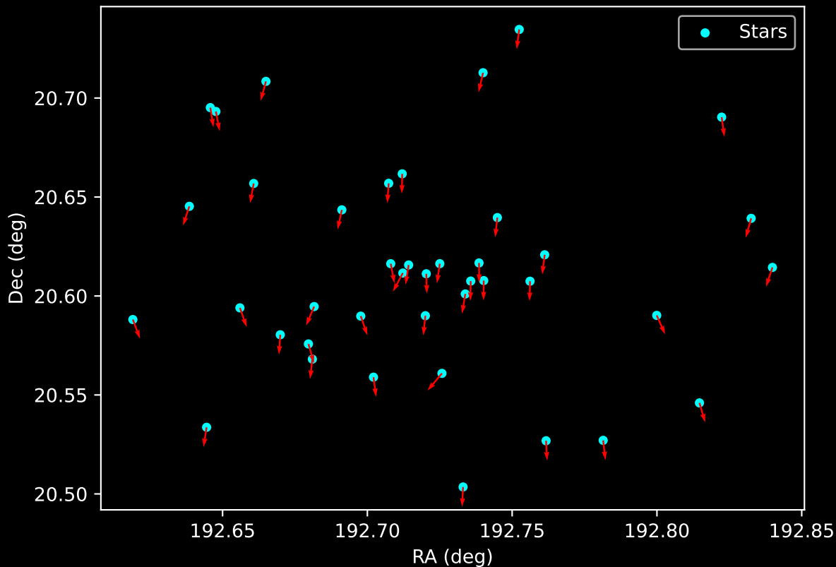
Gaia Cluster: [Pismis_27] Proper Motion Vectors for Gaia Star Field (n= 41)
