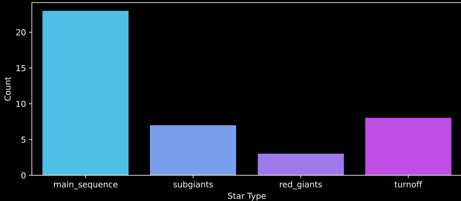
Gaia Cluster: [Pismis_27] Count plot of Star Type
