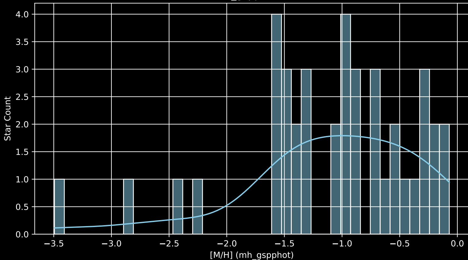
Gaia Cluster: [Pismis_27 [M/H] (mh_gspphot) (n= 40)
