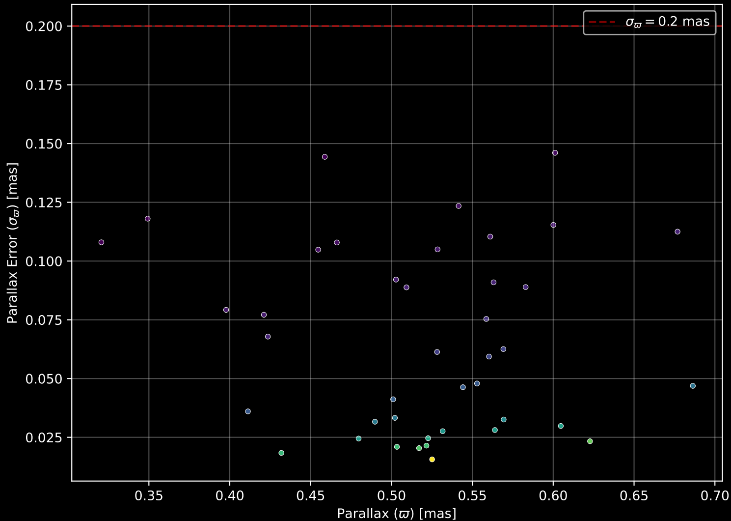
Gaia Cluster: [Pismis_27] Parallax Quality (n= 41)
