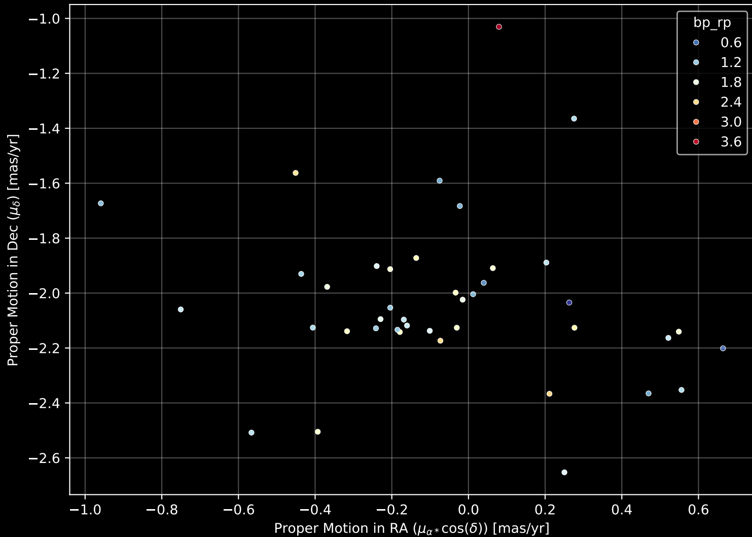
Gaia Cluster: [Pismis 27] Proper Motion Diagram (n= 41)
