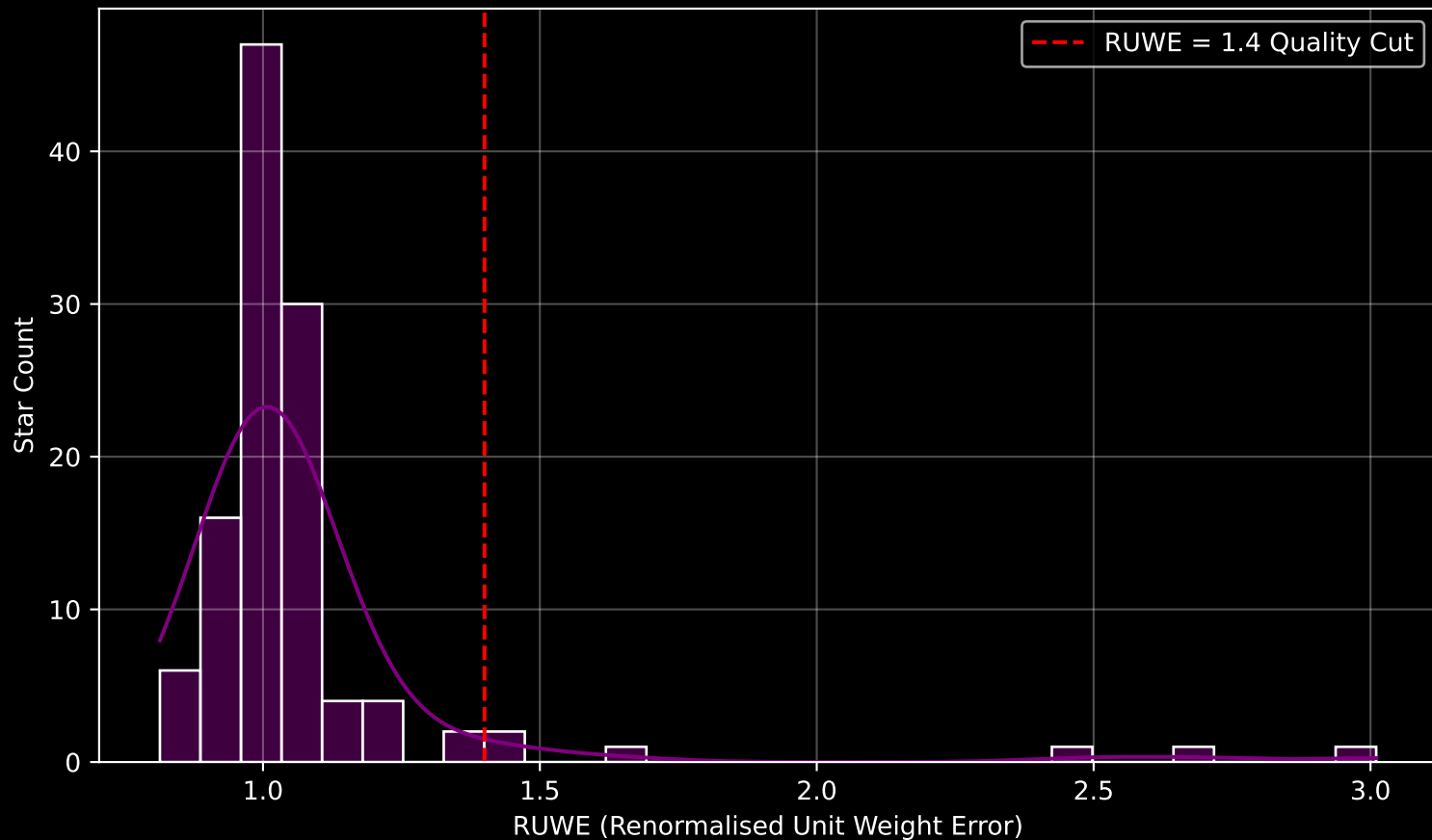
Gaia Cluster: [Pismis_4] RUWE Distribution (n= 115)
