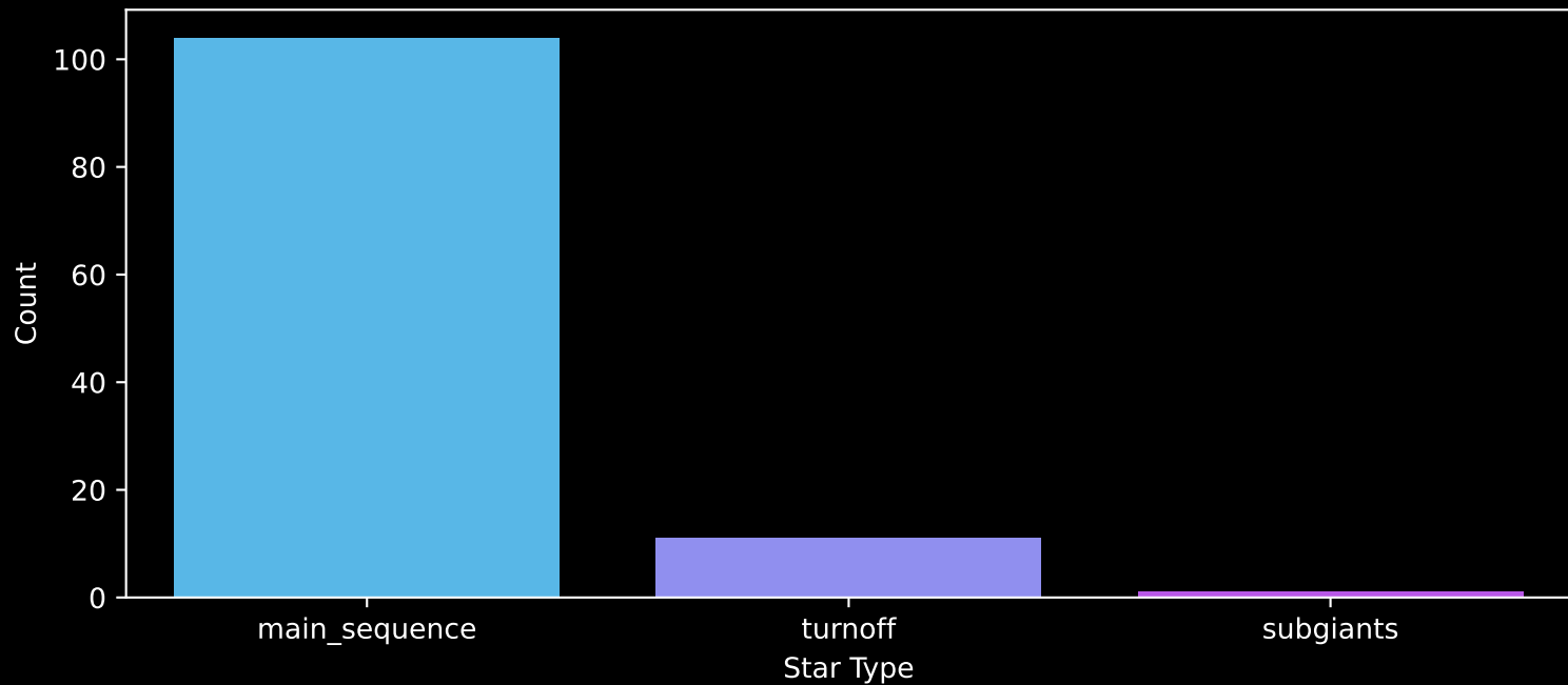
Gaia Cluster: [Pismis_4] Count plot of Star Type
