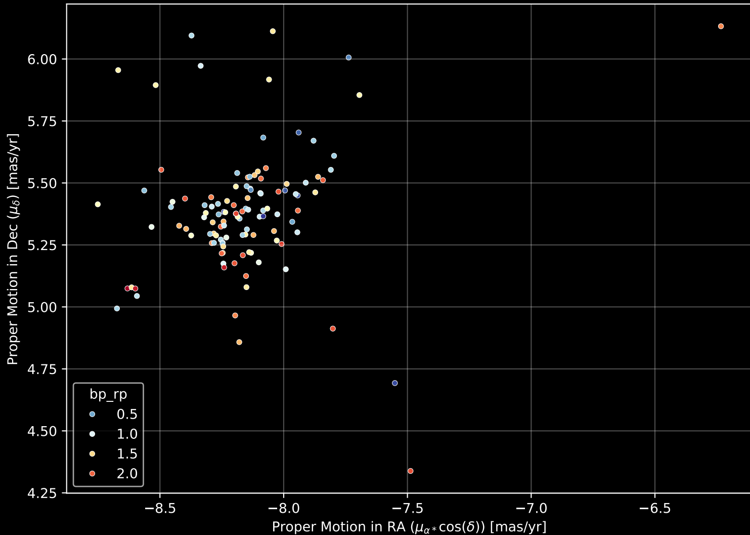
Gaia Cluster: [Pismis_4] Proper Motion Diagram (n= 116)
