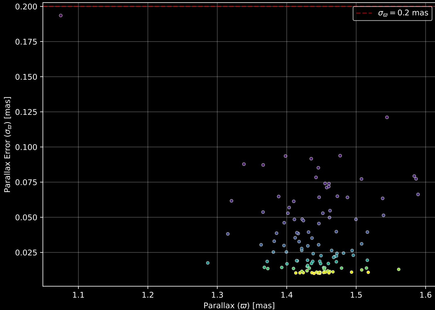
Gaia Cluster: [Pismis_4] Parallax Quality (n= 116)
