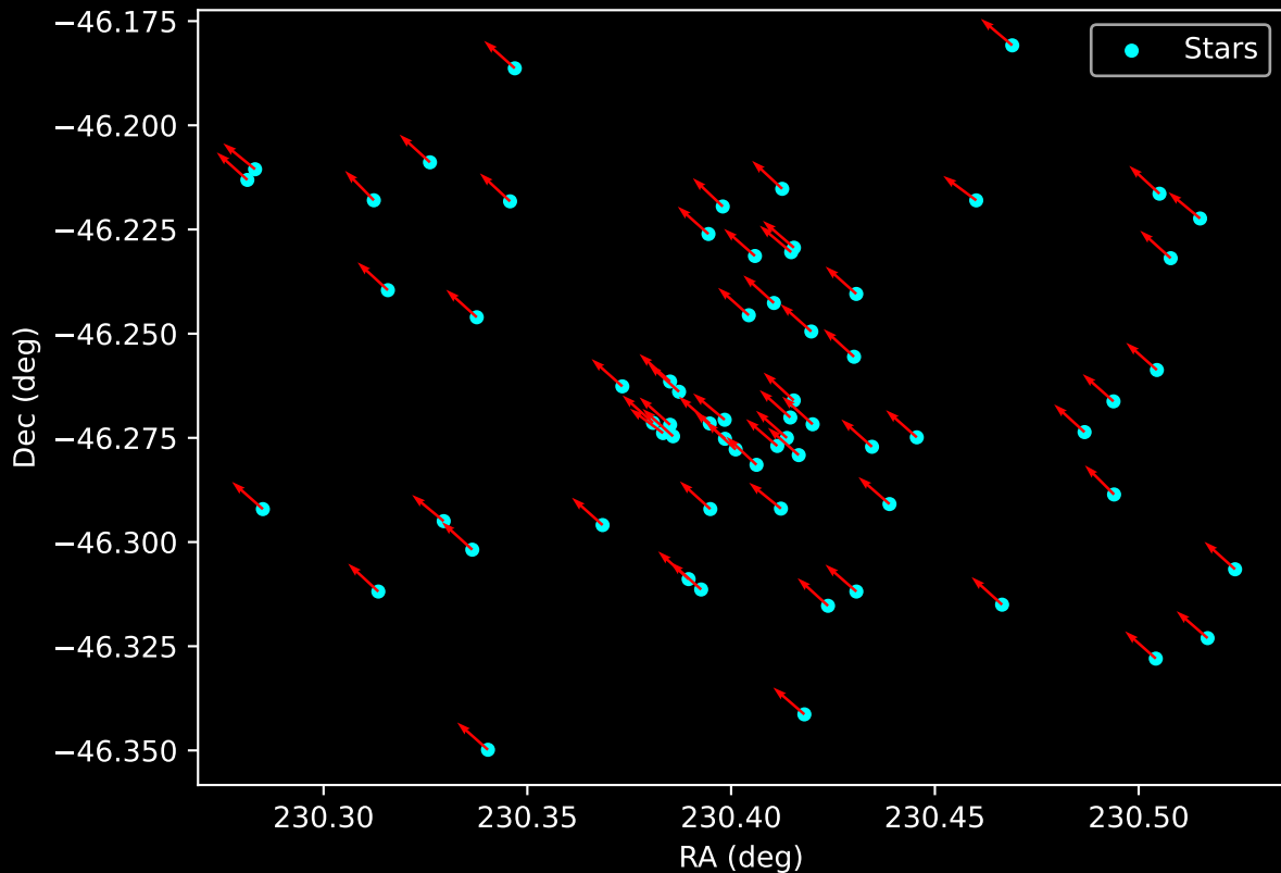
Gaia Cluster: [Pismis_8] Proper Motion Vectors for Gaia Star Field (n= 66)
