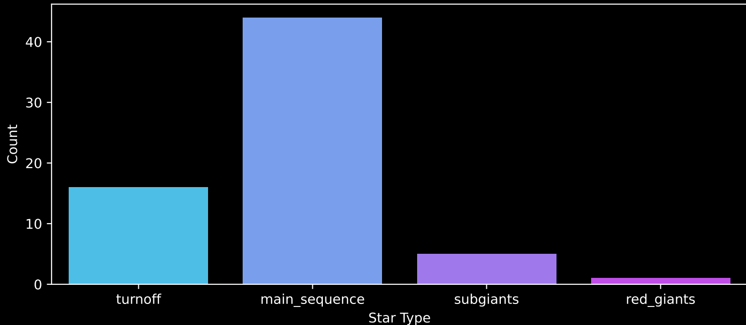
Gaia Cluster: [Pismis_8] Count plot of Star Type
