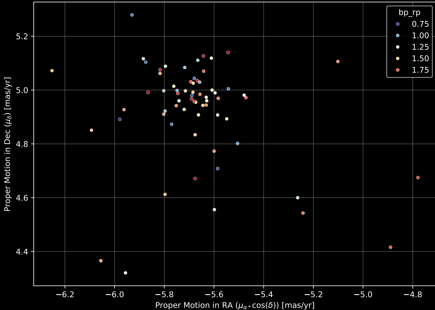
Gaia Cluster: [Pismis_8] Proper Motion Diagram (n= 66)
