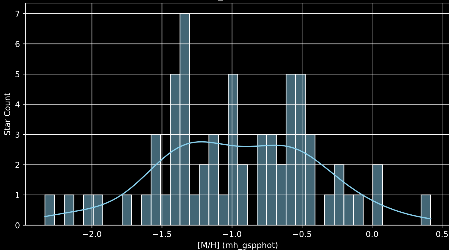
Gaia Cluster: [Pismis_8 [M/H] (mh_gspphot) (n= 65)
