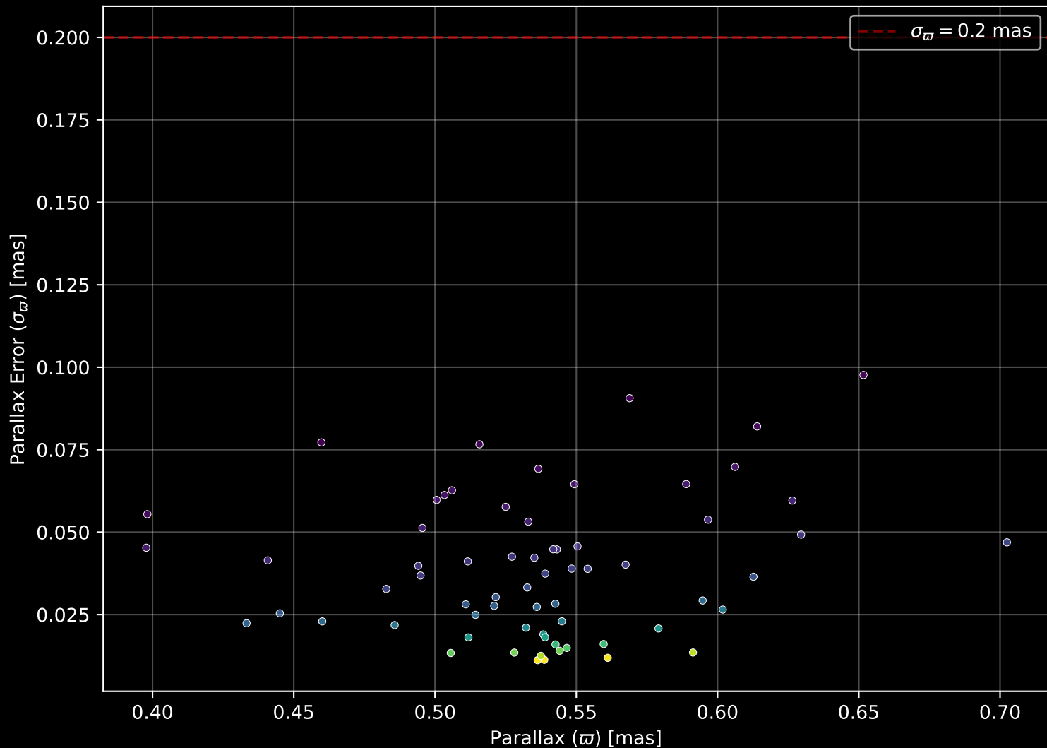
Gaia Cluster: [Pismis_8] Parallax Quality (n= 66)
