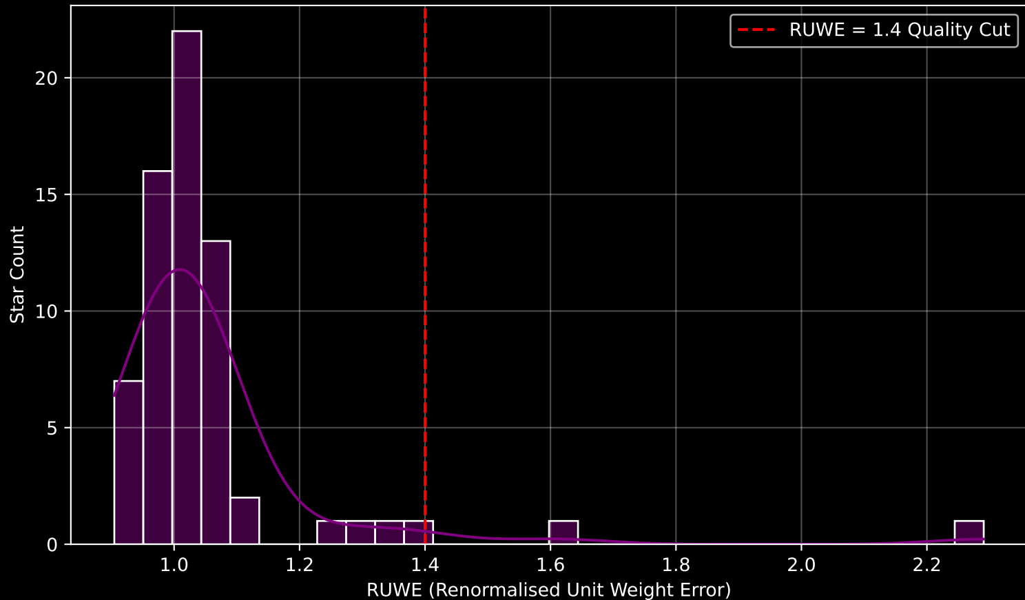
Gaia Cluster: [Pismis_8] RUWE Distribution (n= 66)
