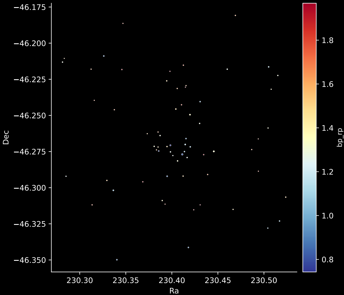
Gaia Cluster: [Pismis_8] Stars: 66
