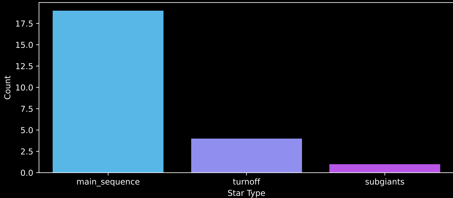
Gaia Cluster: [Platais_10] Count plot of Star Type
