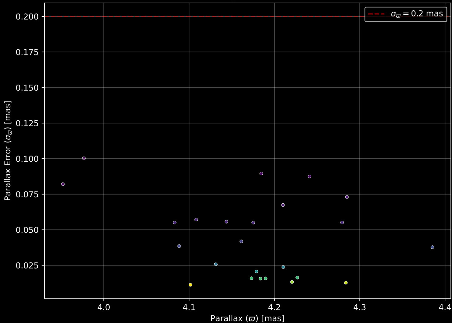
Gaia Cluster: [Platais_10] Parallax Quality (n= 24)
