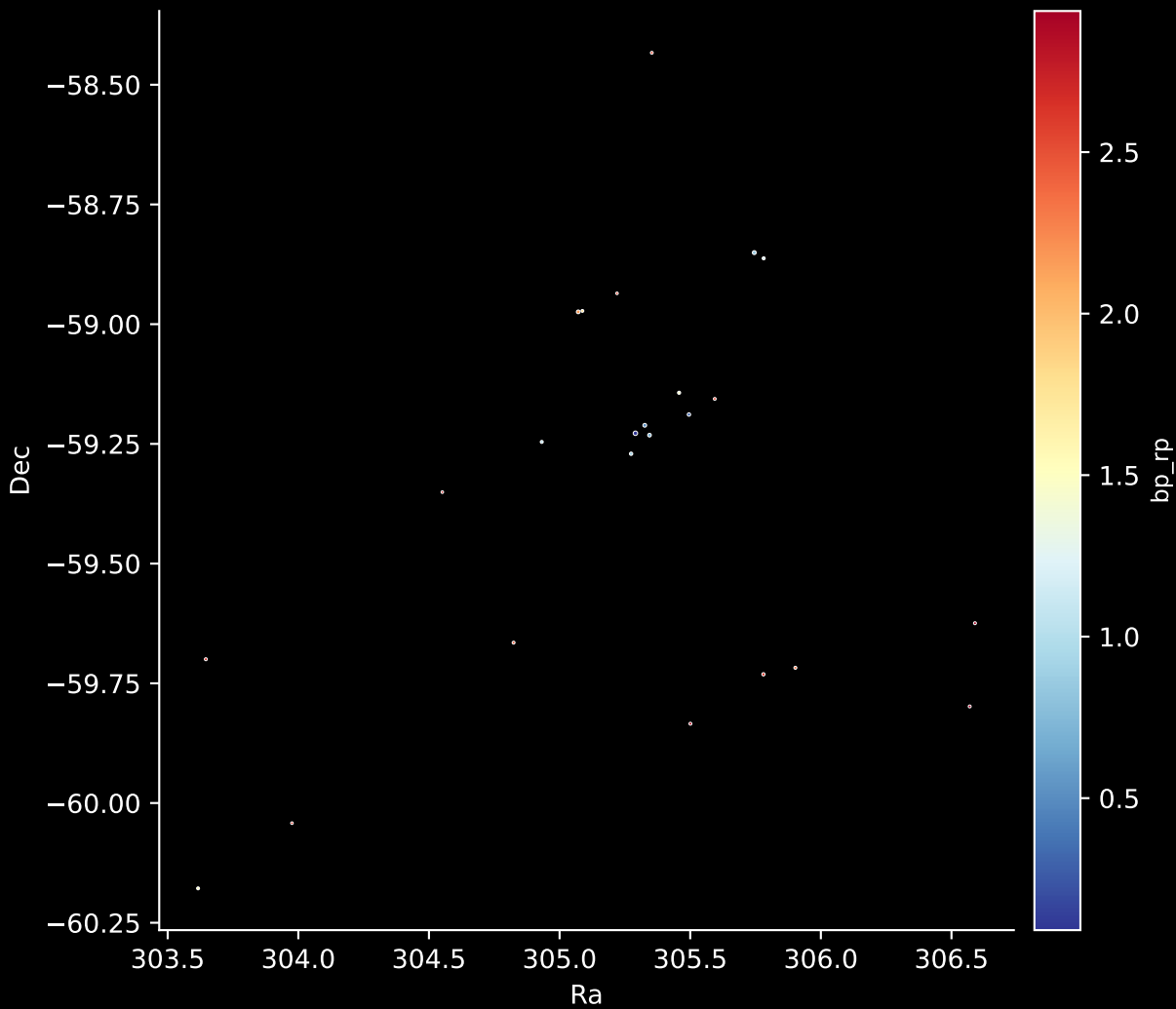
Gaia Cluster: [Platais_10] Stars: 24
