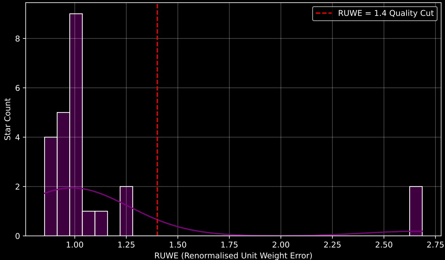
Gaia Cluster: [Platais_10] RUWE Distribution (n= 24)
