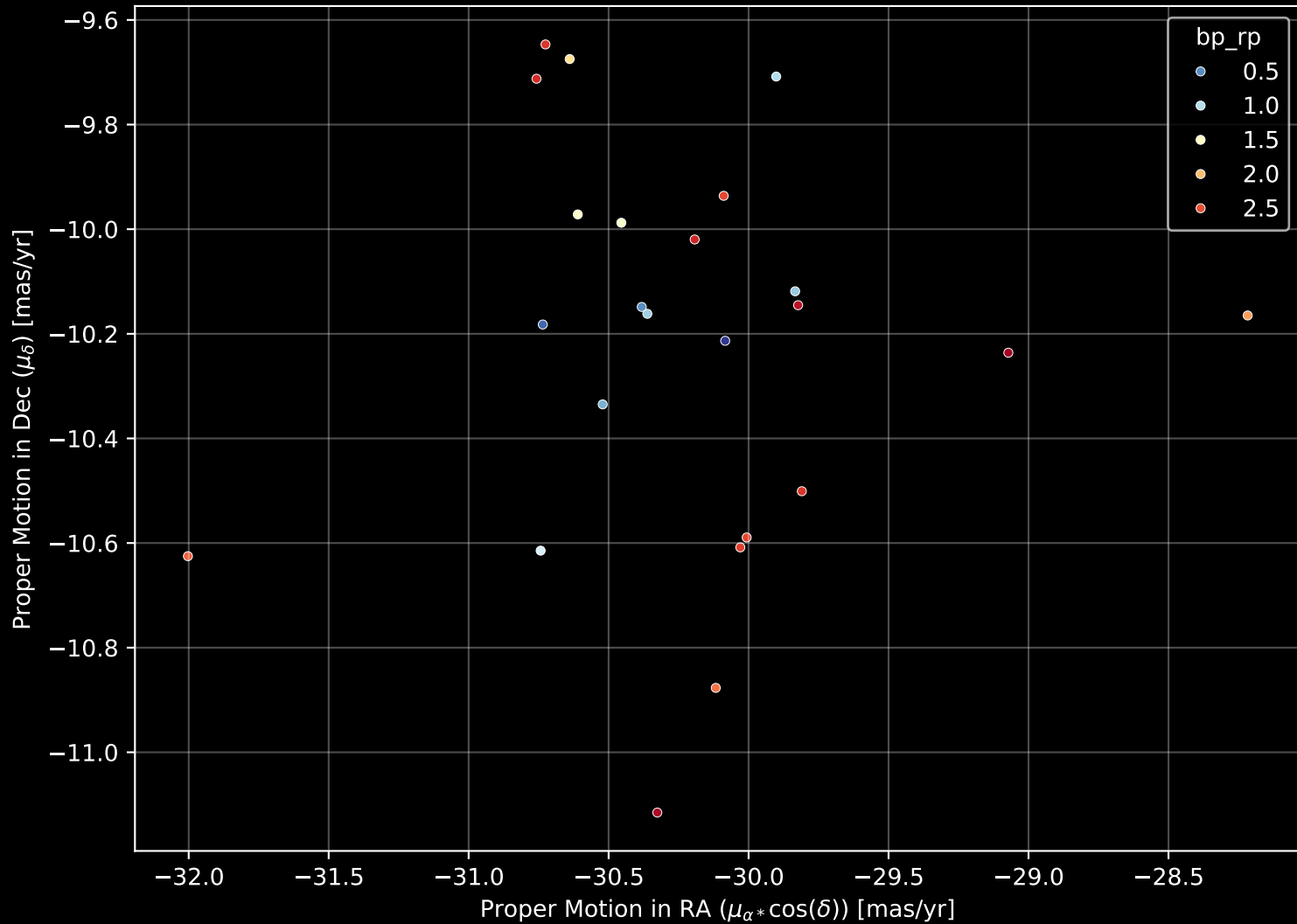
Gaia Cluster: [Platais_10] Proper Motion Diagram (n= 24)
