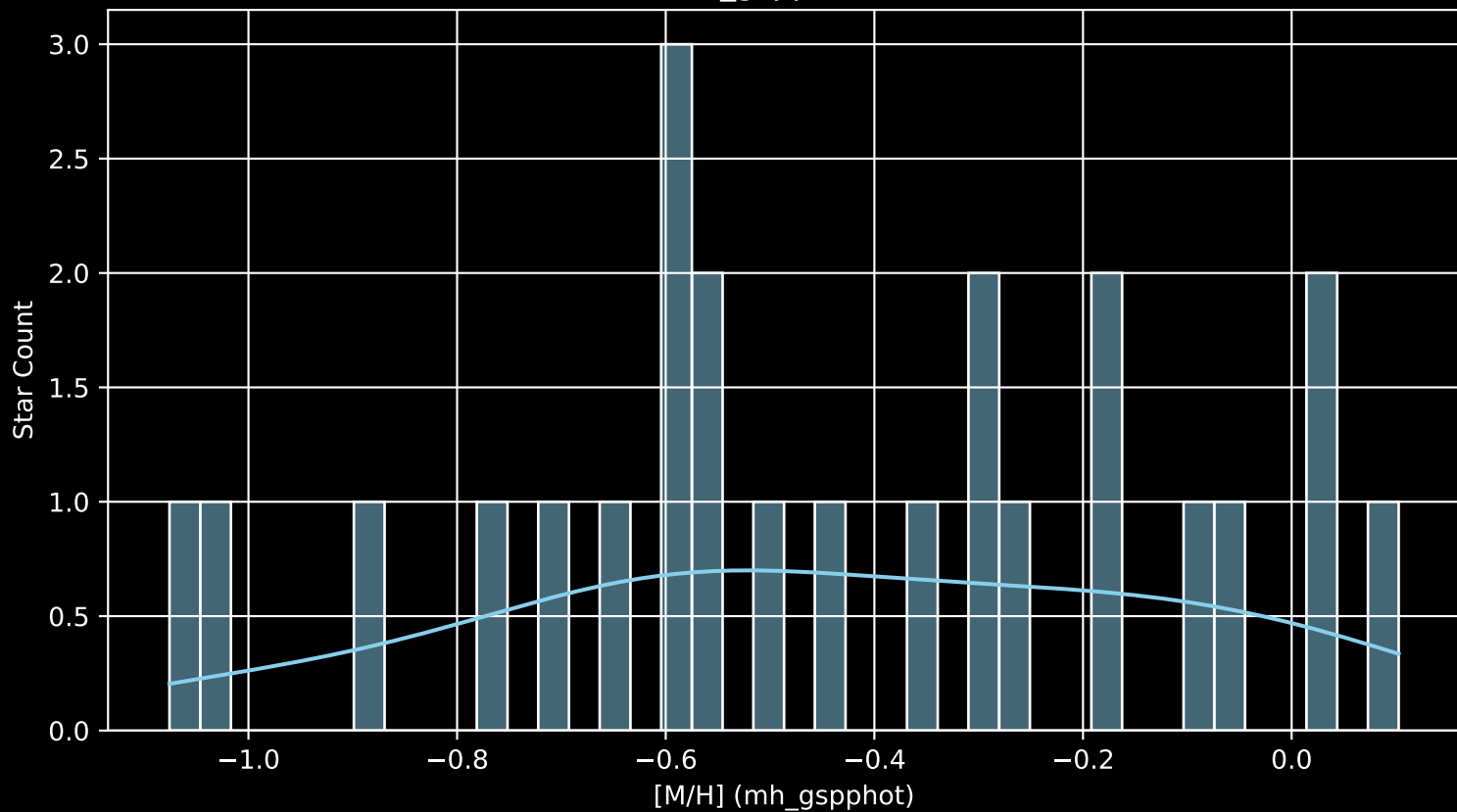
Gaia Cluster: [Platais_10 [M/H] (mh_gspphot) (n= 24)
