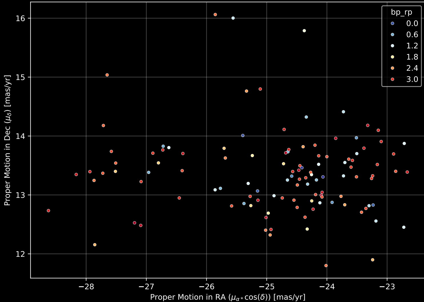
Gaia Cluster: [Platais_9] Proper Motion Diagram (n= 116)
