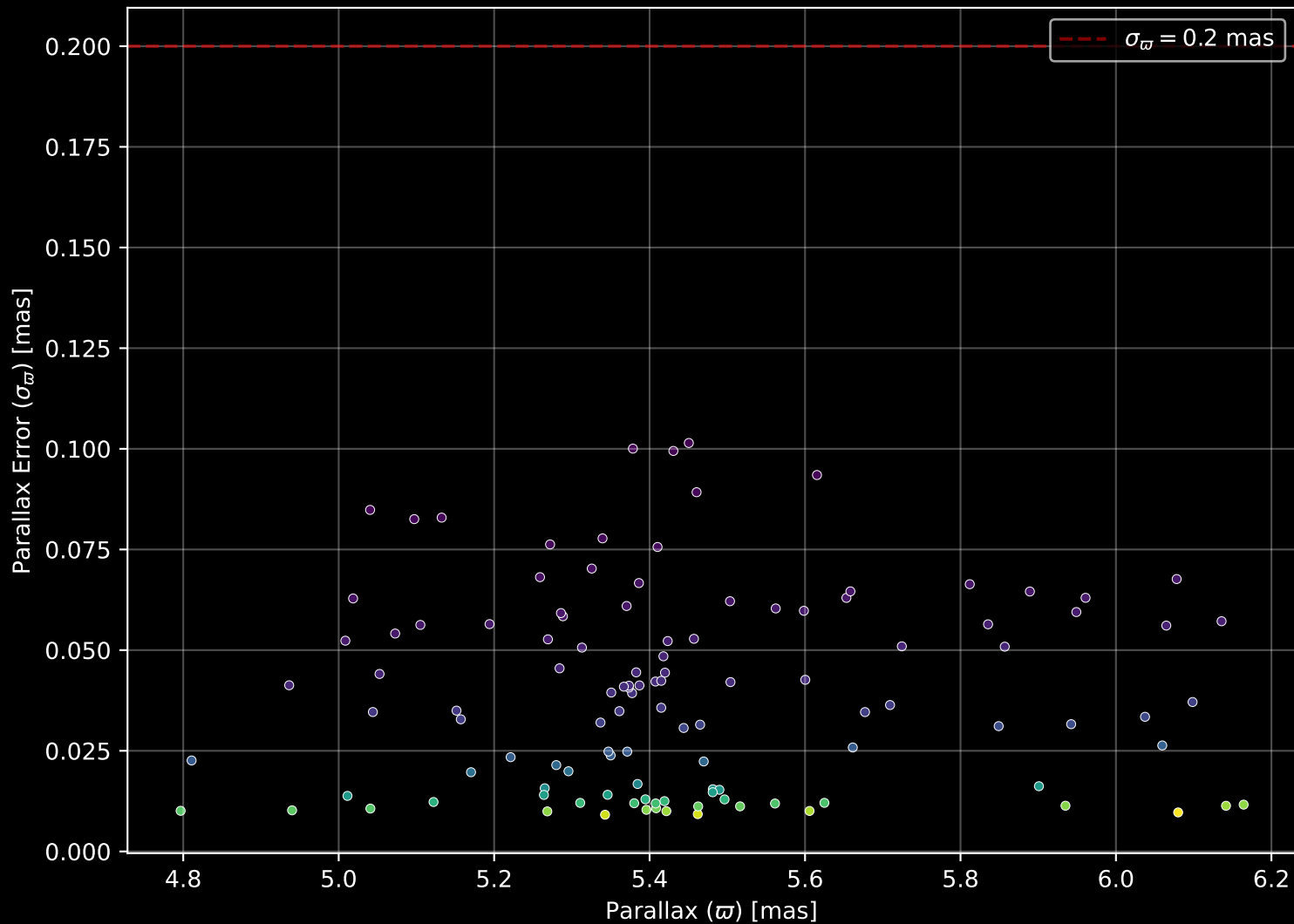
Gaia Cluster: [Platais_9] Parallax Quality (n= 116)
