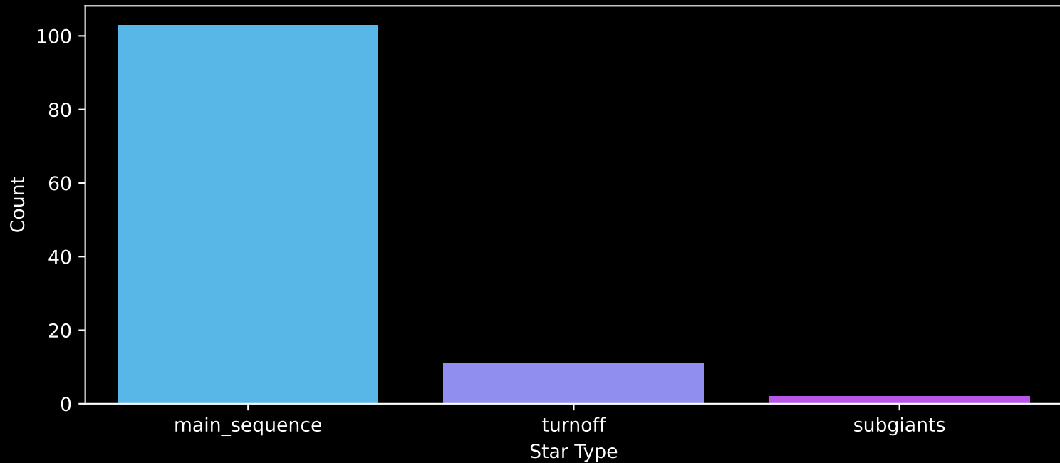
Gaia Cluster: [Platais_9] Count plot of Star Type
