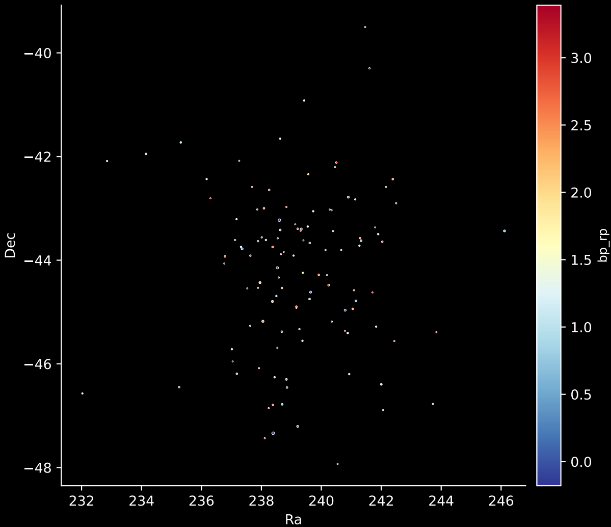
Gaia Cluster: [Platais_9] Stars: 116
