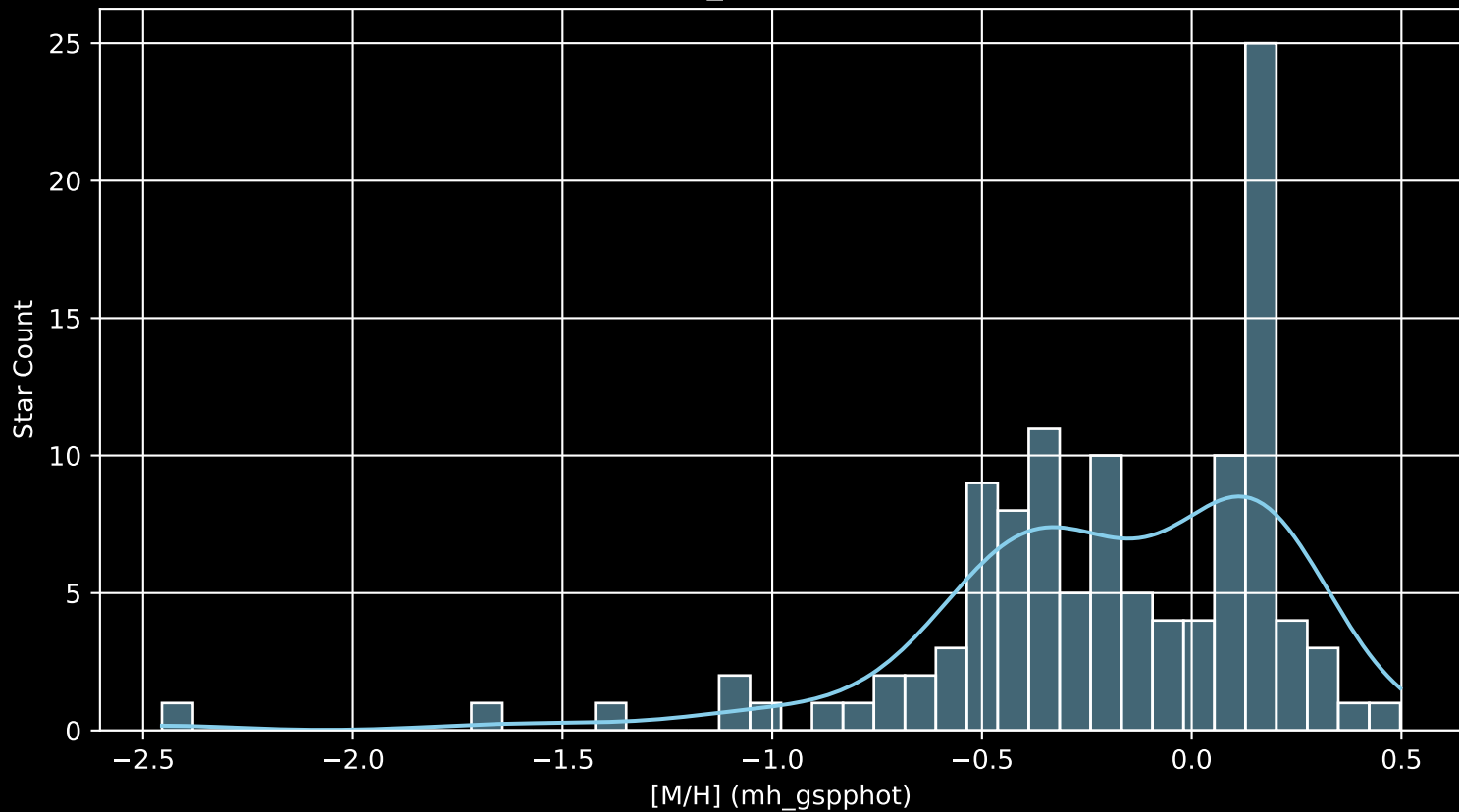
Gaia Cluster: [Platais_9 [M/H] (mh_gspphot) (n= 115)
