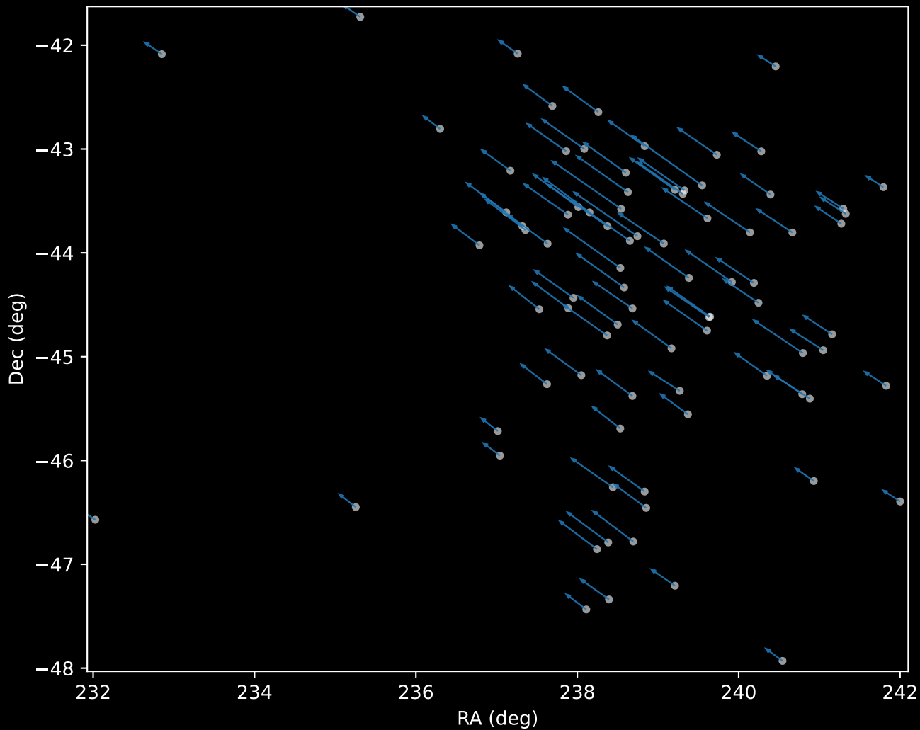
Gaia DR3 Cluster 0 Proper Motion Vectors (n=85)
