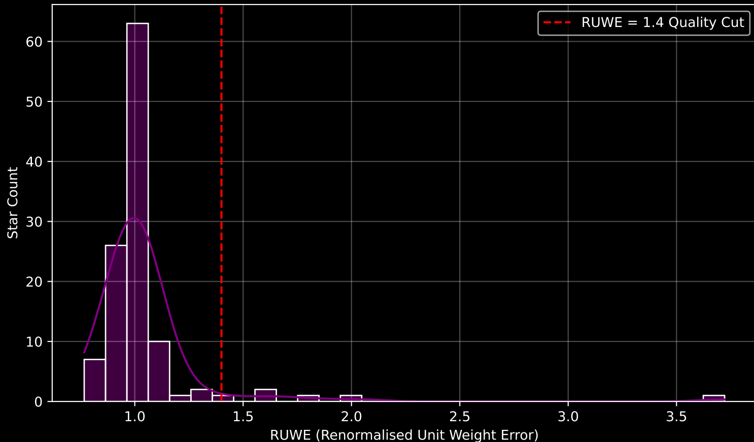
Gaia Cluster: [Platais_9] RUWE Distribution (n= 115)
