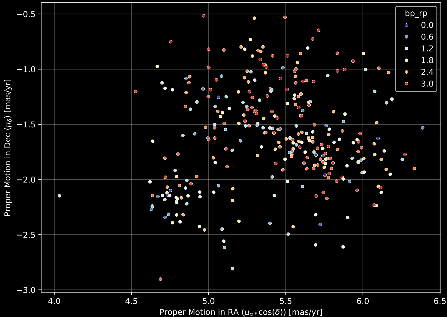
Gaia Cluster: [RSG_8] Proper Motion Diagram (n= 316)
