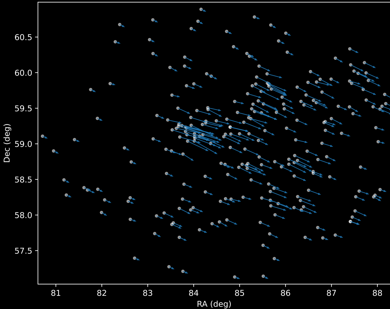
Gaia DR3 Cluster 0 Proper Motion Vectors (n=242)
