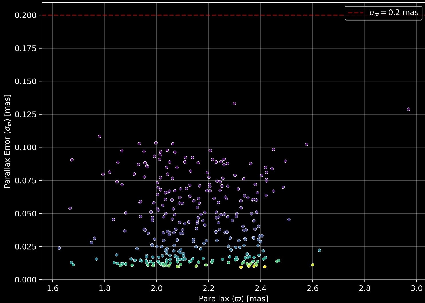
Gaia Cluster: [RSG_8] Parallax Quality (n= 316)
