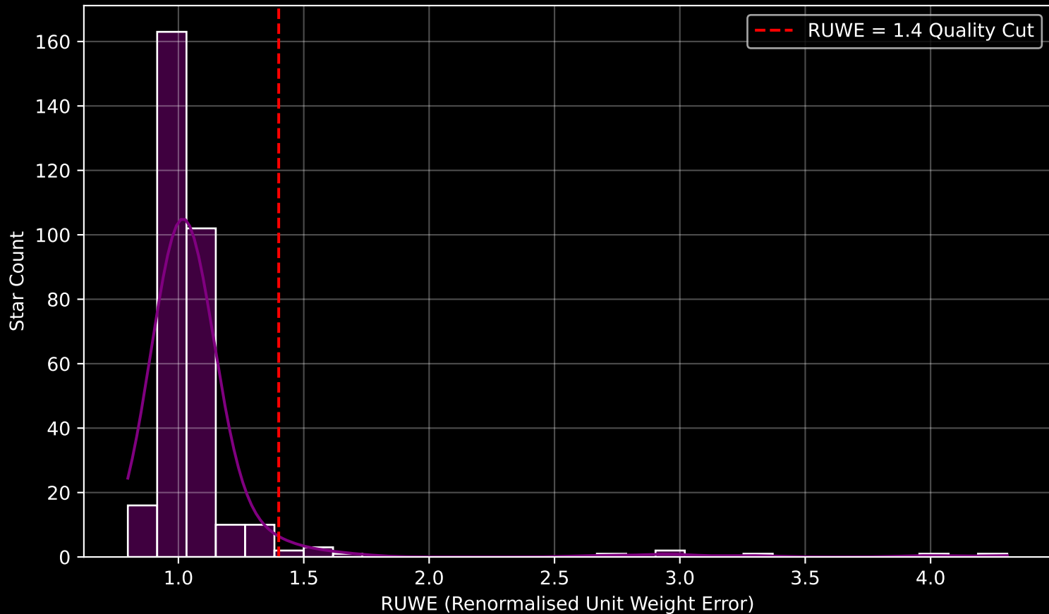
Gaia Cluster: [RSG_8] RUWE Distribution (n= 313)
