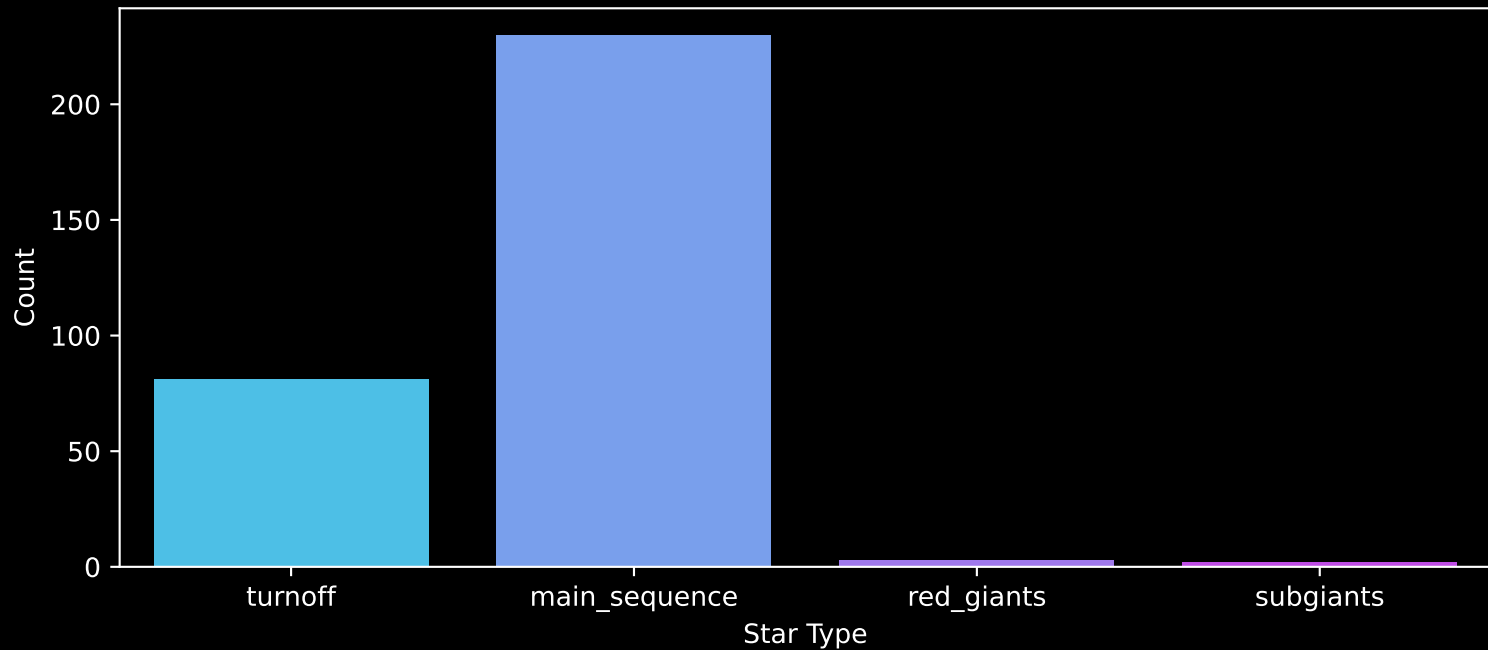
Gaia Cluster: [RSG_8] Count plot of Star Type
