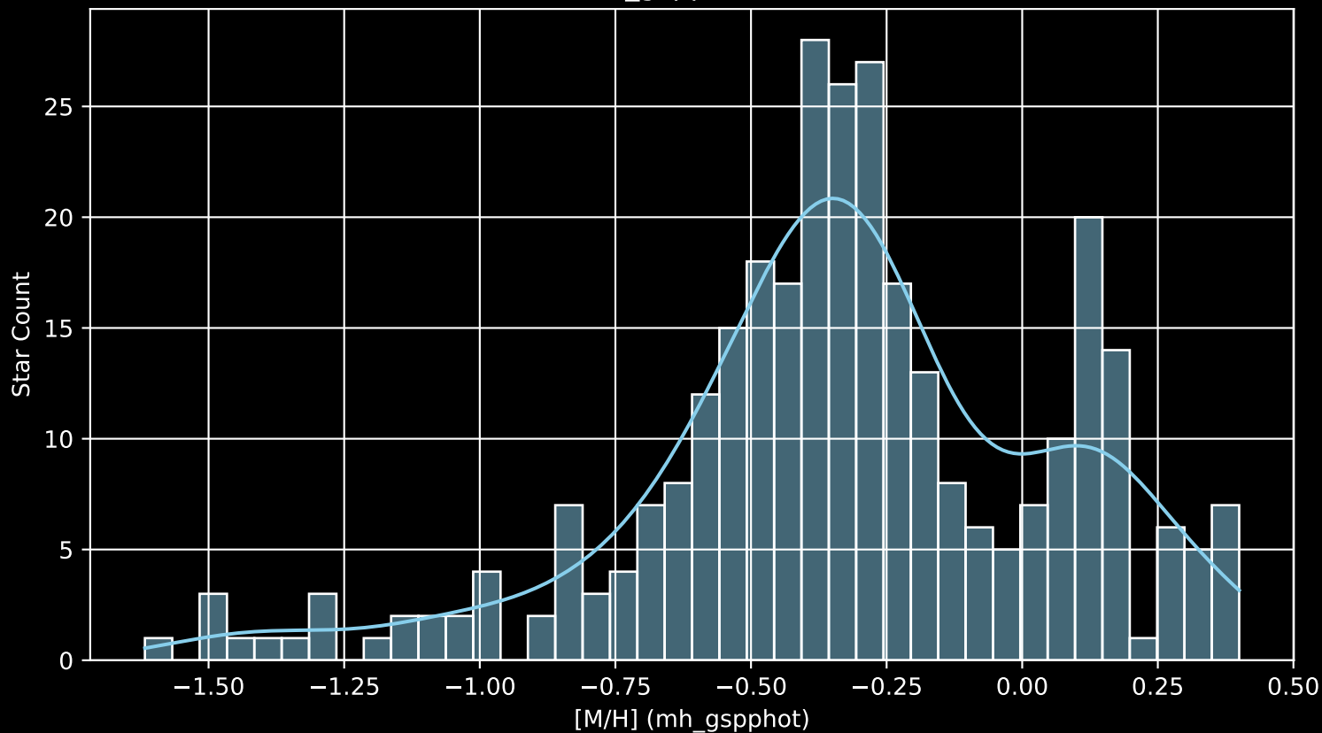
Gaia Cluster: [RSG_8 [M/H] (mh_gspphot) (n= 314)
