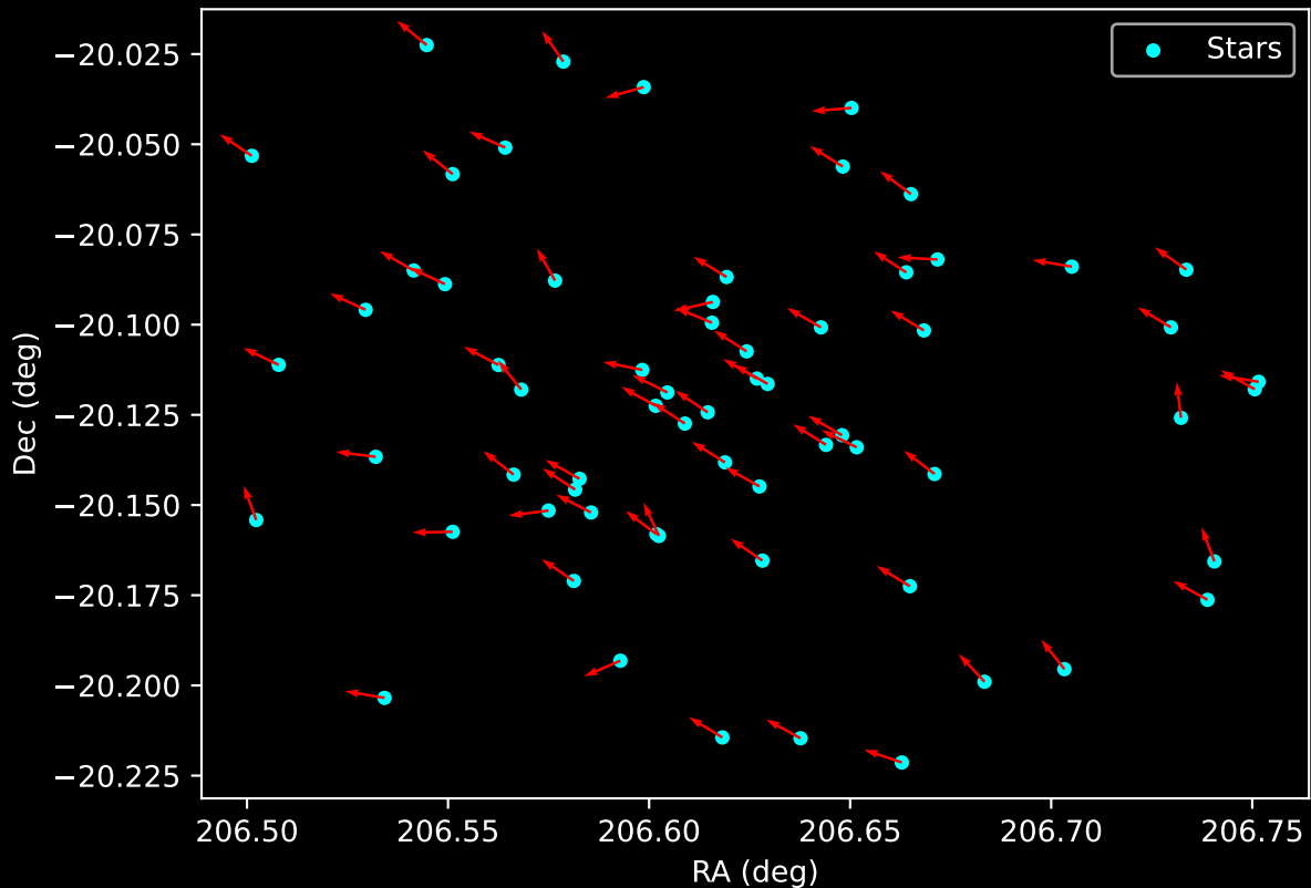
Gaia Cluster: [Ruprecht_10] Proper Motion Vectors for Gaia Star Field (n= 65)
