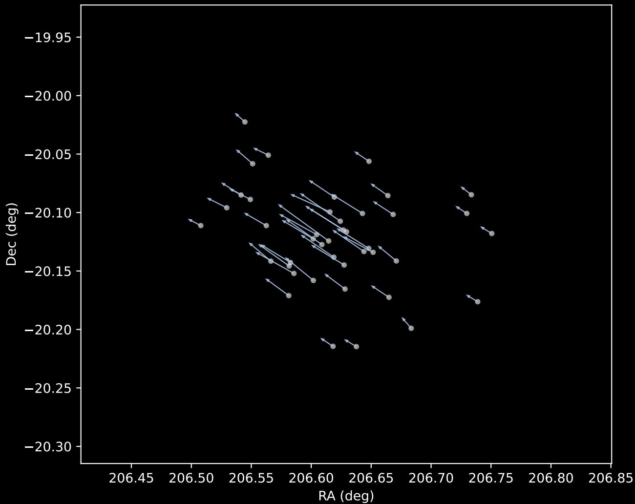
Gaia DR3 Cluster 1 Proper Motion Vectors (n=42)
