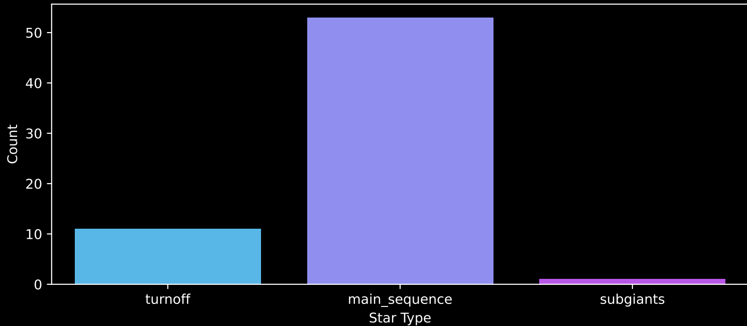
Gaia Cluster: [Ruprecht_10] Count plot of Star Type
