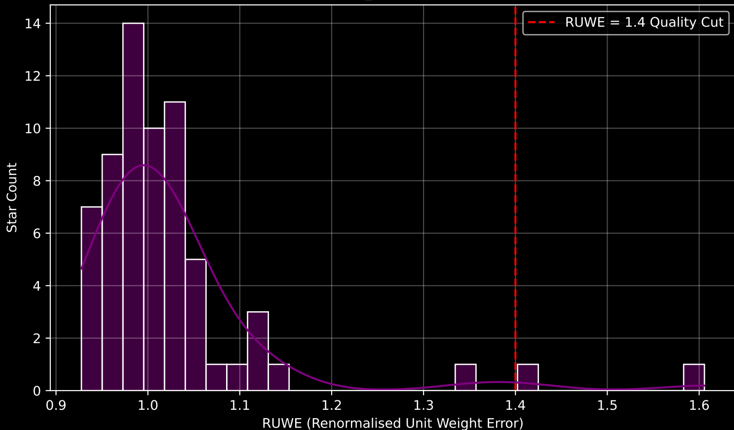
Gaia Cluster: [Ruprecht_10] RUWE Distribution (n= 65)
