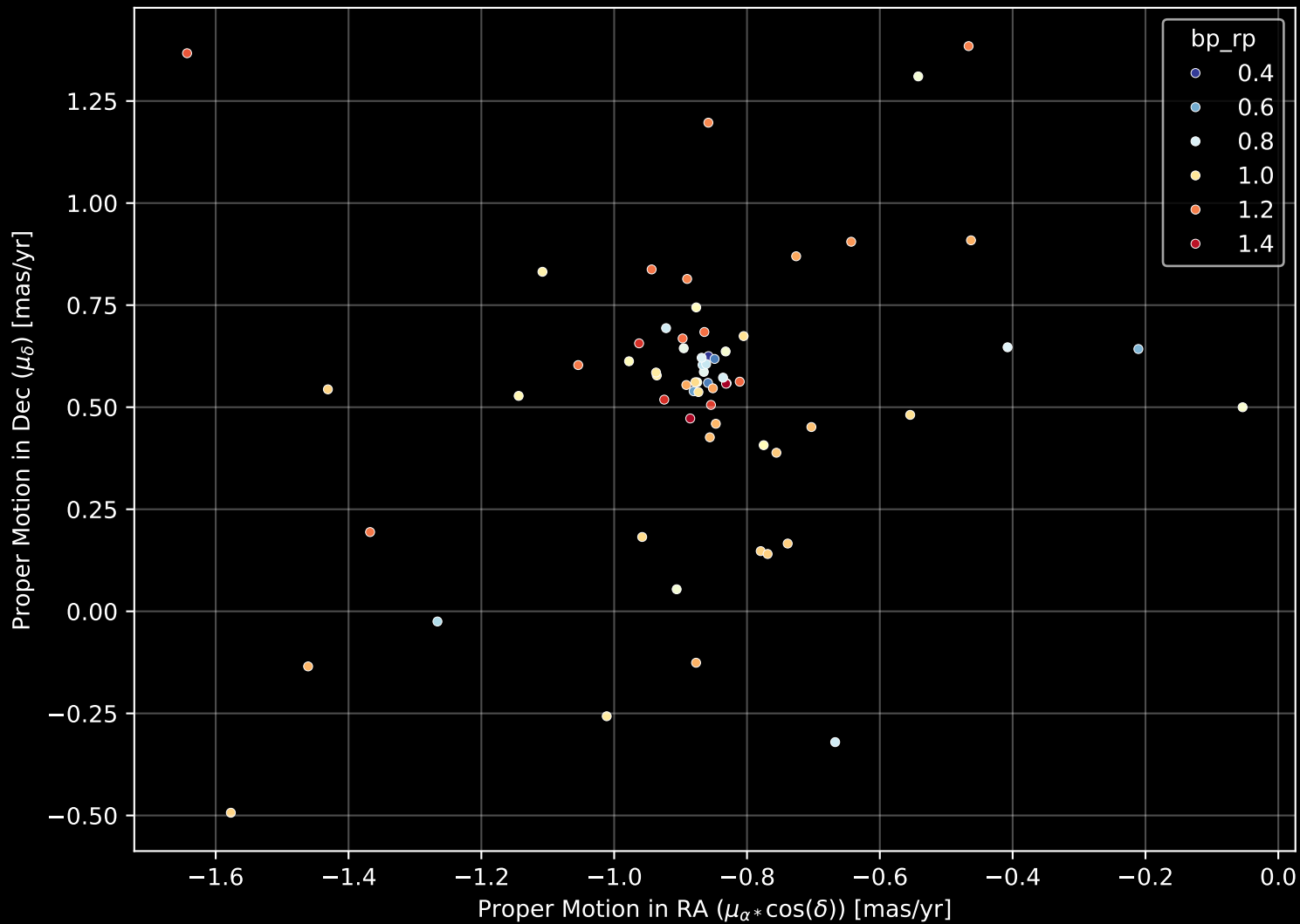
Gaia Cluster: [Ruprecht_10] Proper Motion Diagram (n= 65)
