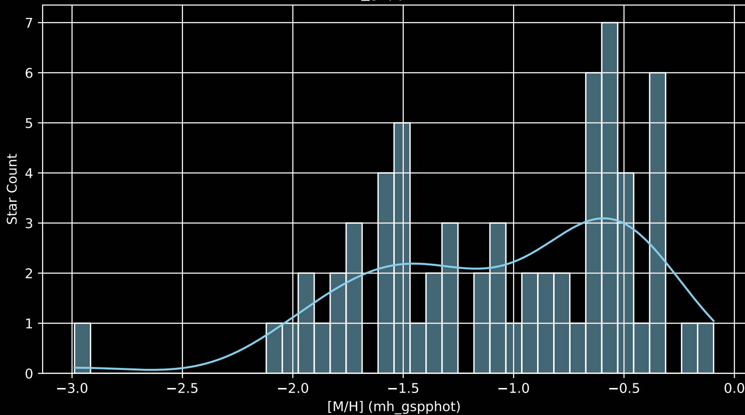
Gaia Cluster: [Ruprecht_10 [M/H] (mh_gspphot) (n= 65)
