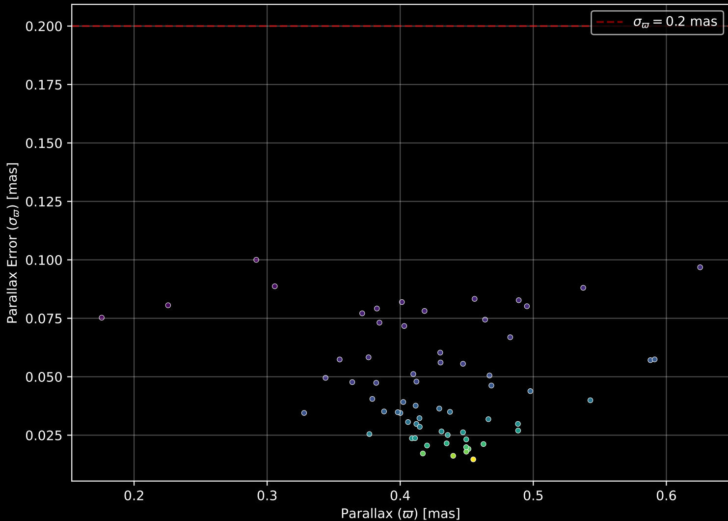
Gaia Cluster: [Ruprecht_10] Parallax Quality (n= 65)
