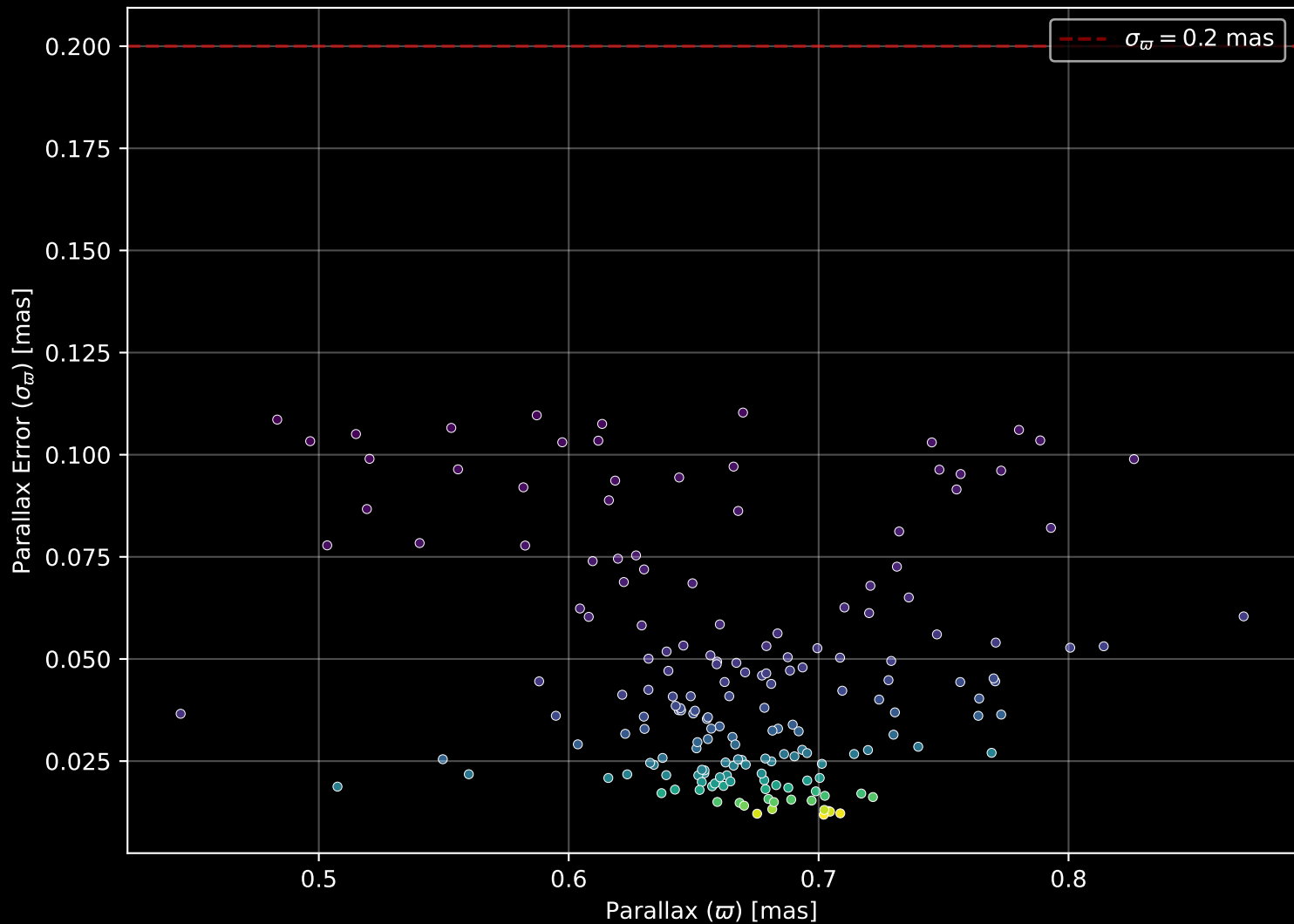
Gaia Cluster: [Ruprecht_111] Parallax Quality (n= 179)
