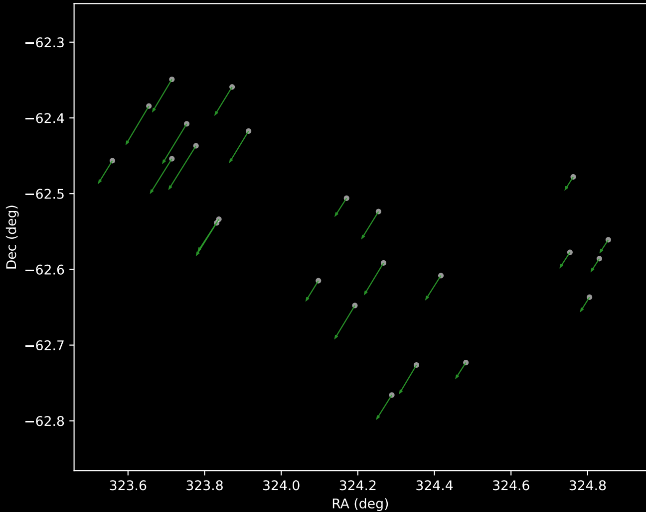
Gaia DR3 Cluster 4 Proper Motion Vectors (n=24)
