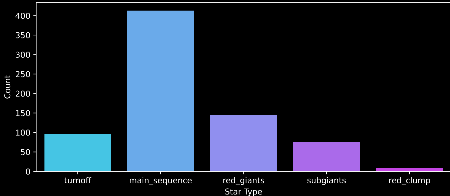
Gaia Cluster: [Ruprecht_112] Count plot of Star Type
