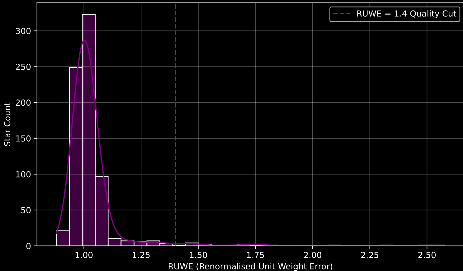
Gaia Cluster: [Ruprecht_112] RUWE Distribution (n= 740)
