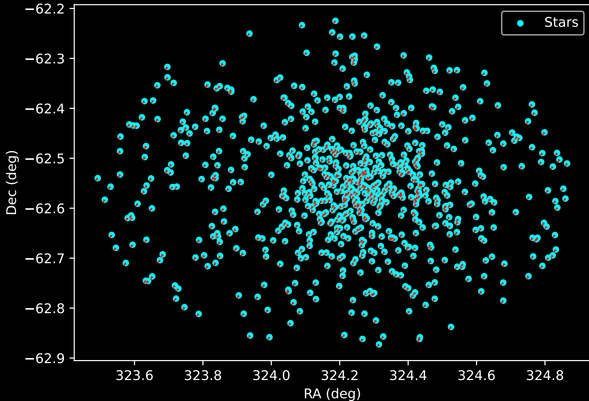
Gaia Cluster: [Ruprecht_112] Proper Motion Vectors for Gaia Star Field (n= 740)
