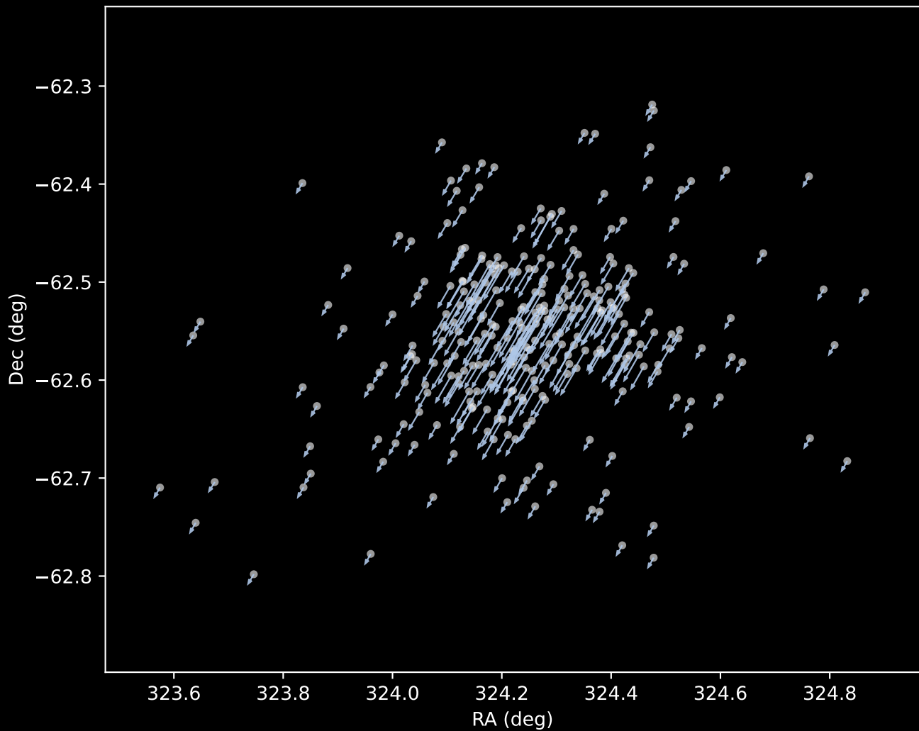
Gaia DR3 Cluster 21 Proper Motion Vectors (n=285)
