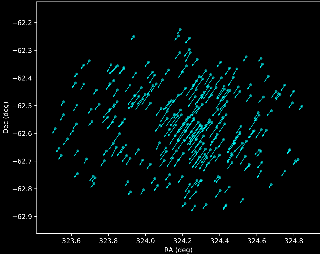
Gaia DR3 Noise Stream Proper Motion Vectors (n=250)
