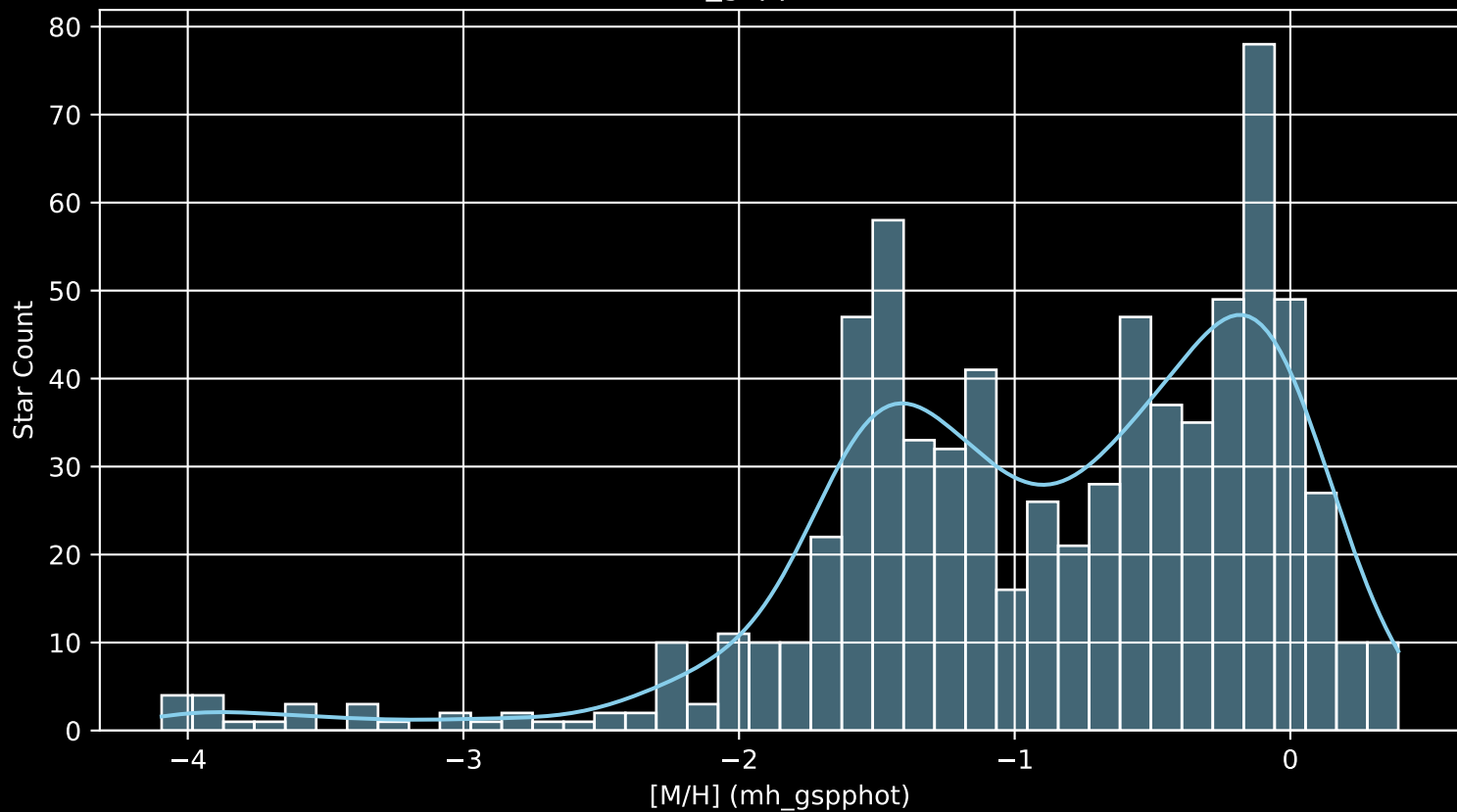
Gaia Cluster: [Ruprecht_112 [M/H] (mh_gspphot) (n= 738)
