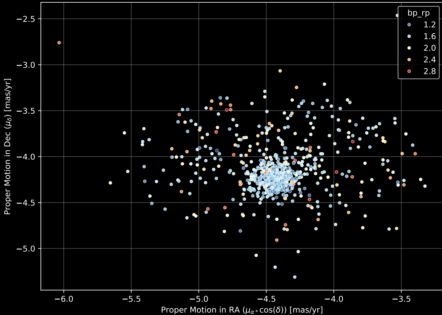
Gaia Cluster: [Ruprecht_112] Proper Motion Diagram (n= 740)
