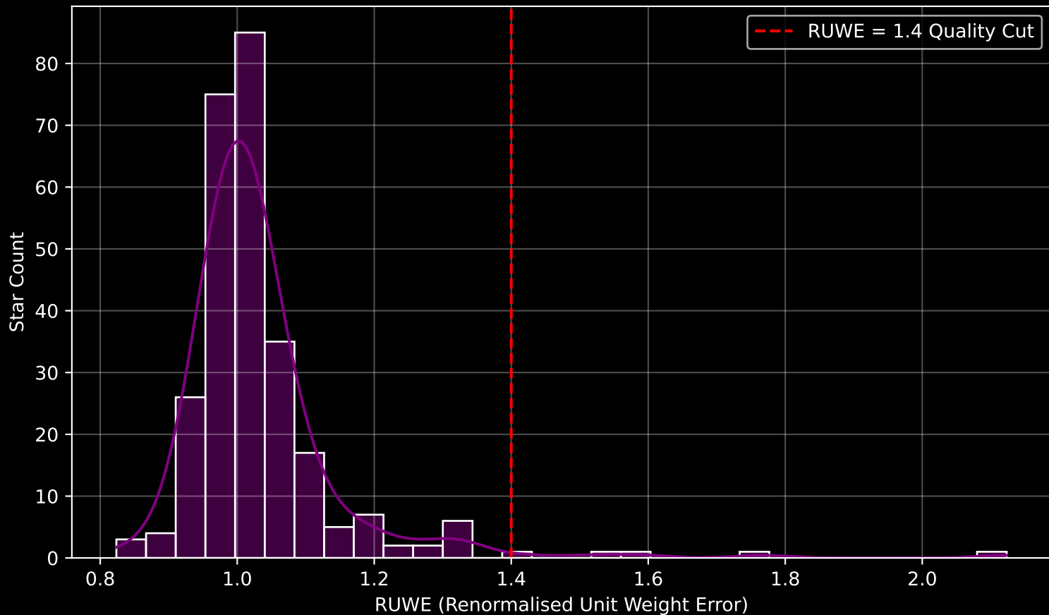
Gaia Cluster: [Ruprecht_117] RUWE Distribution (n= 272)
