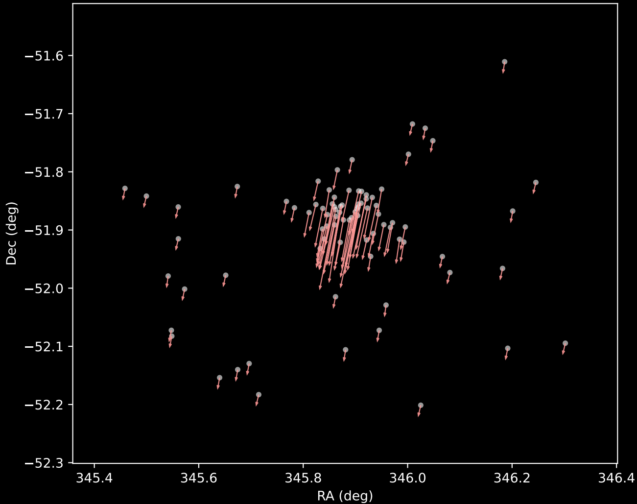
Gaia DR3 Cluster 7 Proper Motion Vectors (n=83)
