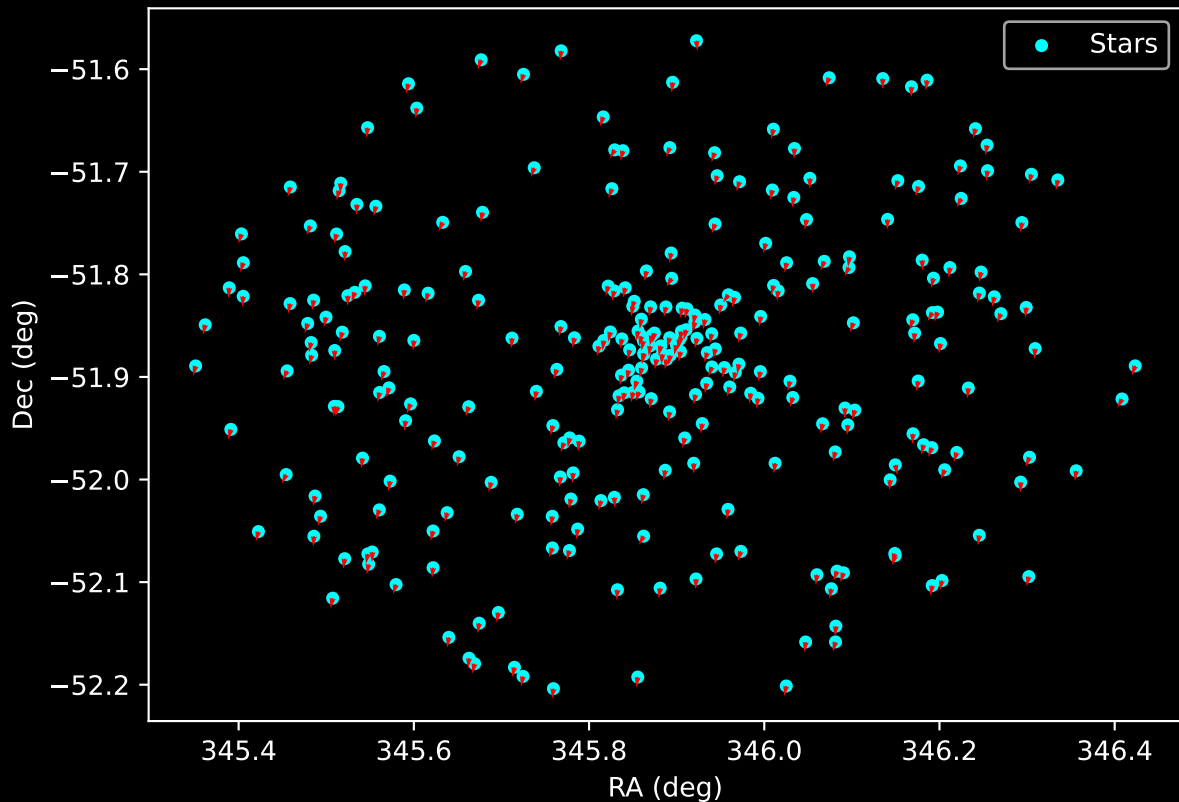
Gaia Cluster: [Ruprecht_117] Proper Motion Vectors for Gaia Star Field (n= 272)
