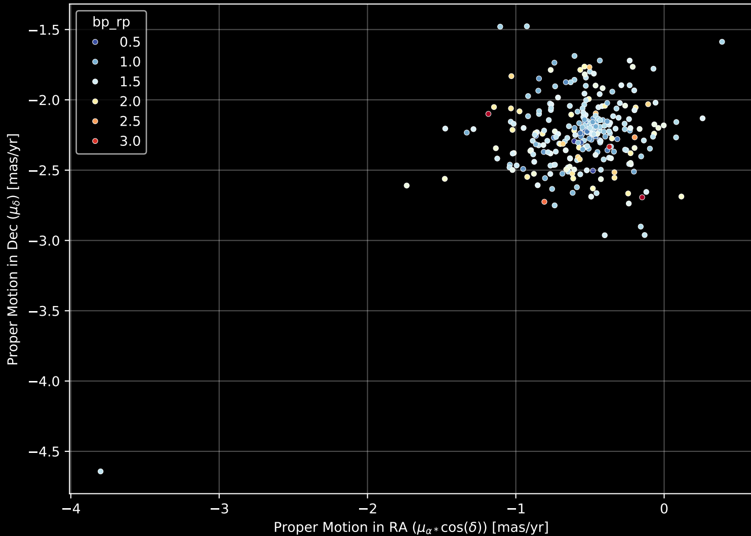
Gaia Cluster: [Ruprecht_117] Proper Motion Diagram (n= 272)
