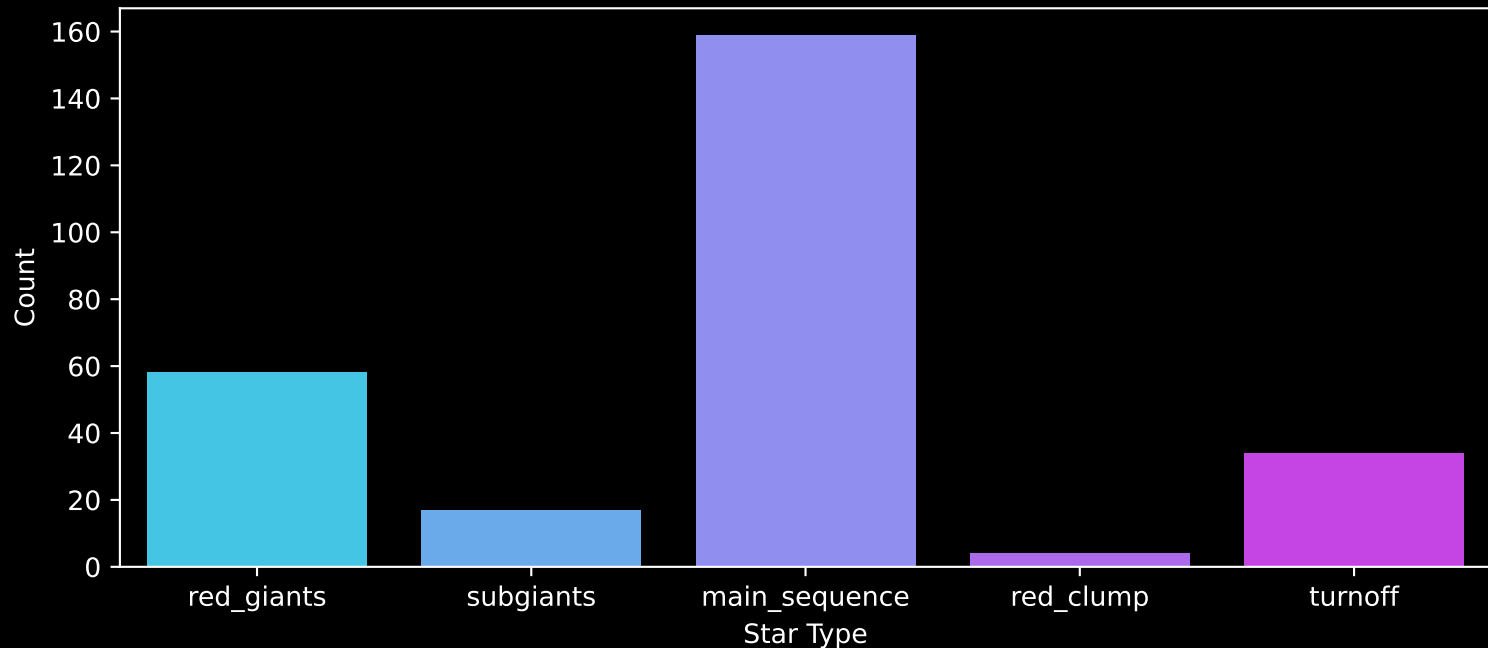
Gaia Cluster: [Ruprecht_117] Count plot of Star Type
