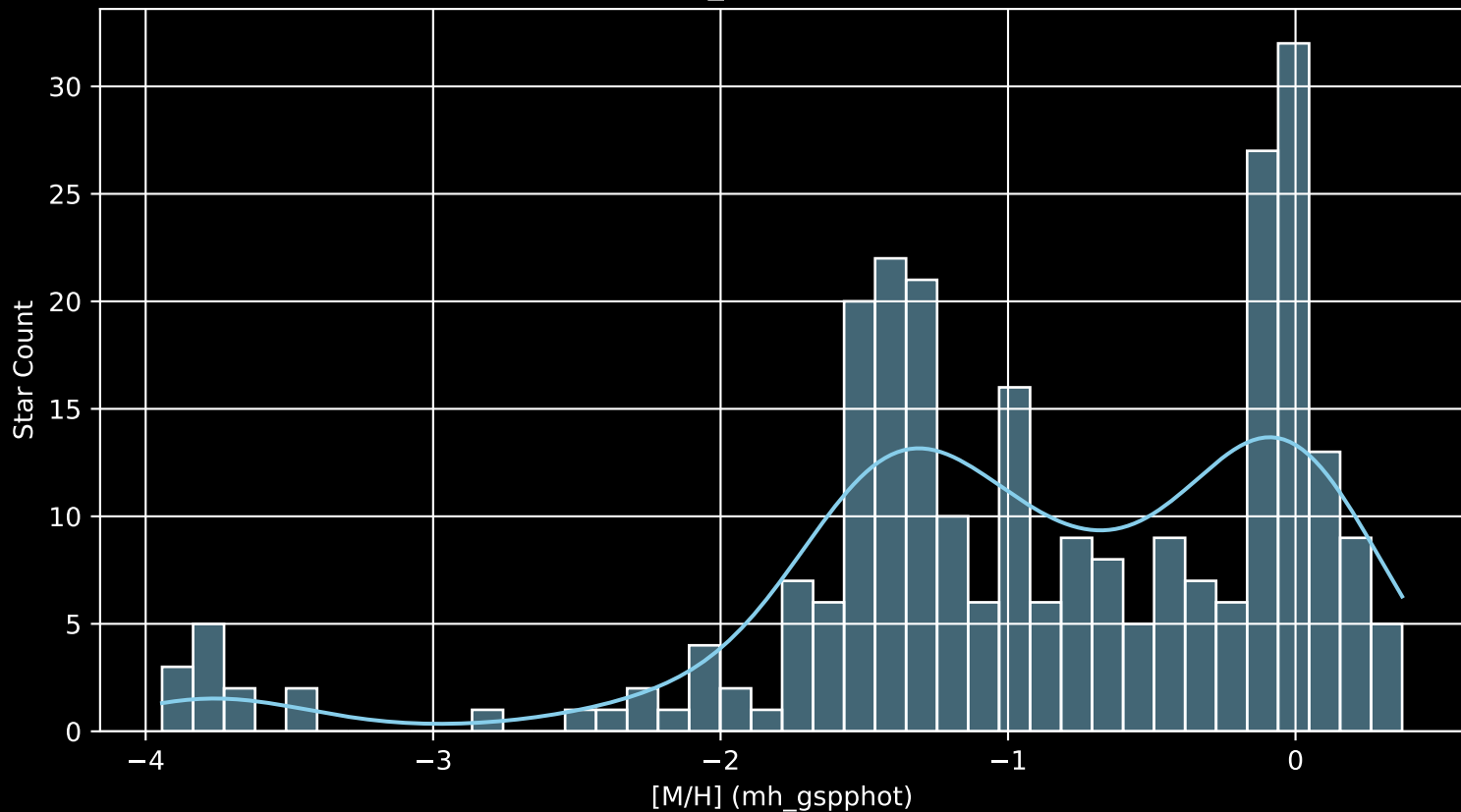
Gaia Cluster: [Ruprecht_117 [M/H] (mh_gspphot) (n= 269)
