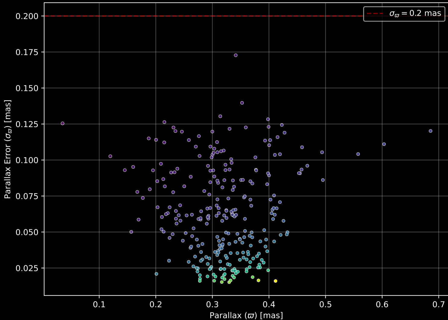
Gaia Cluster: [Ruprecht_117] Parallax Quality (n= 272)
