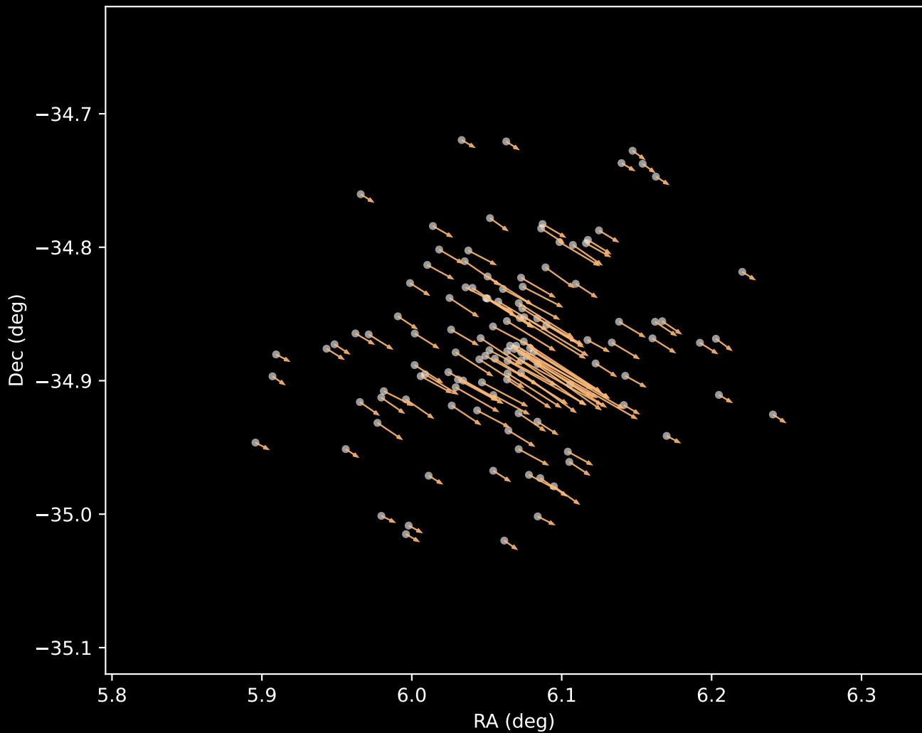
Gaia DR3 Cluster 3 Proper Motion Vectors (n=121)
