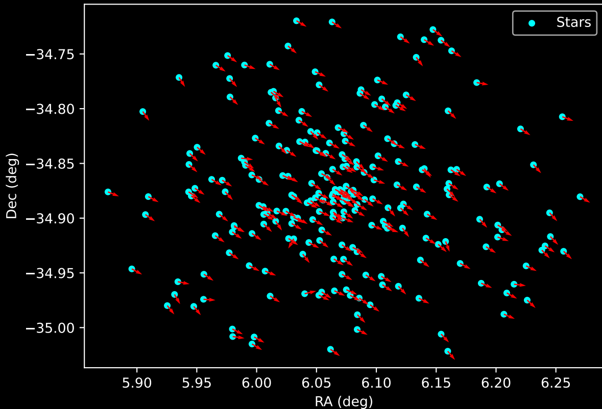
Gaia Cluster: [Ruprecht_128] Proper Motion Vectors for Gaia Star Field (n= 229)
