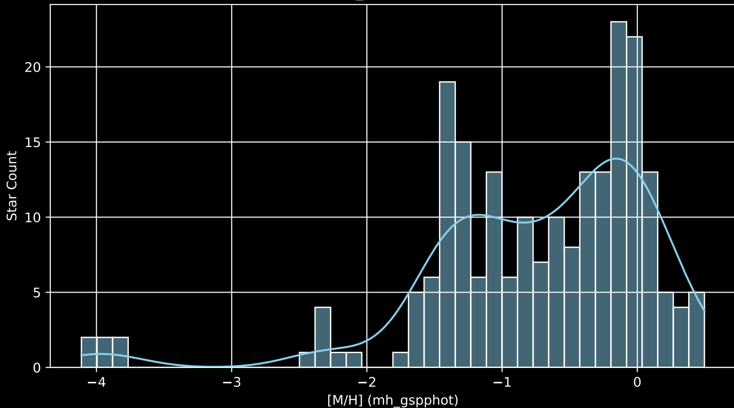
Gaia Cluster: [Ruprecht_128 [M/H] (mh_gspphot) (n= 217)
