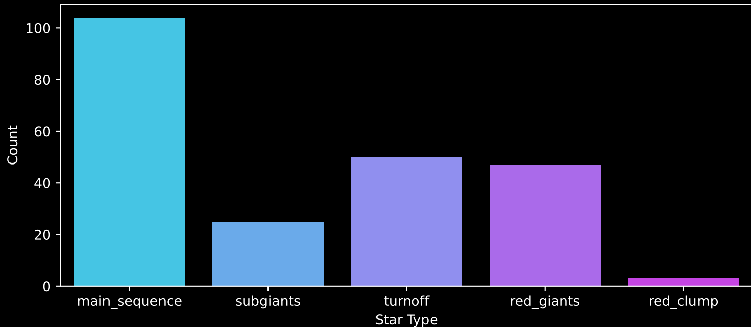
Gaia Cluster: [Ruprecht_128] Count plot of Star Type
