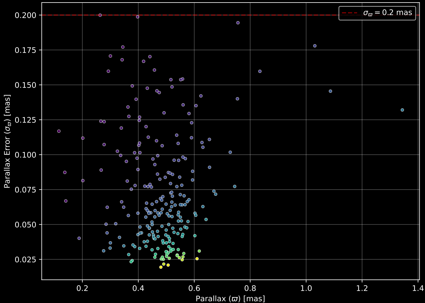
Gaia Cluster: [Ruprecht_128] Parallax Quality (n= 229)
