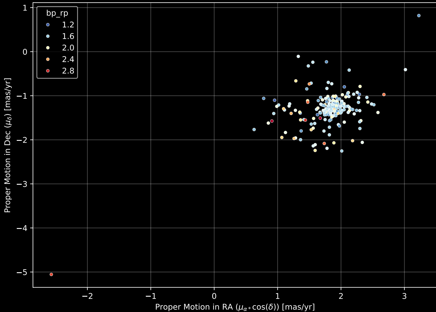
Gaia Cluster: [Ruprecht_128] Proper Motion Diagram (n= 229)
