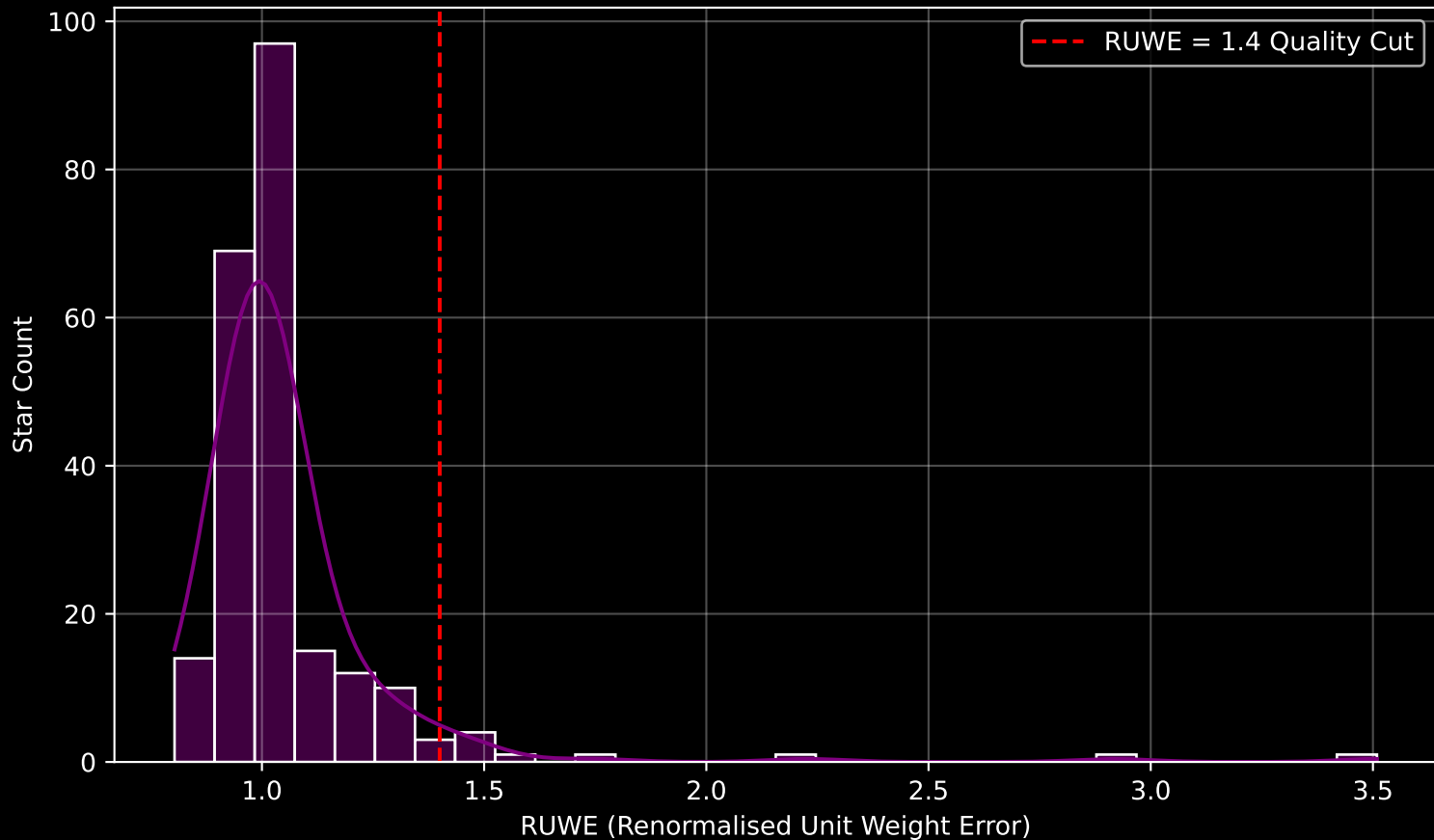
Gaia Cluster: [Ruprecht_128] RUWE Distribution (n= 229)
